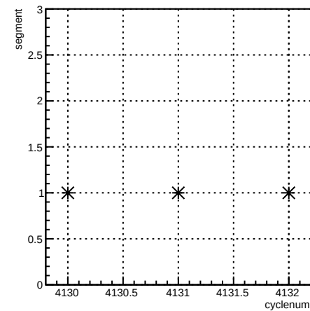
segment:cyclenum {run == 5455}
