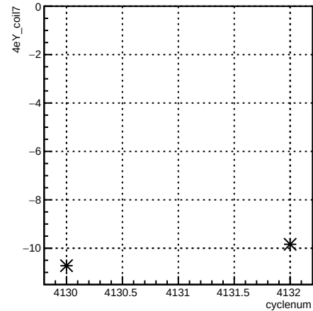
4eY_coil7:cyclenum {run == 5455}
