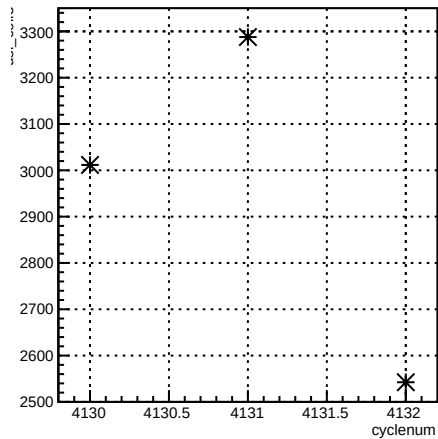
usl_coil7:cyclenum {run == 5455}
