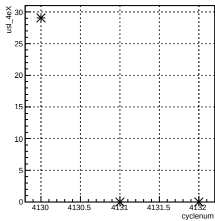
usl_4eX:cyclenum {run == 5455}
