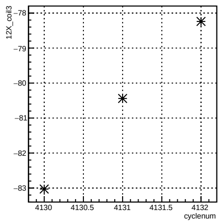
12X_coil3:cyclenum {run == 5455}
