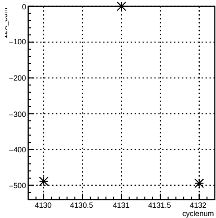
12X_coil7:cyclenum {run == 5455}
