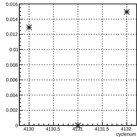
delta46_12X4eY:cyclenum {run == 5455}
