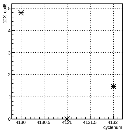
12X_coil6:cyclenum {run == 5455}
