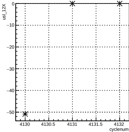
usl_12X:cyclenum {run == 5455}
