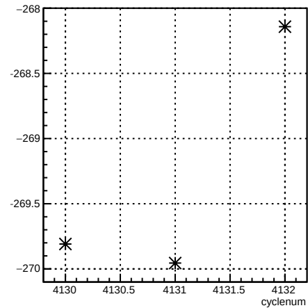
4eX_coil1:cyclenum {run == 5455}
