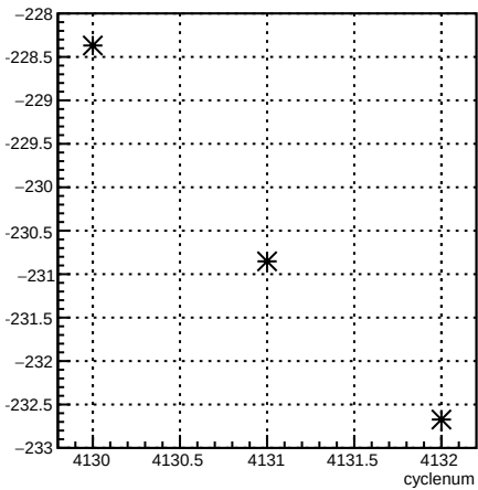
12X_coil1:cyclenum {run == 5455}
