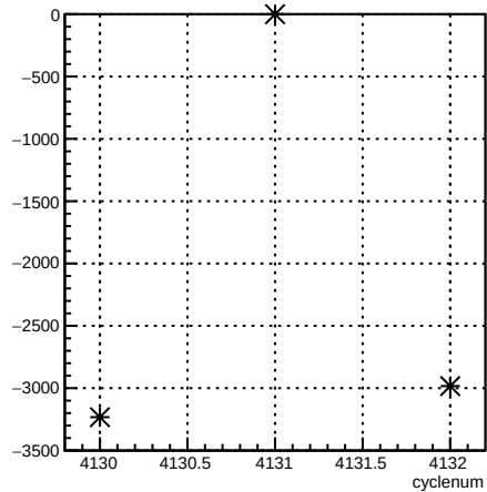
usr_coil6:cyclenum {run == 5455}
