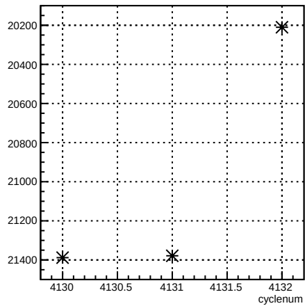
usr_coil6:cyclenum {run == 5455}
