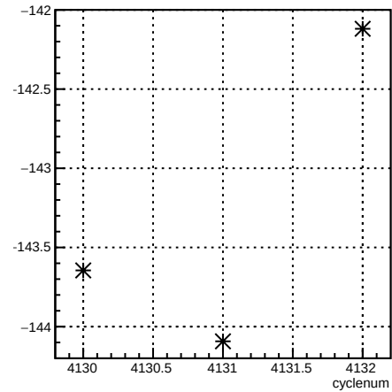
1X_coil1:cyclenum {run == 5455}
