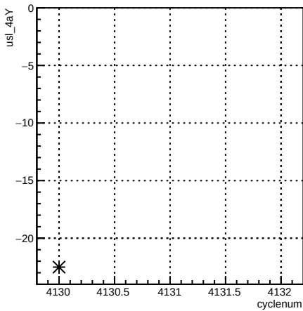
usl_4aY:cyclenum {run == 5455}
