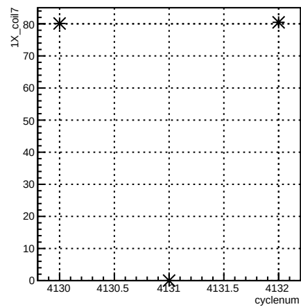
1X_coil7:cyclenum {run == 5455}
