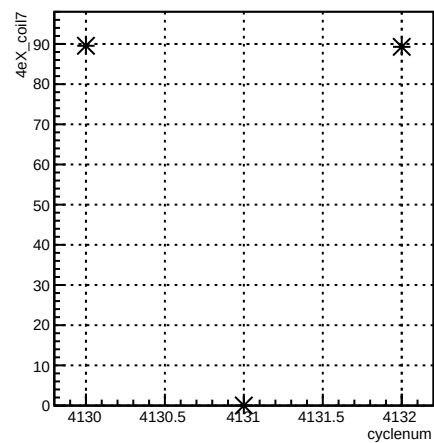
4eX_coil7:cyclenum {run == 5455}
