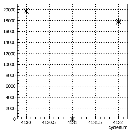
usl_coil7:cyclenum {run == 5455}
