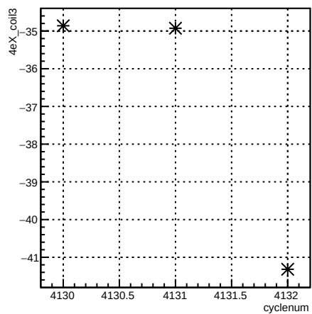
4eX_coil3:cyclenum {run == 5455}
