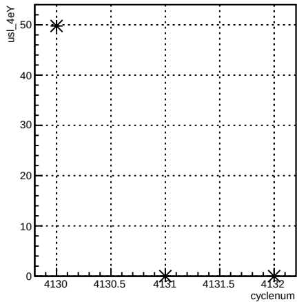
usl_4eY:cyclenum {run == 5455}
