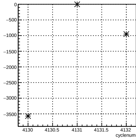
usl_coil6:cyclenum {run == 5455}
