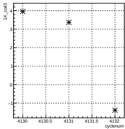
1X_coil3:cyclenum {run == 5455}
