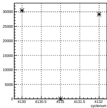
usr_coil7:cyclenum {run == 5455}
