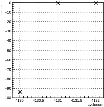
usl_1X:cyclenum {run == 5455}
