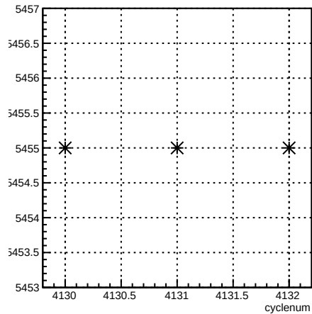
run:cyclenum {run == 5455}
