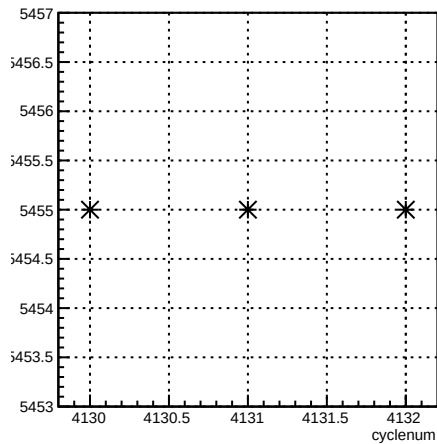
run:cyclenum {run == 5455}
