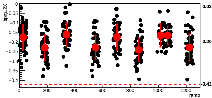
bmod_trim2,cyc=4130
