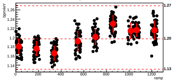
bmod_trim6,cyc=4130
