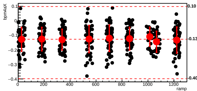
bmod_trim6,cyc=4130
