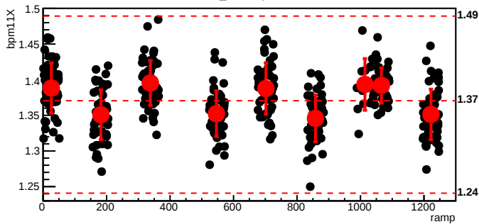
bmod_trim2,cyc=4130
