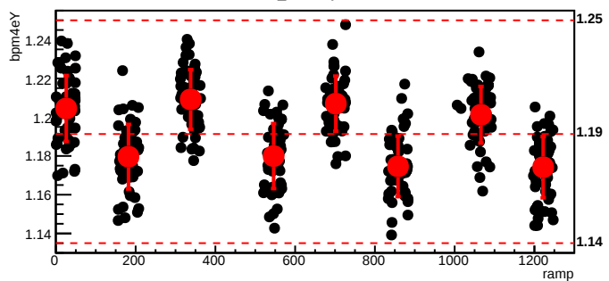
bmod_trim3,cyc=4130
