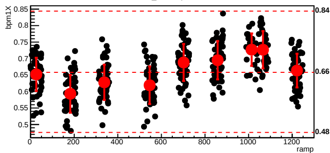
bmod_trim1,cyc=4130
