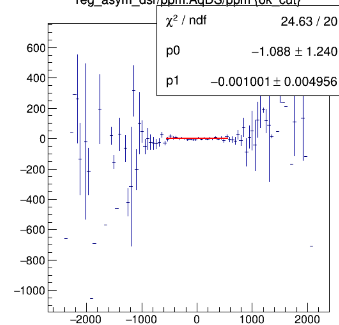
reg_asym_dsr/ppm:AqDS/ppm {ok_cut}
