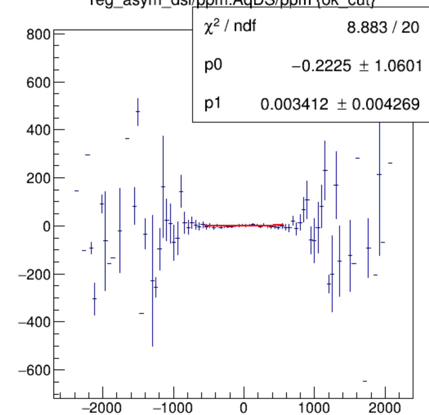
reg_asym_dsl/ppm:AqDS/ppm {ok_cut}
