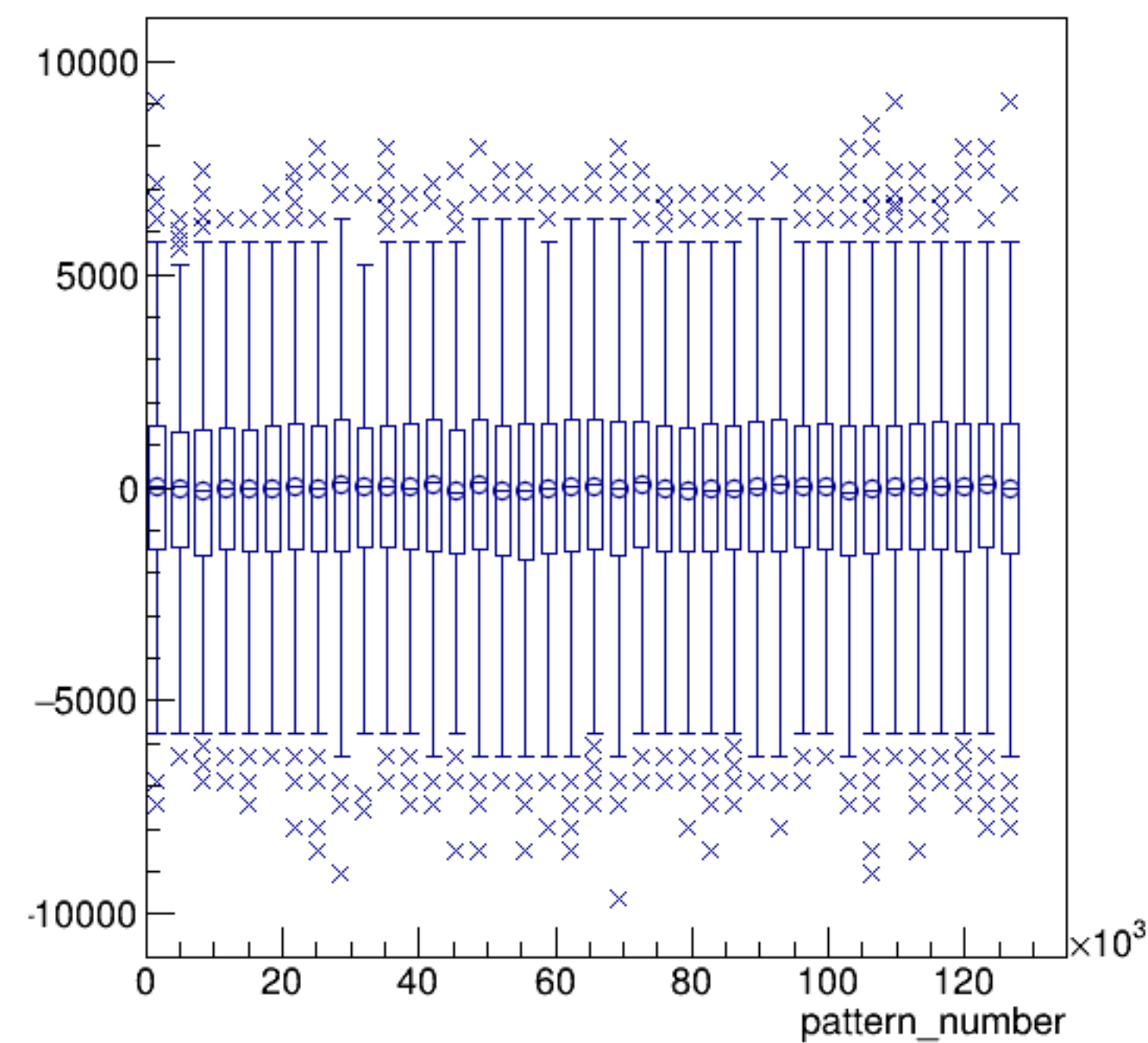
asym_sam4/ppm:pattern_number {ErrorFlag==0}
