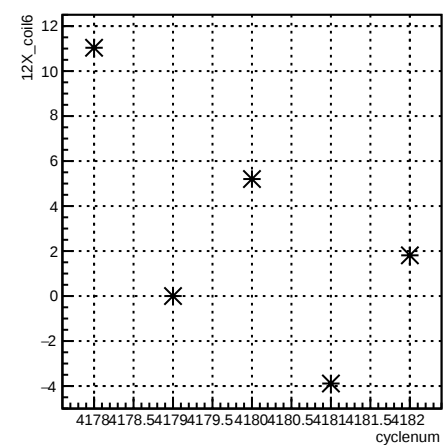
12X_coil6:cyclenum {run == 5465}
