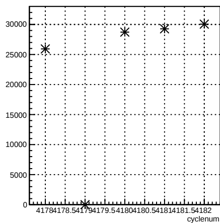
usr_coil7:cyclenum {run == 5465}
