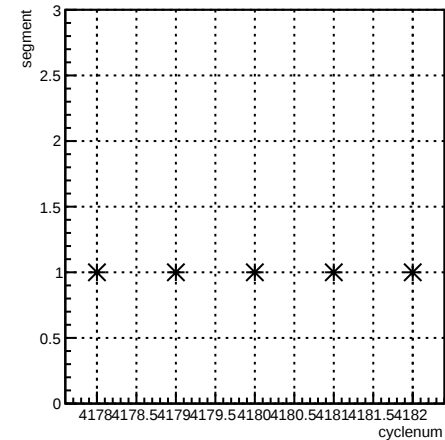
segment:cyclenum {run == 5465}
