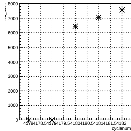
usl_coil4:cyclenum {run == 5465}
