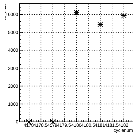
usr_coil4:cyclenum {run == 5465}
