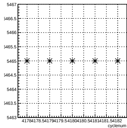
run:cyclenum {run == 5465}
