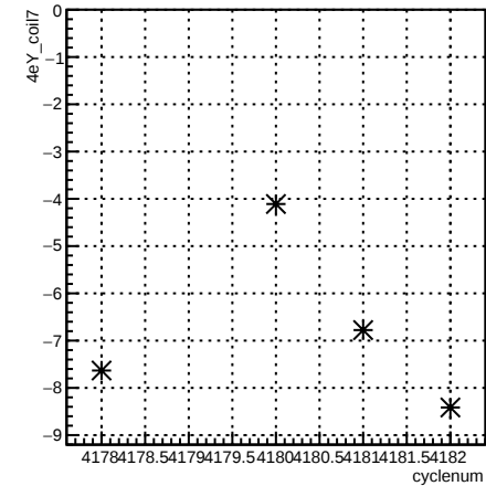
4eY_coil7:cyclenum {run == 5465}
