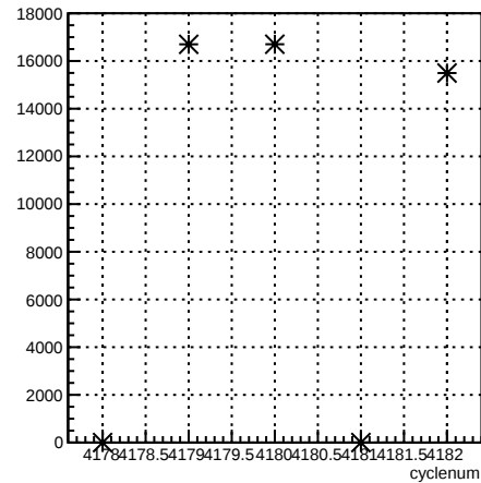
usl_coil1:cyclenum {run == 5465}
