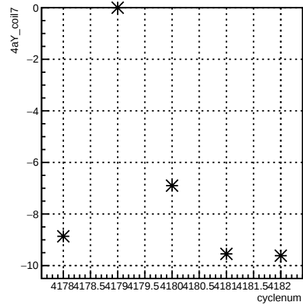
4aY_coil7:cyclenum {run == 5465}
