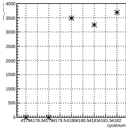
usl_coil3:cyclenum {run == 5465}
