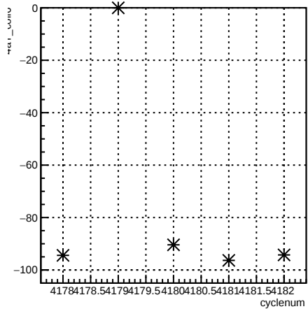
4aY_coil6:cyclenum {run == 5465}
