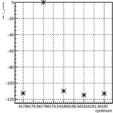
4eY_coil6:cyclenum {run == 5465}
