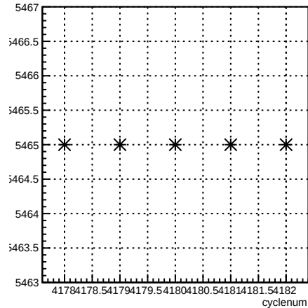
run:cyclenum {run == 5465}
