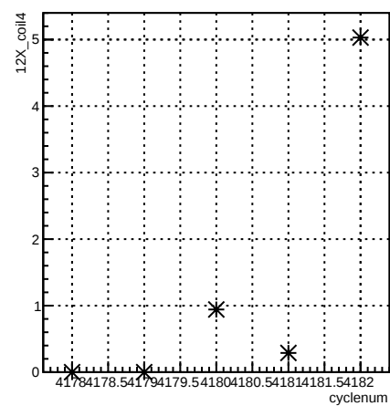
12X_coil4:cyclenum {run == 5465}
