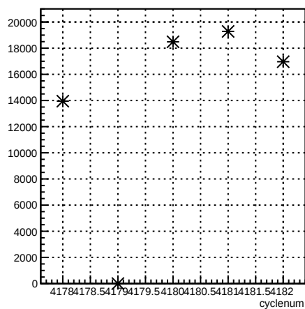
usl_coil7:cyclenum {run == 5465}
