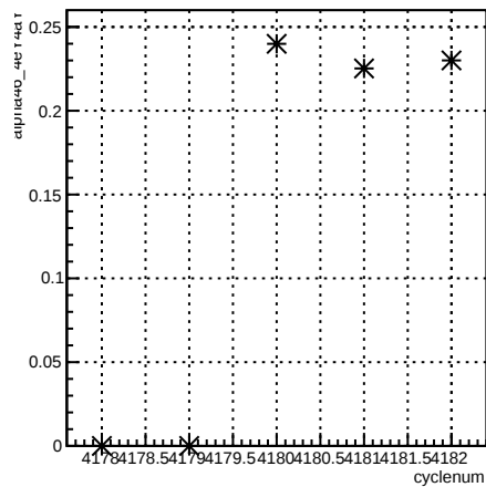
alpha46_4eY4aY:cyclenum {run == 5465}
