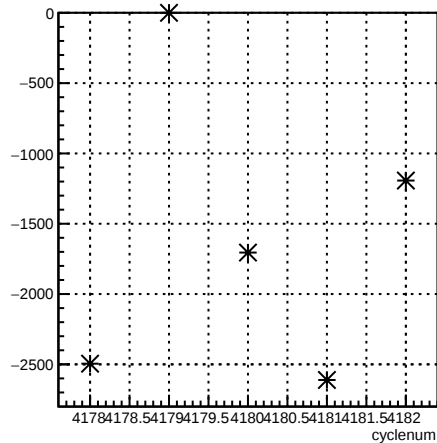
usr_coil6:cyclenum {run == 5465}
