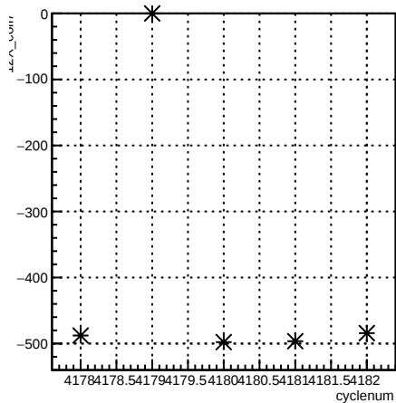
12X_coil7:cyclenum {run == 5465}
