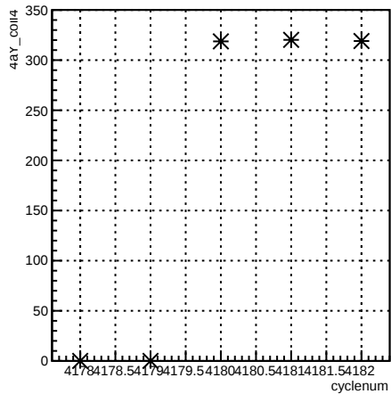
4aY_coil4:cyclenum {run == 5465}
