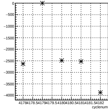
usl_coil6:cyclenum {run == 5465}
