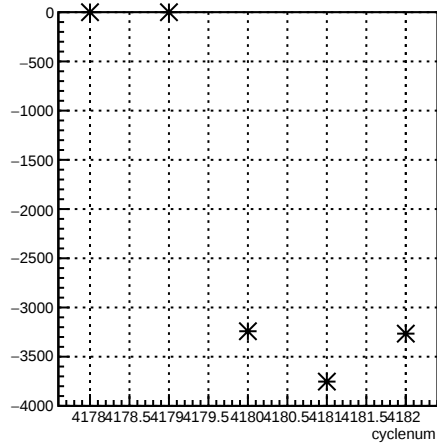
usr_coil3:cyclenum {run == 5465}
