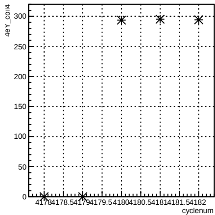
4eY_coil4:cyclenum {run == 5465}
