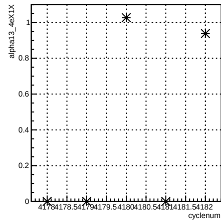
alpha13_4eX1X:cyclenum {run == 5465}
