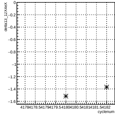
delta13_12X4eX:cyclenum {run == 5465}
