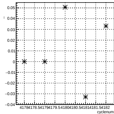
delta46_12X4eY:cyclenum {run == 5465}
