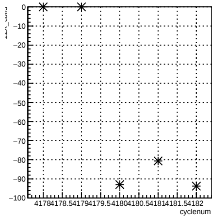
12X_coil3:cyclenum {run == 5465}
