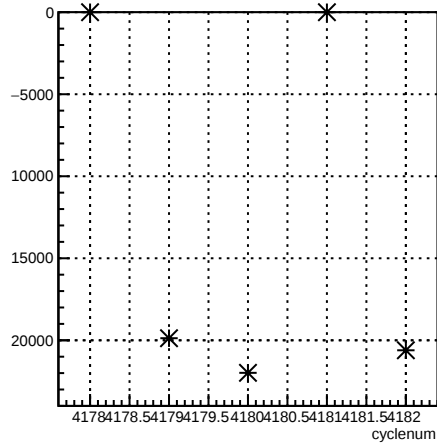
usr_coil1:cyclenum {run == 5465}
