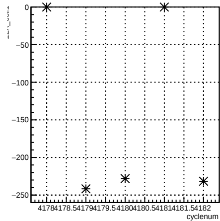
12X_coil1:cyclenum {run == 5465}
