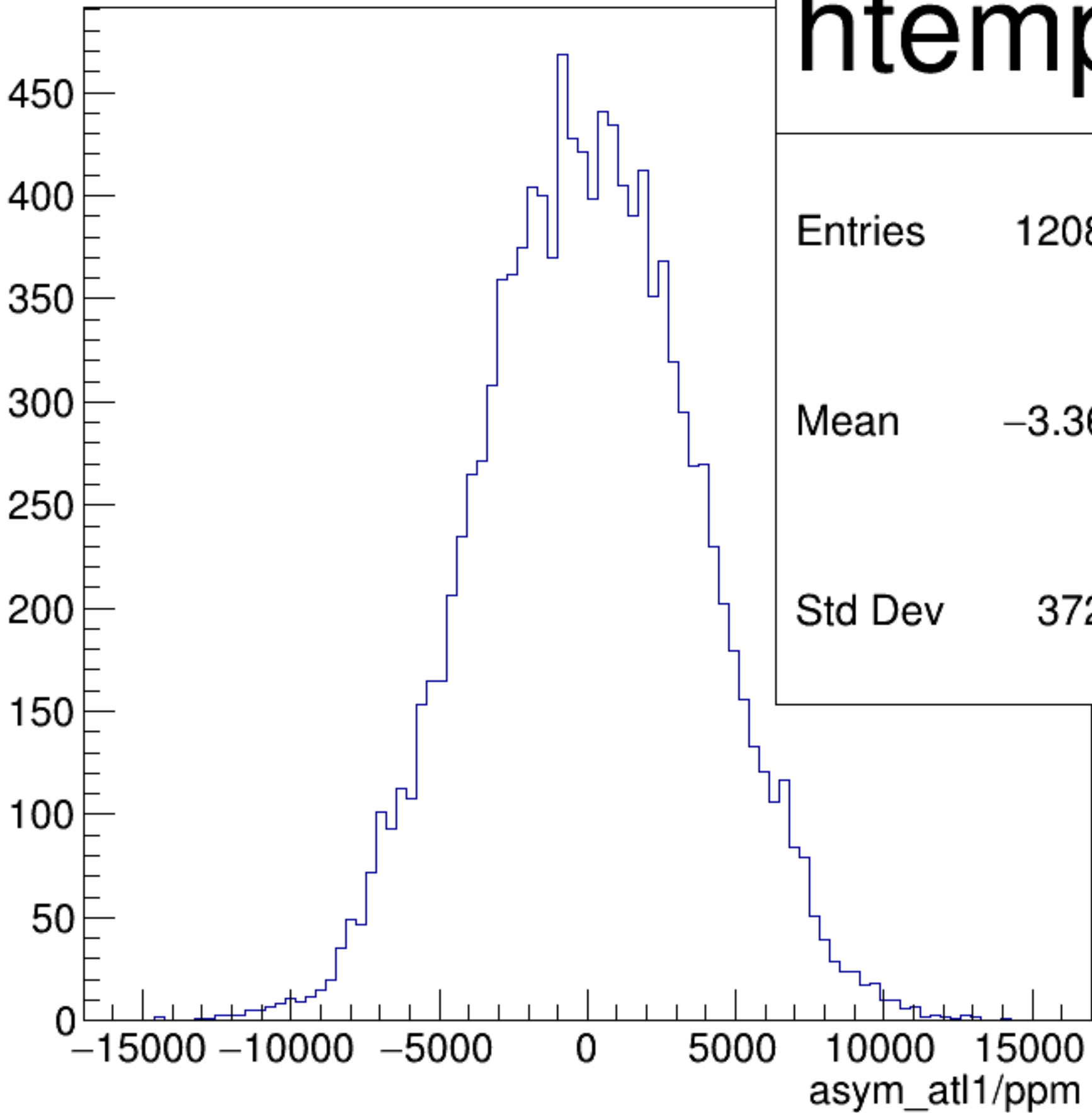
asym_atl1/ppm {ok_cut}
