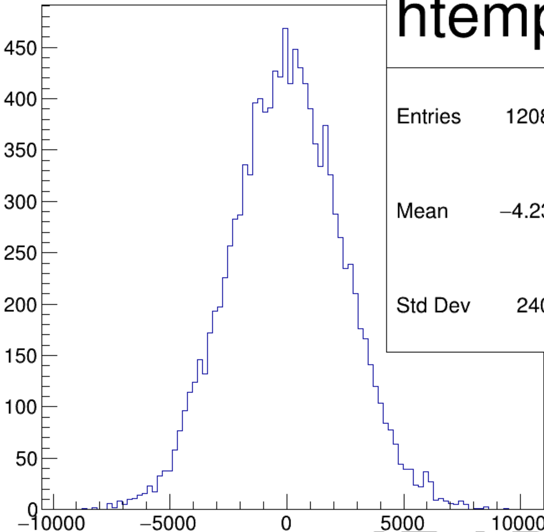
(asym_atl1/ppm-asym_atr1/ppm)/2 {ok_cut}
