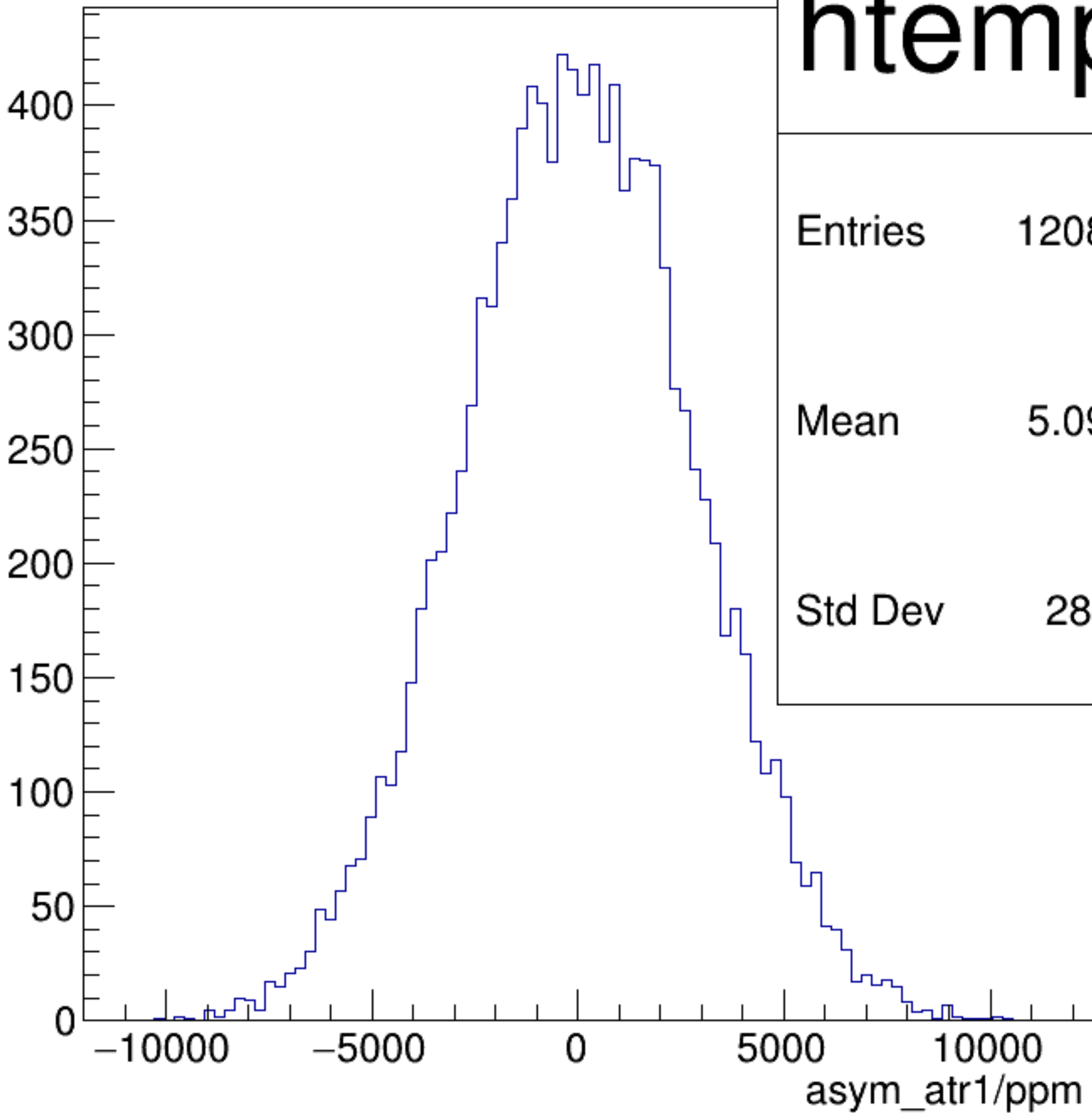
asym_atr1/ppm {ok_cut}
