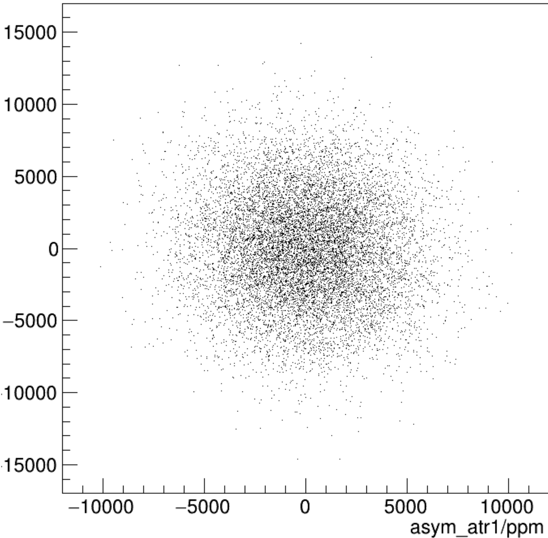
asym_atl1/ppm:asym_atr1/ppm {ok_cut}
