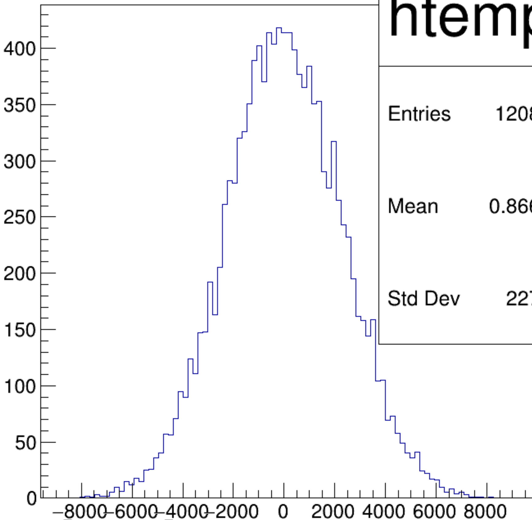
(asym_atl1/ppm+asym_atr1/ppm)/2 {ok_cut}
