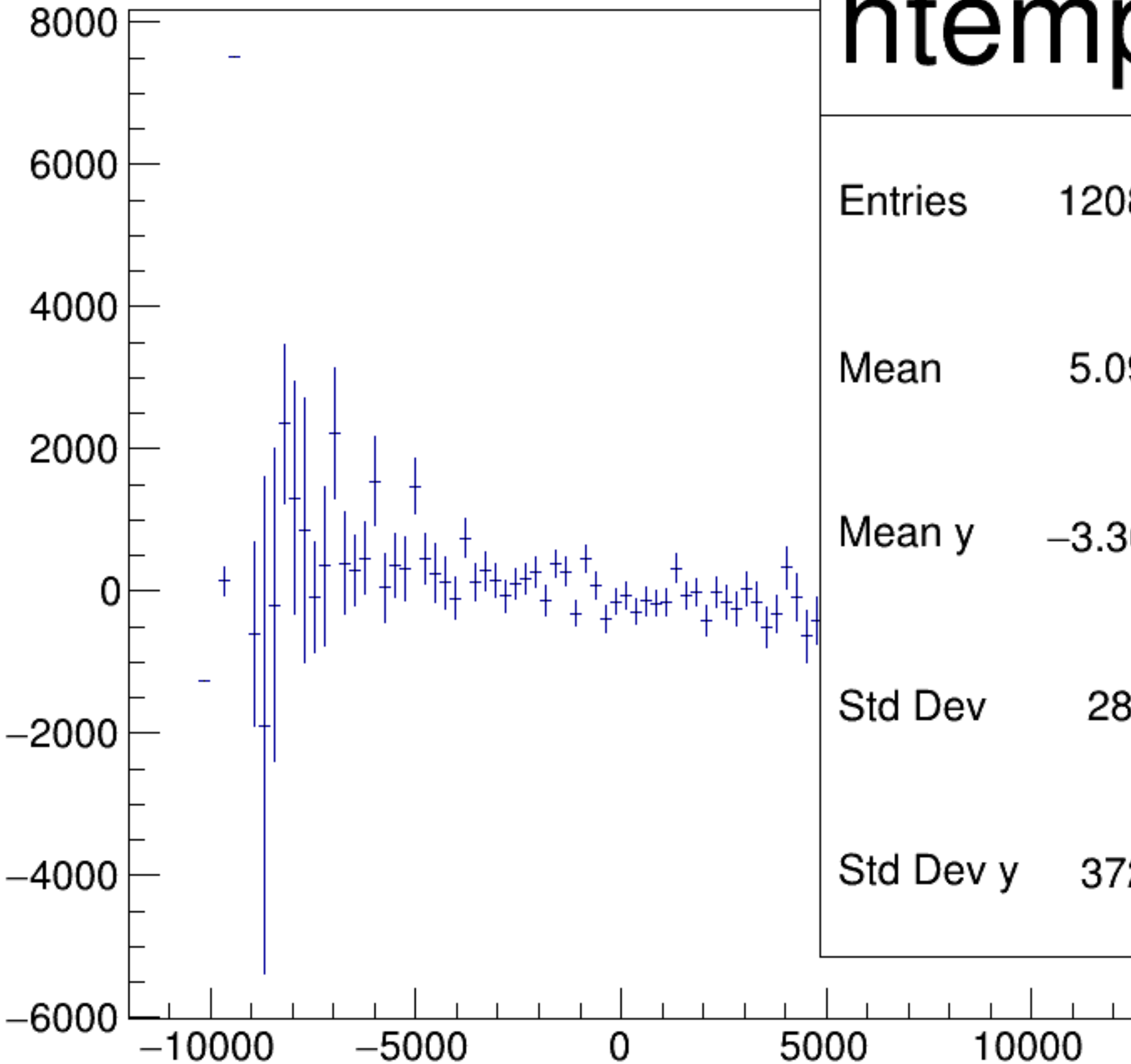
asym_atl1/ppm:asym_atr1/ppm {ok_cut}
