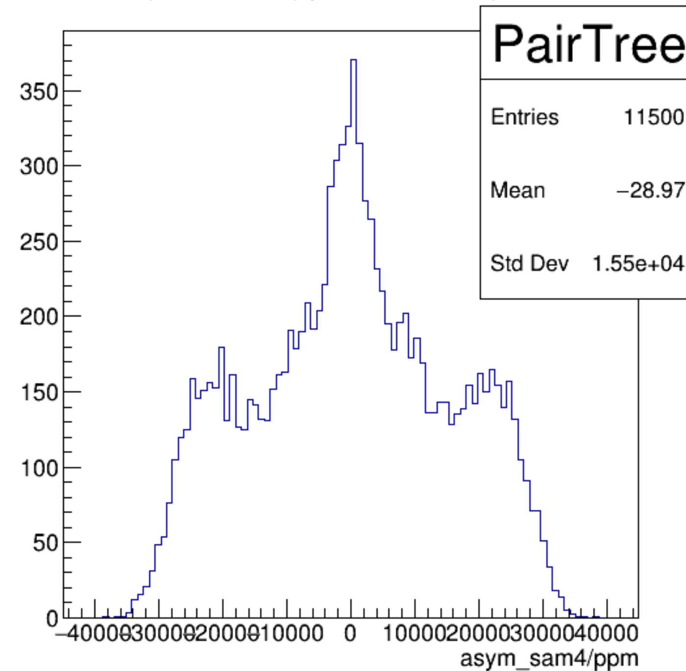
asym_sam4/ppm {ErrorFlag==0}
