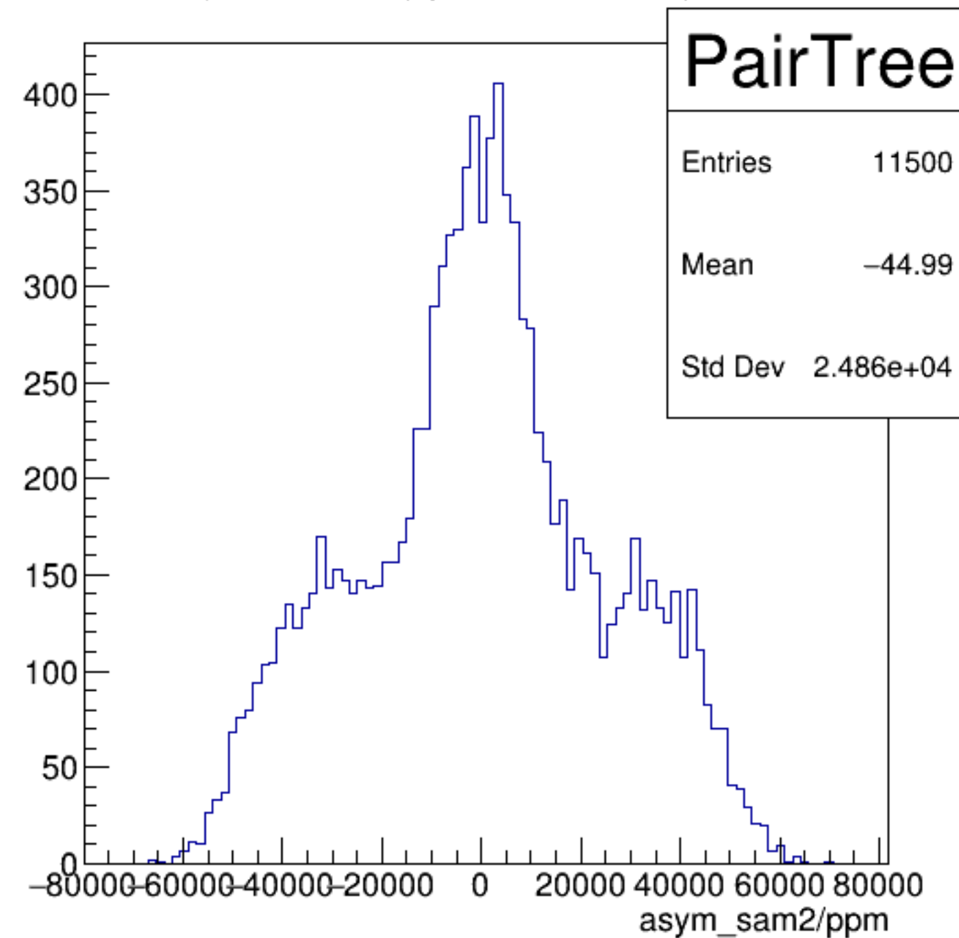
asym_sam2/ppm {ErrorFlag==0}
