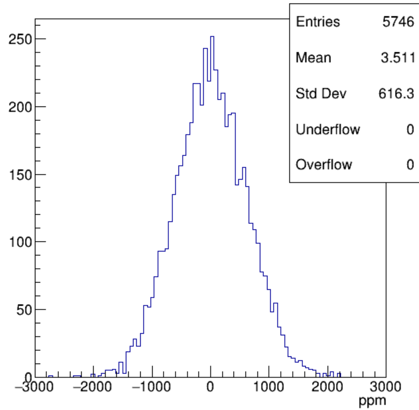
asym_sam1
