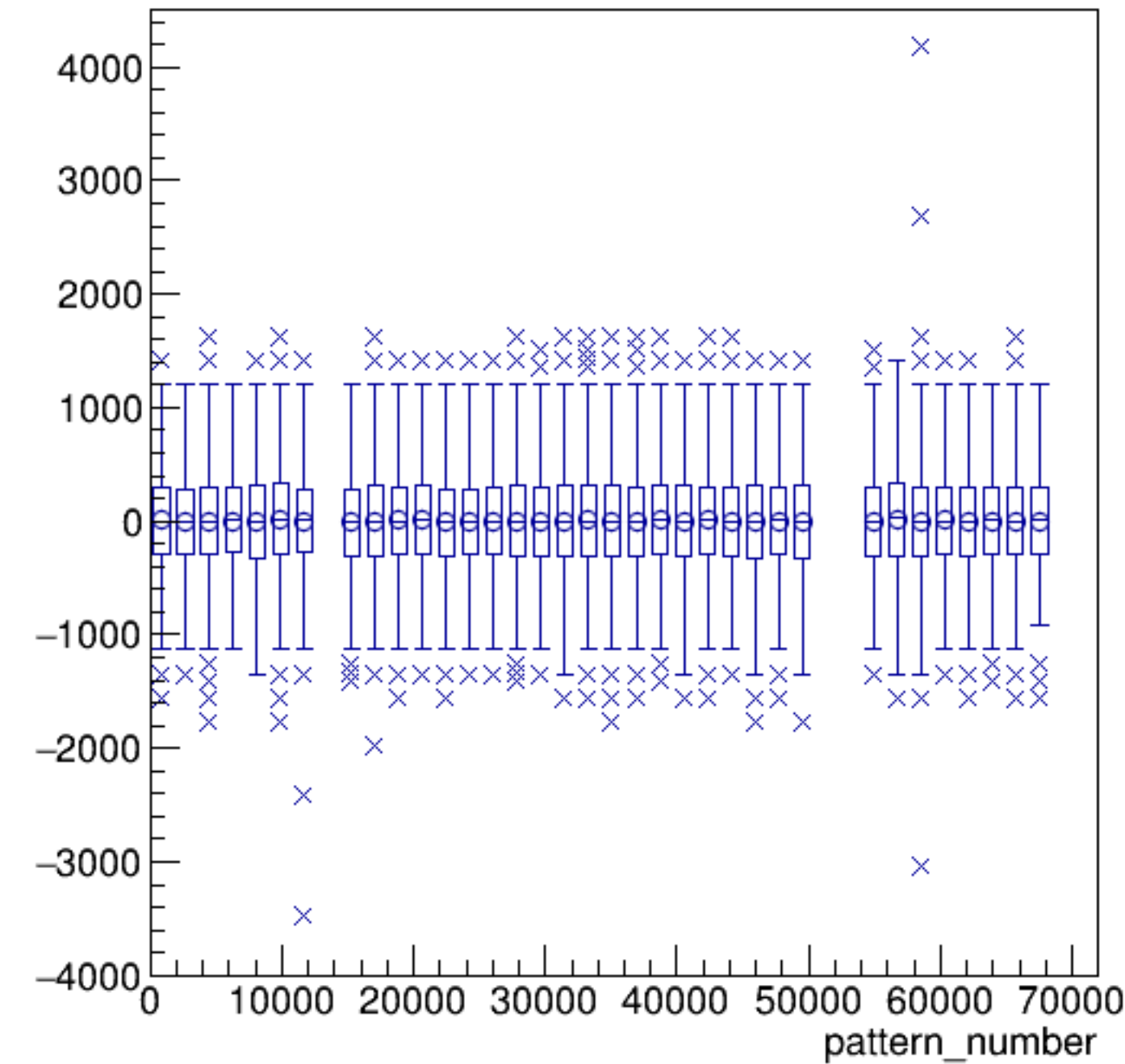
asym_sam8/ppm:pattern_number {ErrorFlag==0}
