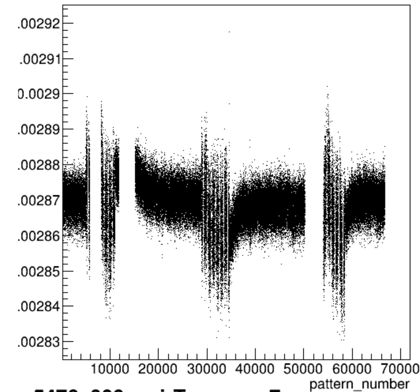
yield_sam7:pattern_number {ErrorFlag==0}
