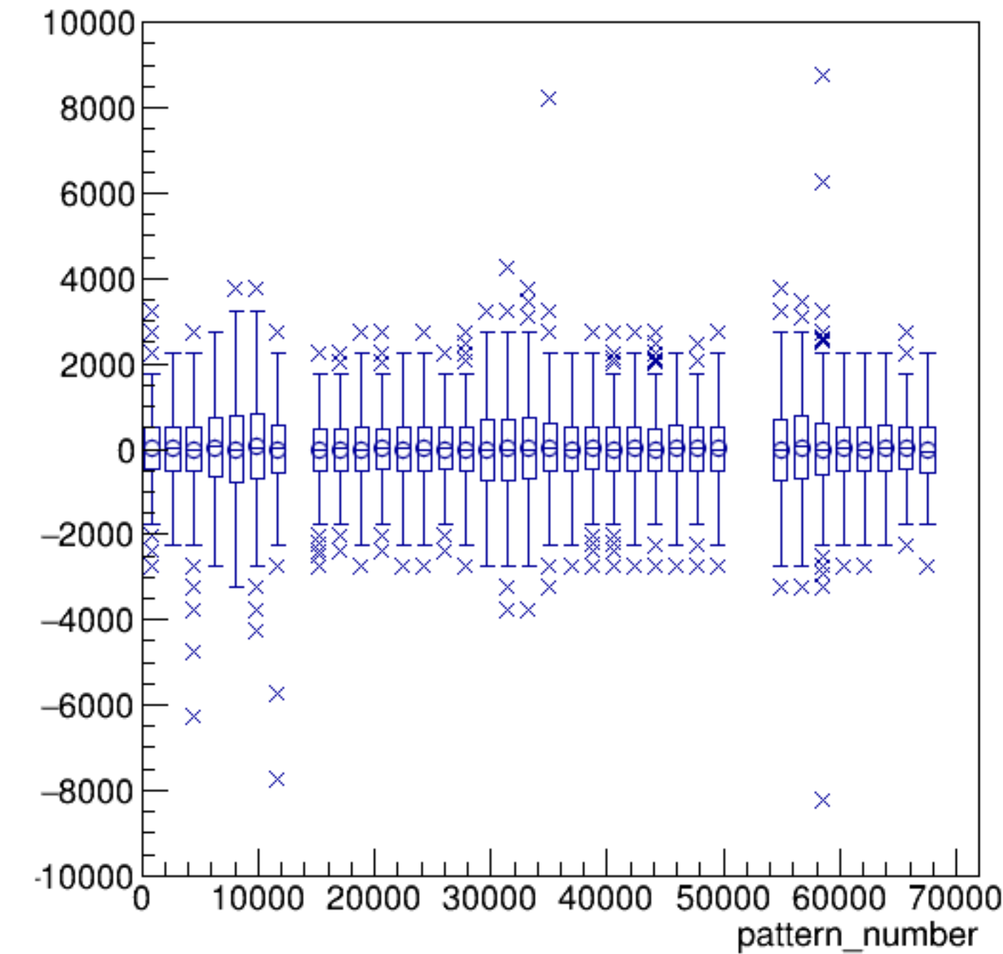
asym_sam7/ppm:pattern_number {ErrorFlag==0}
