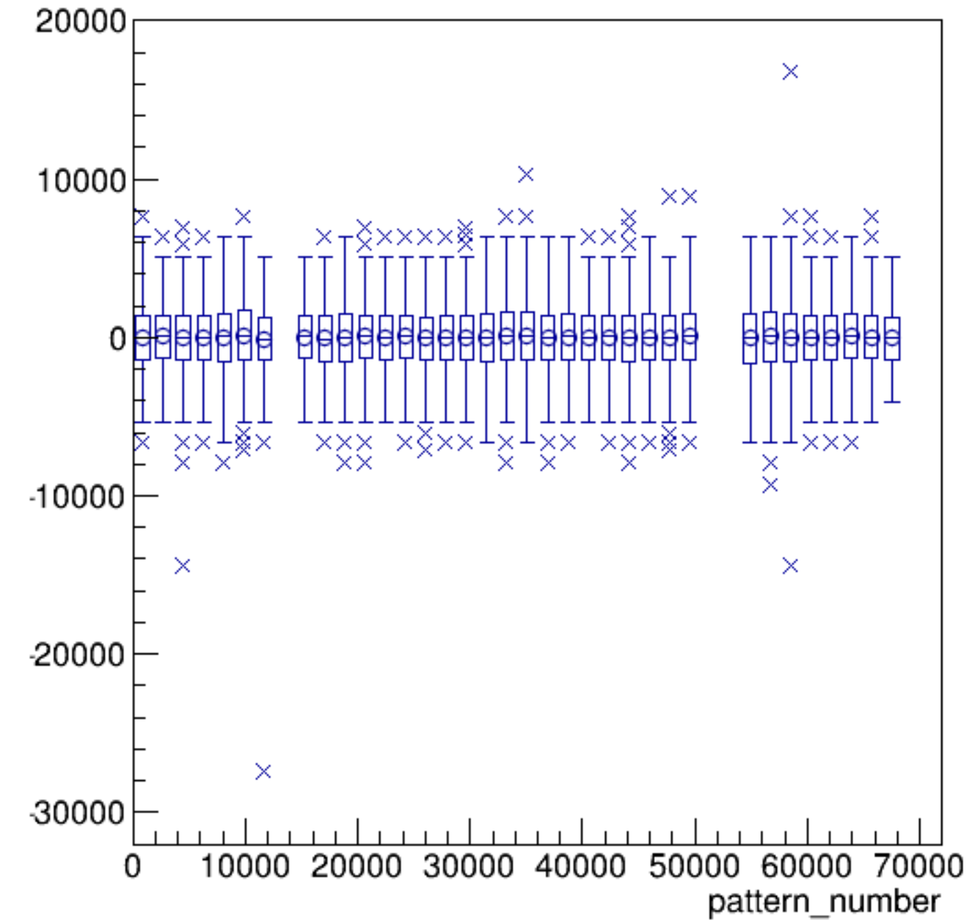
asym_sam4/ppm:pattern_number {ErrorFlag==0}
