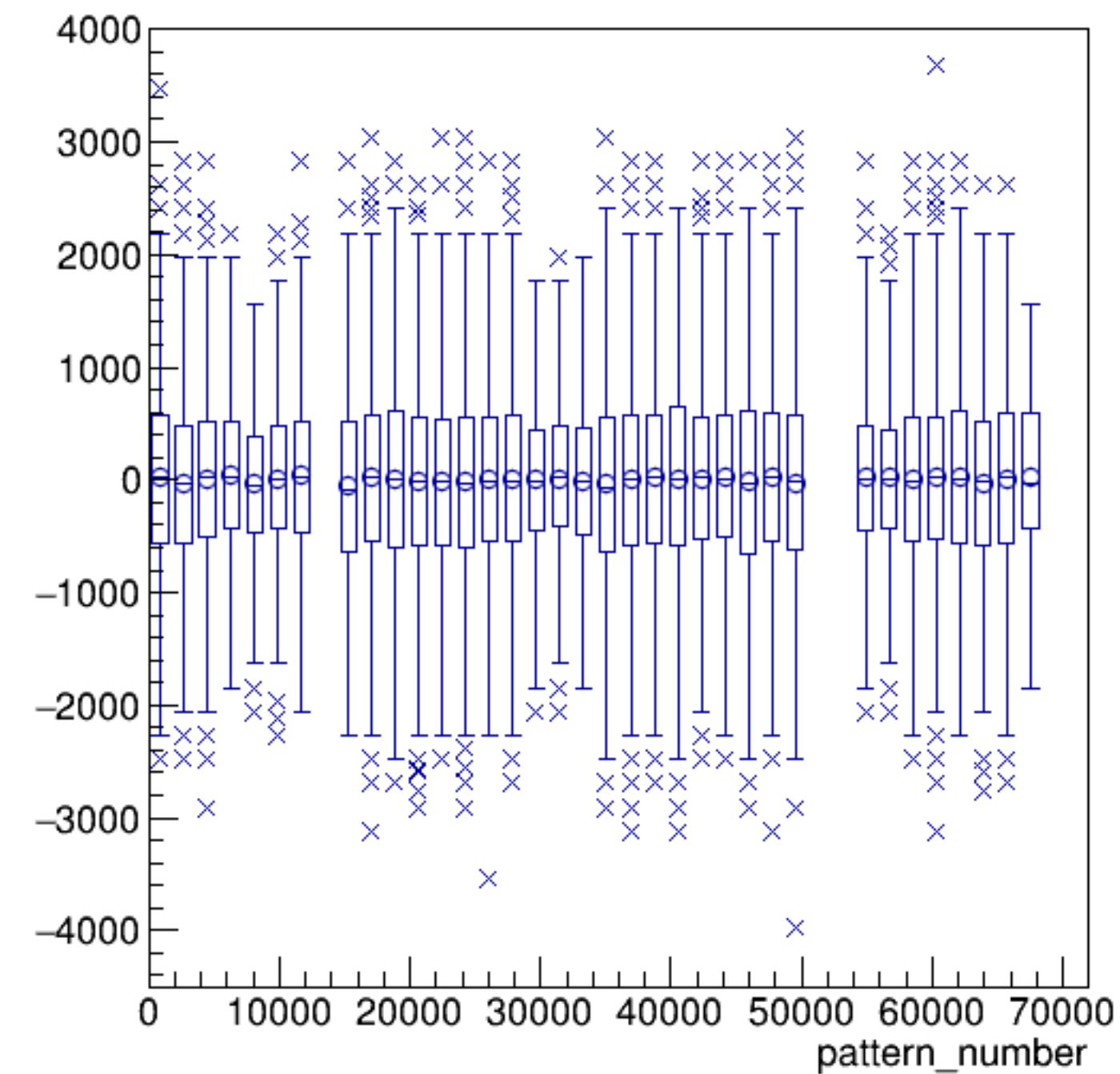
asym_sam1/ppm:pattern_number {ErrorFlag==0}
