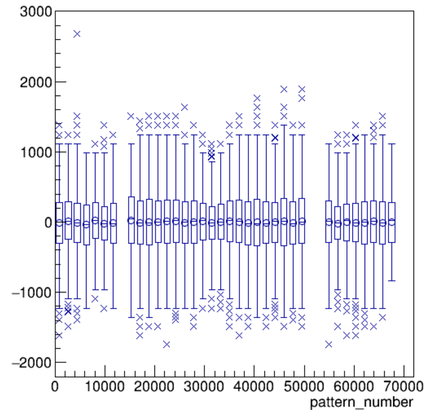
asym_sam6/ppm:pattern_number {ErrorFlag==0}
