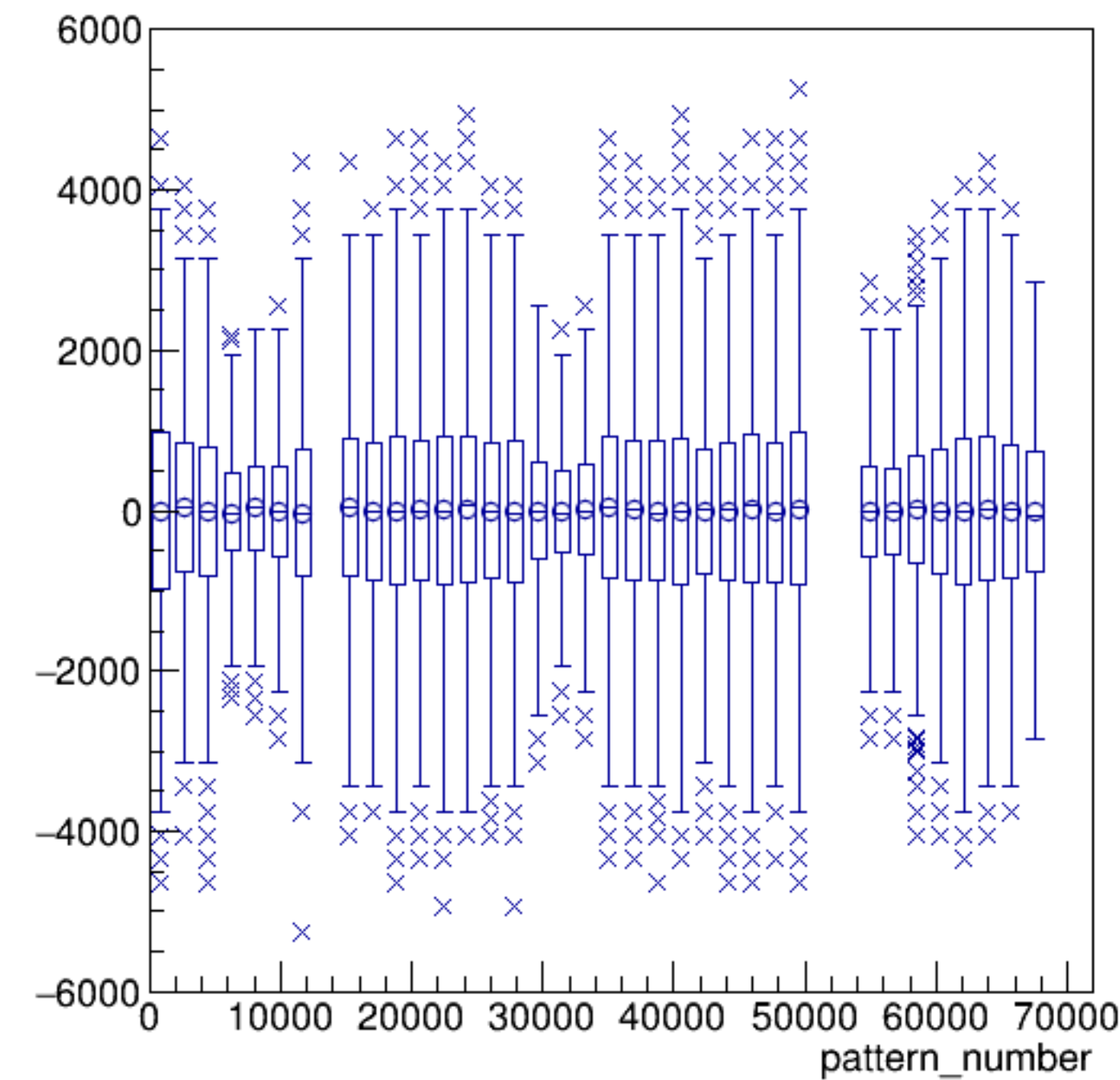
asym_sam5/ppm:pattern_number {ErrorFlag==0}
