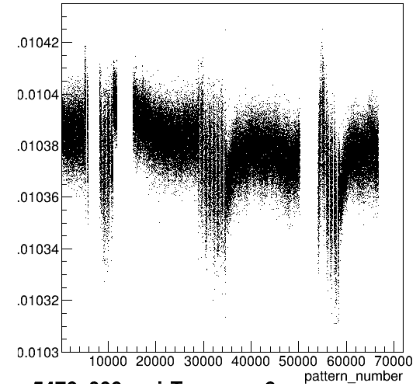
yield_sam8:pattern_number {ErrorFlag==0}
