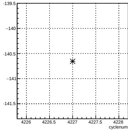
1X_coil1:cyclenum {run == 5477}
