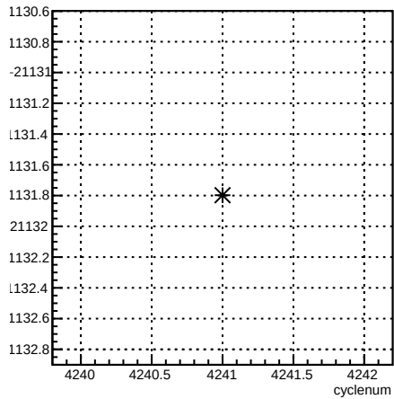
usr_coil1:cyclenum {run == 5486}
