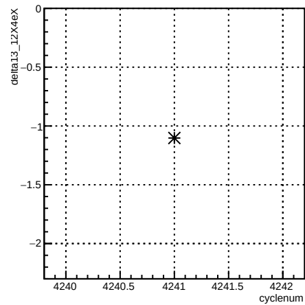
delta13_12X4eX:cyclenum {run == 5486}
