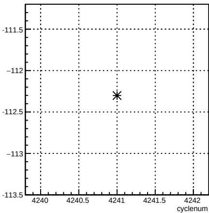
4eY_coil6:cyclenum {run == 5486}
