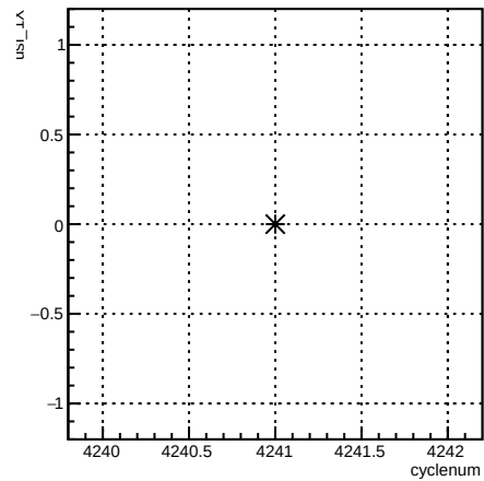
usl_4eY:cyclenum {run == 5486}
