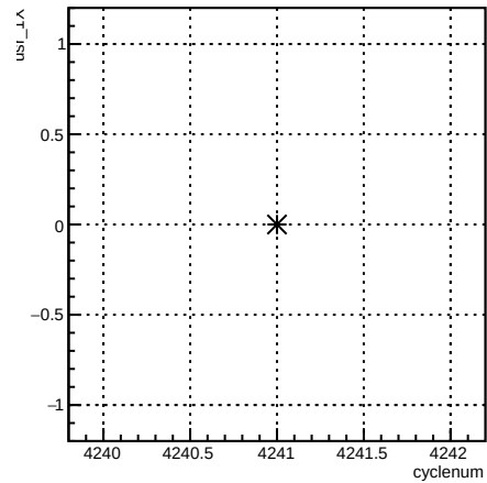
usr_4eY:cyclenum {run == 5486}
