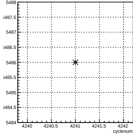
run:cyclenum {run == 5486}
