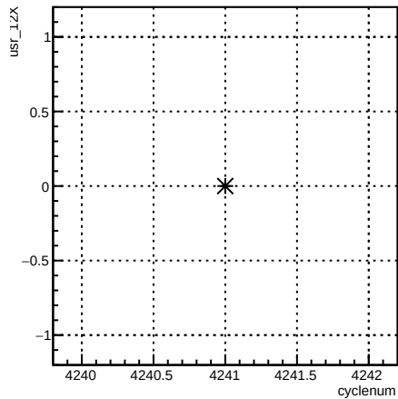
usr_12X:cyclenum {run == 5486}
