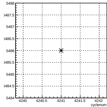
run:cyclenum {run == 5486}
