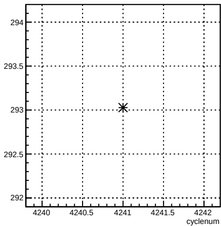
4eY_coil4:cyclenum {run == 5486}
