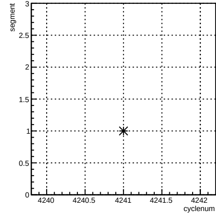
segment:cyclenum {run == 5486}
