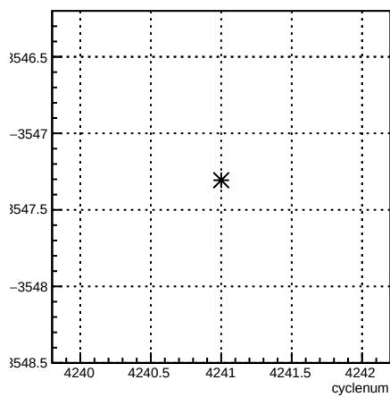
usr_coil3:cyclenum {run == 5486}
