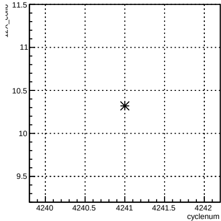
12X_coil6:cyclenum {run == 5486}
