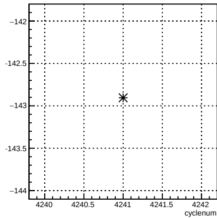
4eX_coil1:cyclenum {run == 5486}
