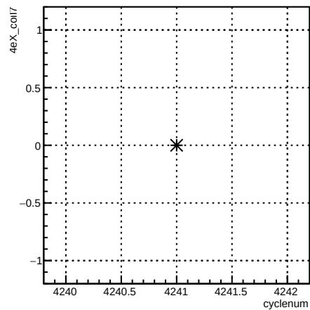
4eX_coil7:cyclenum {run == 5486}
