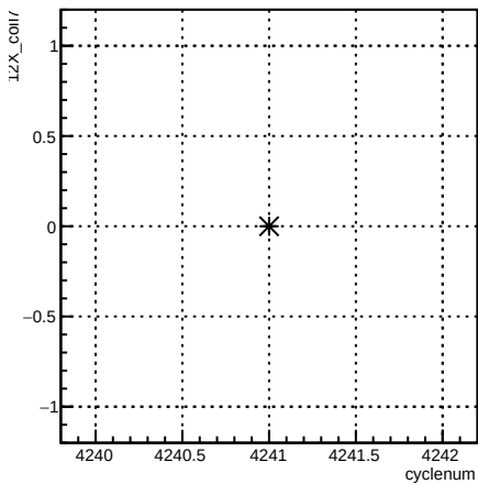
12X_coil7:cyclenum {run == 5486}
