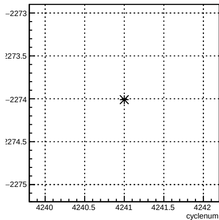
usl_coil6:cyclenum {run == 5486}
