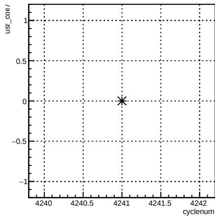
usr_coil7:cyclenum {run == 5486}
