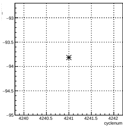
4aY_coil6:cyclenum {run == 5486}
