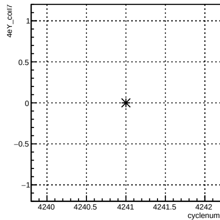
4eY_coil7:cyclenum {run == 5486}
