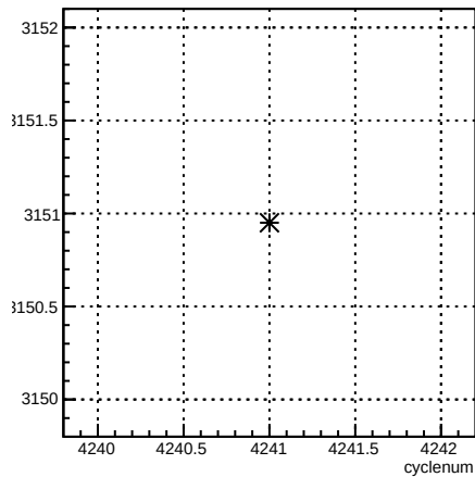
usl_coil7:cyclenum {run == 5486}
