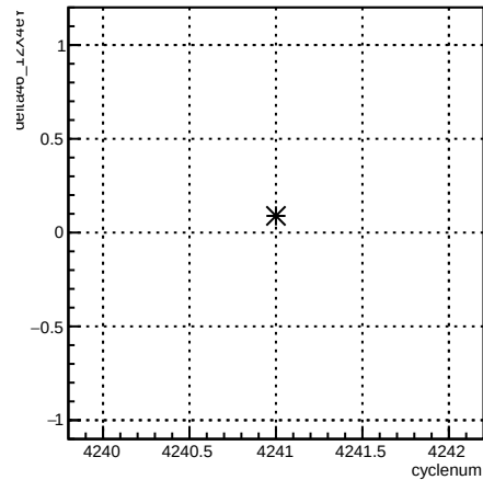
delta46_12X4eY:cyclenum {run == 5486}
