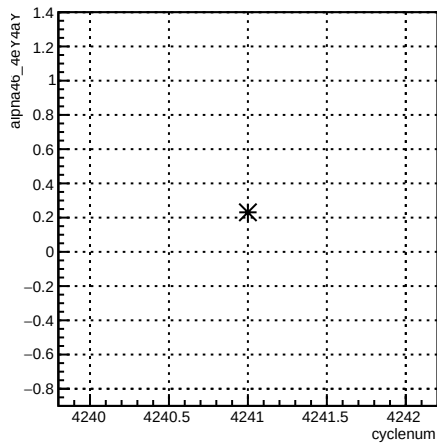
alpha46_4eY4aY:cyclenum {run == 5486}
