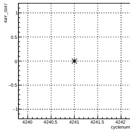
4aY_coil7:cyclenum {run == 5486}
