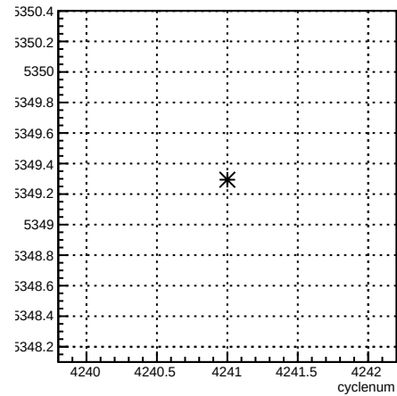
usr_coil4:cyclenum {run == 5486}
