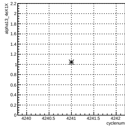
alpha13_4eX1X:cyclenum {run == 5486}
