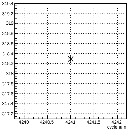
4aY_coil4:cyclenum {run == 5486}
