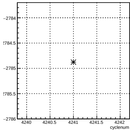
usr_coil6:cyclenum {run == 5486}
