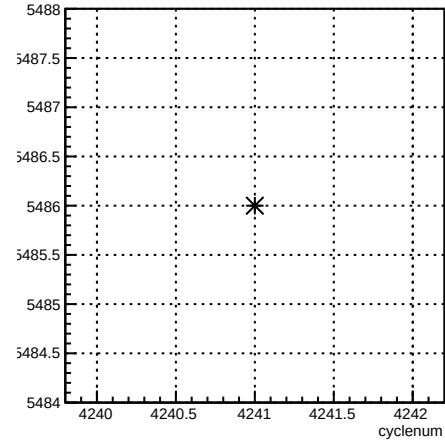
run:cyclenum {run == 5486}
