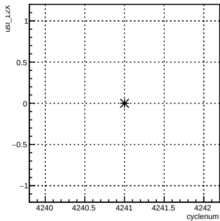
usl_12X:cyclenum {run == 5486}
