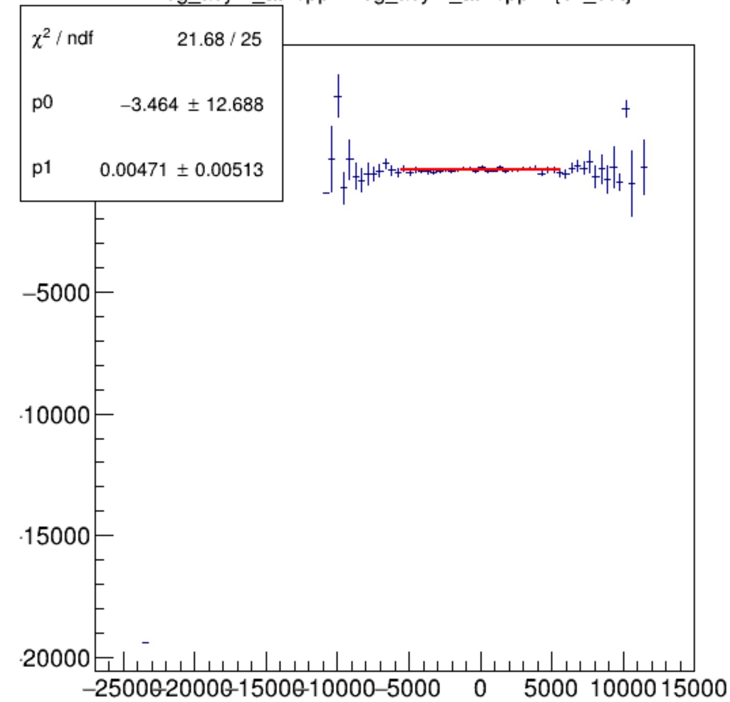
reg_asym_atl1/ppm:reg_asym_atr1/ppm {ok_cut}
