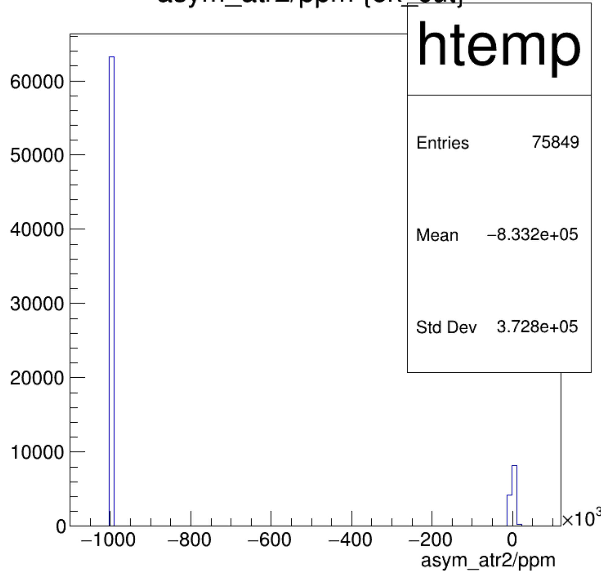
asym_atr2/ppm {ok_cut}
