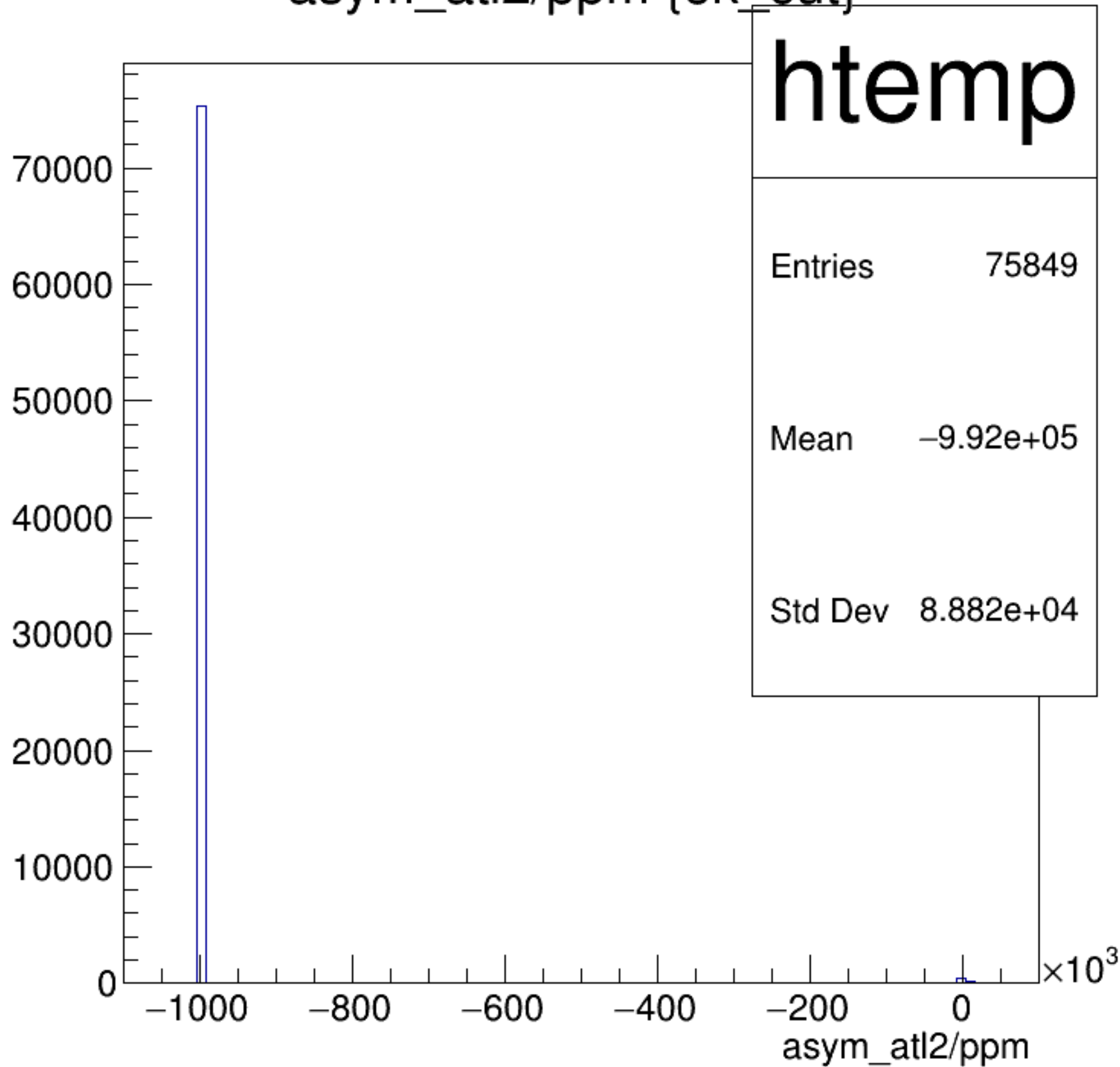
asym_atl2/ppm {ok_cut}
