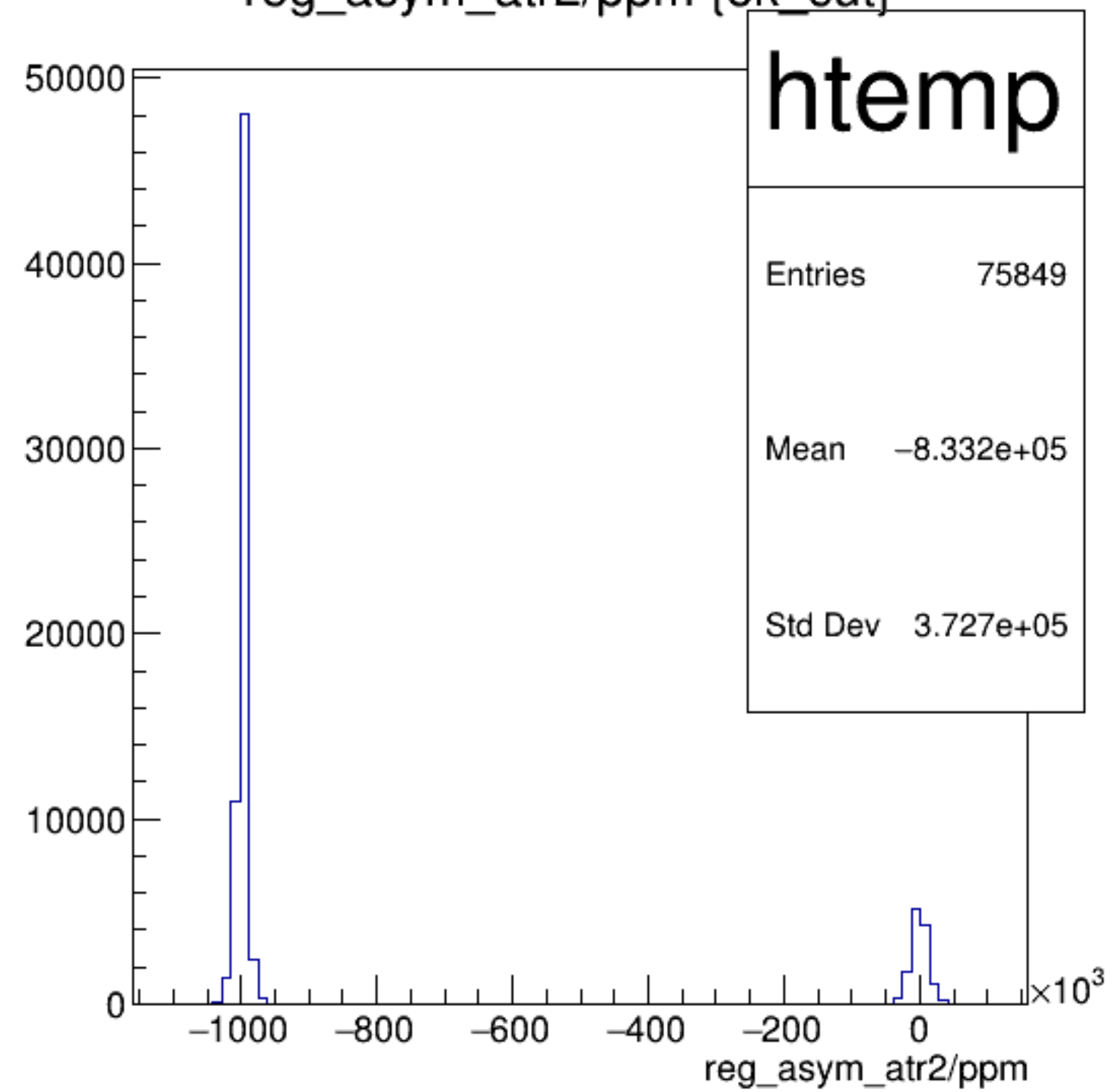
reg_asym_atr2/ppm {ok_cut}
