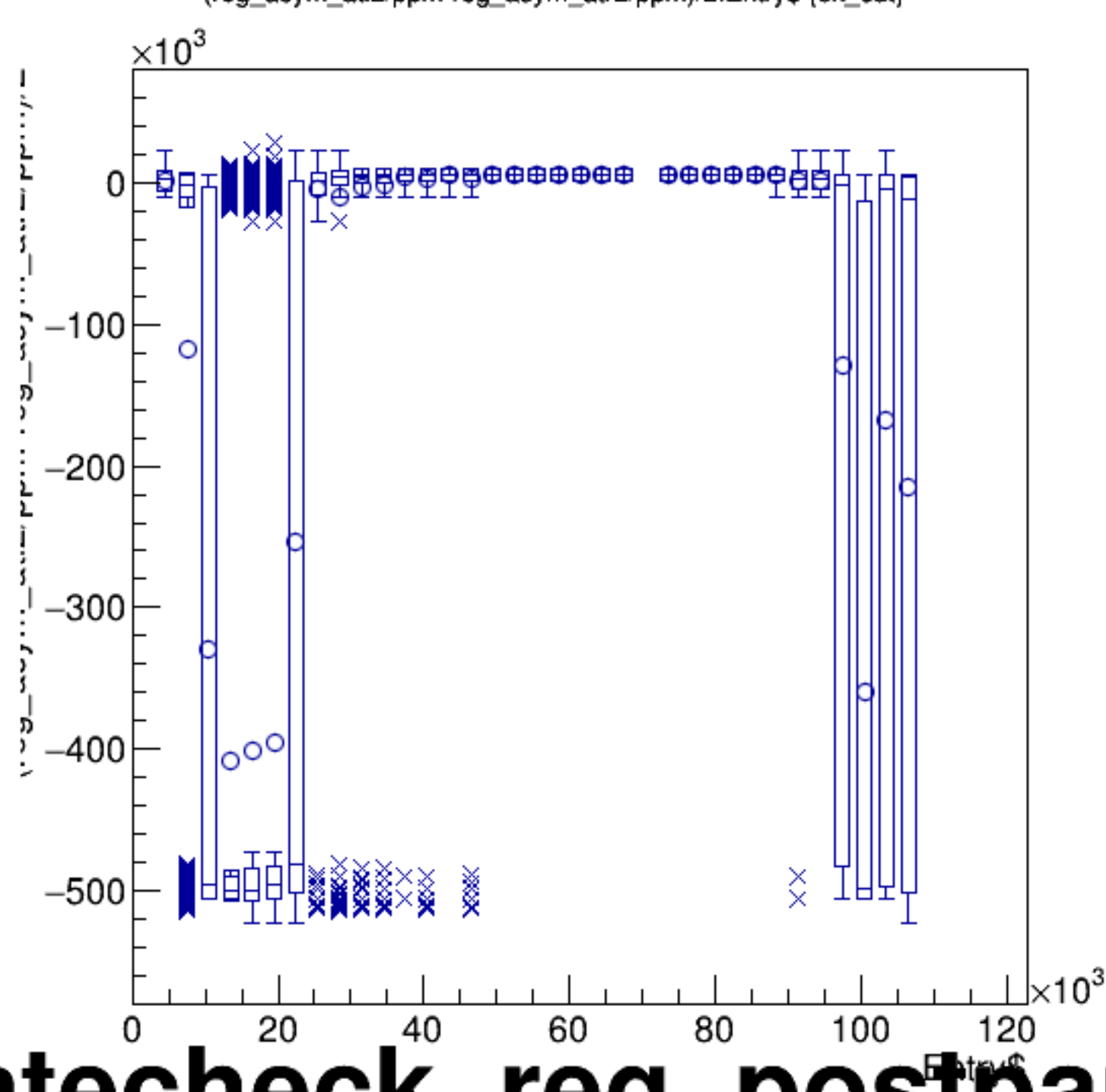
(reg_asym_atl2/ppm-reg_asym_atr2/ppm)/2:Entry$ {ok_cut}
