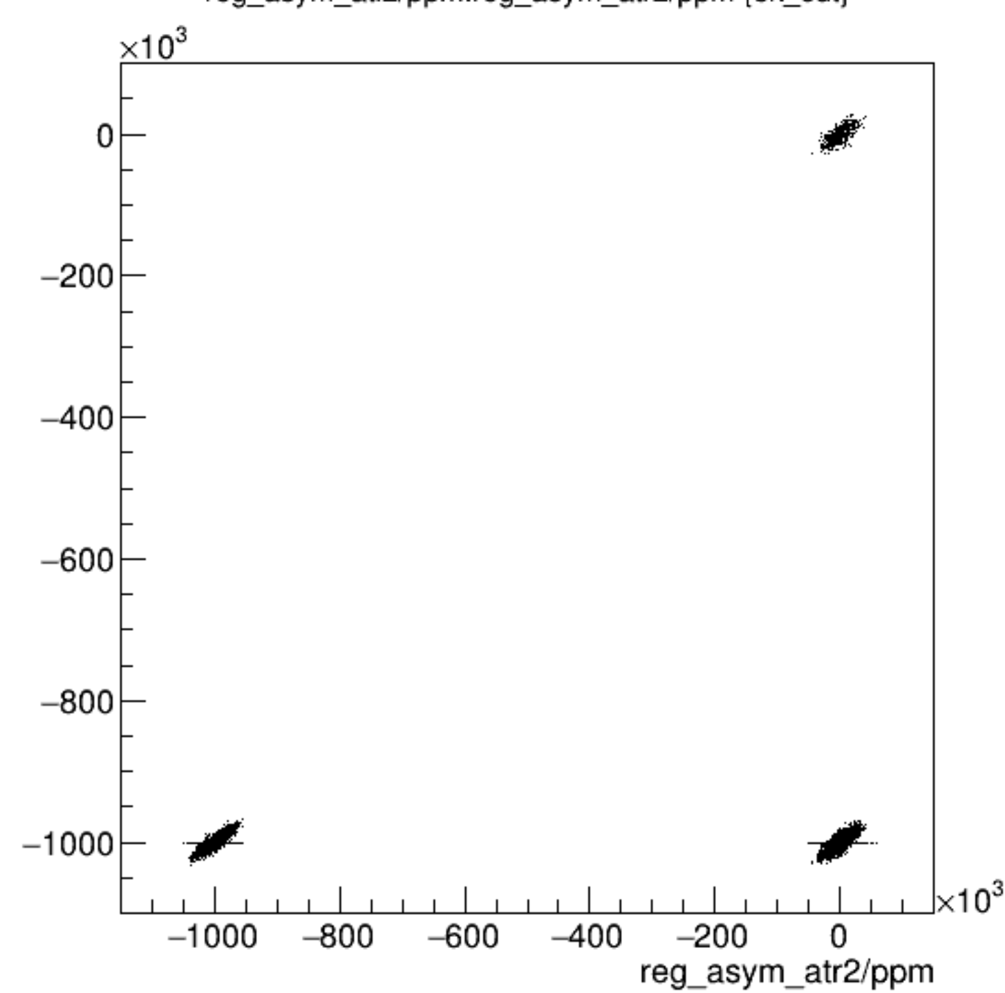
reg_asym_atl2/ppm:reg_asym_atr2/ppm {ok_cut}
