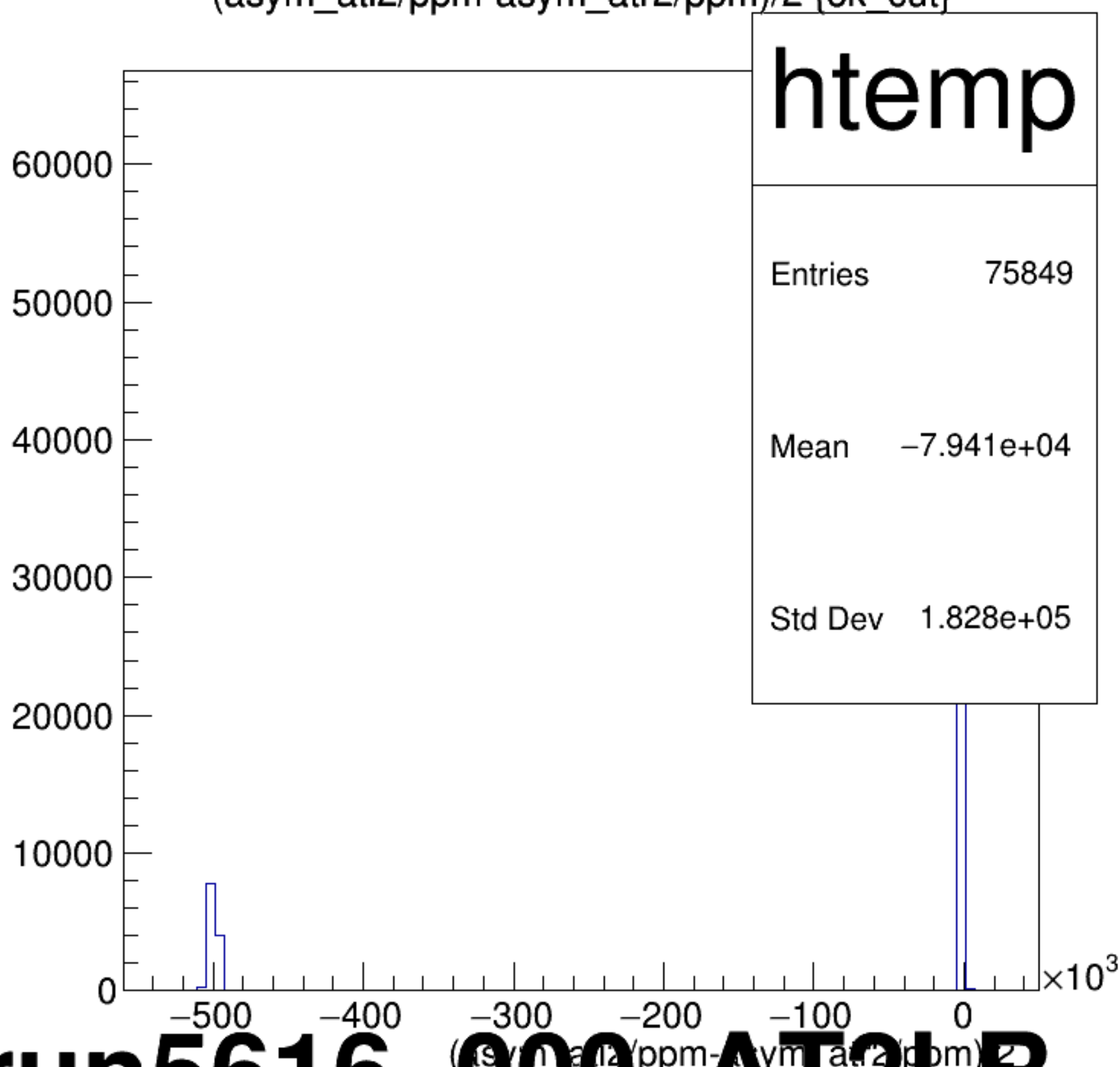
(asym_atl2/ppm-asym_atr2/ppm)/2 {ok_cut}
