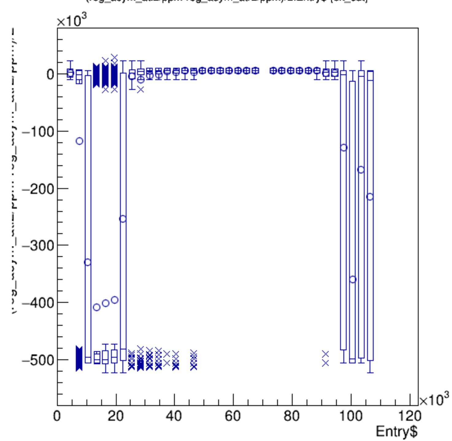
(reg_asym_atl2/ppm-reg_asym_atr2/ppm)/2:Entry$ {ok_cut}
