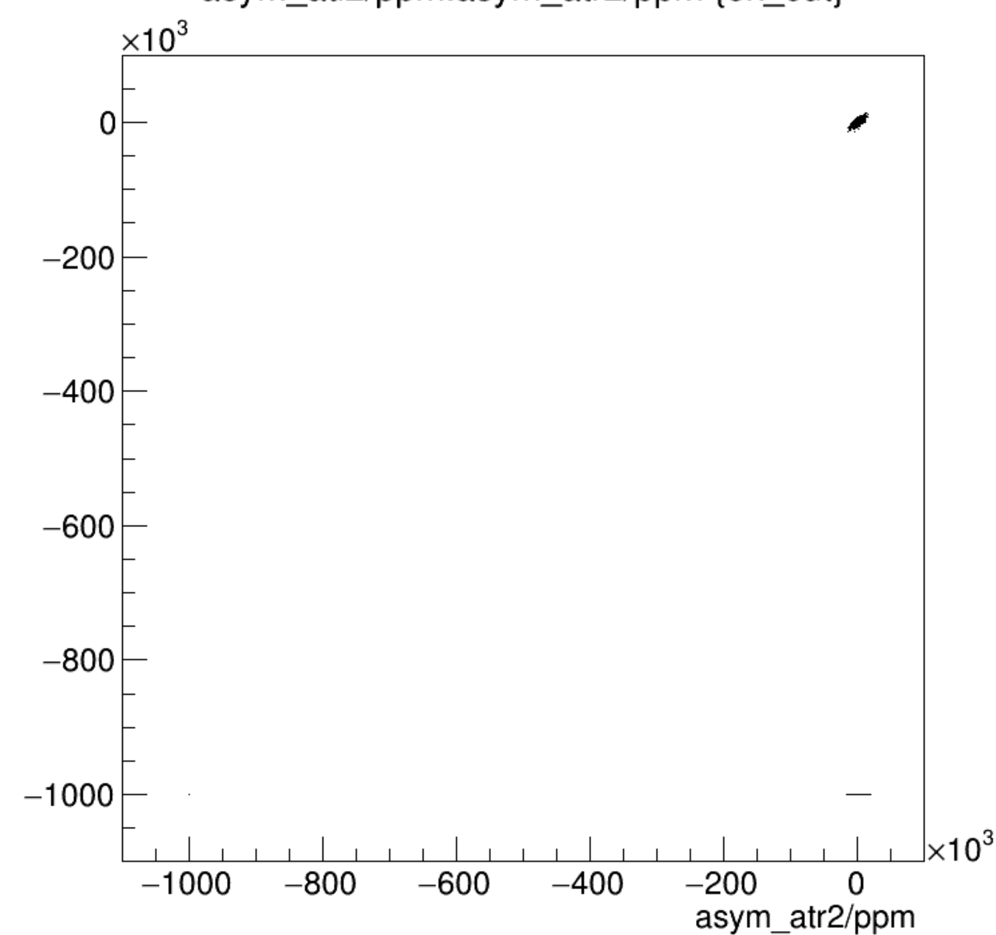
asym_atl2/ppm:asym_atr2/ppm {ok_cut}
