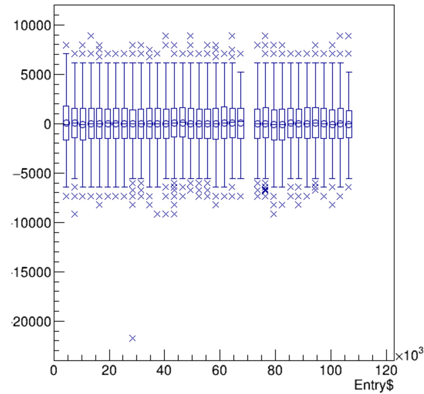
(reg_asym_atl1/ppm+reg_asym_atr1/ppm)/2:Entry$ {ok_cut}
