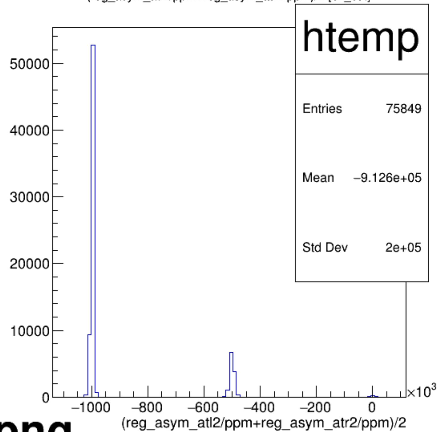
(reg_asym_atl2/ppm+reg_asym_atr2/ppm)/2 {ok_cut}
