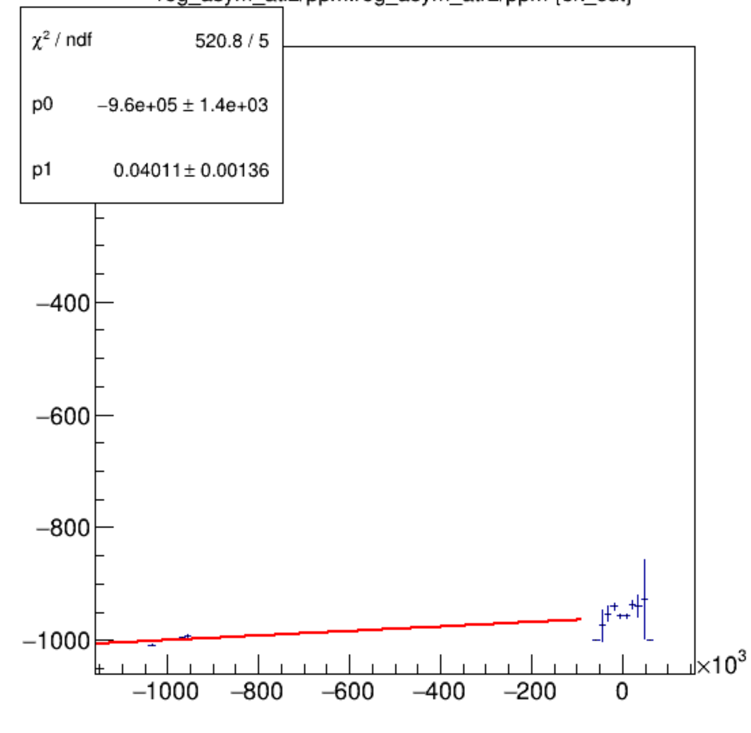
reg_asym_atl2/ppm:reg_asym_atr2/ppm {ok_cut}
