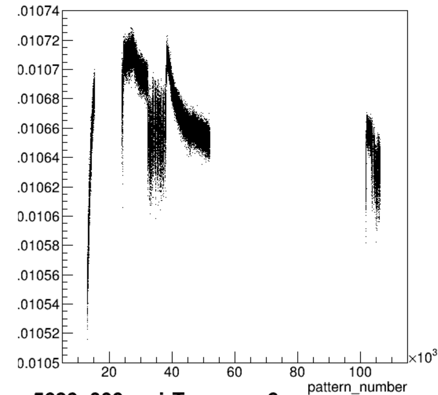
yield_sam8:pattern_number {ErrorFlag==0}
