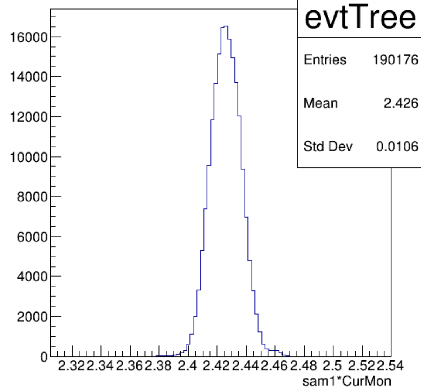
sam1*CurMon {ErrorFlag==0}
