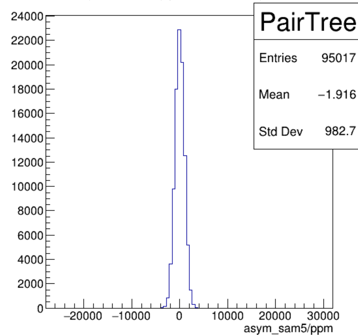
asym_sam5/ppm {ErrorFlag==0}
