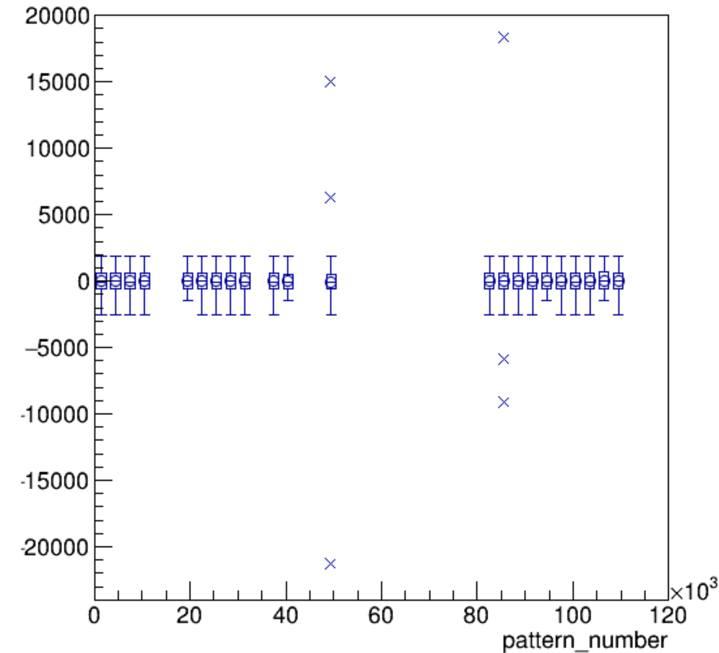
asym_sam1/ppm:pattern_number {ErrorFlag==0}
