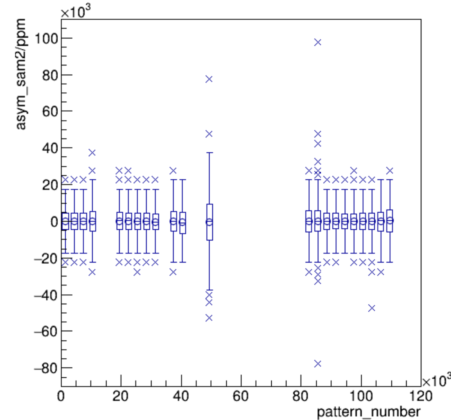
asym_sam2/ppm:pattern_number {ErrorFlag==0}
