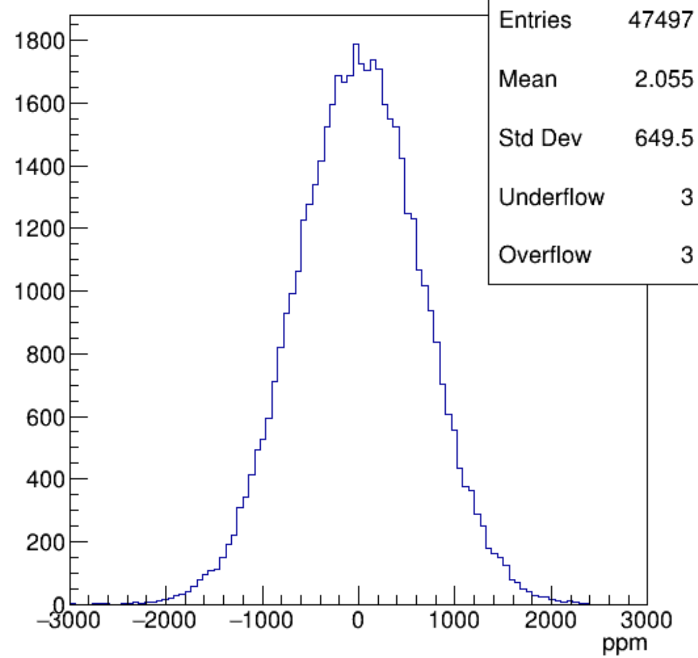
asym_sam1
