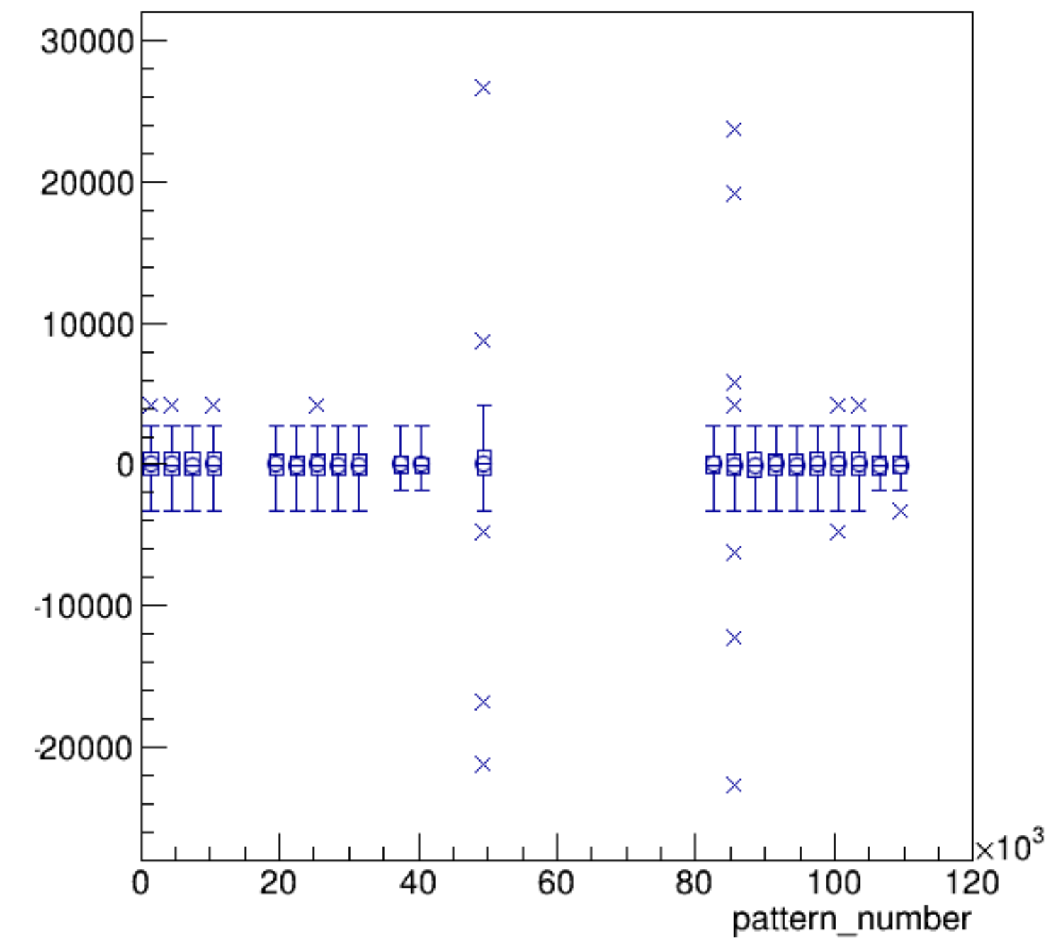
asym_sam5/ppm:pattern_number {ErrorFlag==0}
