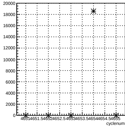
usl_coil1:cyclenum {run == 5645}
