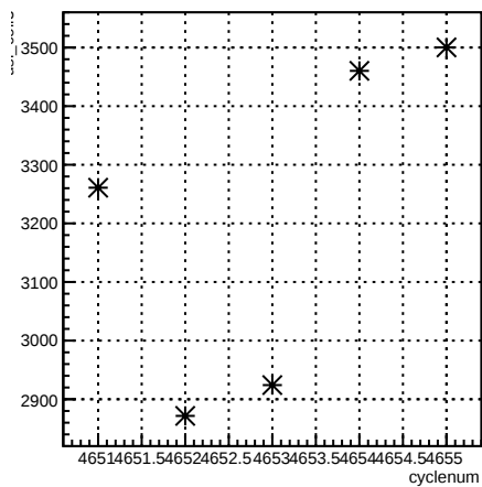
usl_coil3:cyclenum {run == 5645}
