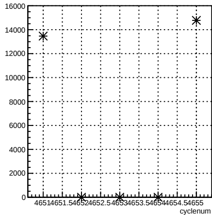
usl_coil7:cyclenum {run == 5645}
