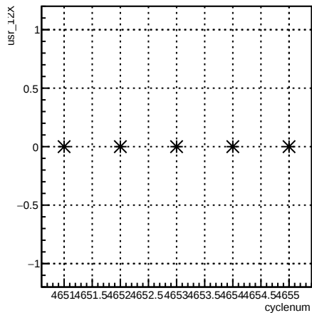
usr_12X:cyclenum {run == 5645}
