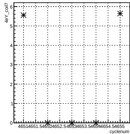
4eY_coil7:cyclenum {run == 5645}
