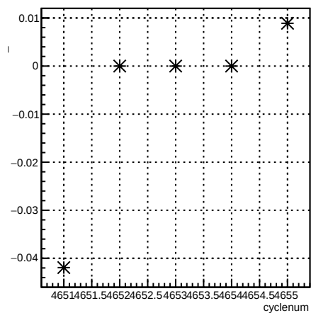
delta46_12X4eY:cyclenum {run == 5645}
