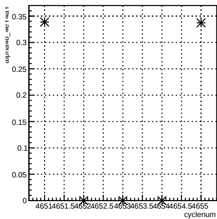
alpha46_4eY4aY:cyclenum {run == 5645}
