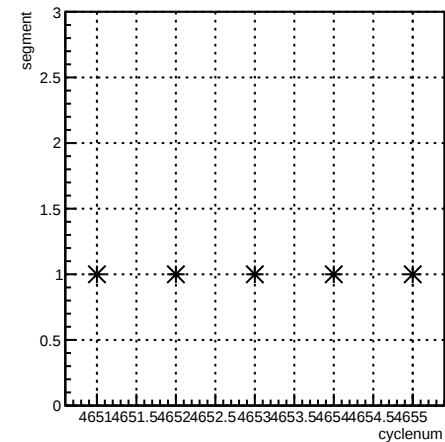
segment:cyclenum {run == 5645}
