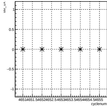
usl_4eY:cyclenum {run == 5645}
