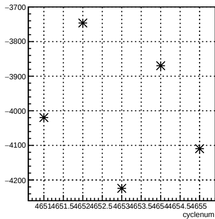
usr_coil3:cyclenum {run == 5645}
