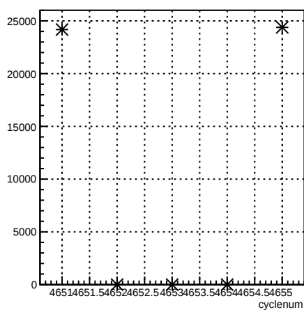
usr_coil7:cyclenum {run == 5645}
