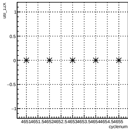
usl_12X:cyclenum {run == 5645}
