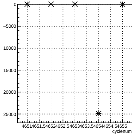
usr_coil1:cyclenum {run == 5645}
