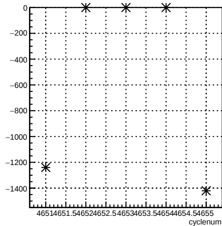
usr_coil6:cyclenum {run == 5645}
