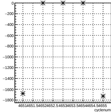
usl_coil6:cyclenum {run == 5645}
