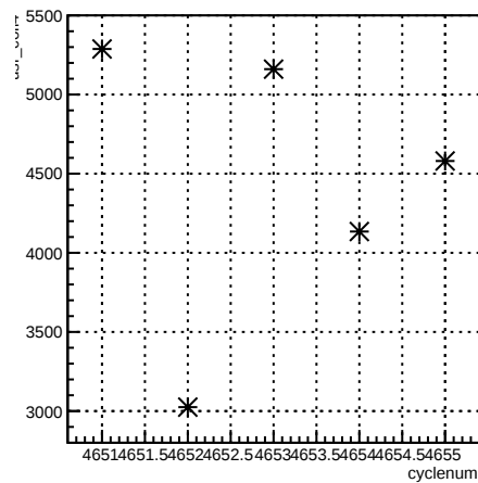
usr_coil4:cyclenum {run == 5645}
