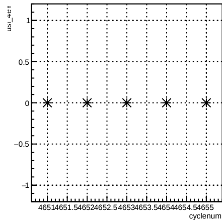
usl_4eY:cyclenum {run == 5645}
