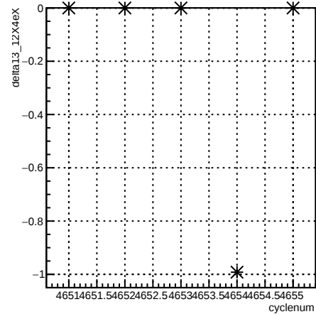
delta13_12X4eX:cyclenum {run == 5645}
