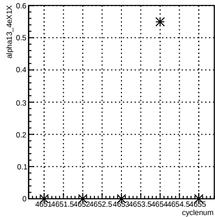
alpha13_4eX1X:cyclenum {run == 5645}
