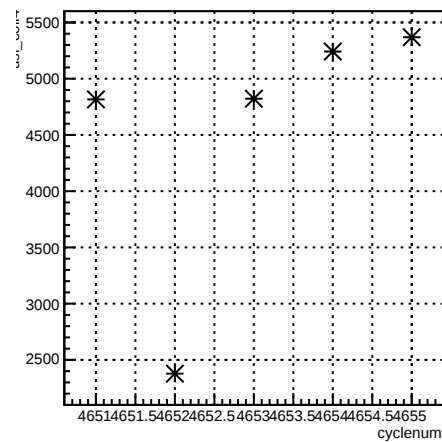
usl_coil4:cyclenum {run == 5645}
