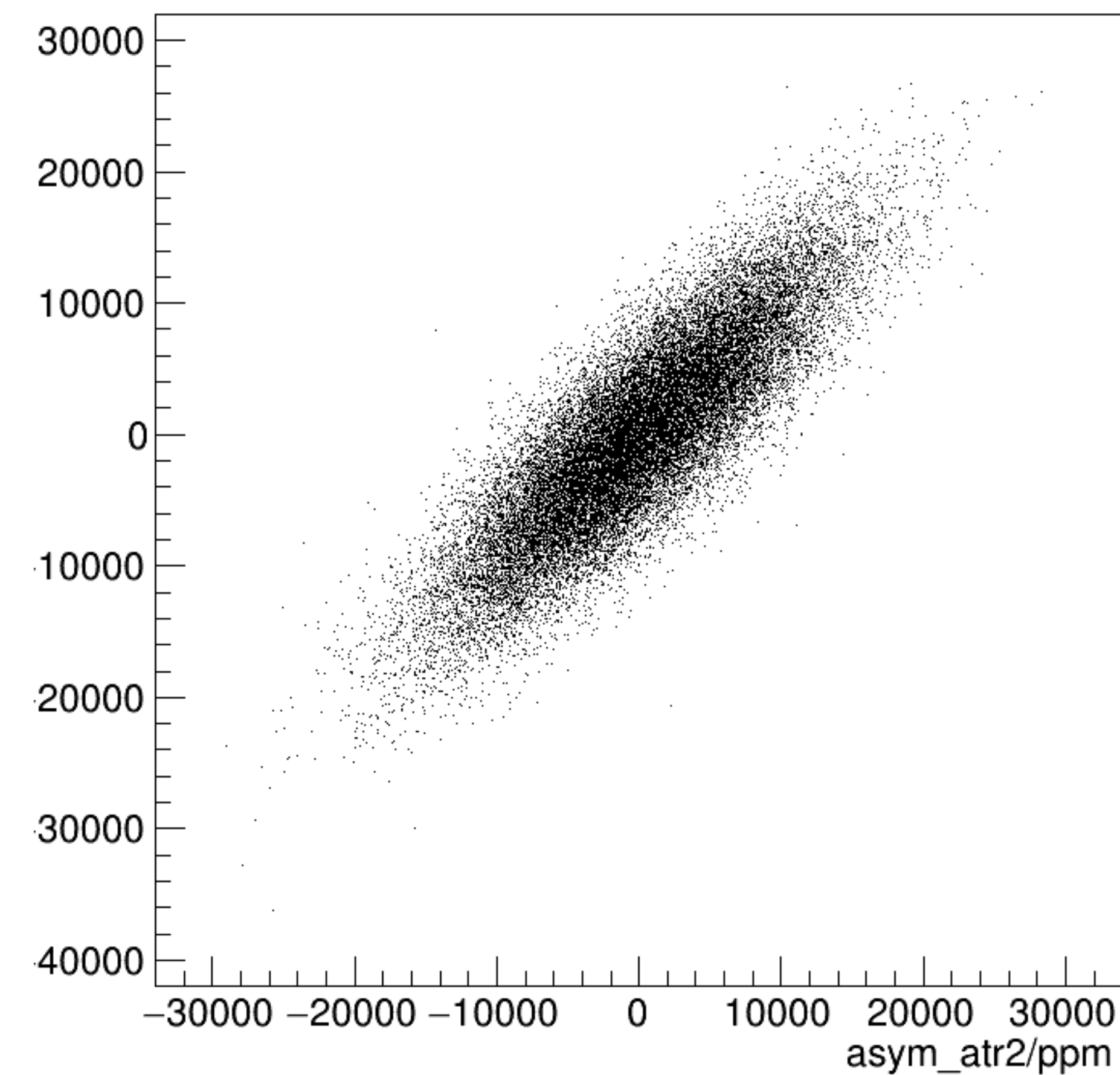
asym_atl2/ppm:asym_atr2/ppm {ok_cut}
