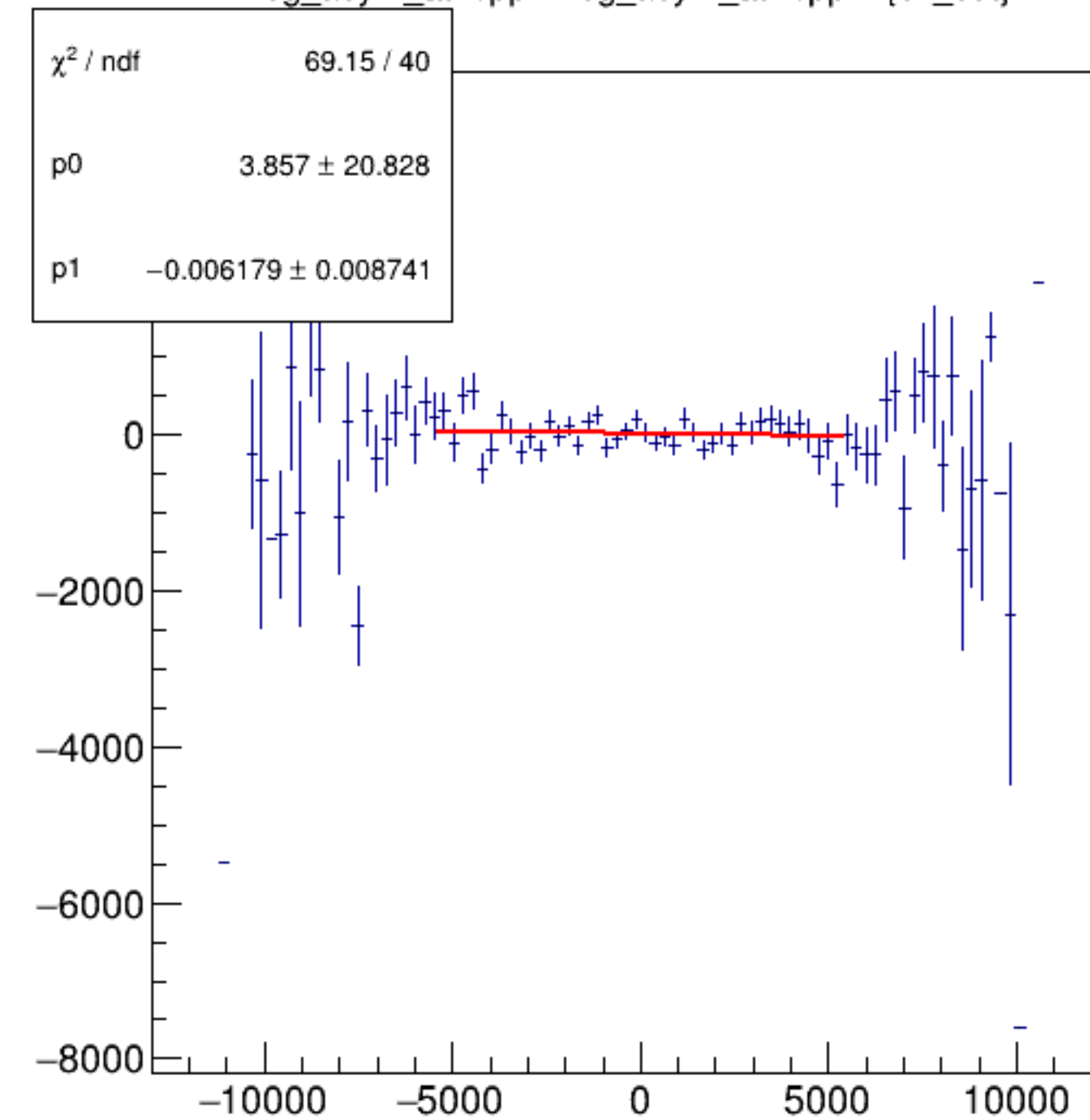
reg_asym_atl1/ppm:reg_asym_atr1/ppm {ok_cut}
