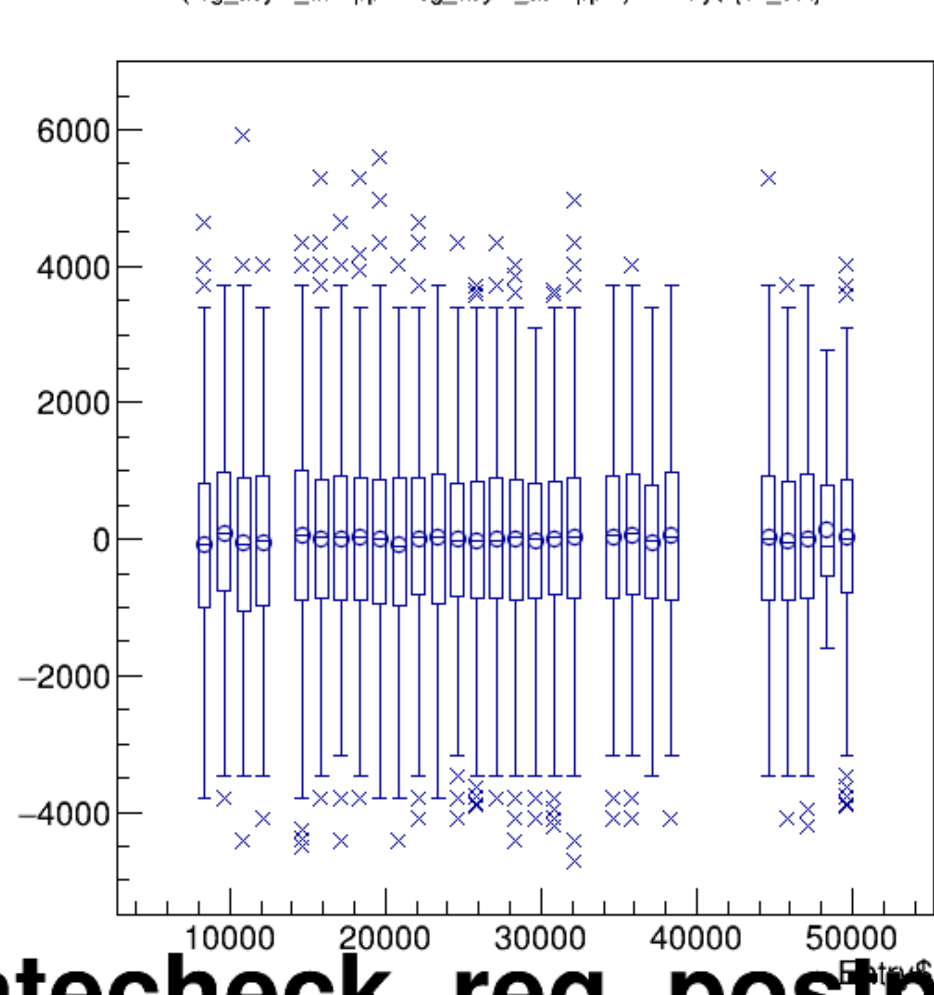
(reg_asym_atl2/ppm-reg_asym_atr2/ppm)/2:Entry$ {ok_cut}
