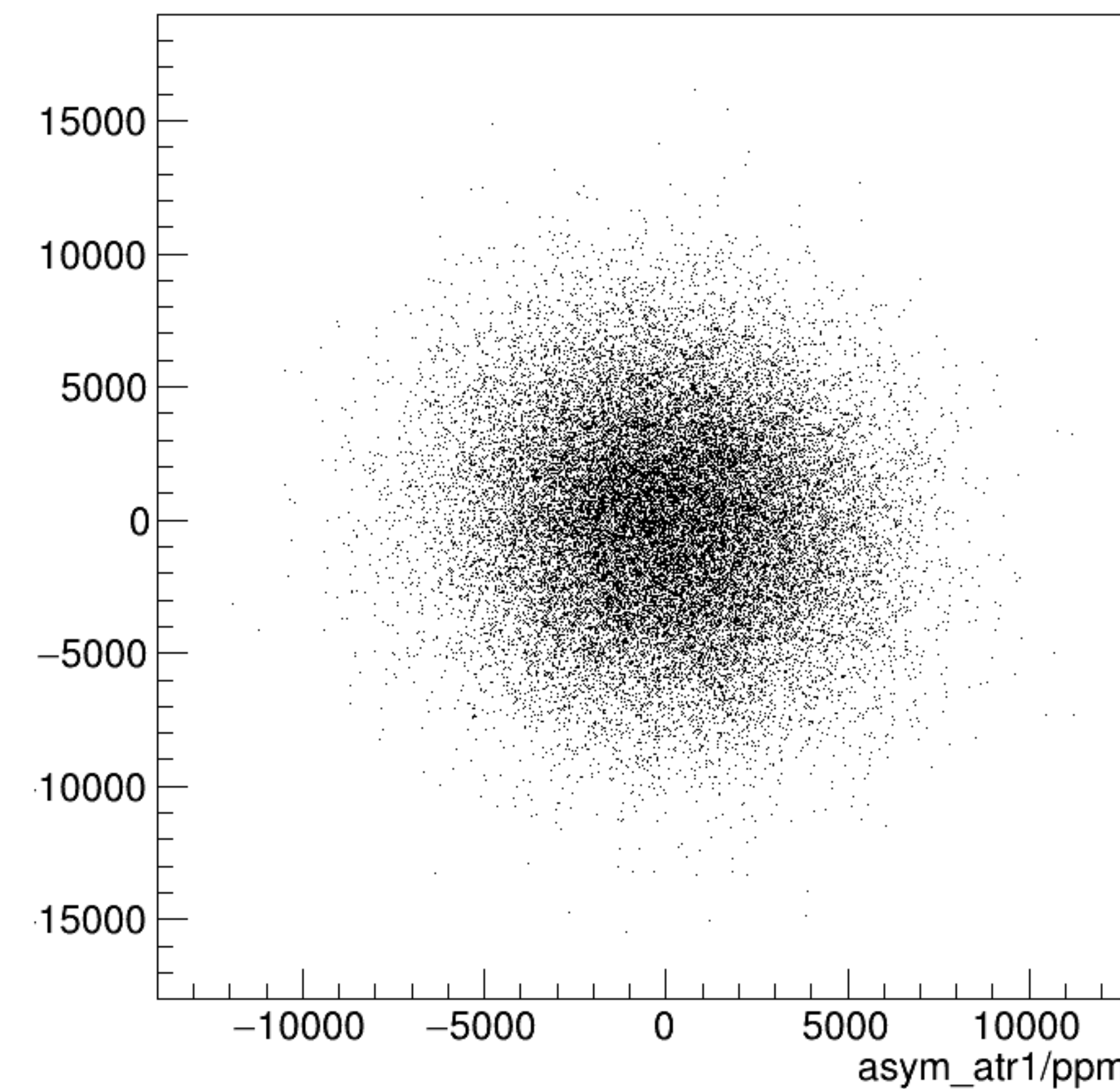
asym_atl1/ppm:asym_atr1/ppm {ok_cut}
