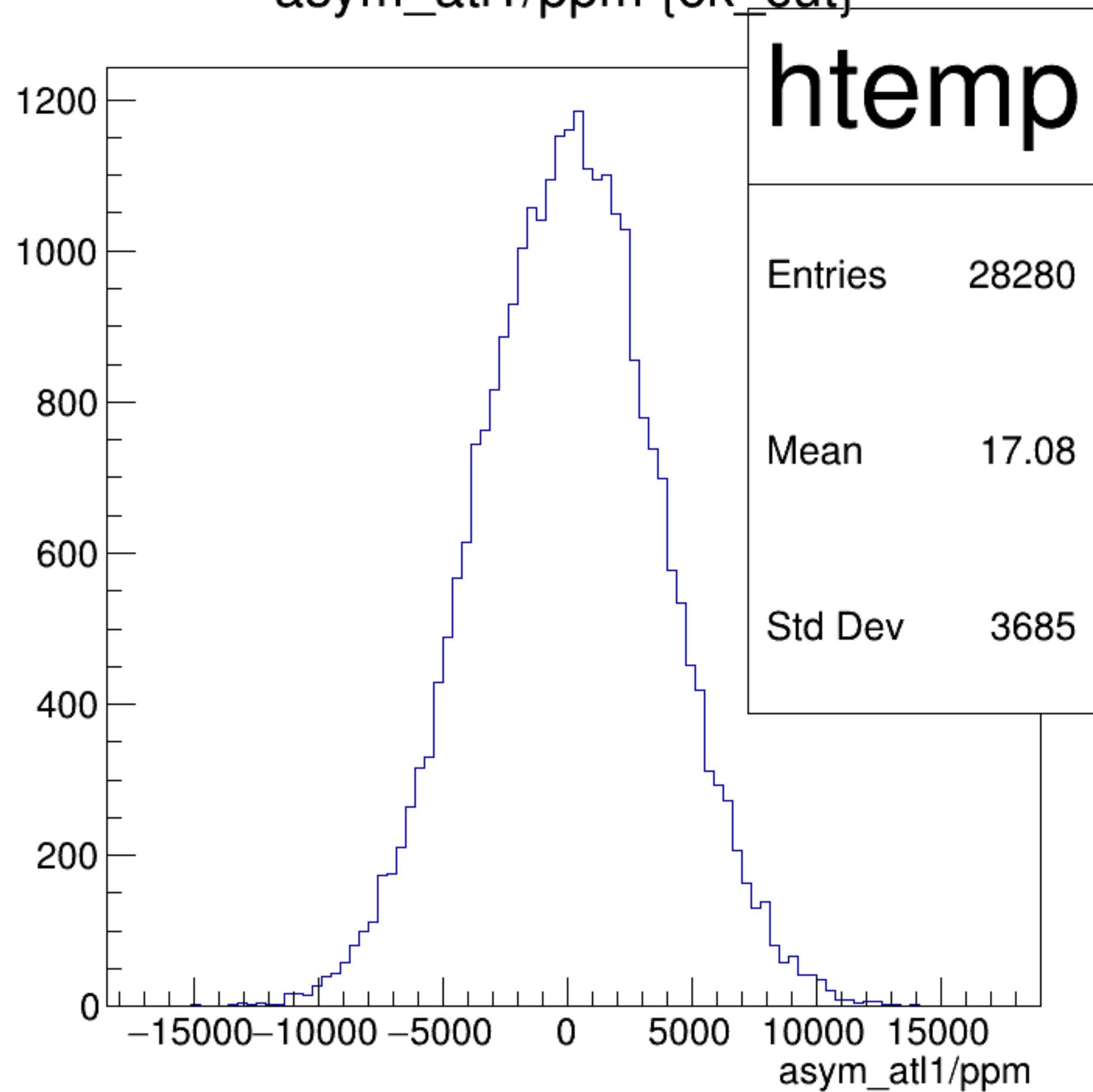
asym_atl1/ppm {ok_cut}
