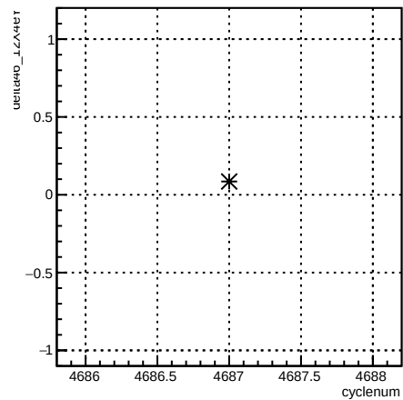
delta46_12X4eY:cyclenum {run == 5655}
