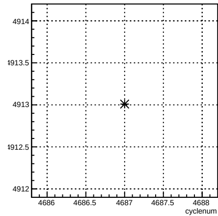
run:cyclenum {run == 5655}
