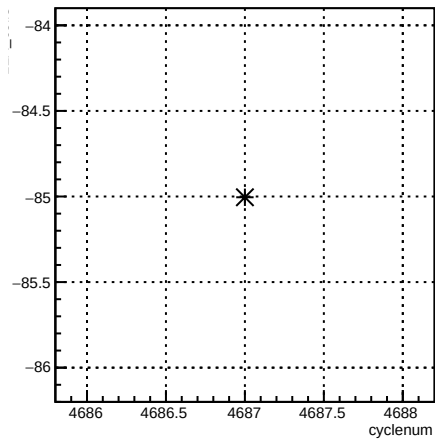
12X_coil7:cyclenum {run == 5655}
