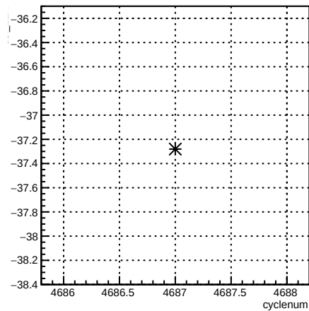
usl_12X:cyclenum {run == 5655}
