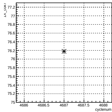
1X_coil7:cyclenum {run == 5655}
