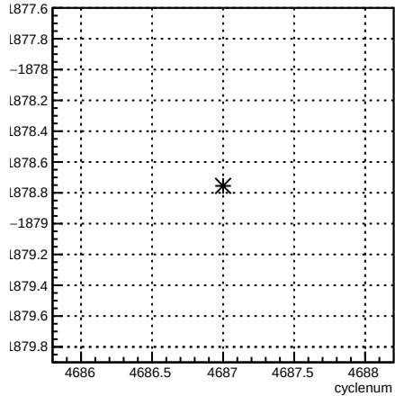
usl_coil6:cyclenum {run == 5655}
