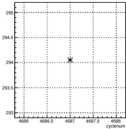
4eY_coil4:cyclenum {run == 5655}
