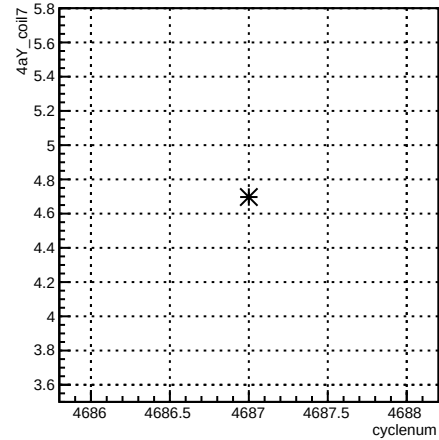
4eY_coil7:cyclenum {run == 5655}
