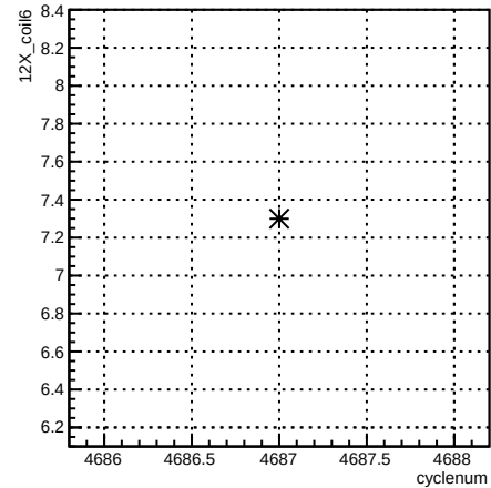
12X_coil6:cyclenum {run == 5655}
