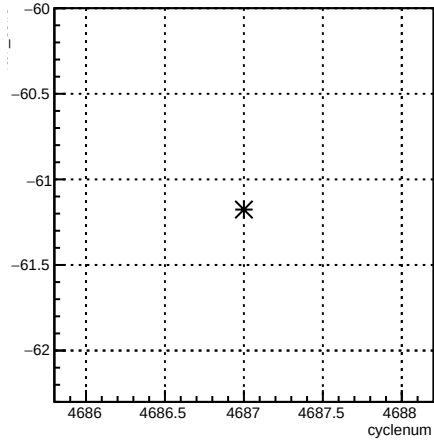
4eY_coil6:cyclenum {run == 5655}
