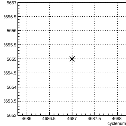
run:cyclenum {run == 5655}
