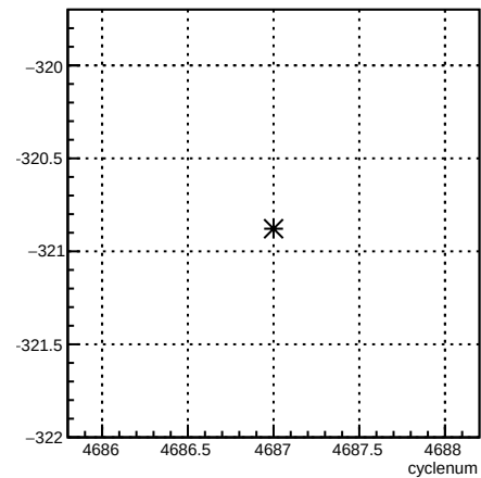
4eX_coil1:cyclenum {run == 5655}
