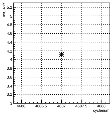
usr_4aY:cyclenum {run == 5655}
