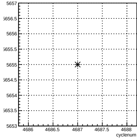
run:cyclenum {run == 5655}
