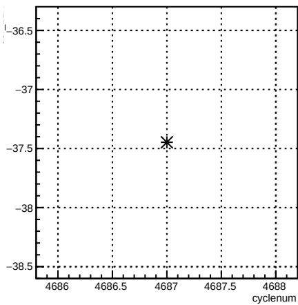
usr_12X:cyclenum {run == 5655}
