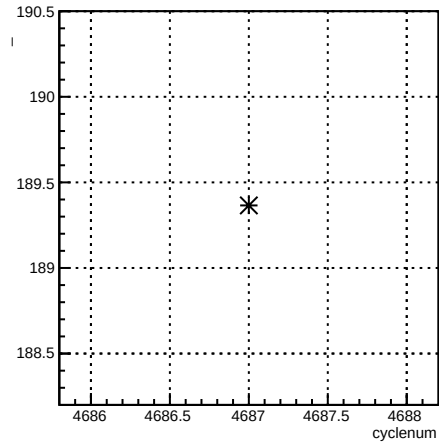
usr_4eX:cyclenum {run == 5655}
