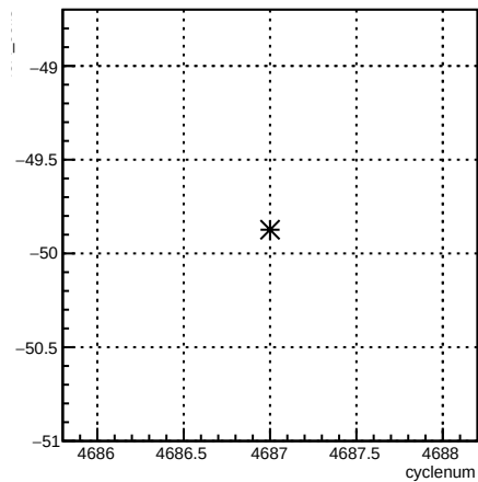
4eX_coil3:cyclenum {run == 5655}
