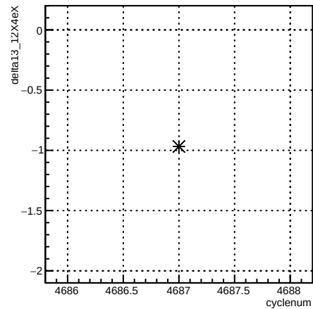
delta13_12X4eX:cyclenum {run == 5655}
