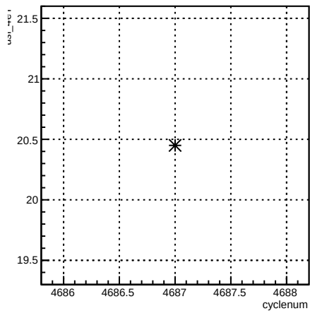
usl_4eY:cyclenum {run == 5655}
