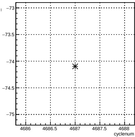
usl_4eY:cyclenum {run == 5655}
