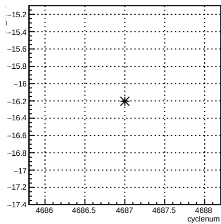
1X_coil3:cyclenum {run == 5655}
