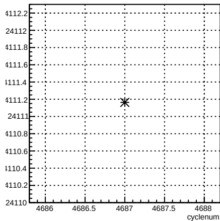
usr_coil7:cyclenum {run == 5655}
