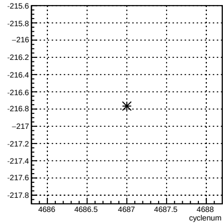
1X_coil1:cyclenum {run == 5655}
