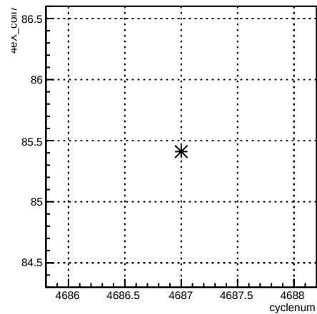
4eX_coil7:cyclenum {run == 5655}
