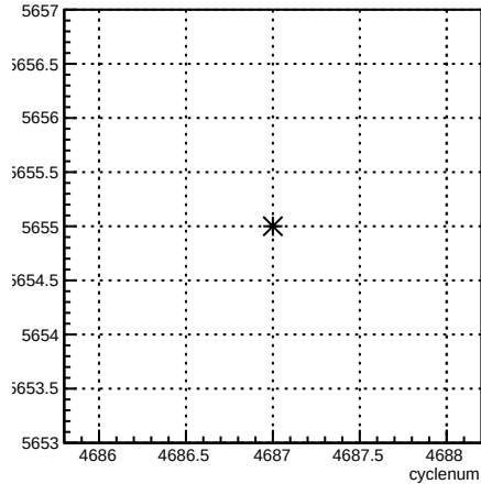
run:cyclenum {run == 5655}
