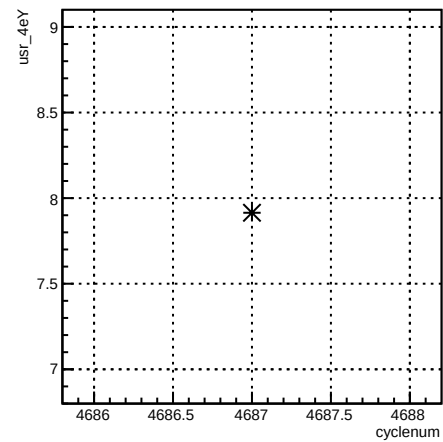
usr_4eY:cyclenum {run == 5655}
