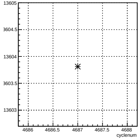
usl_coil7:cyclenum {run == 5655}
