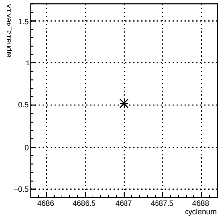
alpha13_4eX1X:cyclenum {run == 5655}
