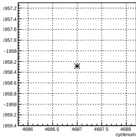
usr_coil6:cyclenum {run == 5655}
