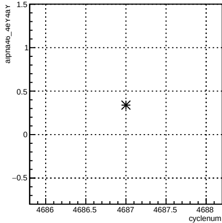
alpha46_4eY4aY:cyclenum {run == 5655}
