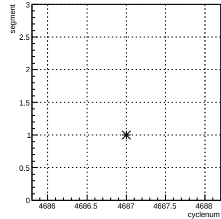
segment:cyclenum {run == 5655}
