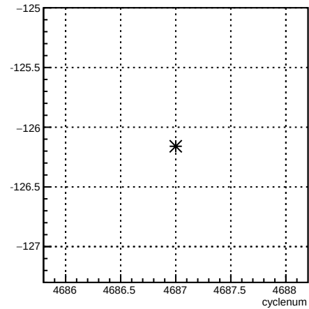
usr_1X:cyclenum {run == 5655}
