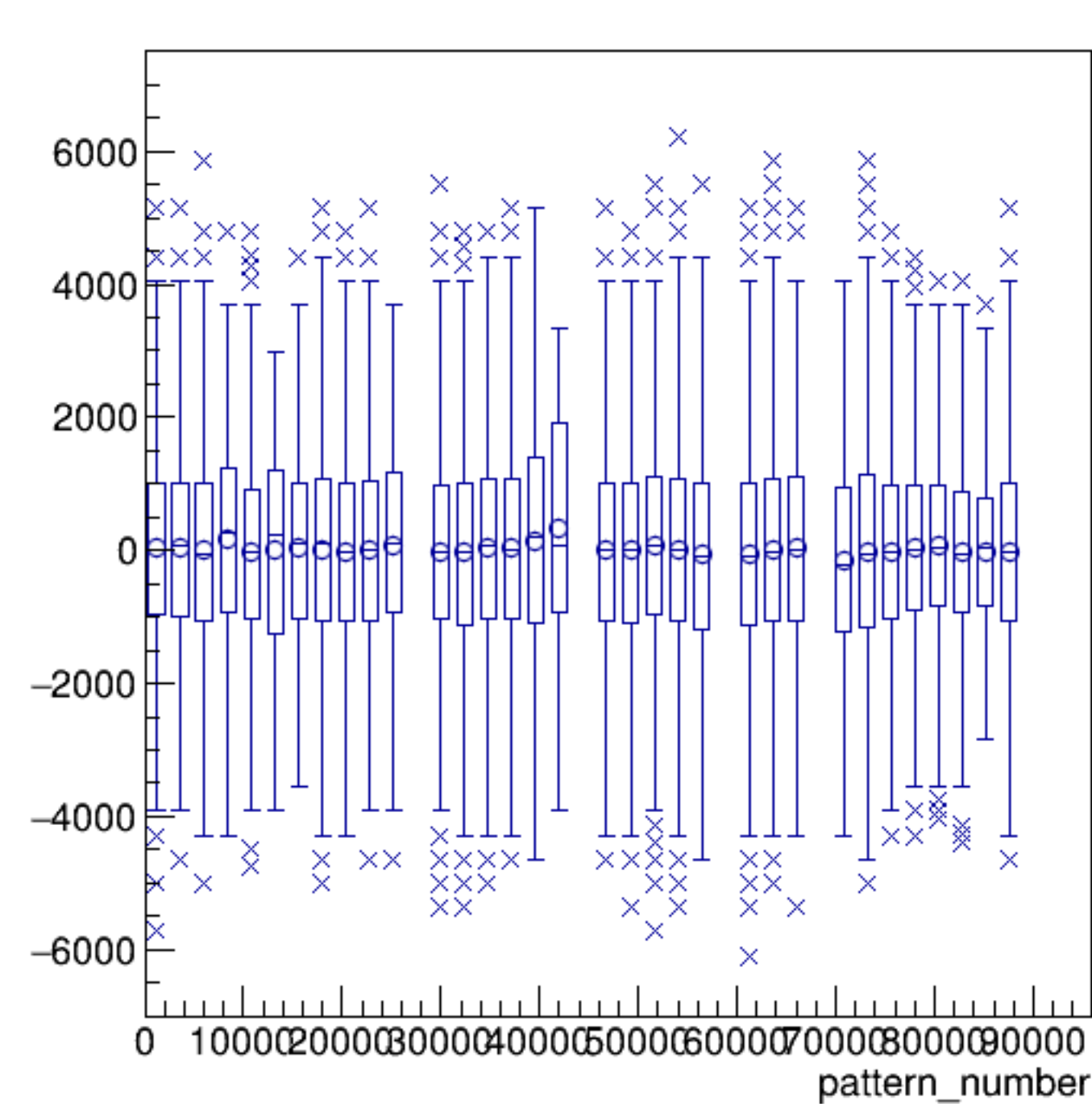
asym_sam4/ppm:pattern_number {ErrorFlag==0}
