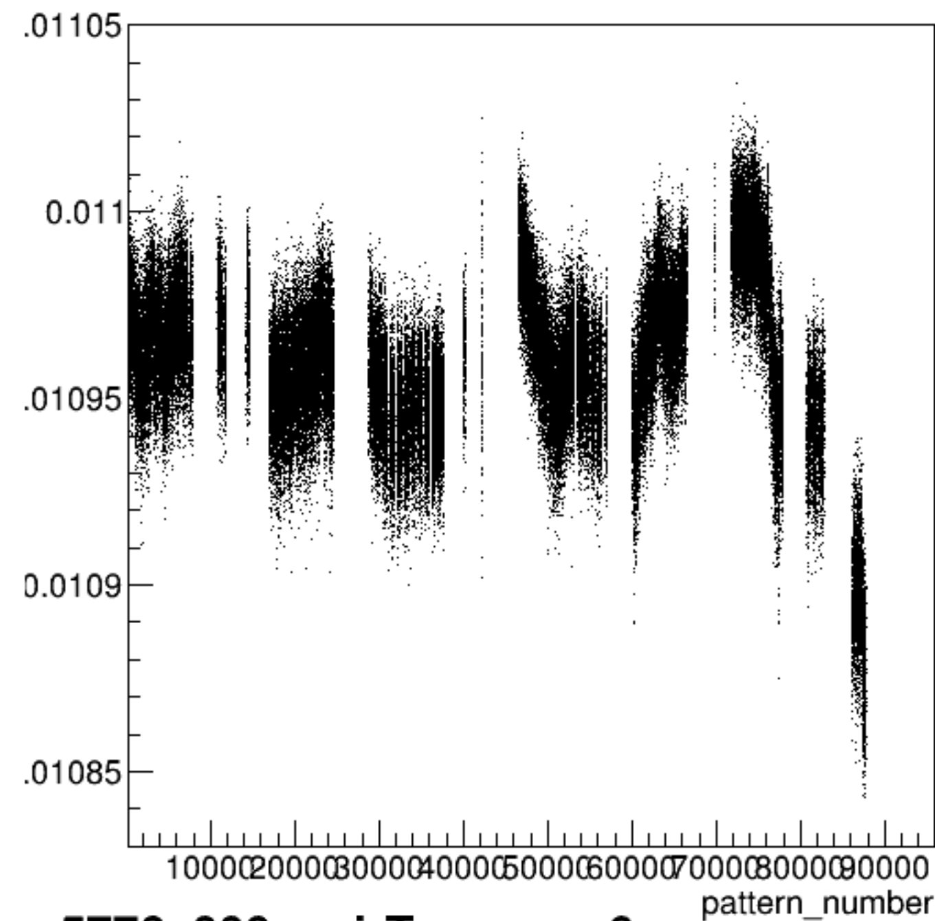
yield_sam6:pattern_number {ErrorFlag==0}
