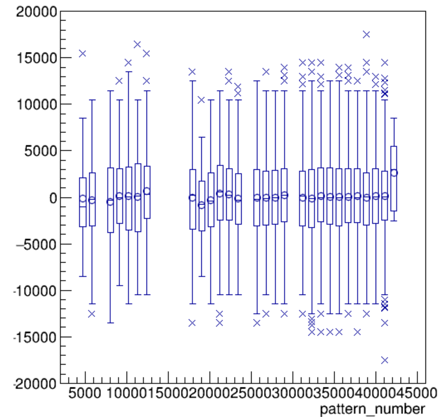
asym_atl1/ppm:pattern_number {ErrorFlag==0}
