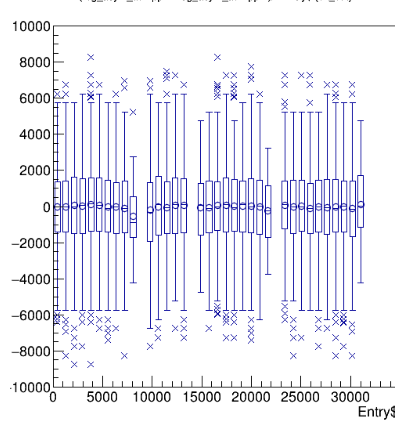
(reg_asym_atl1/ppm+reg_asym_atr1/ppm)/2:Entry$ {ok_cut}
