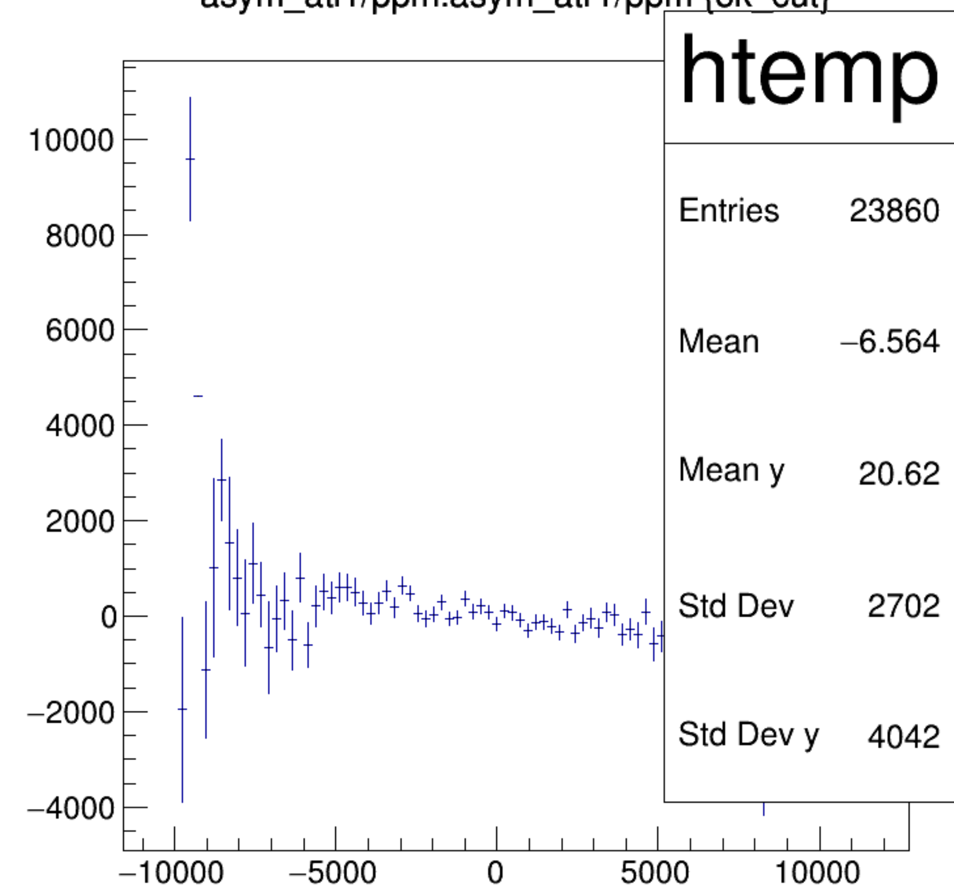
asym_atl1/ppm:asym_atr1/ppm {ok_cut}
