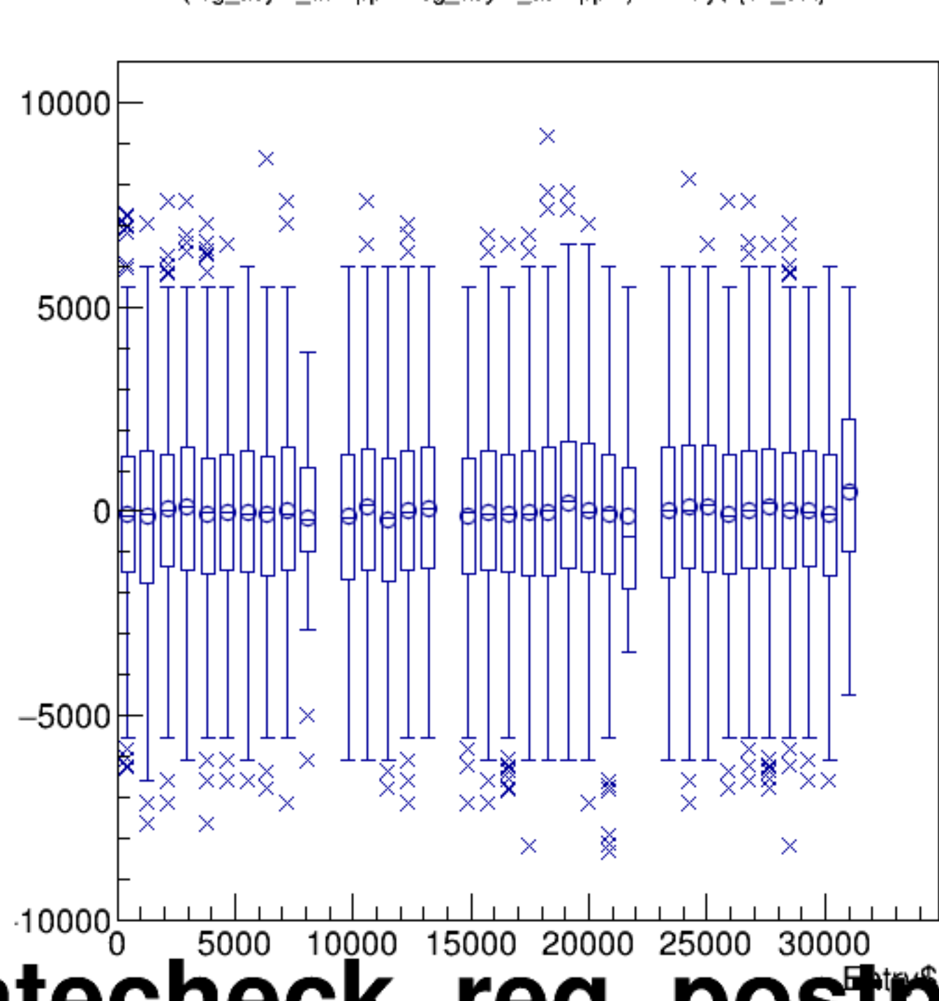
(reg_asym_atl1/ppm-reg_asym_atr1/ppm)/2:Entry$ {ok_cut}
