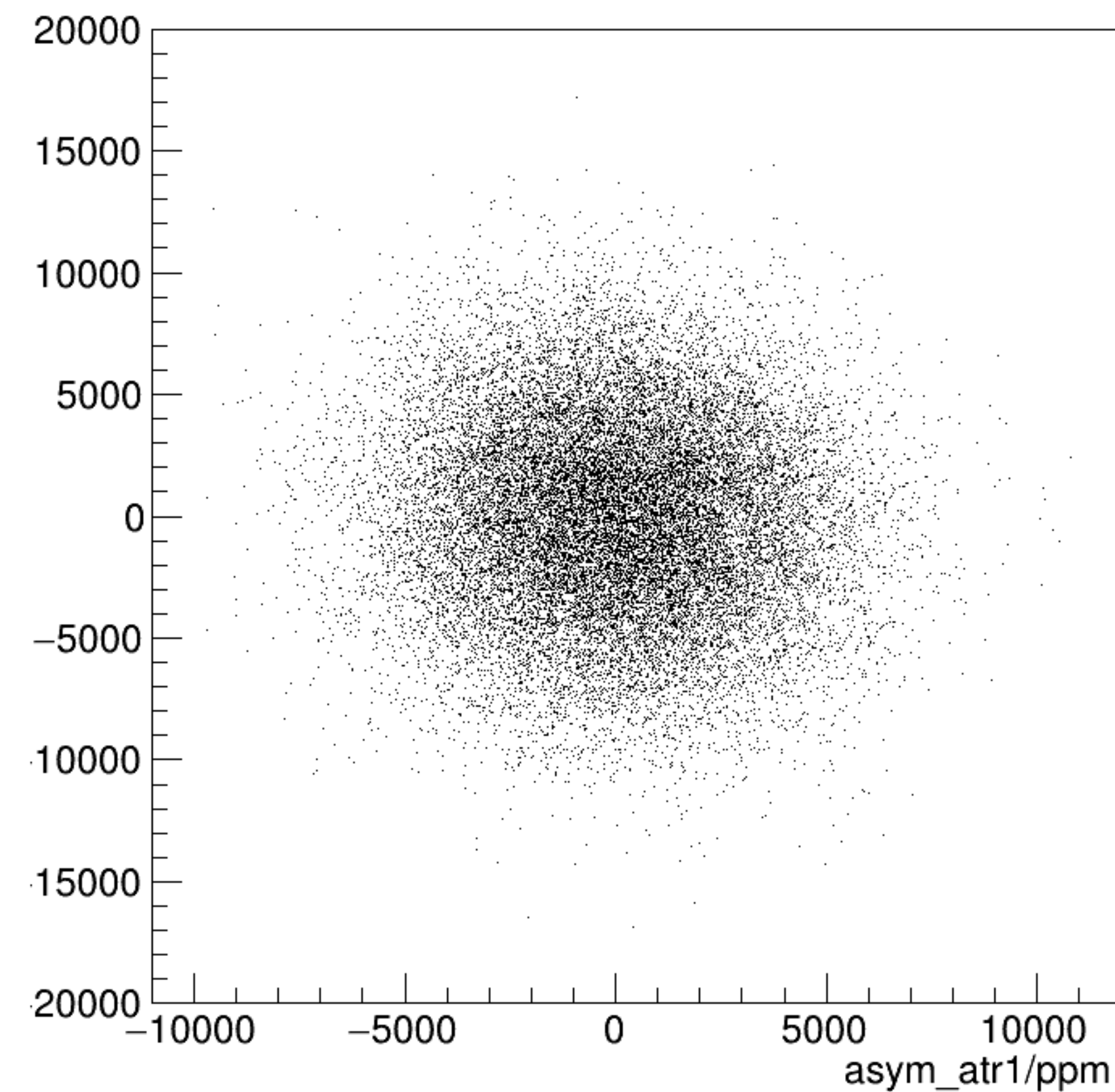
asym_atl1/ppm:asym_atr1/ppm {ok_cut}
