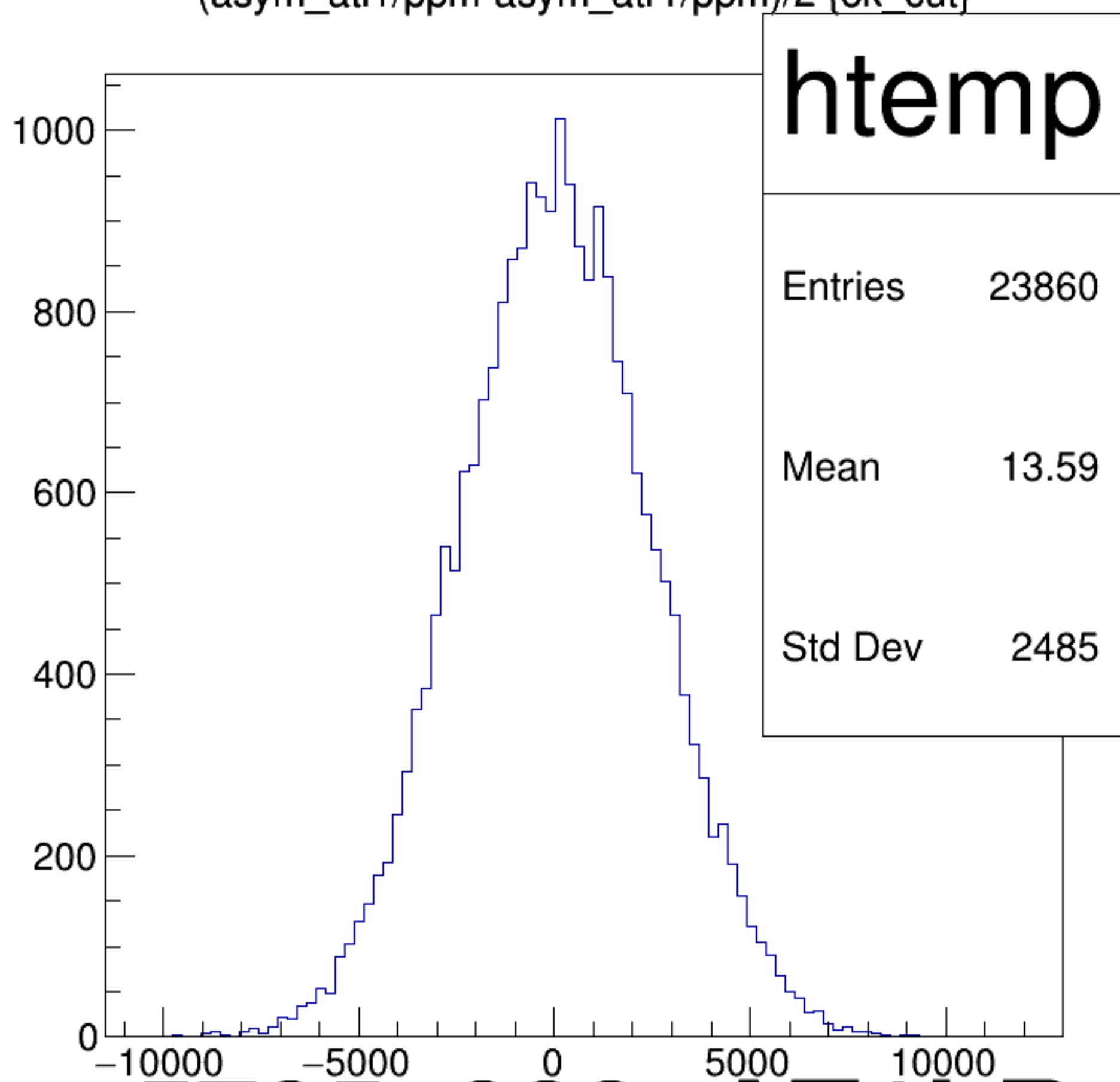
(asym_atl1/ppm-asym_atr1/ppm)/2 {ok_cut}
