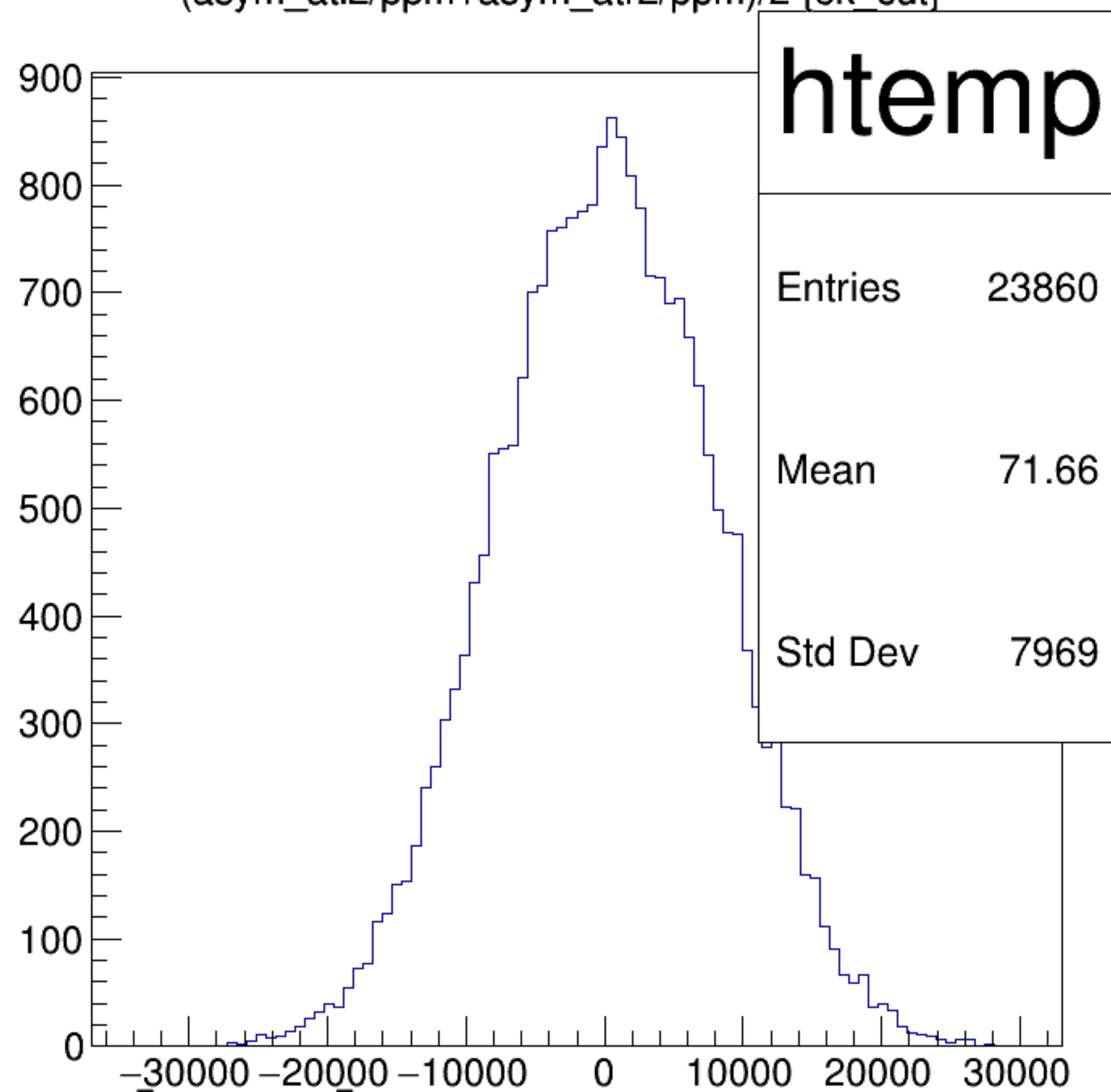
(asym_atl2/ppm+asym_atr2/ppm)/2 {ok_cut}
