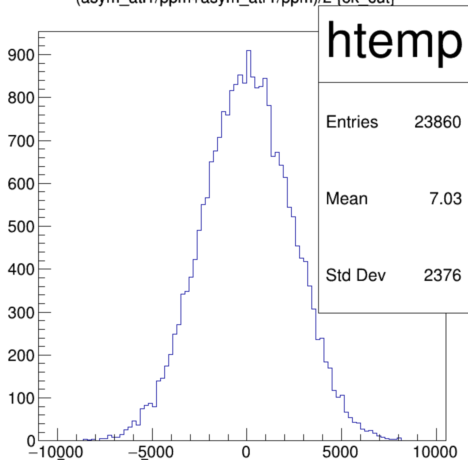
(asym_atl1/ppm+asym_atr1/ppm)/2 {ok_cut}
