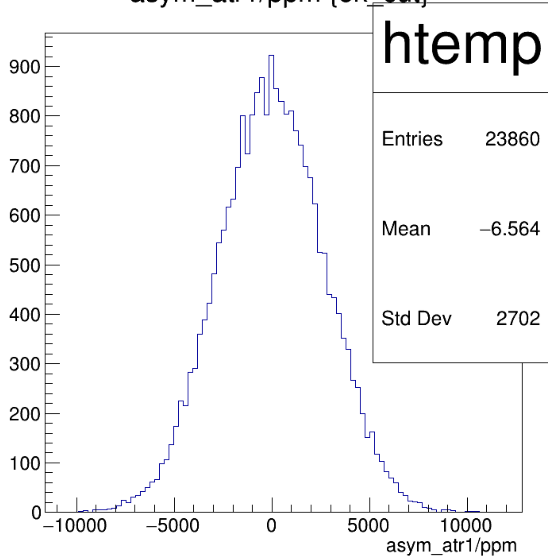
asym_atr1/ppm {ok_cut}
