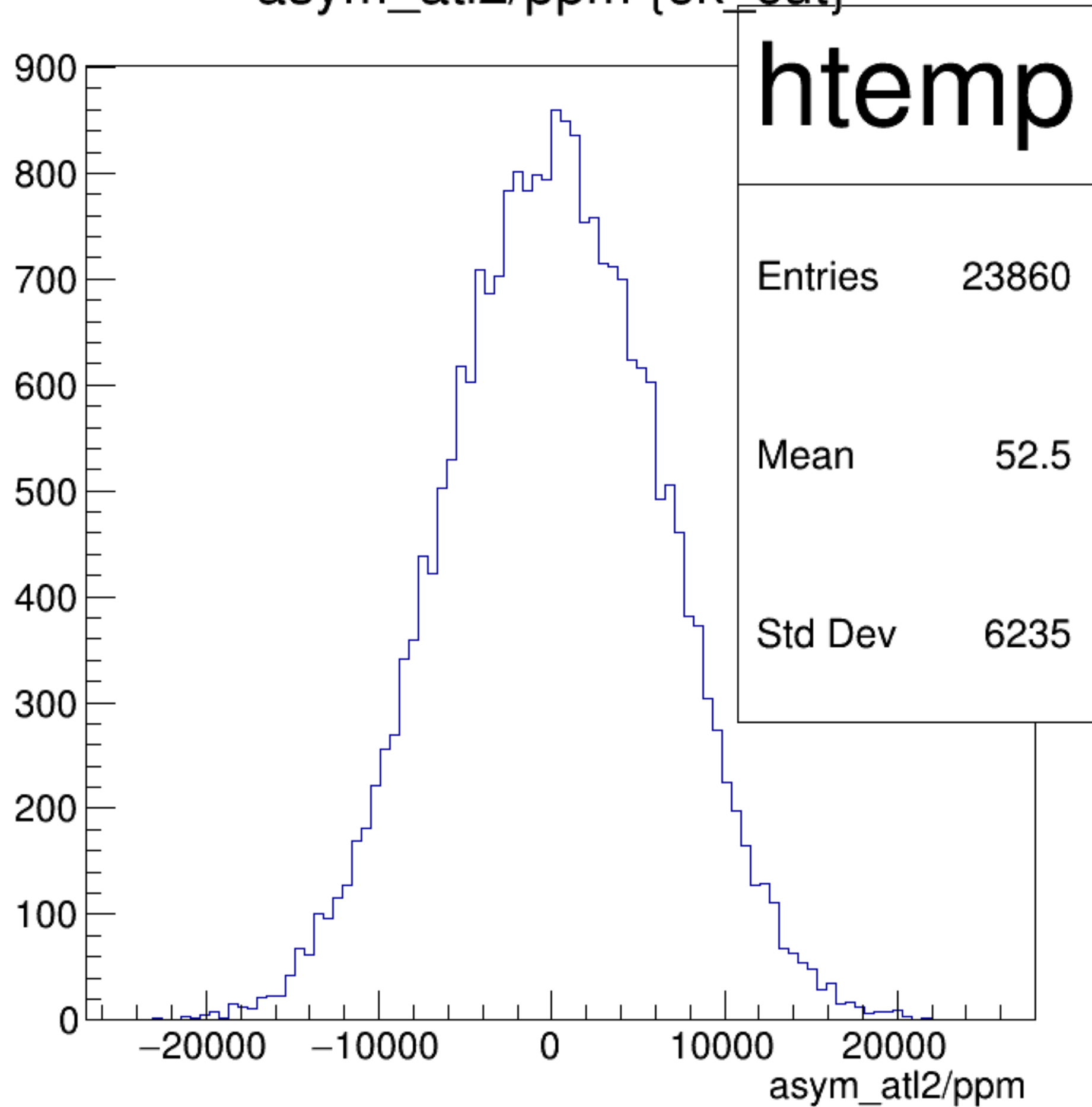
asym_atl2/ppm {ok_cut}
