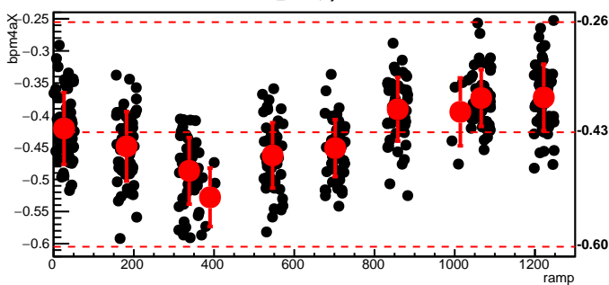
bmod_trim3,cyc=4895
