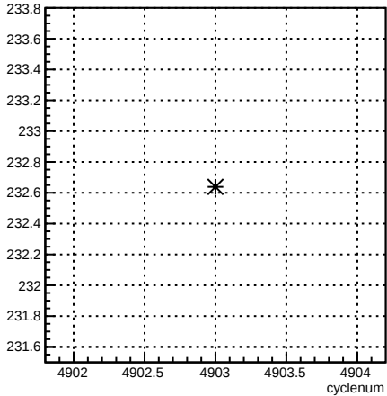
4eY_coil4:cyclenum {run == 5798}
