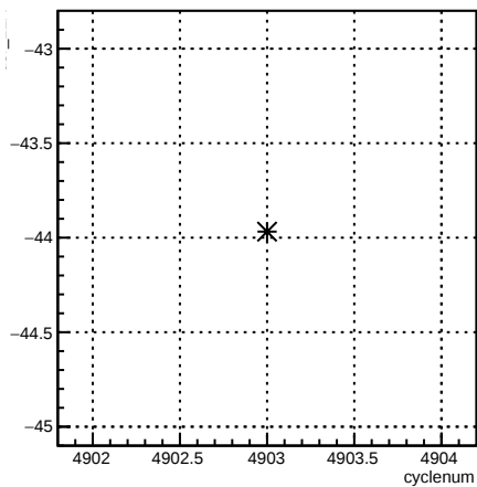
usr_12X:cyclenum {run == 5798}
