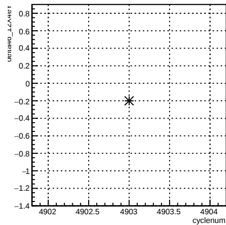
delta46_12X4eY:cyclenum {run == 5798}
