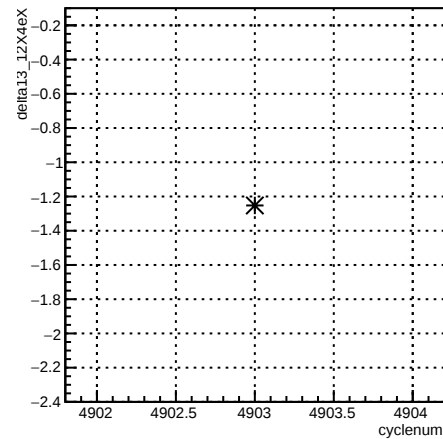
delta13_12X4eX:cyclenum {run == 5798}
