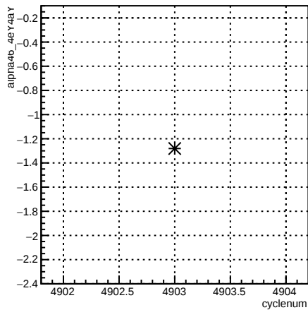
alpha46_4eY4aY:cyclenum {run == 5798}
