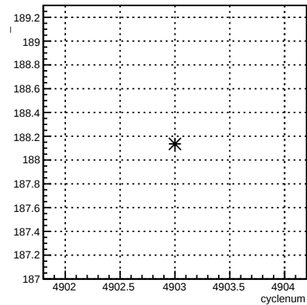
4eX_coil7:cyclenum {run == 5798}
