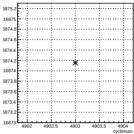
usl_coil7:cyclenum {run == 5798}
