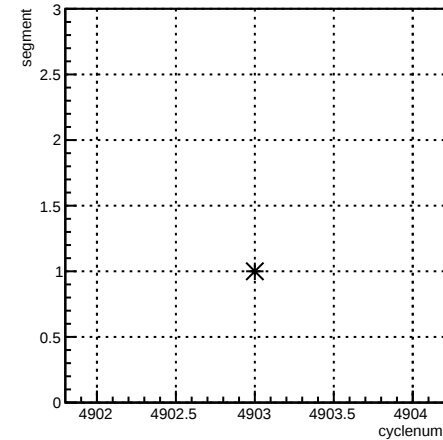
segment:cyclenum {run == 5798}
