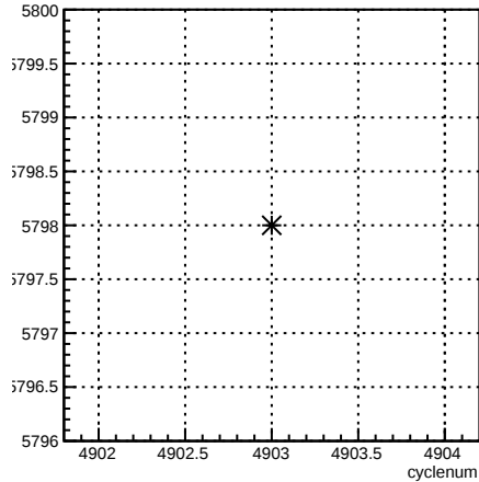
run:cyclenum {run == 5798}
