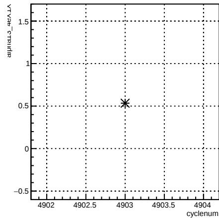
alpha13_4eX1X:cyclenum {run == 5798}
