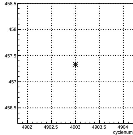
usl_coil6:cyclenum {run == 5798}
