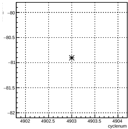
12X_coil7:cyclenum {run == 5798}
