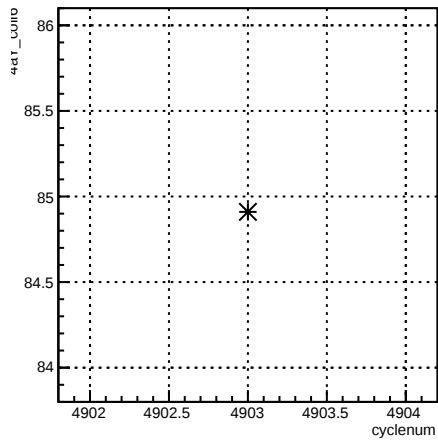
4eY_coil6:cyclenum {run == 5798}
