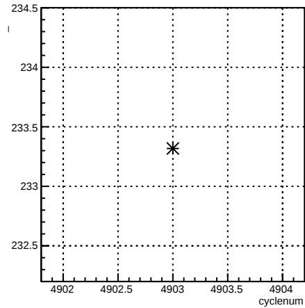
usr_4eX:cyclenum {run == 5798}
