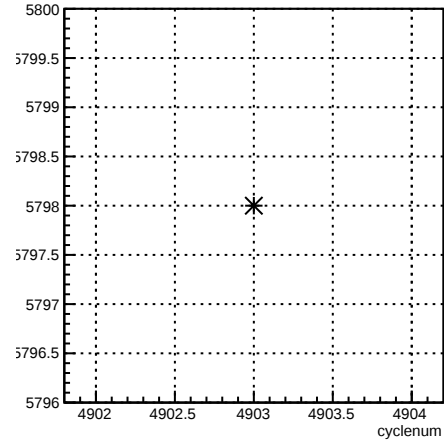
run:cyclenum {run == 5798}
