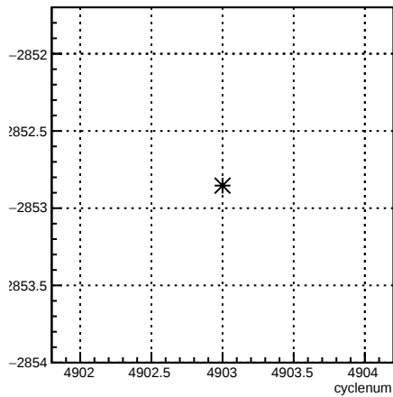
usr_coil7:cyclenum {run == 5798}
