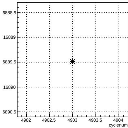
usr_coil6:cyclenum {run == 5798}
