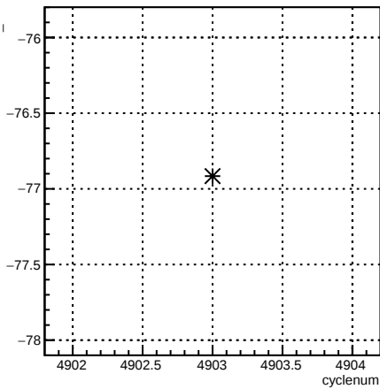
usl_4eY:cyclenum {run == 5798}
