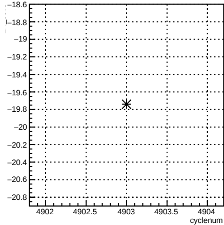
4eX_coil3:cyclenum {run == 5798}
