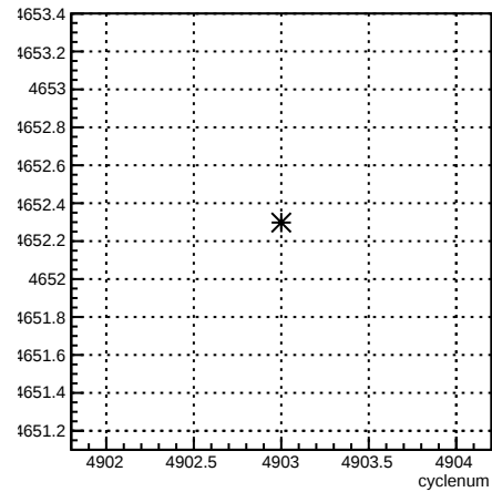
usr_coil4:cyclenum {run == 5798}
