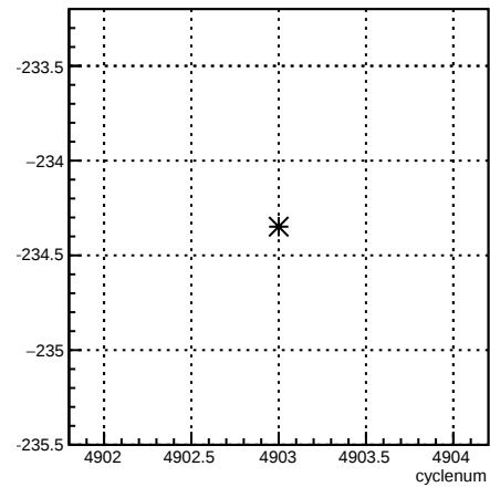
12X_coil6:cyclenum {run == 5798}
