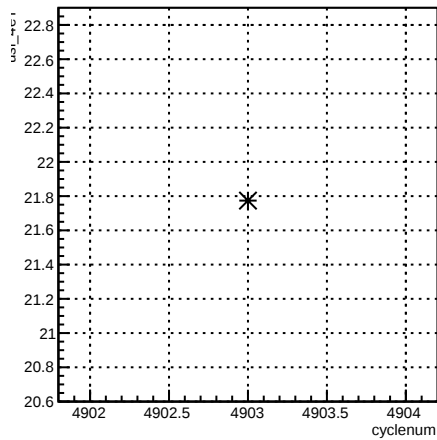
usl_4eY:cyclenum {run == 5798}
