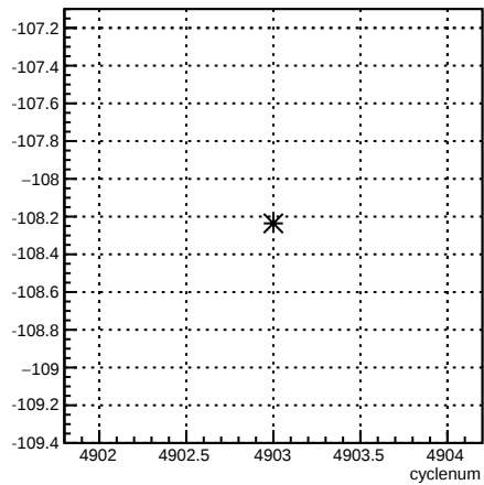
usr_4eY:cyclenum {run == 5798}
