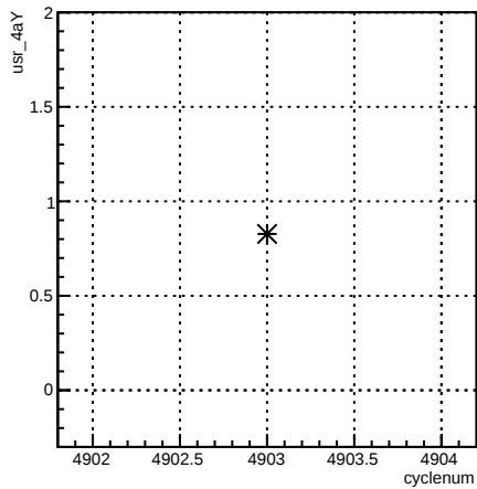
usr_4aY:cyclenum {run == 5798}
