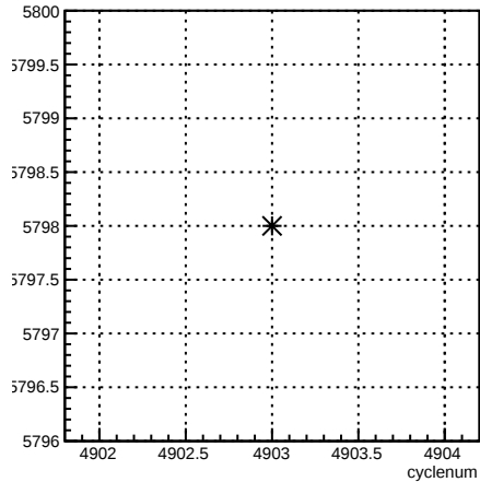
run:cyclenum {run == 5798}
