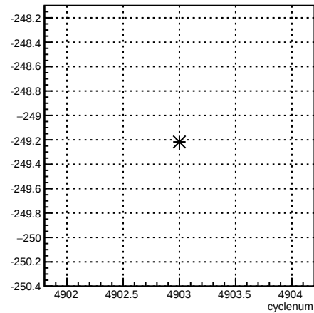
4eX_coil1:cyclenum {run == 5798}
