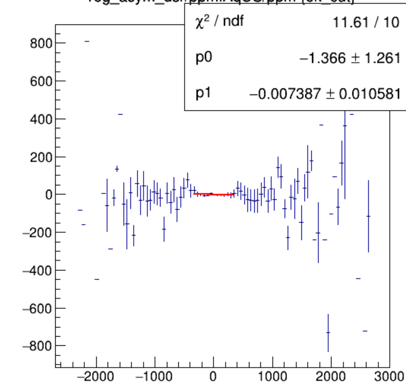
reg_asym_dsr/ppm:AqUS/ppm {ok_cut}
