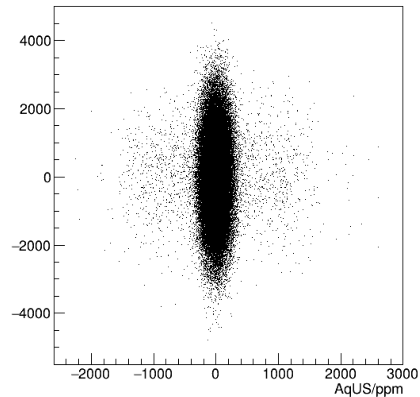
reg_asym_usr/ppm:AqUS/ppm {ok_cut}
