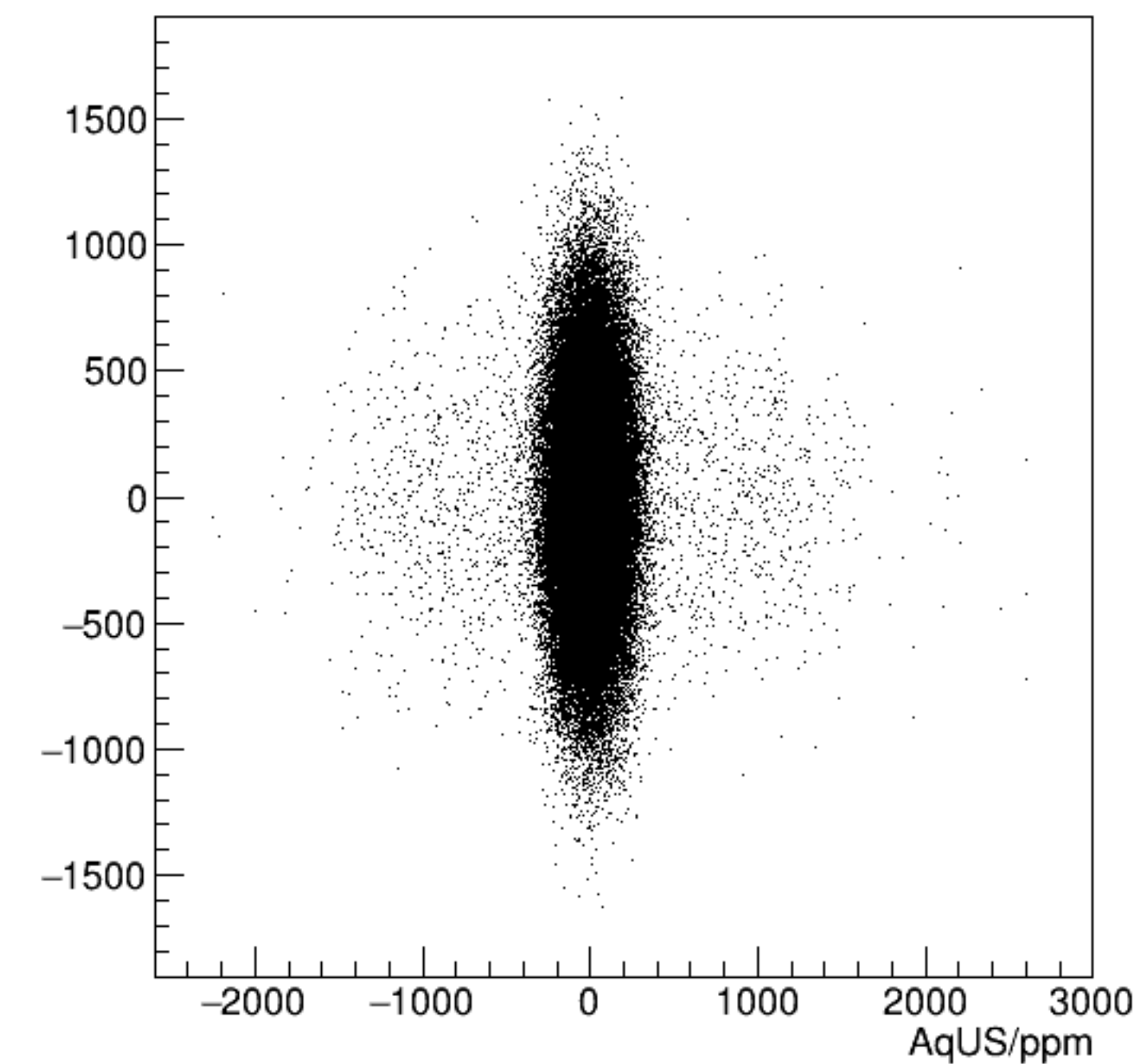
reg_asym_dsr/ppm:AqUS/ppm {ok_cut}
