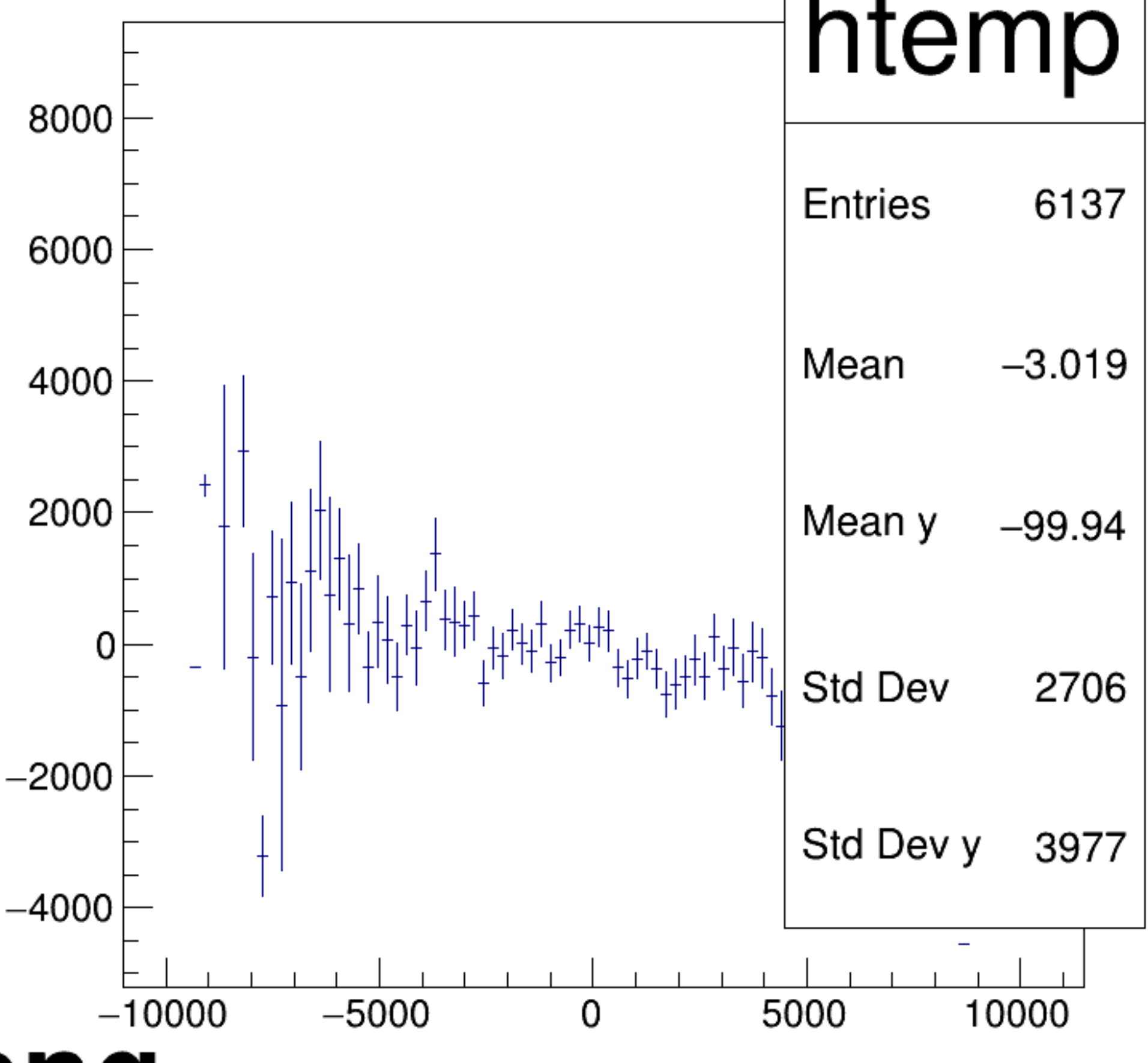
asym_atl1/ppm:asym_atr1/ppm {ok_cut}
