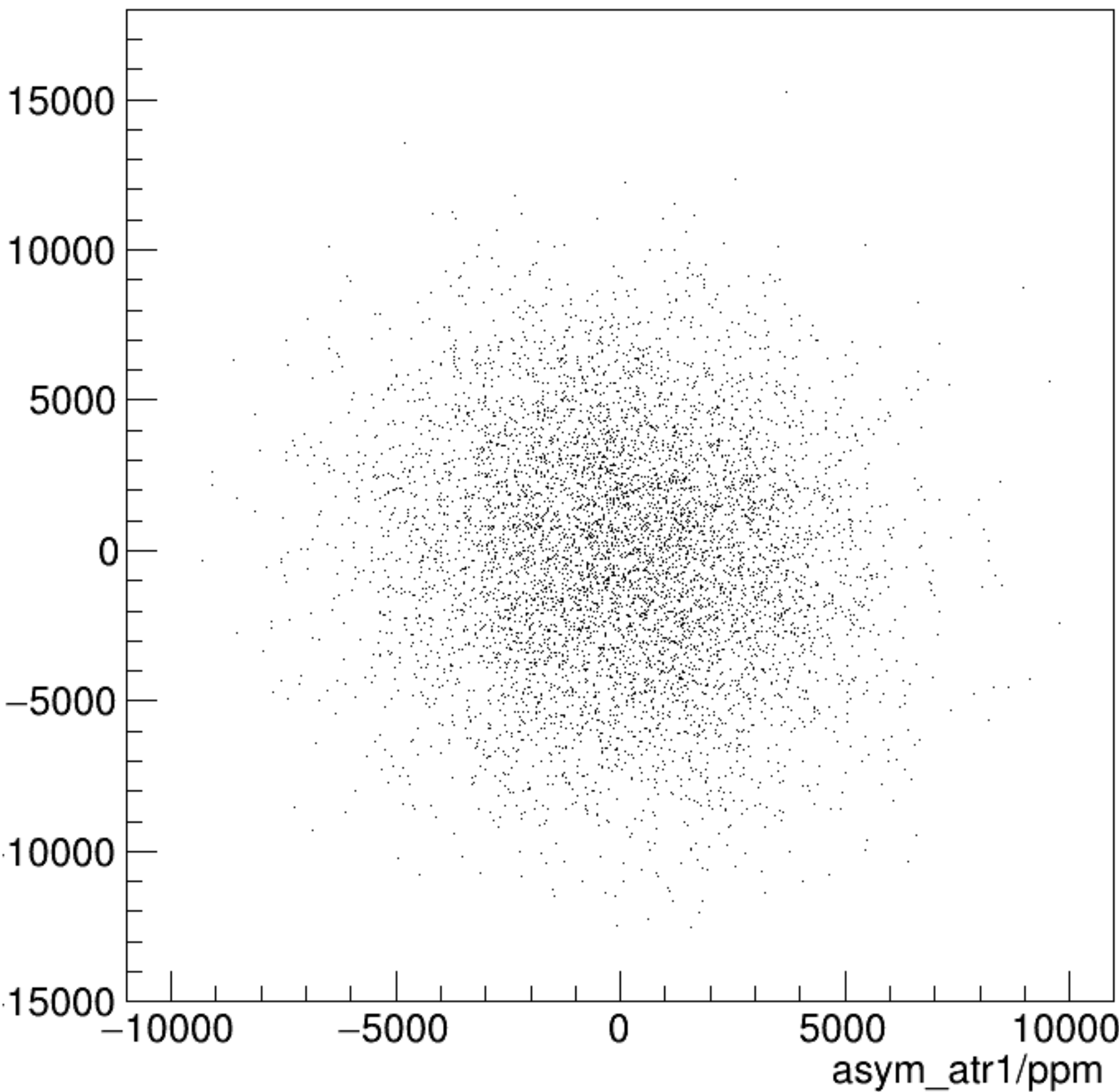
asym_atl1/ppm:asym_atr1/ppm {ok_cut}
