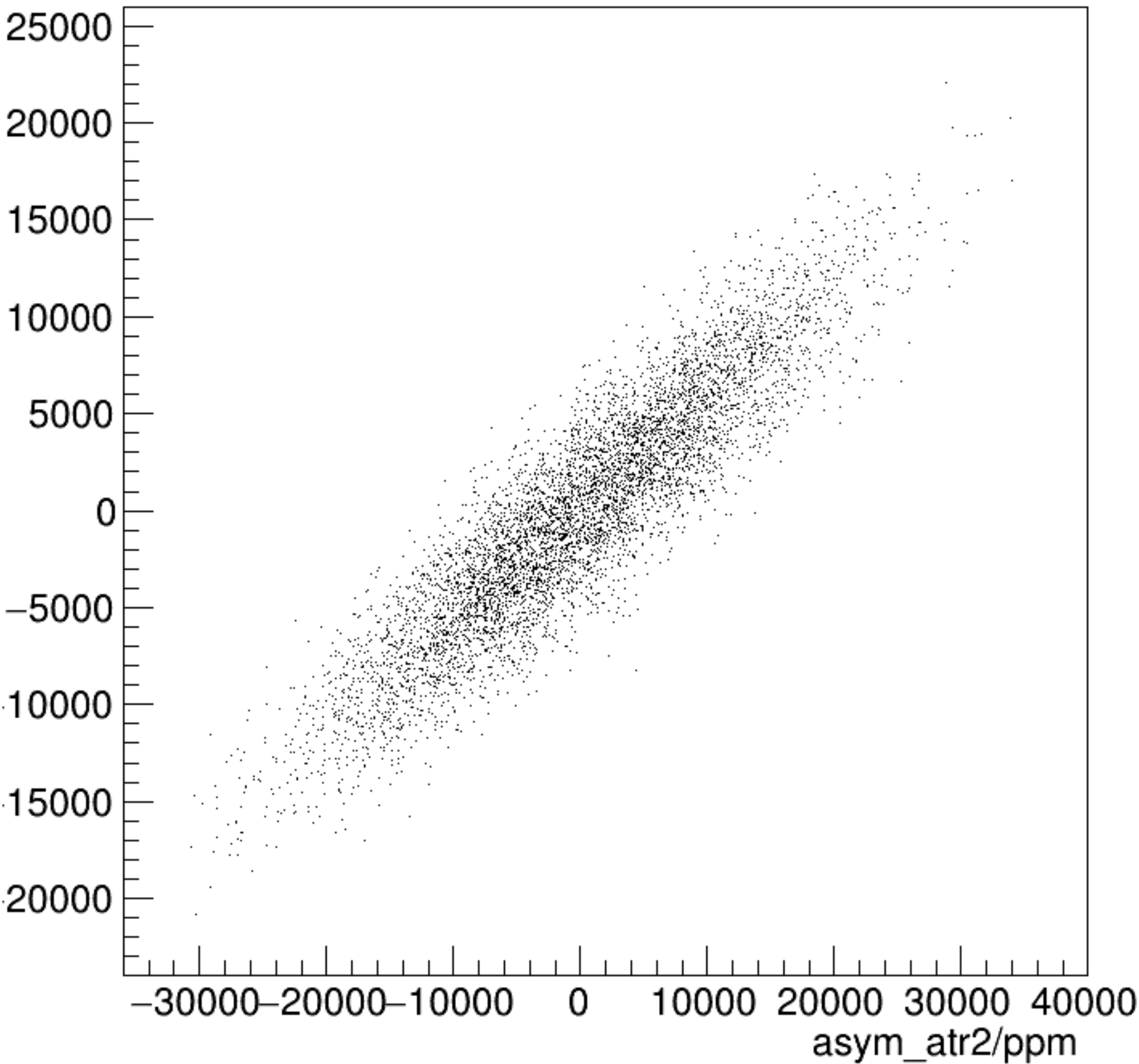
asym_atl2/ppm:asym_atr2/ppm {ok_cut}
