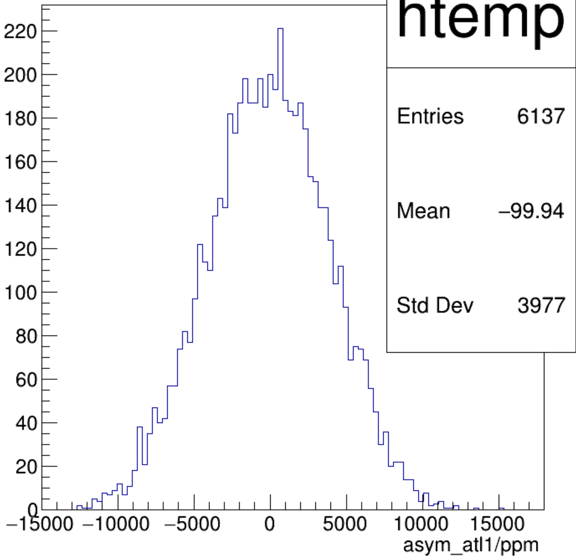
asym_atl1/ppm {ok_cut}
