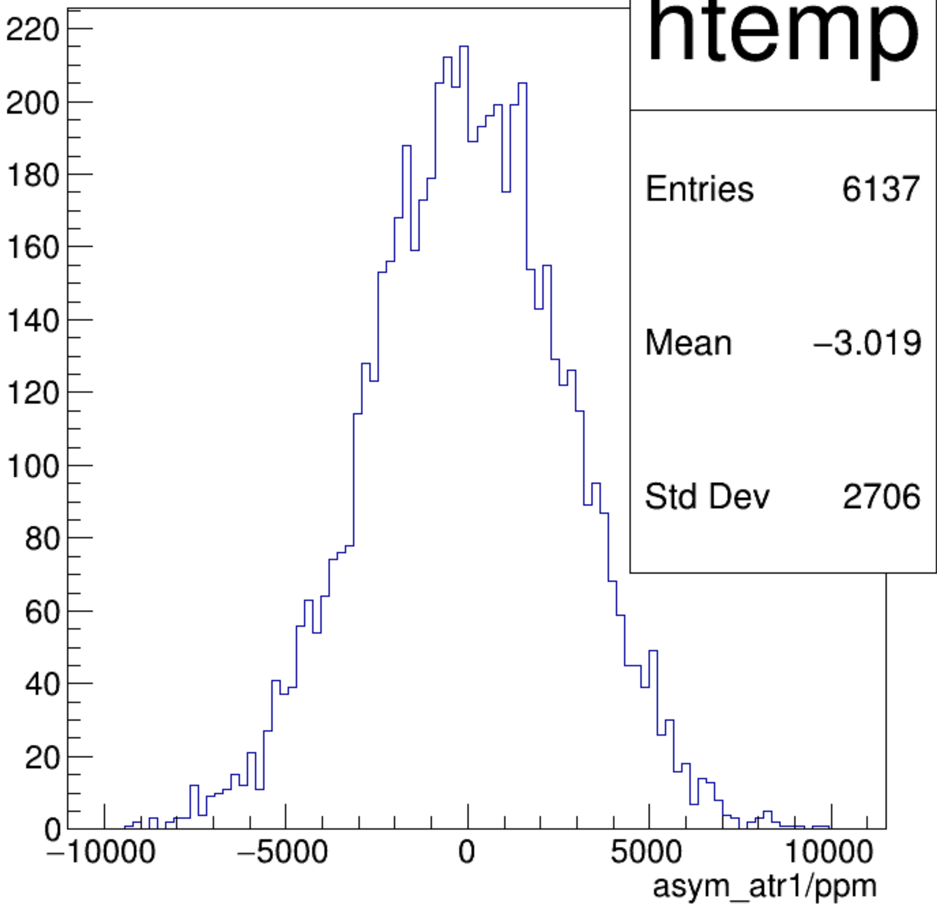
asym_atr1/ppm {ok_cut}
