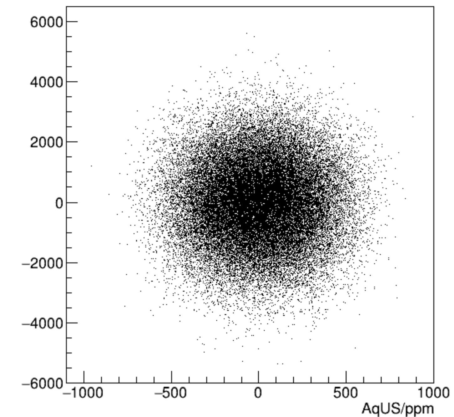
reg_asym_usl/ppm:AqUS/ppm {ok_cut}
