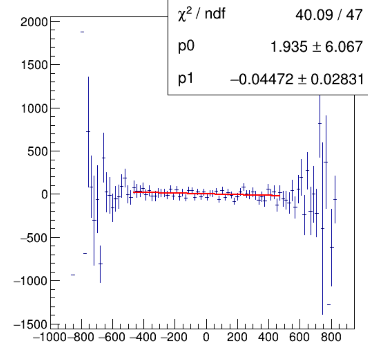
reg_asym_usr/ppm:AqDS/ppm {ok_cut}
