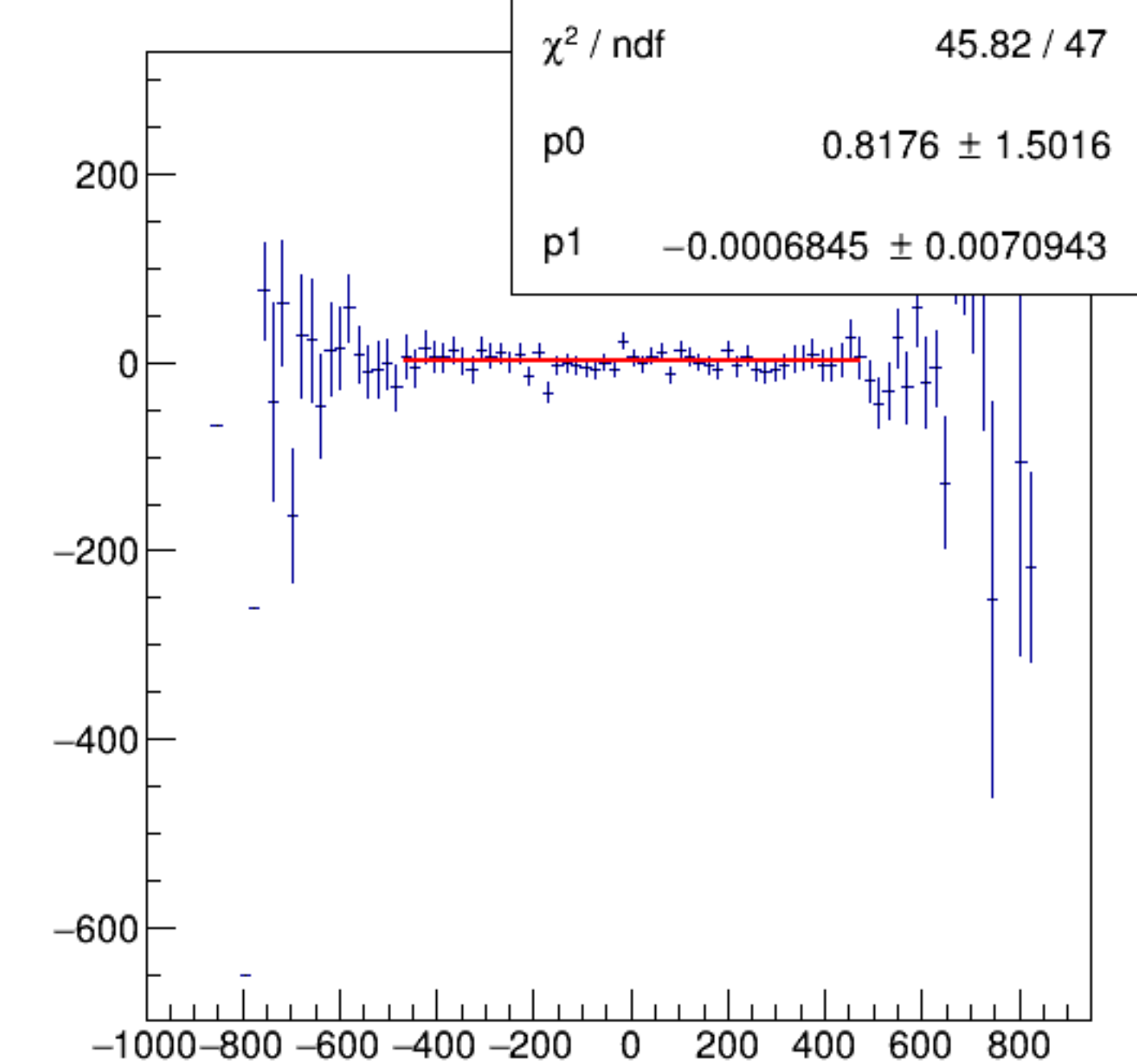
reg_asym_dsl/ppm:AqDS/ppm {ok_cut}
