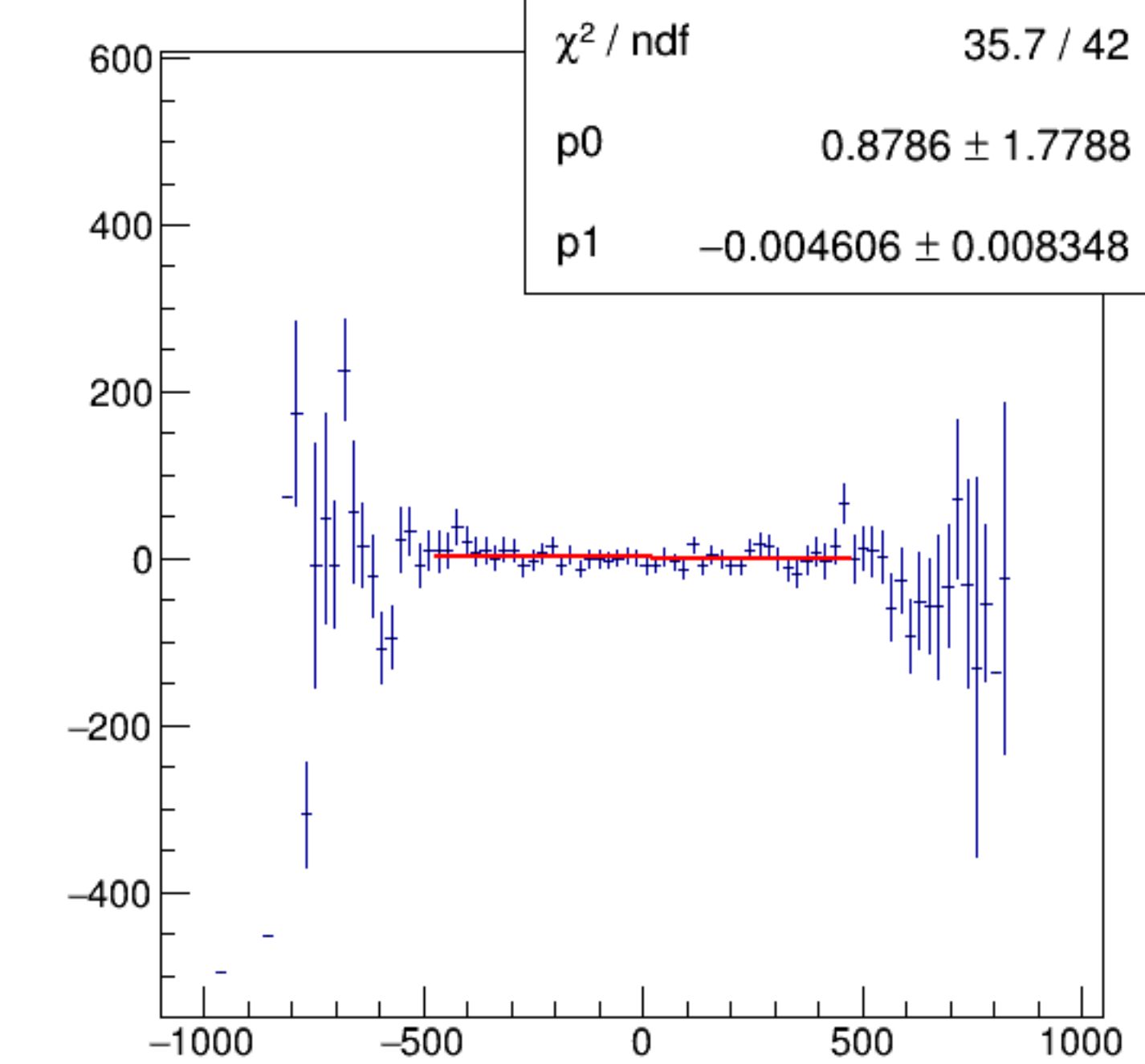
reg_asym_dsr/ppm:AqUS/ppm {ok_cut}
