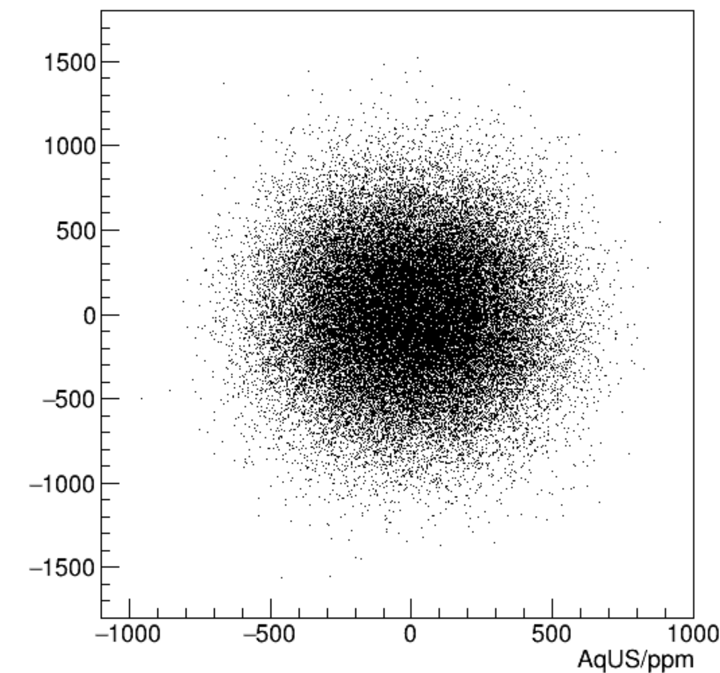
reg_asym_dsr/ppm:AqUS/ppm {ok_cut}
