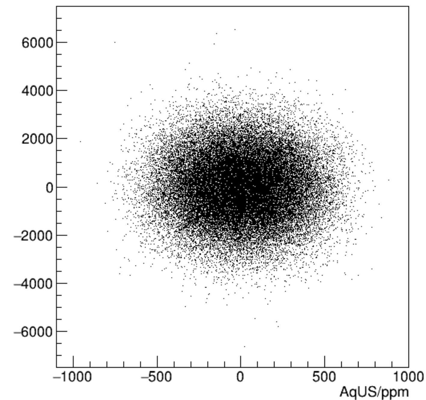
reg_asym_usr/ppm:AqUS/ppm {ok_cut}
