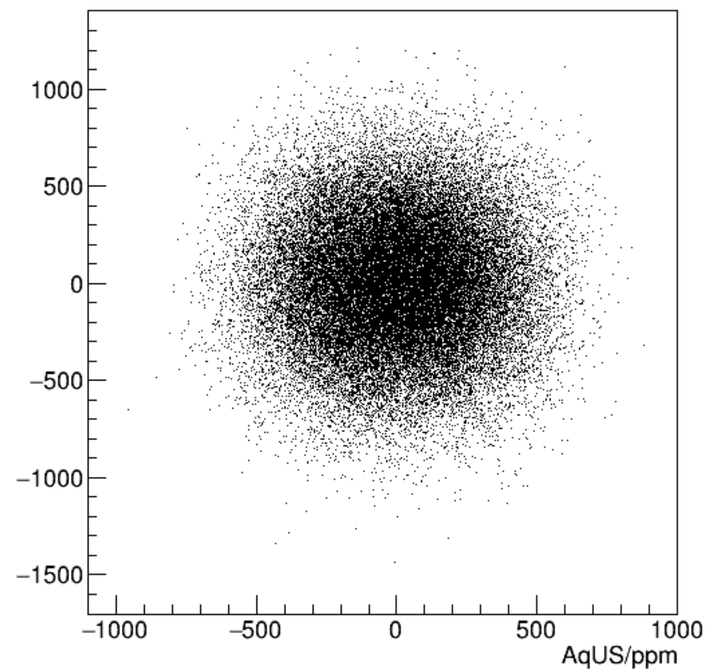
reg_asym_dsl/ppm:AqUS/ppm {ok_cut}
