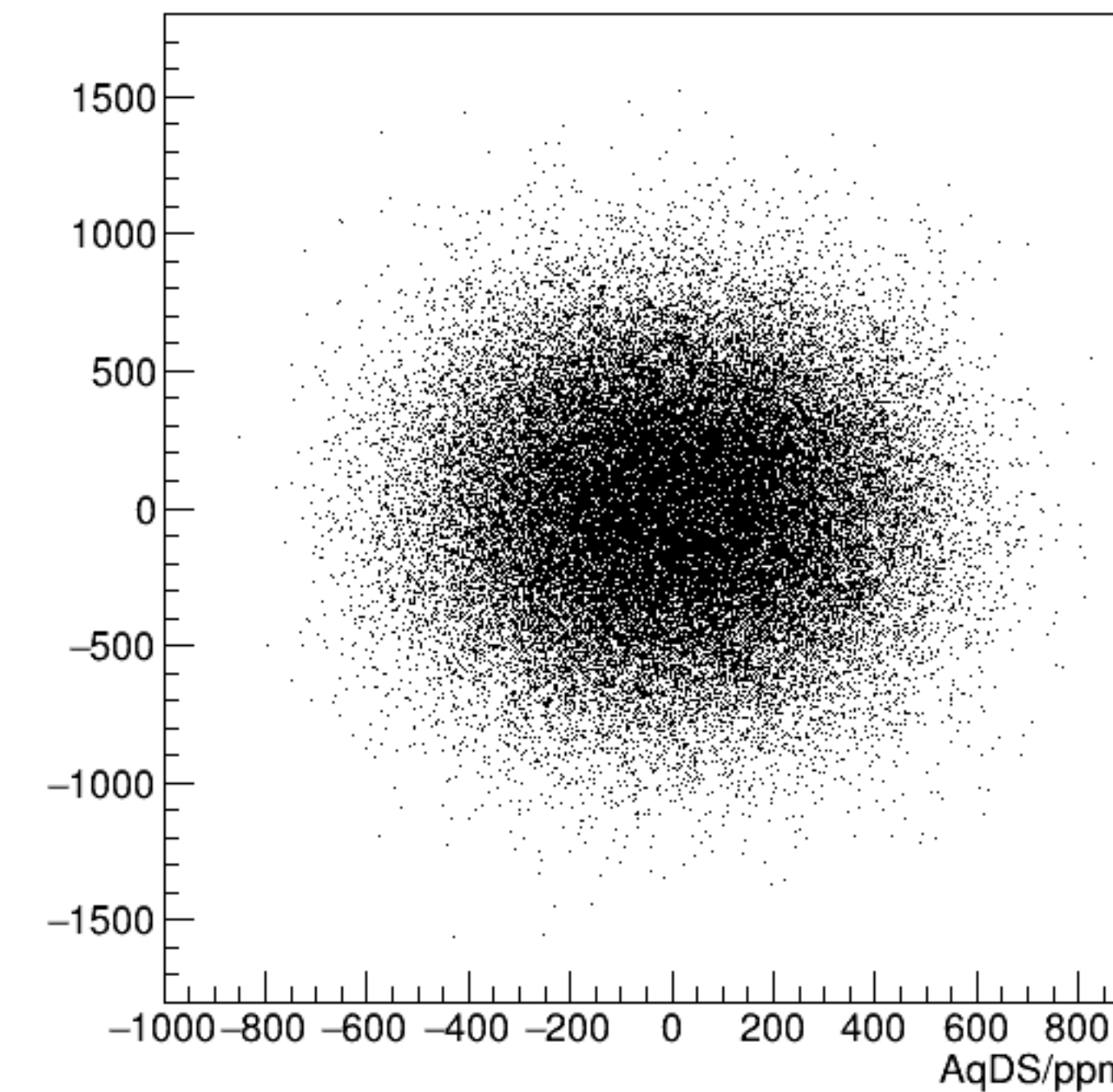
reg_asym_dsr/ppm:AqDS/ppm {ok_cut}
