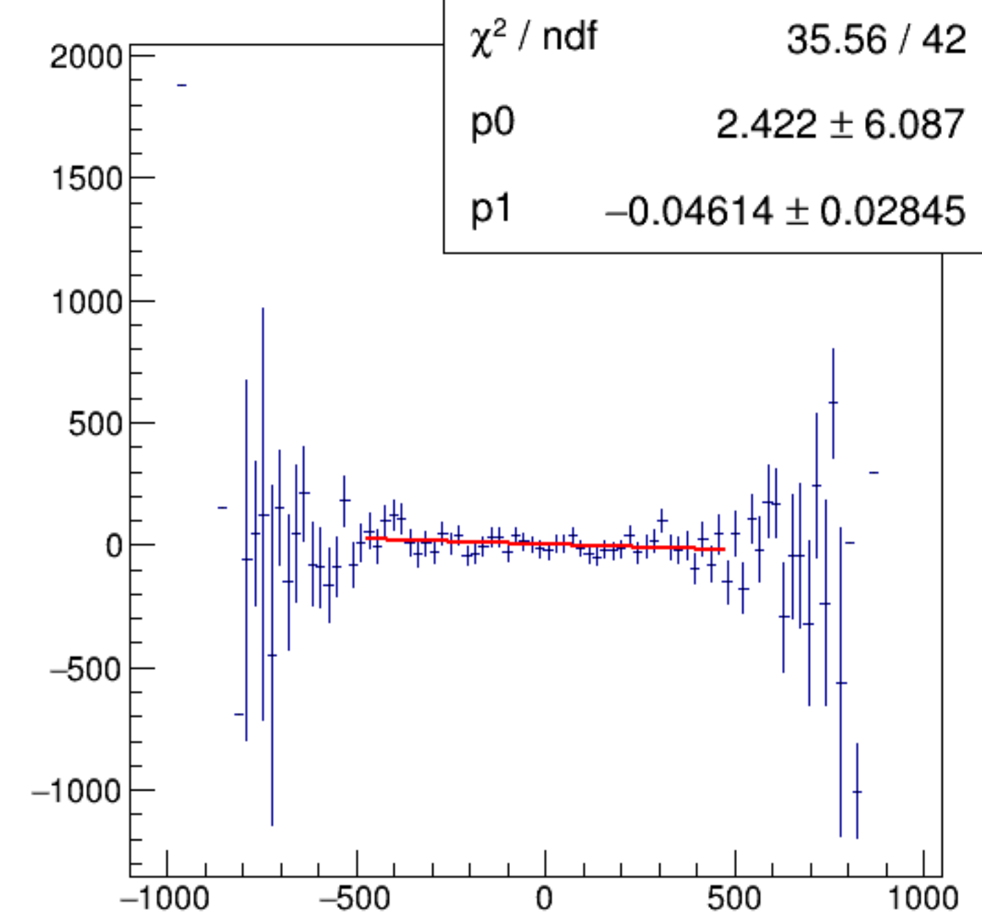
reg_asym_usr/ppm:AqUS/ppm {ok_cut}
