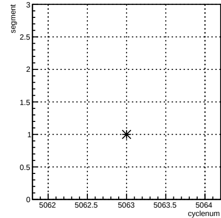
segment:cyclenum {run == 5874}
