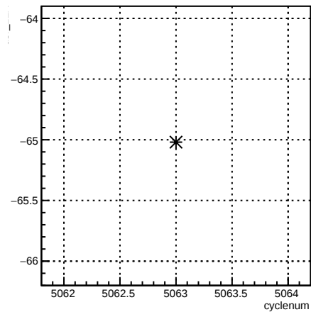
usr_12X:cyclenum {run == 5874}
