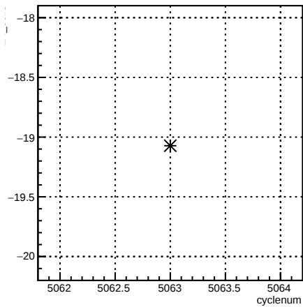
4eX_coil3:cyclenum {run == 5874}
