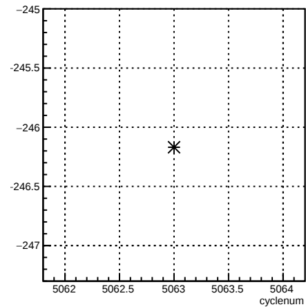
4eX_coil1:cyclenum {run == 5874}
