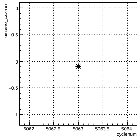
delta46_12X4eY:cyclenum {run == 5874}
