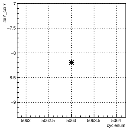
4eY_coil7:cyclenum {run == 5874}
