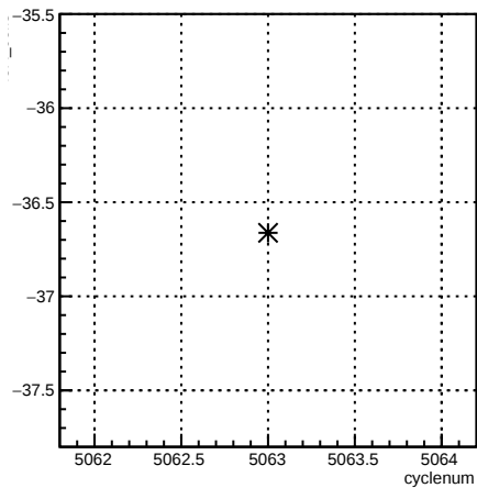
4eX_coil3:cyclenum {run == 5874}
