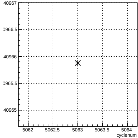
usr_coil7:cyclenum {run == 5874}
