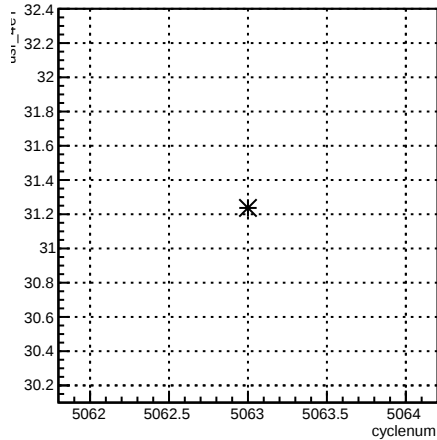
usr_4eY:cyclenum {run == 5874}
