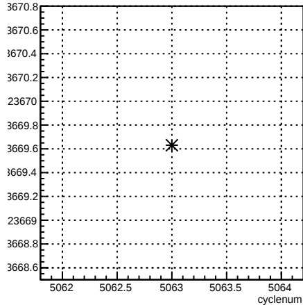
usl_coil7:cyclenum {run == 5874}
