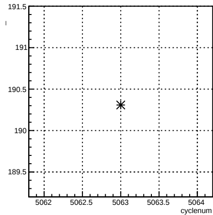
4eX_coil7:cyclenum {run == 5874}
