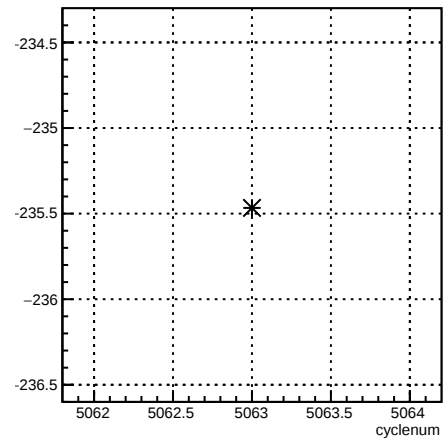
12X_coil1:cyclenum {run == 5874}
