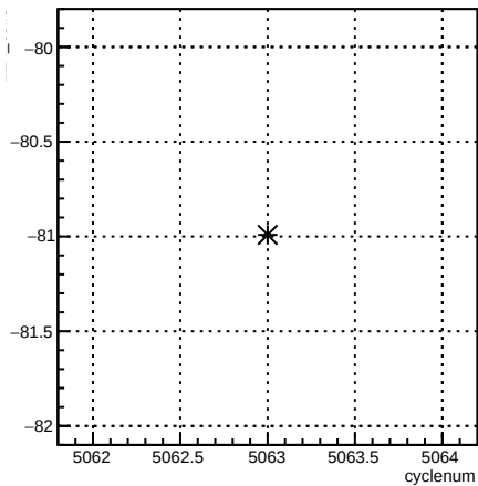
12X_coil3:cyclenum {run == 5874}
