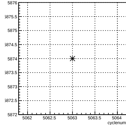
run:cyclenum {run == 5874}
