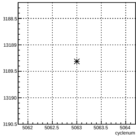
usr_coil6:cyclenum {run == 5874}
