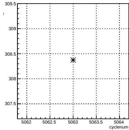
1X_coil7:cyclenum {run == 5874}
