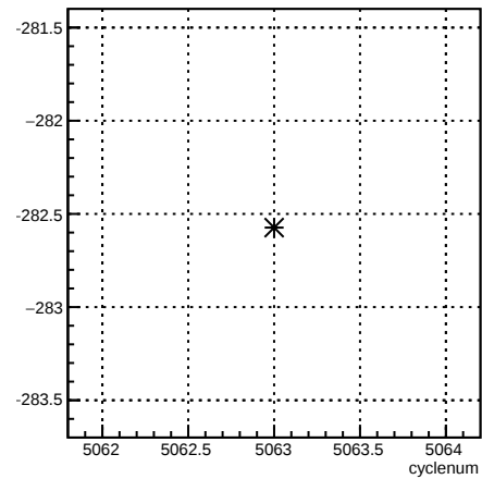
4eX_coil1:cyclenum {run == 5874}
