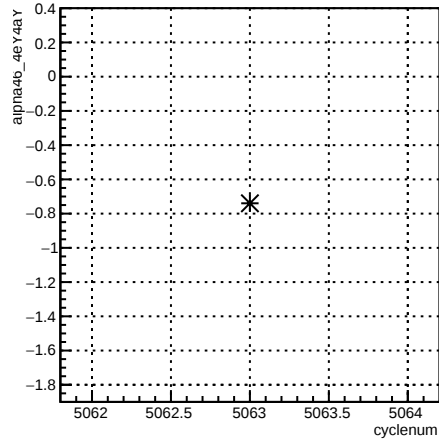
alpha46_4eY4aY:cyclenum {run == 5874}
