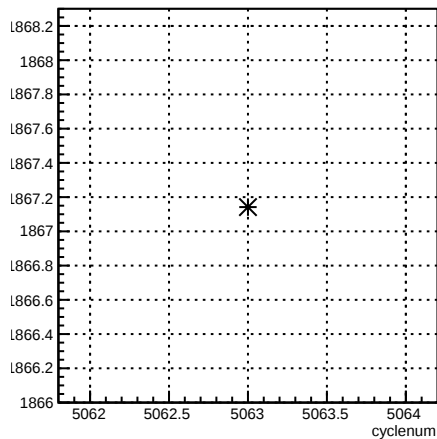
usl_coil6:cyclenum {run == 5874}
