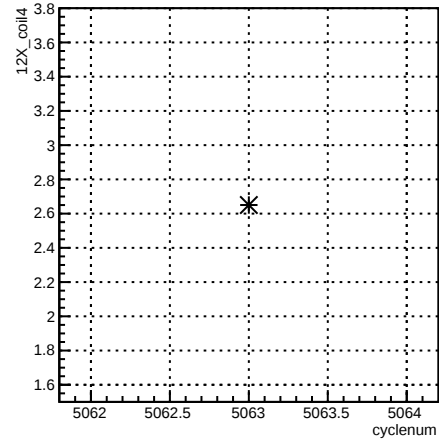
12X_coil4:cyclenum {run == 5874}
