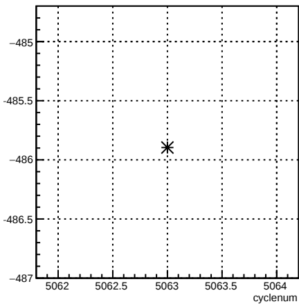
12X_coil7:cyclenum {run == 5874}
