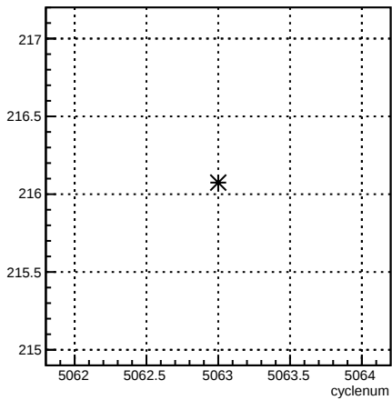
4eY_coil4:cyclenum {run == 5874}
