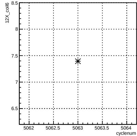
12X_coil6:cyclenum {run == 5874}
