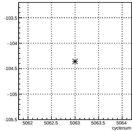
usl_4eY:cyclenum {run == 5874}
