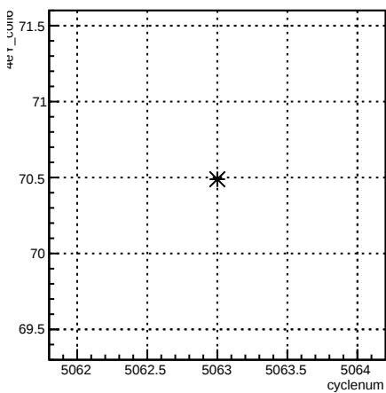
4eY_coil6:cyclenum {run == 5874}
