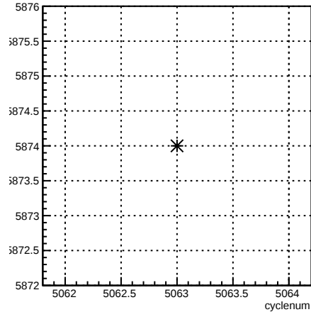
run:cyclenum {run == 5874}
