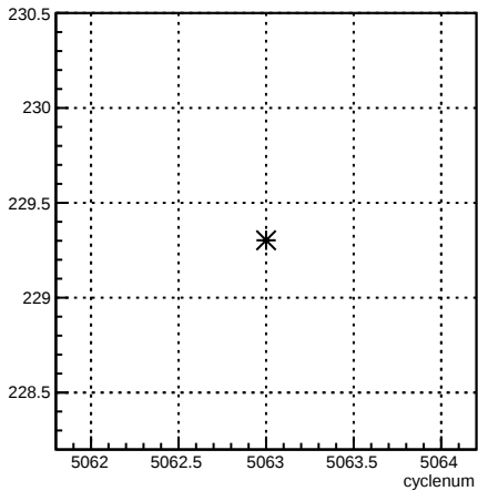
4eY_coil4:cyclenum {run == 5874}
