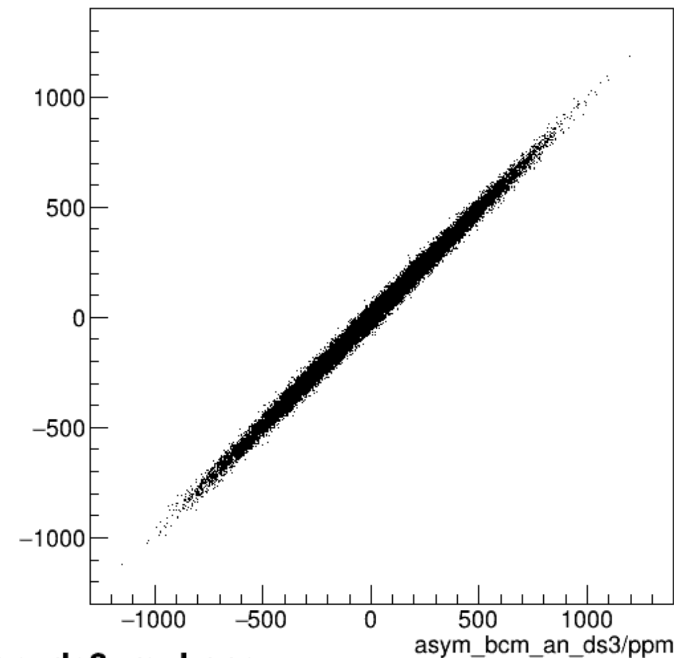
run5876_000_asym_bcm_an_us_vs_asym_bcm_an_ds3_mul.png
