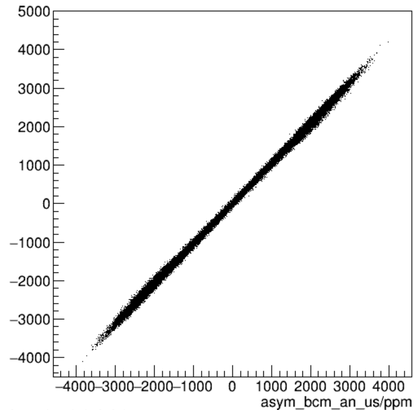
run5876_000_asym_bcm_dg_ds_vs_asym_bcm_an_us_pr.png
