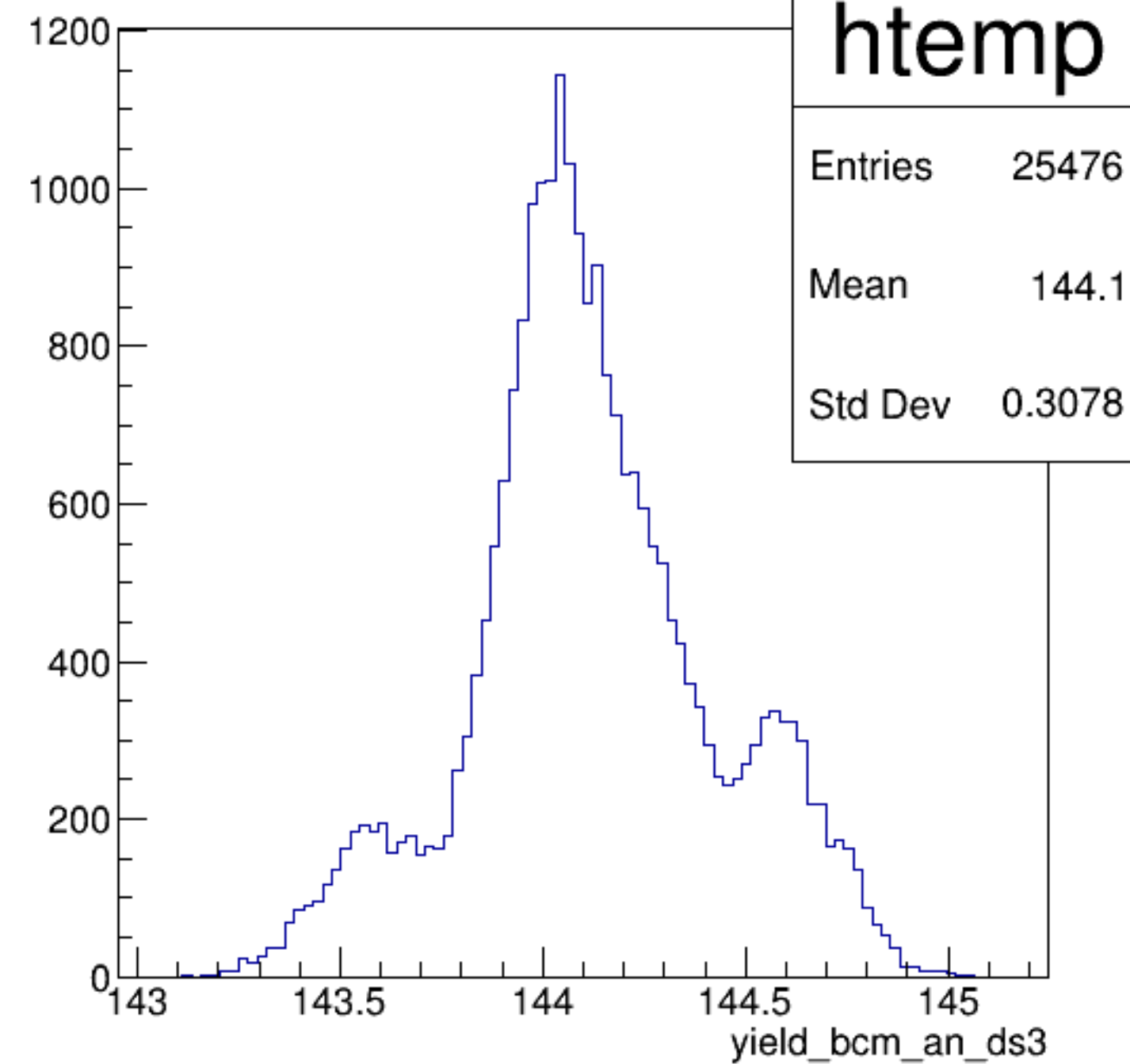
yield_bcm_an_ds3 {ErrorFlag==0}
