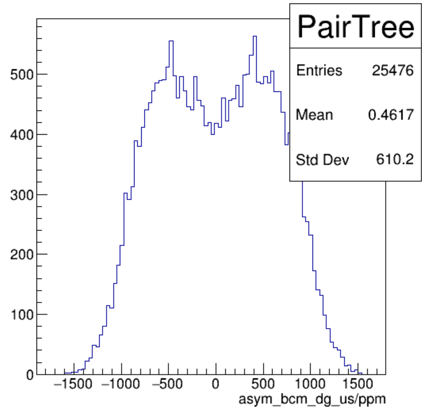
asym_bcm_dg_us/ppm {ErrorFlag==0}
