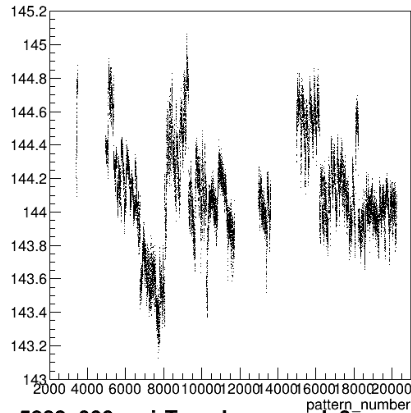
yield_bcm_an_ds3:pattern_number {ErrorFlag==0}
