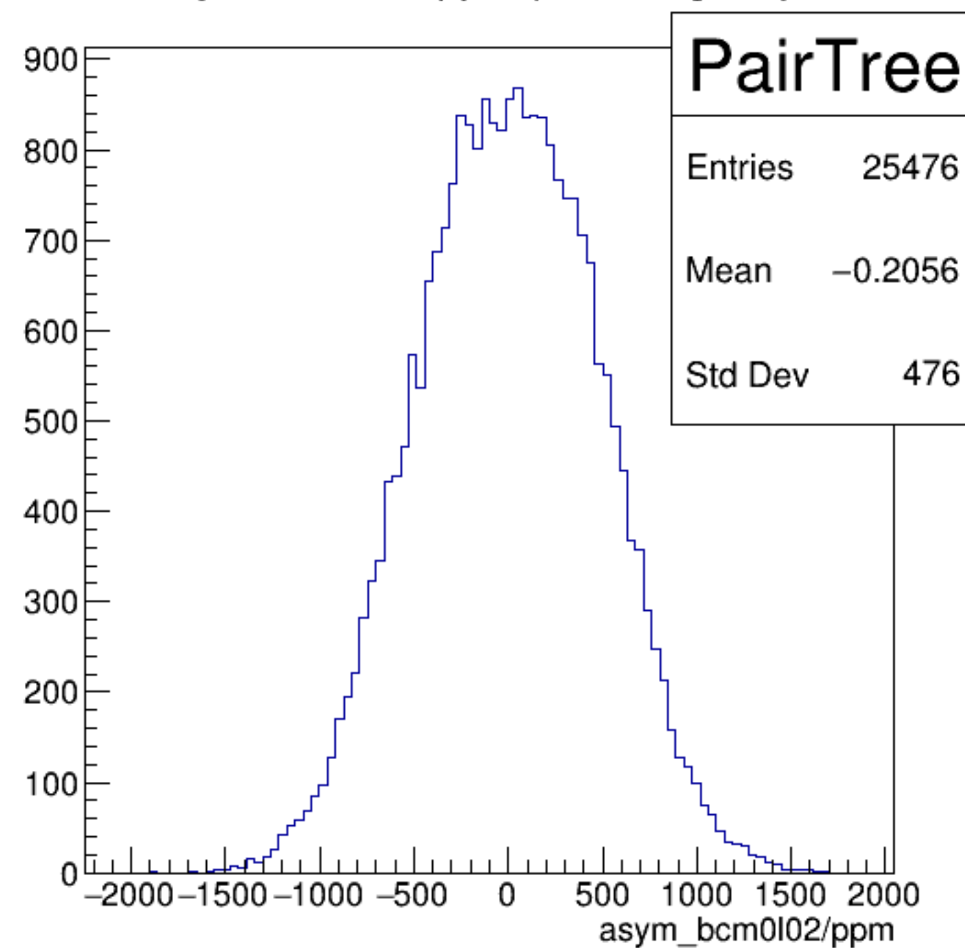
asym_bcm0l02/ppm {ErrorFlag==0}
