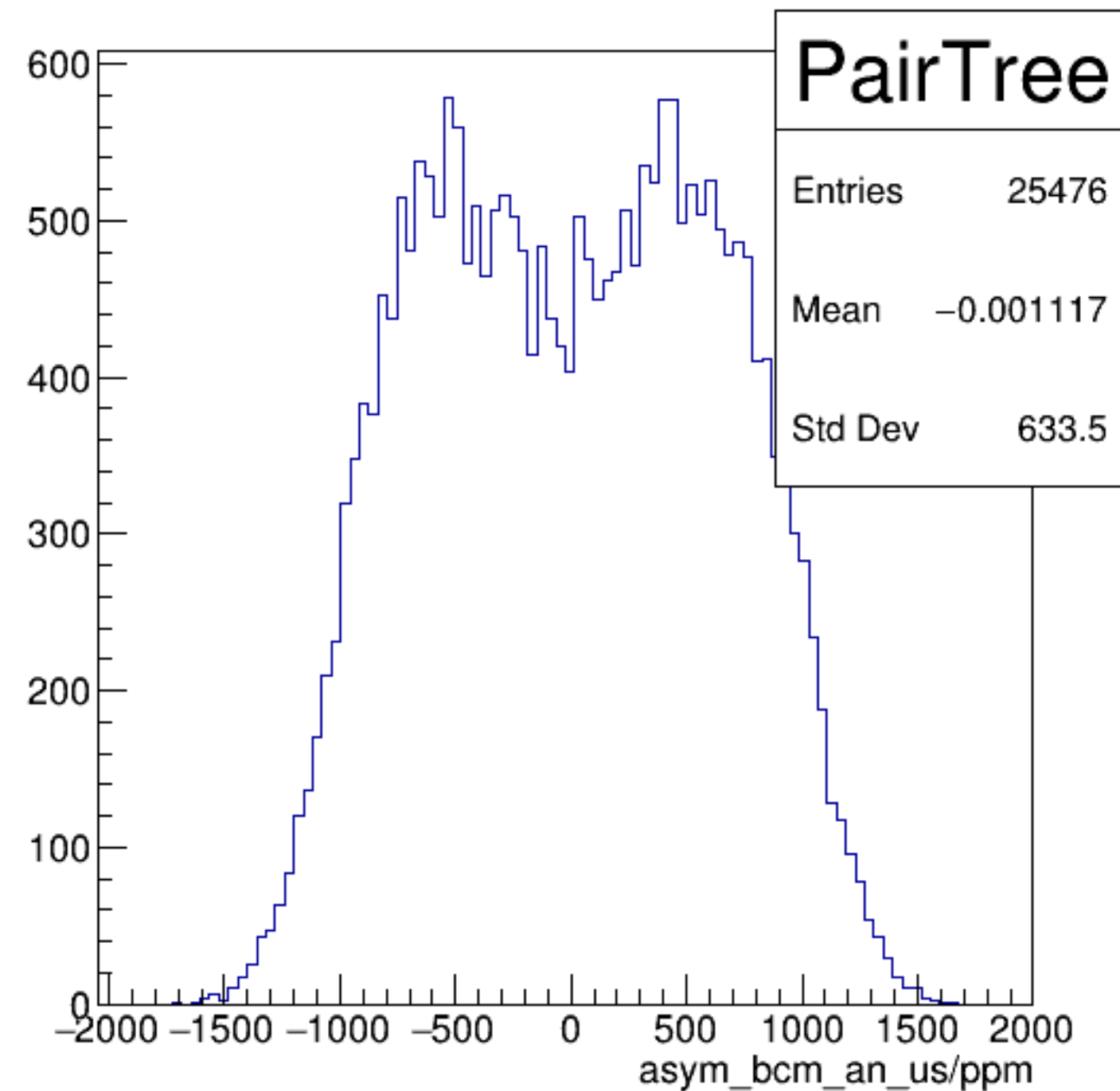
asym_bcm_an_us/ppm {ErrorFlag==0}
