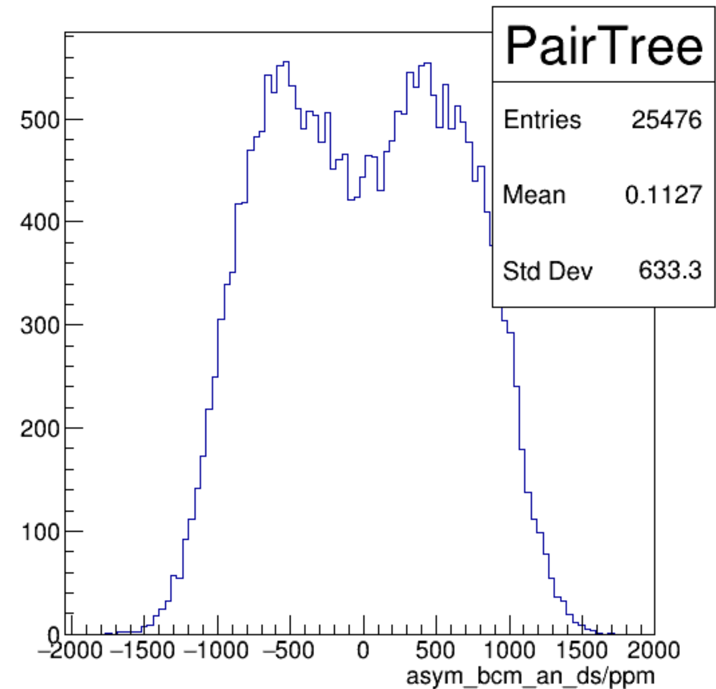
asym_bcm_an_ds/ppm {ErrorFlag==0}
