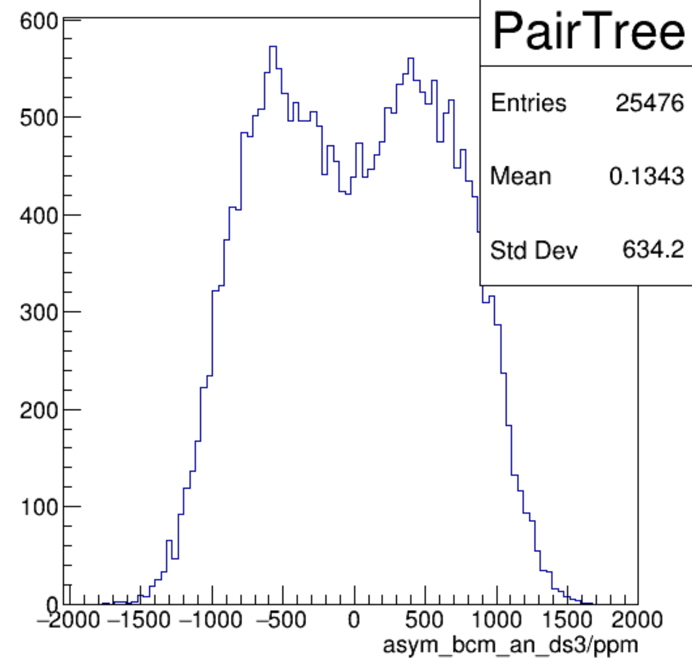
asym_bcm_an_ds3/ppm {ErrorFlag==0}
