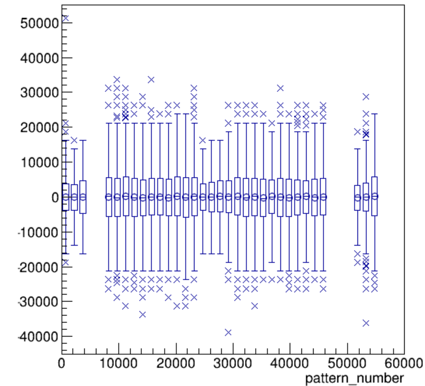
asym_sam4/ppm:pattern_number {ErrorFlag==0}
