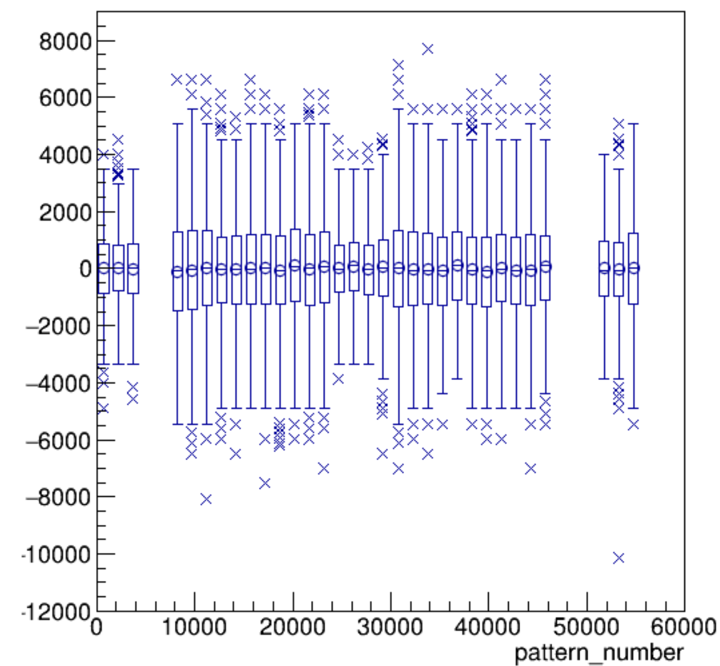
asym_sam6/ppm:pattern_number {ErrorFlag==0}
