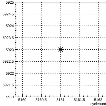
run:cyclenum {run == 5923}
