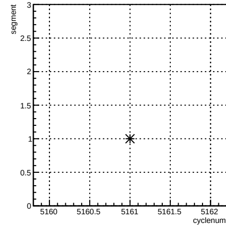
segment:cyclenum {run == 5923}
