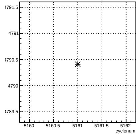
run:cyclenum {run == 5923}
