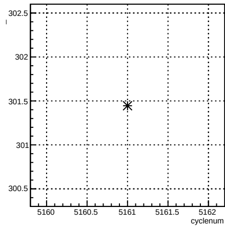
4eX_coil7:cyclenum {run == 5923}
