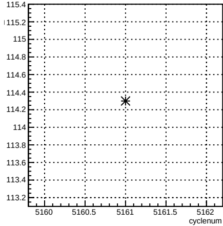
4eY_coil6:cyclenum {run == 5923}
