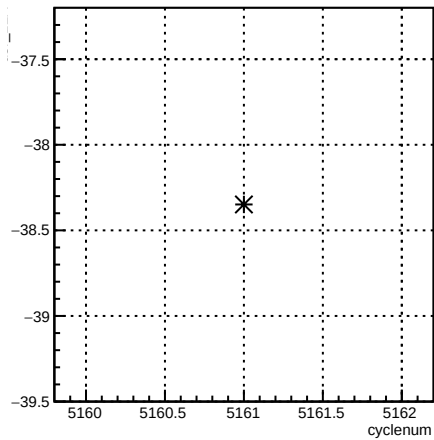
usr_12X:cyclenum {run == 5923}
