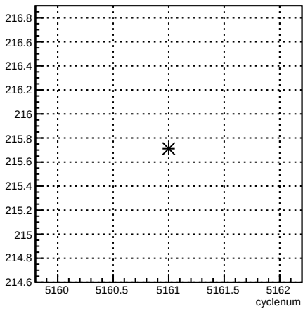
4eY_coil4:cyclenum {run == 5923}
