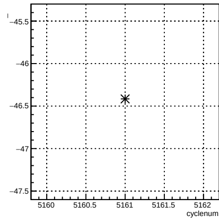
usl_4eY:cyclenum {run == 5923}
