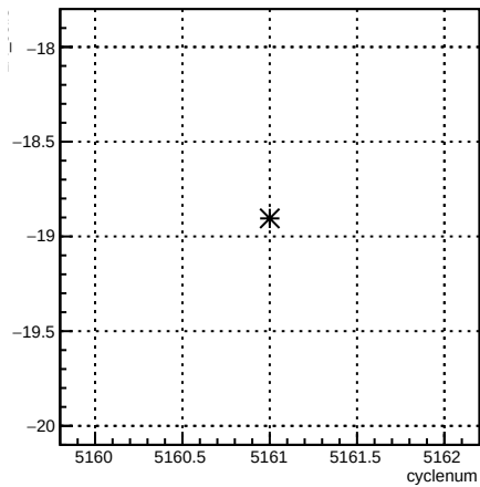
4eX_coil3:cyclenum {run == 5923}
