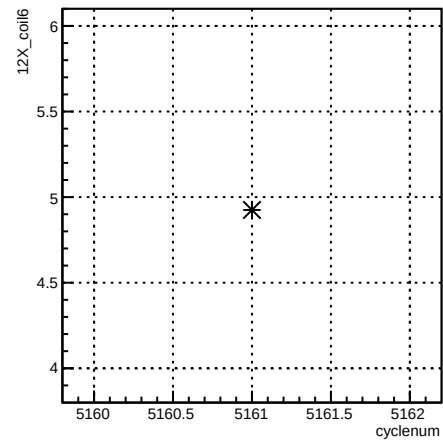
12X_coil6:cyclenum {run == 5923}
