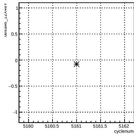
delta46_12X4eY:cyclenum {run == 5923}
