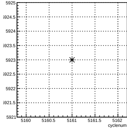
run:cyclenum {run == 5923}
