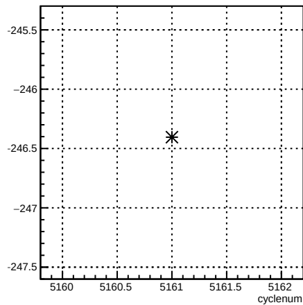
4eX_coil1:cyclenum {run == 5923}
