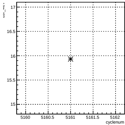
usr_4eY:cyclenum {run == 5923}
