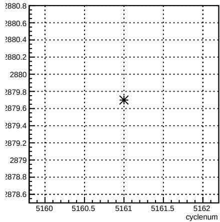
usl_coil3:cyclenum {run == 5923}
