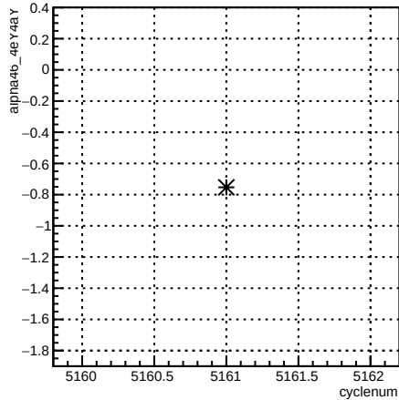
alpha46_4eY4aY:cyclenum {run == 5923}
