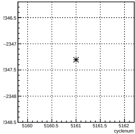
usr_coil7:cyclenum {run == 5923}
