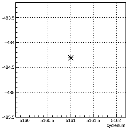
12X_coil7:cyclenum {run == 5923}
