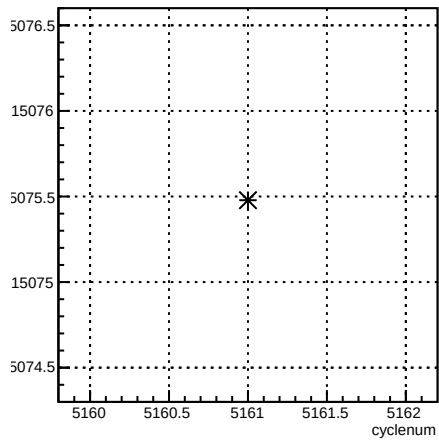
usl_coil6:cyclenum {run == 5923}
