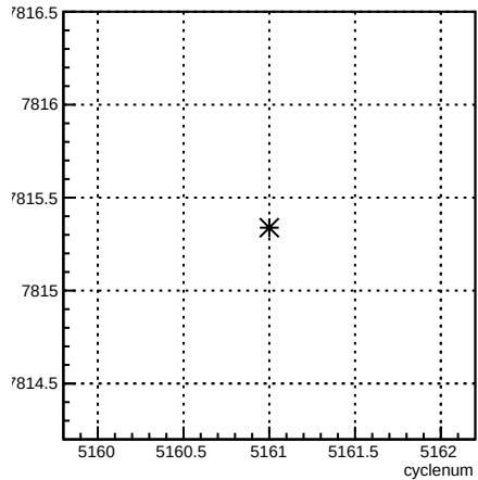
usl_coil7:cyclenum {run == 5923}
