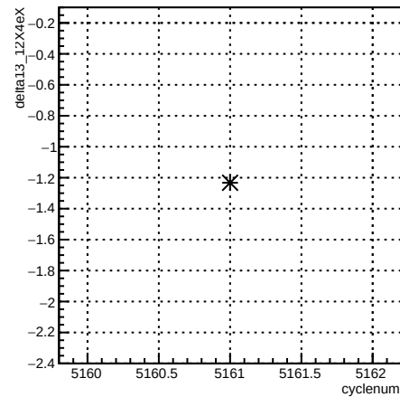
delta13_12X4eX:cyclenum {run == 5923}
