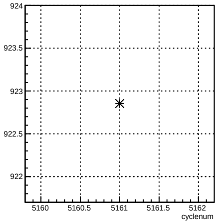
usl_coil6:cyclenum {run == 5923}
