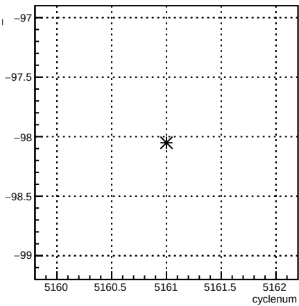
usr_4eY:cyclenum {run == 5923}
