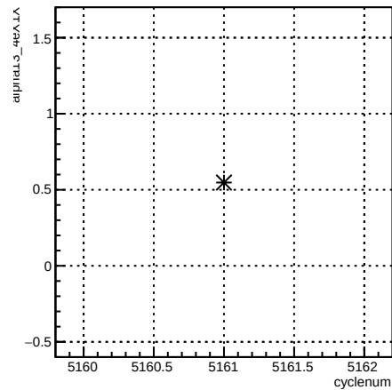
alpha13_4eX1X:cyclenum {run == 5923}
