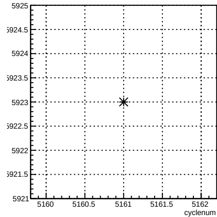
run:cyclenum {run == 5923}
