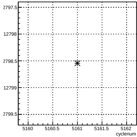
usr_coil6:cyclenum {run == 5923}
