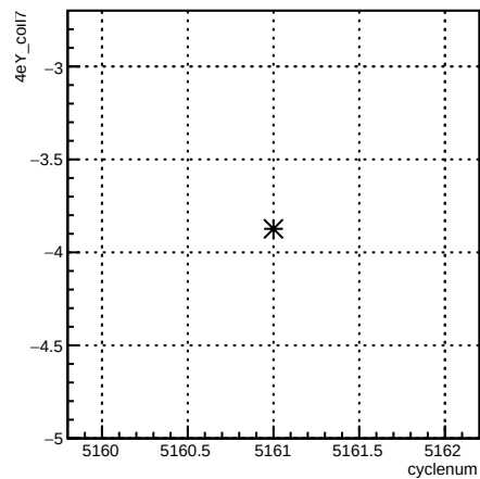
4eY_coil7:cyclenum {run == 5923}
