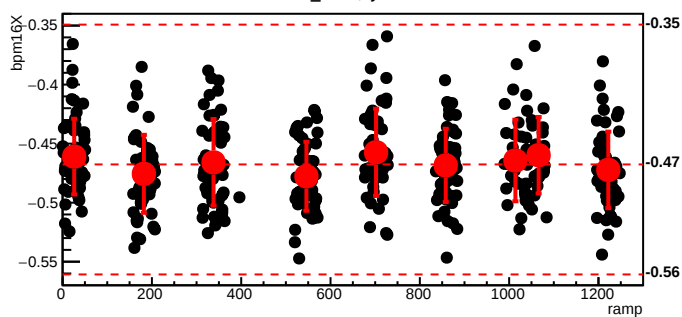
bmod_trim2,cyc=5167
