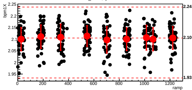
bmod_trim2,cyc=5167
