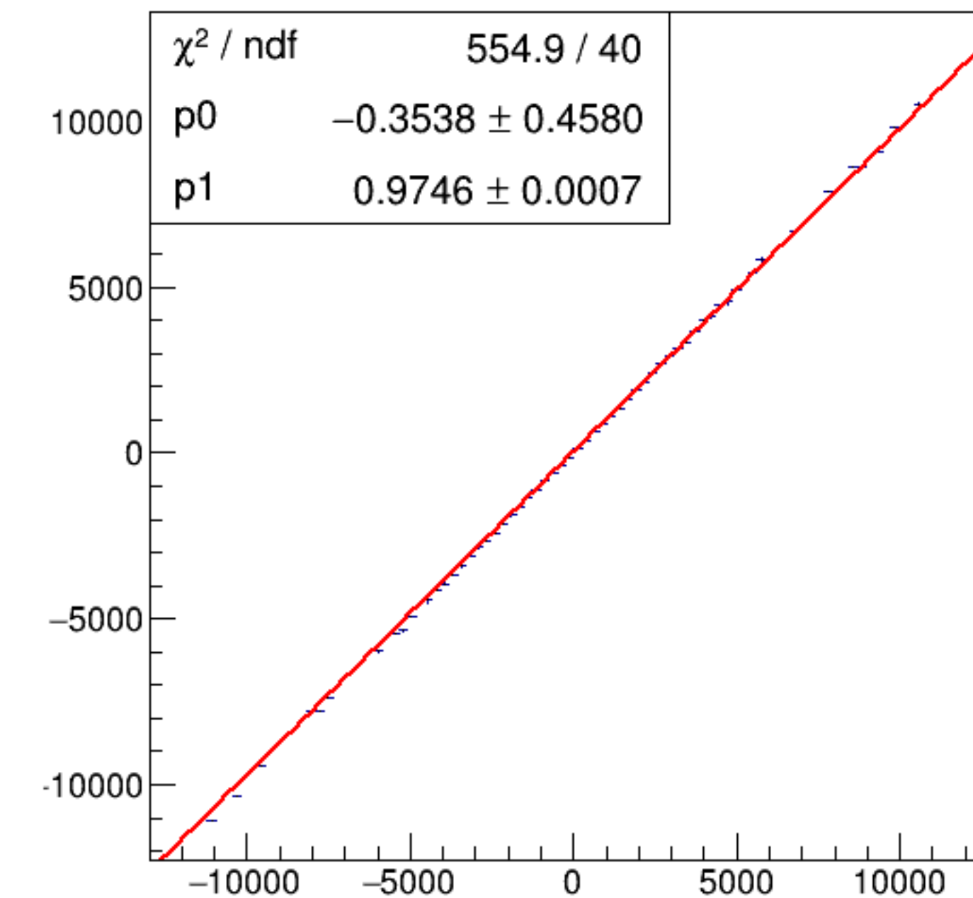
run5948_000_asym_bcm_dg_us_vs_asym_bcm_dg_ds_pr.png
