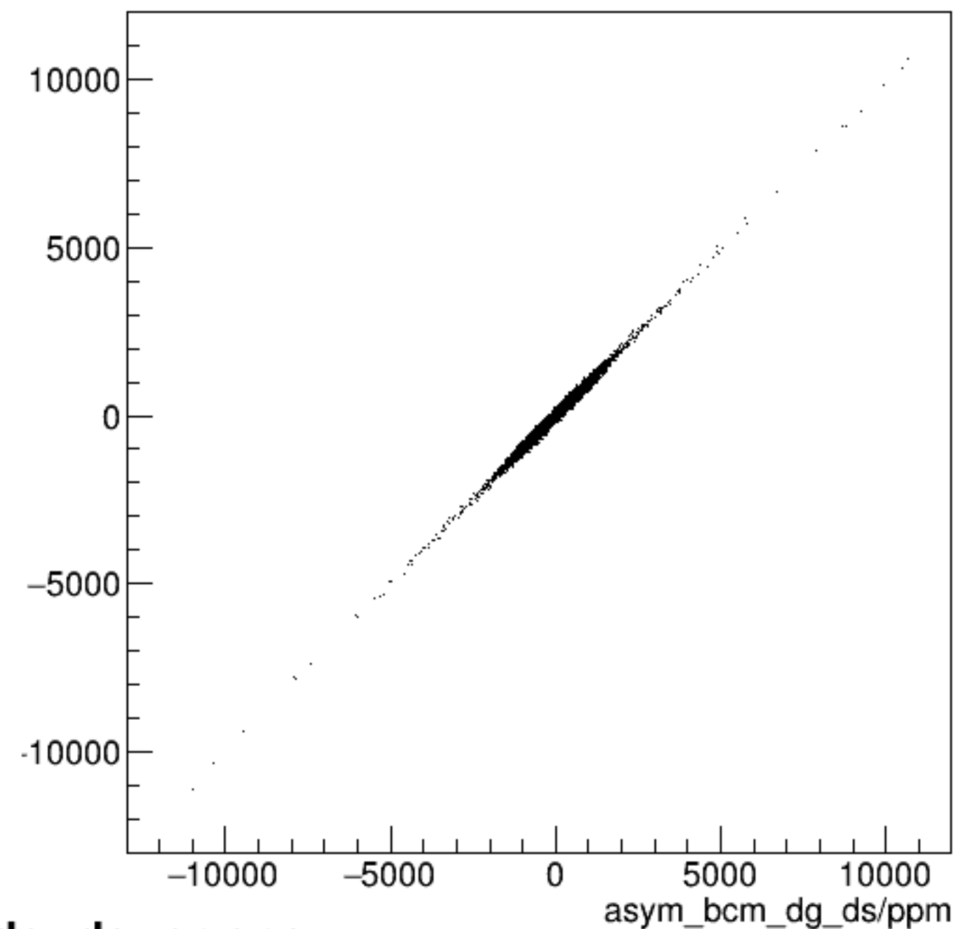
run5948_000_asym_bcm_dg_us_vs_asym_bcm_dg_ds_pr.png
