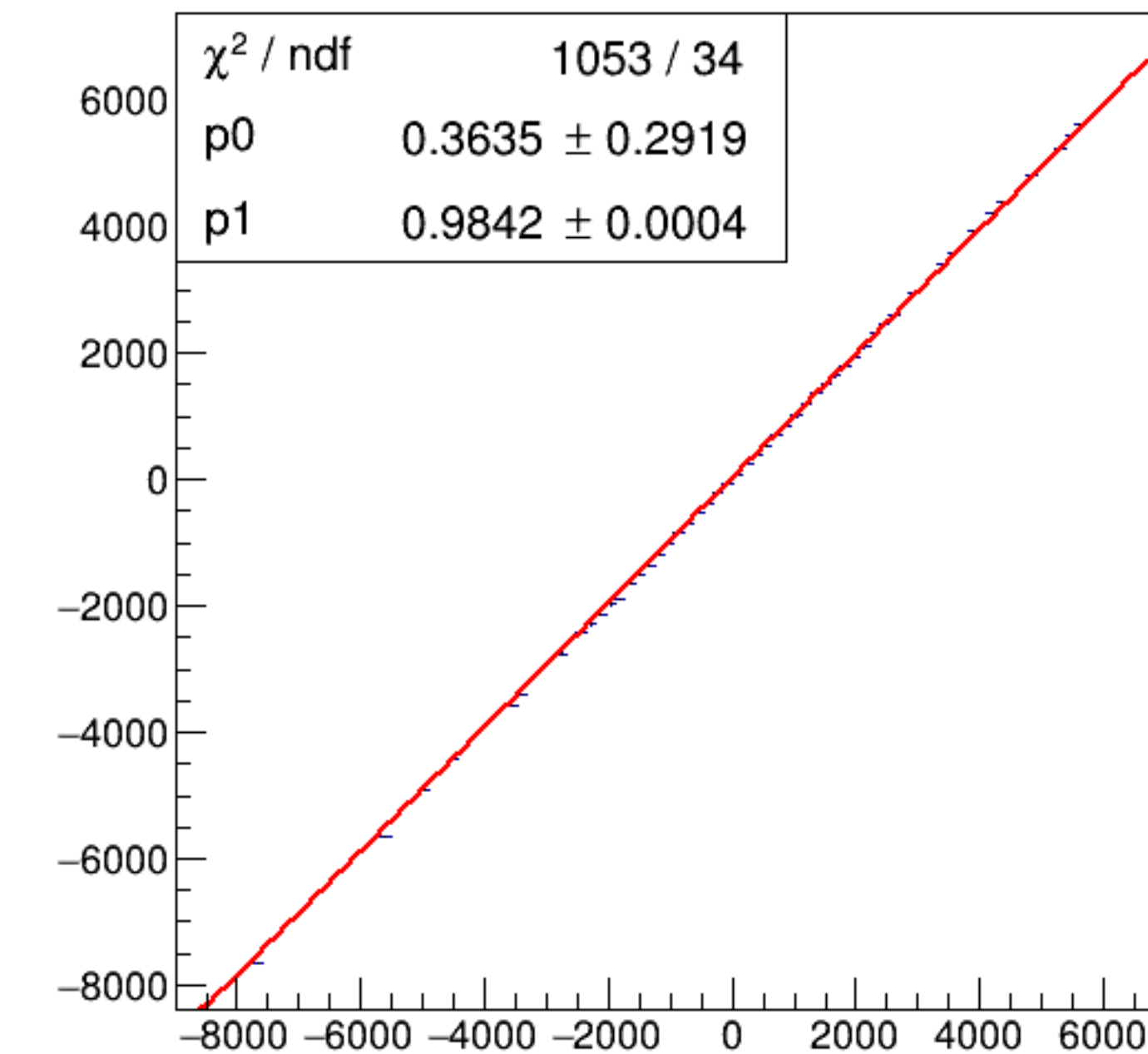
run5948_000_asym_bcm_an_ds_vs_asym_bcm_an_ds3_mul.png
