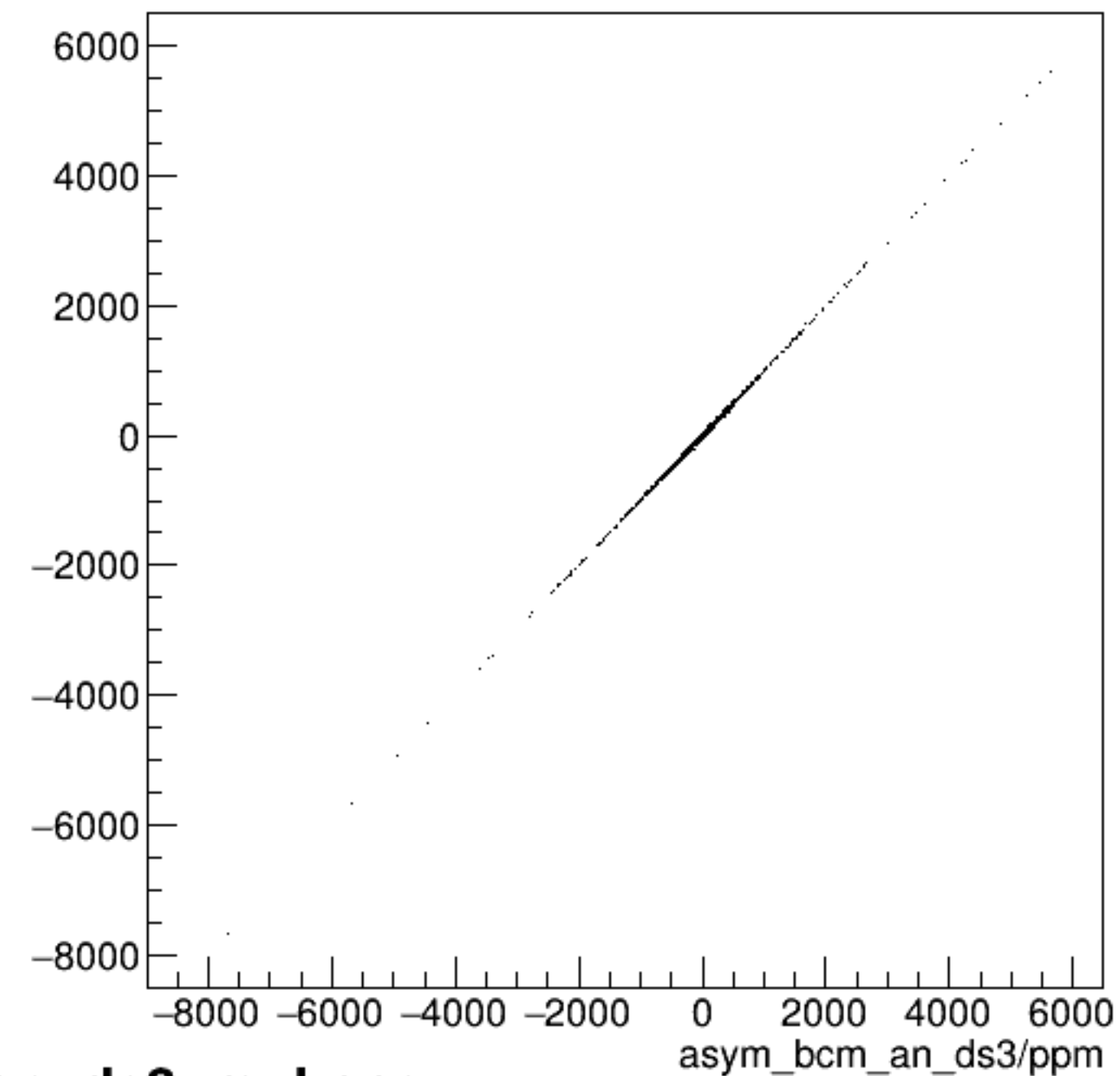
run5948_000_asym_bcm_an_ds_vs_asym_bcm_an_ds3_mul.png
