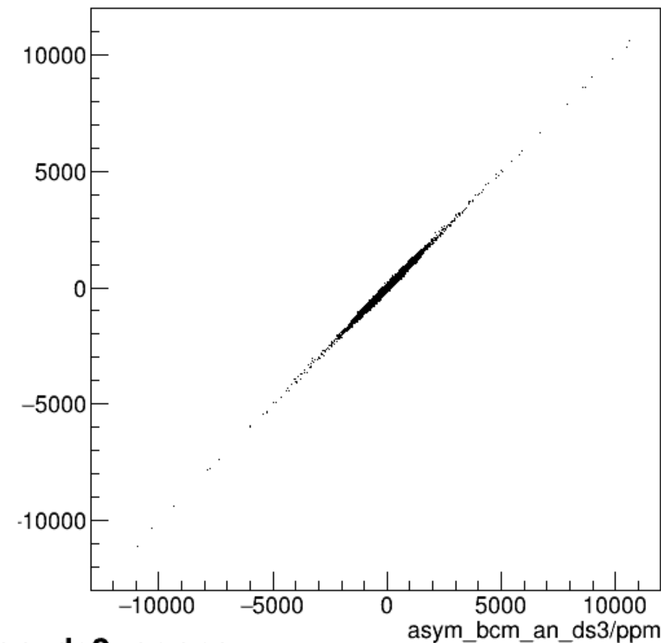
run5948_000_asym_bcm_dg_us_vs_asym_bcm_an_ds3_pr.png
