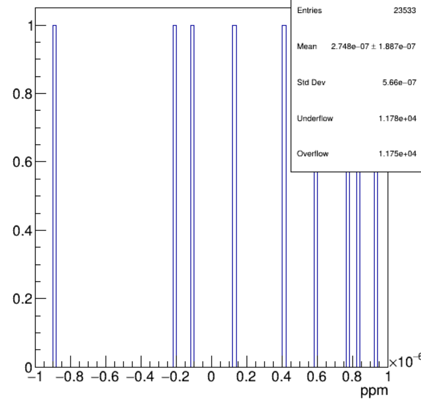
asym_bcm_an_diff
