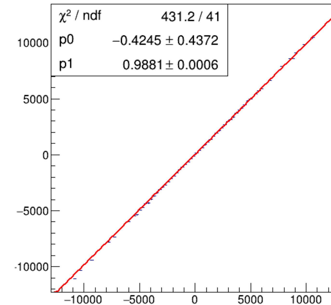
run5948_000_asym_bcm_dg_us_vs_asym_bcm_an_ds3_pr.png
