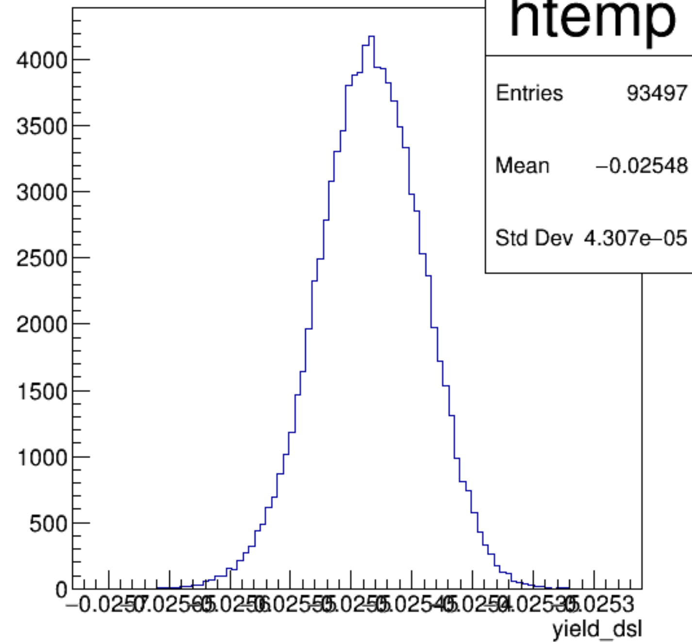
yield_dsl {ErrorFlag==0}
