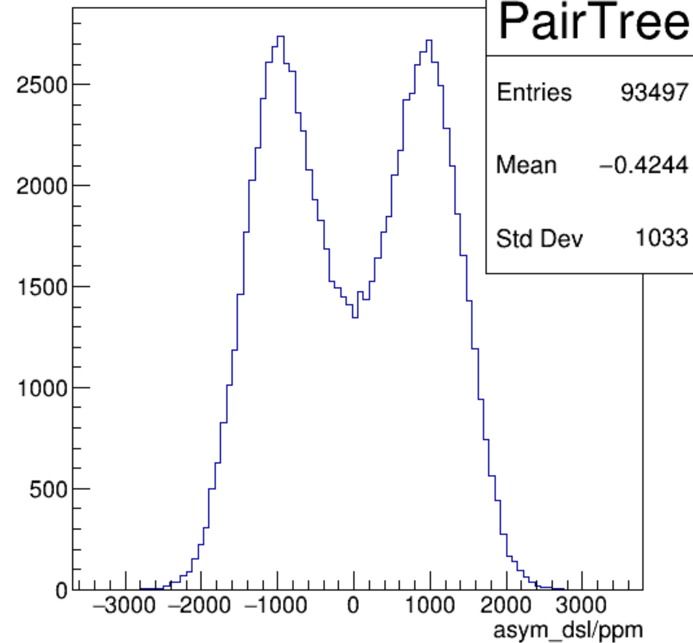
asym_dsl/ppm {ErrorFlag==0}
