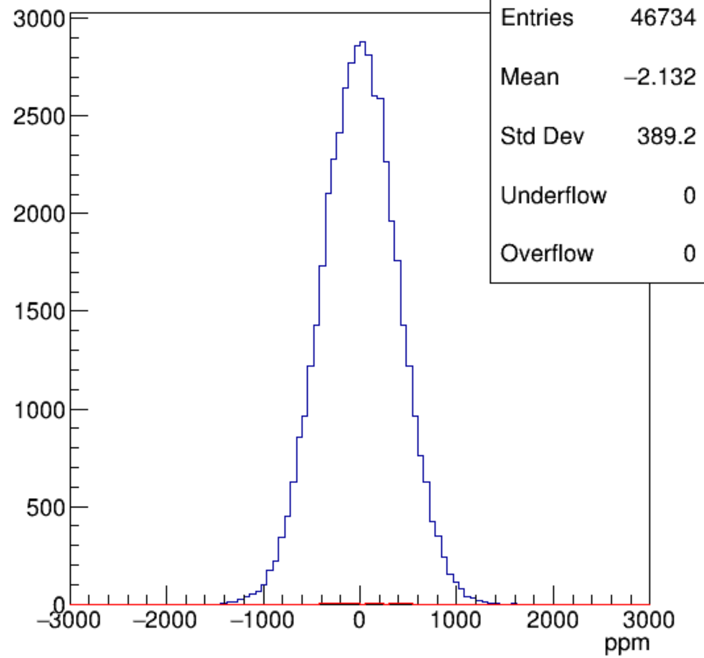
asym_dsr
