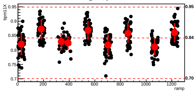
bmod_trim6,cyc=5252
