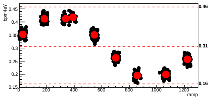
bmod_trim4,cyc=5252
