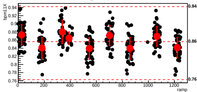
bmod_trim4,cyc=5252
