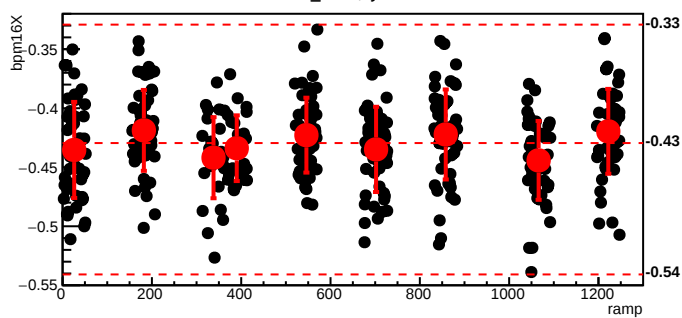
bmod_trim6,cyc=5252
