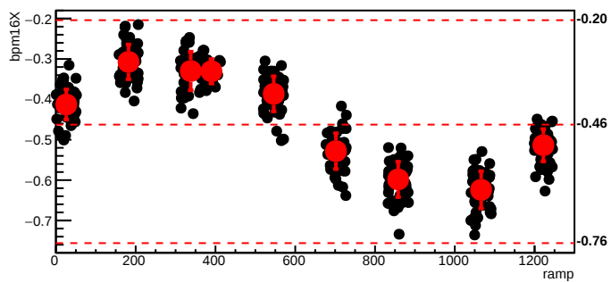
bmod_trim1,cyc=5252
