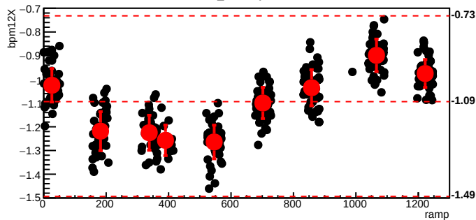
bmod_trim3,cyc=5252
