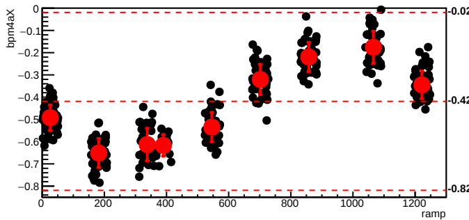
bmod_trim1,cyc=5252
