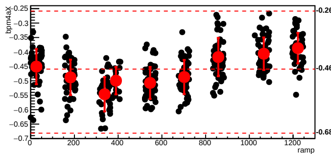
bmod_trim3,cyc=5252
