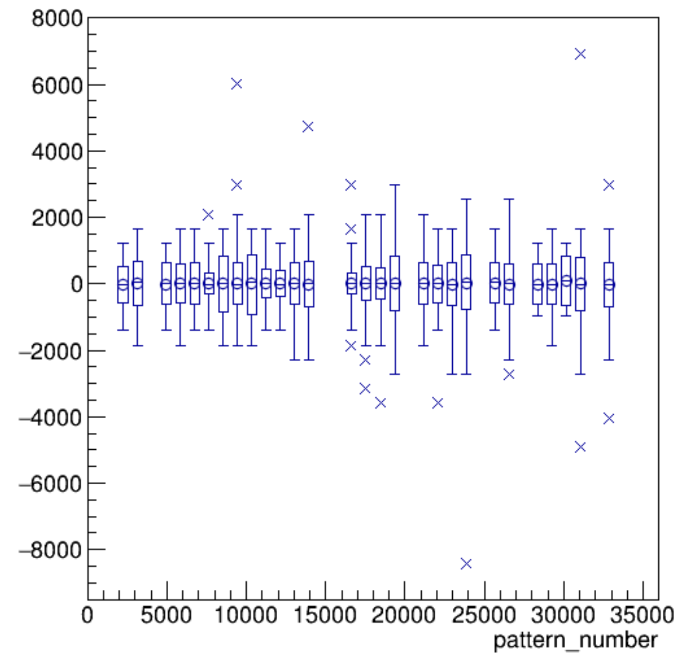
asym_bcm_dg_us/ppm:pattern_number {ErrorFlag==0}
