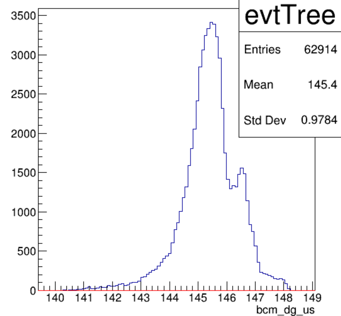
bcm_dg_us {ErrorFlag==0}
