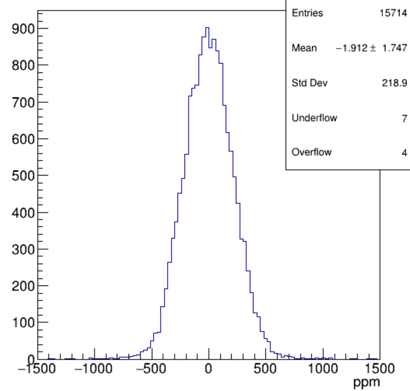
asym_bcm_an_ds
