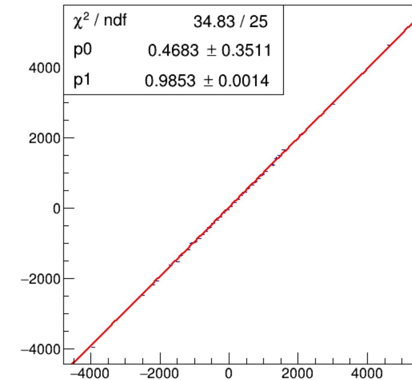
run5957_000_asym_bcm_dg_ds_vs_asym_bcm_an_us_mul.png
