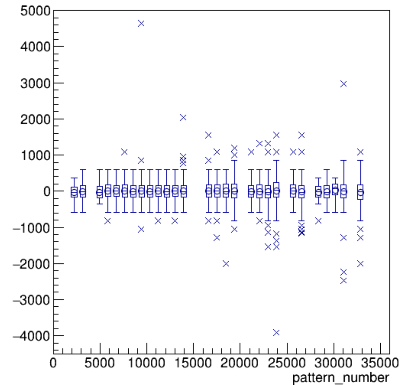
asym_bcm_dg_ds/ppm:pattern_number {ErrorFlag==0}
