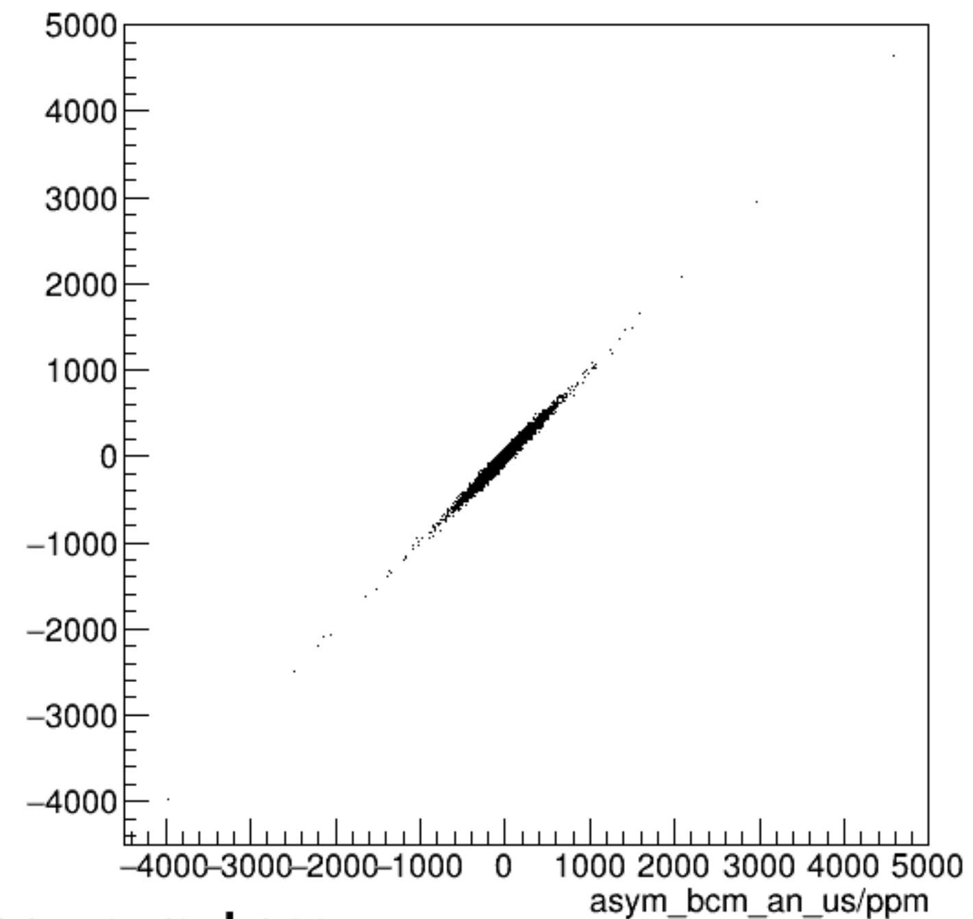
run5957_000_asym_bcm_dg_ds_vs_asym_bcm_an_us_mul.png
