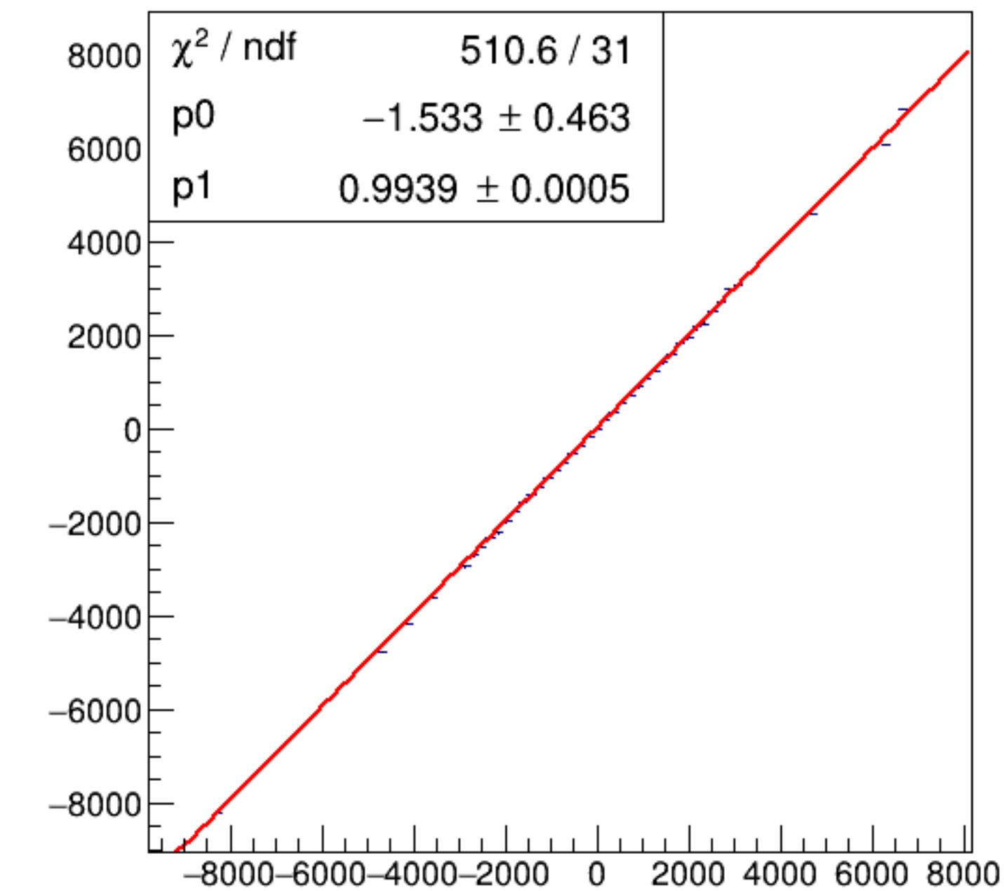
run5957_000_asym_bcm_dg_us_vs_asym_bcm_an_ds3_pr.png
