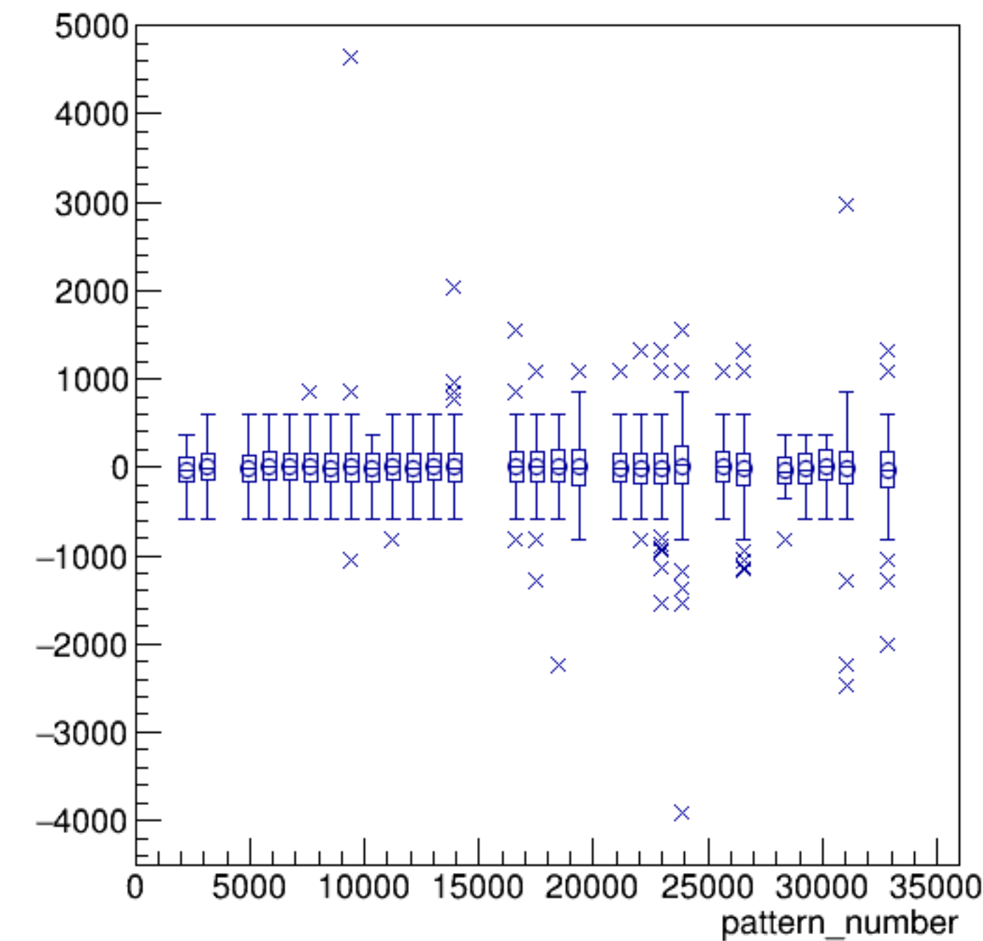
asym_bcm_an_us/ppm:pattern_number {ErrorFlag==0}
