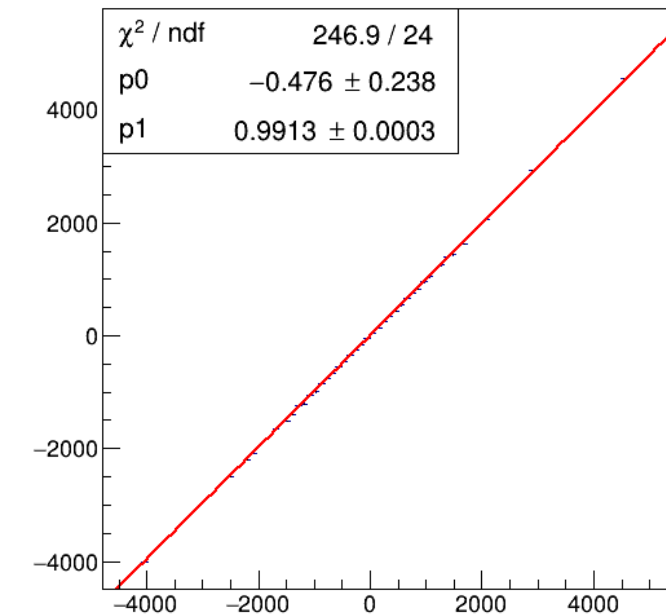
run5957_000_asym_bcm_an_ds_vs_asym_bcm_an_ds3_mul.png
