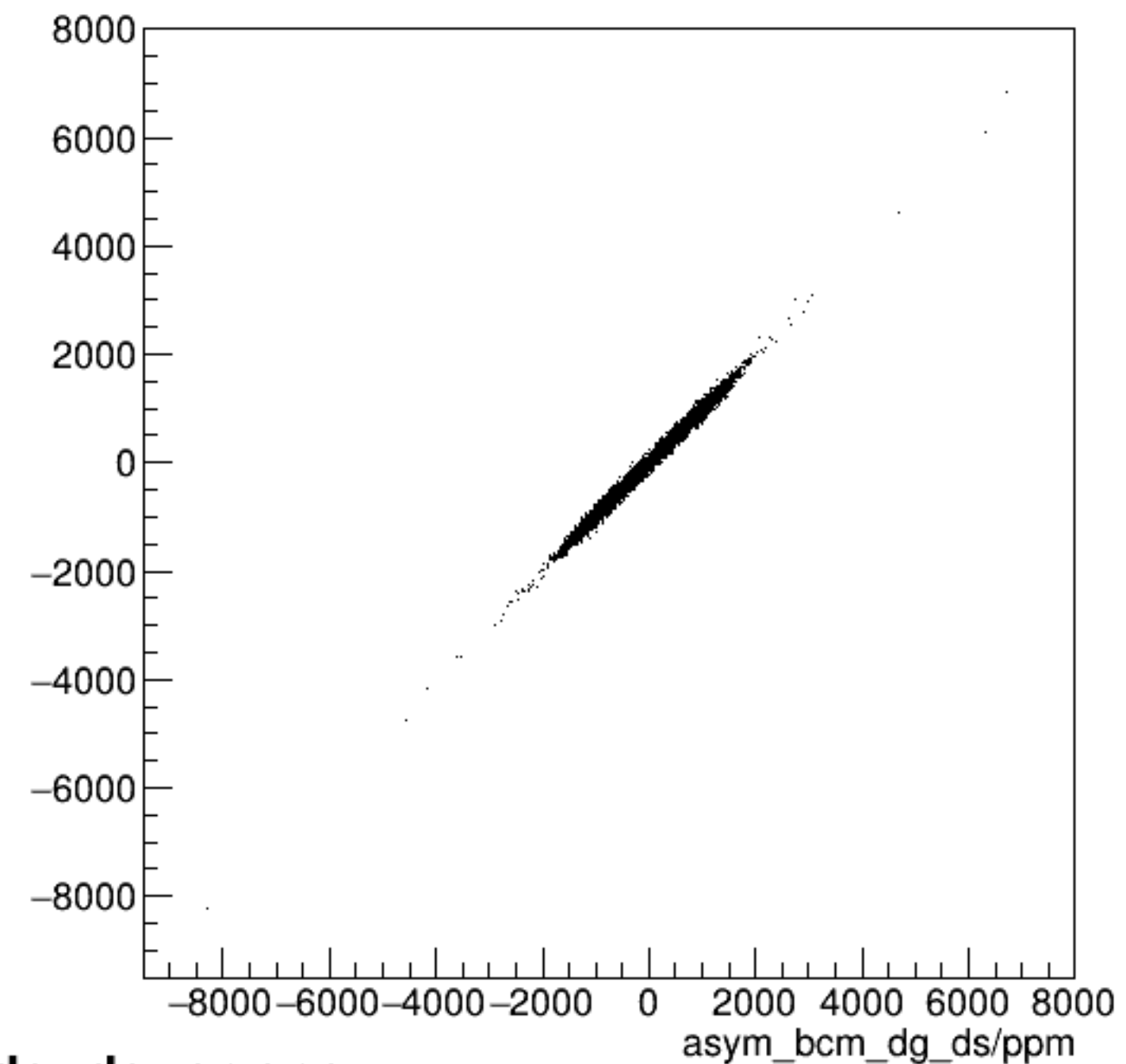
run5957_000_asym_bcm_dg_us_vs_asym_bcm_dg_ds_pr.png
