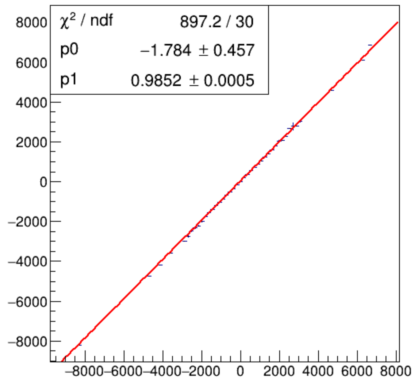
run5957_000_asym_bcm_dg_us_vs_asym_bcm_dg_ds_pr.png
