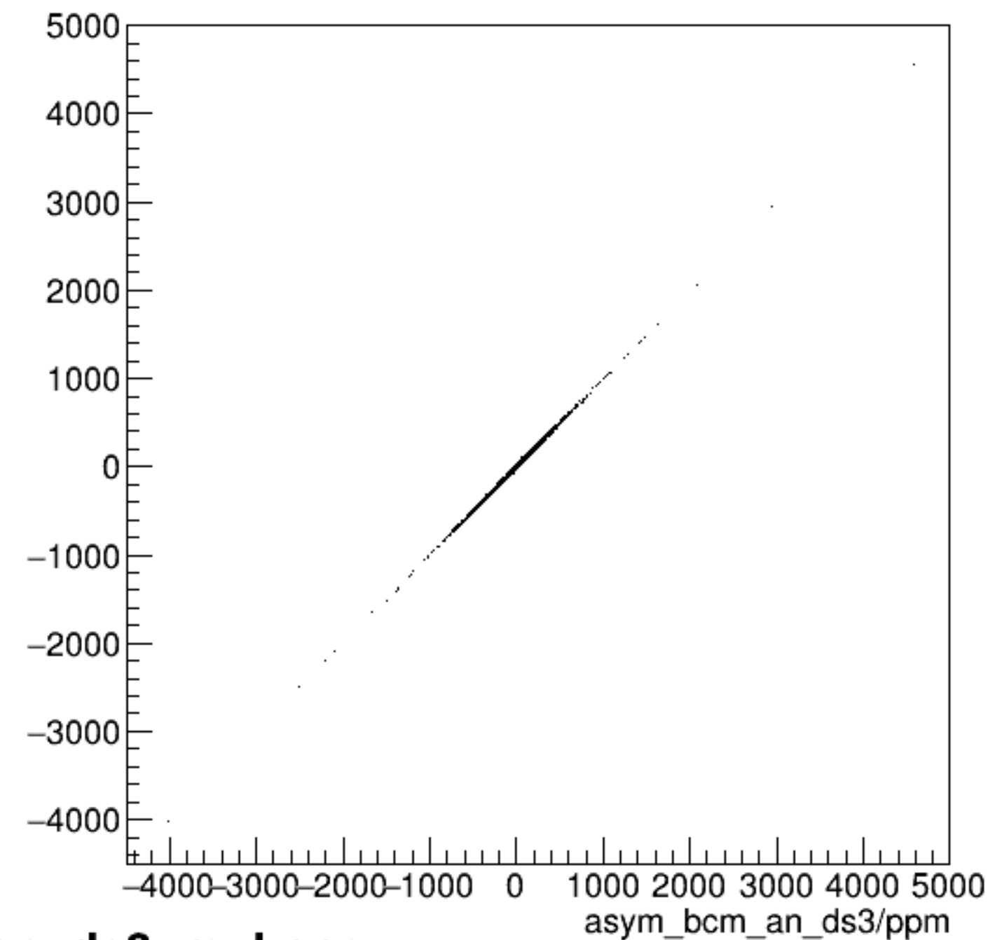
run5957_000_asym_bcm_an_ds_vs_asym_bcm_an_ds3_mul.png
