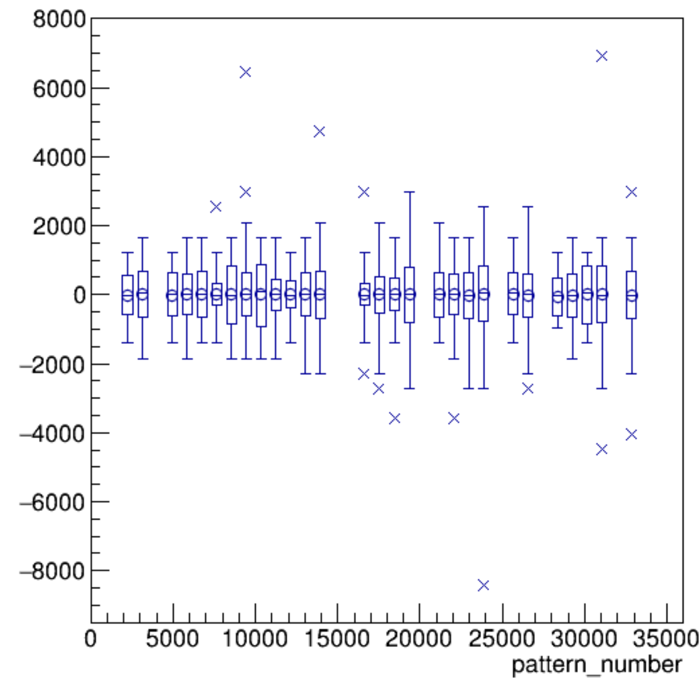
asym_bcm_dg_ds/ppm:pattern_number {ErrorFlag==0}
