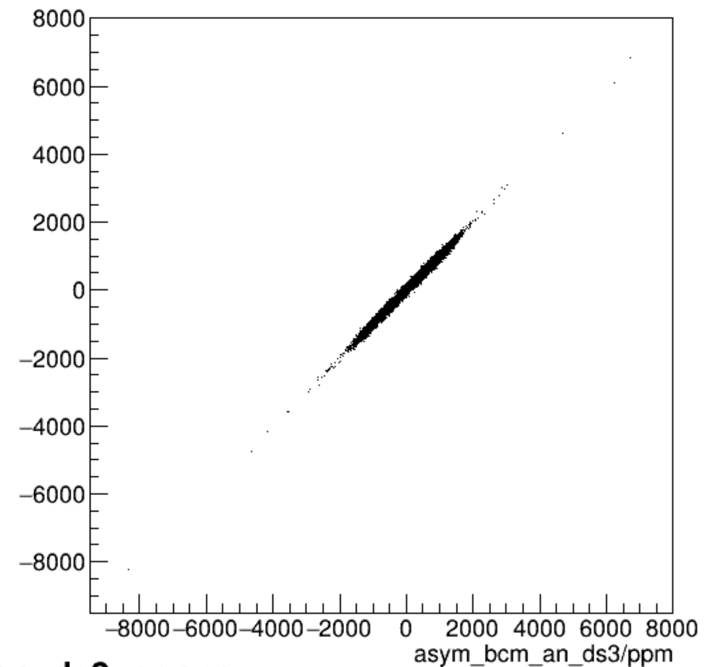
run5957_000_asym_bcm_dg_us_vs_asym_bcm_an_ds3_pr.png
