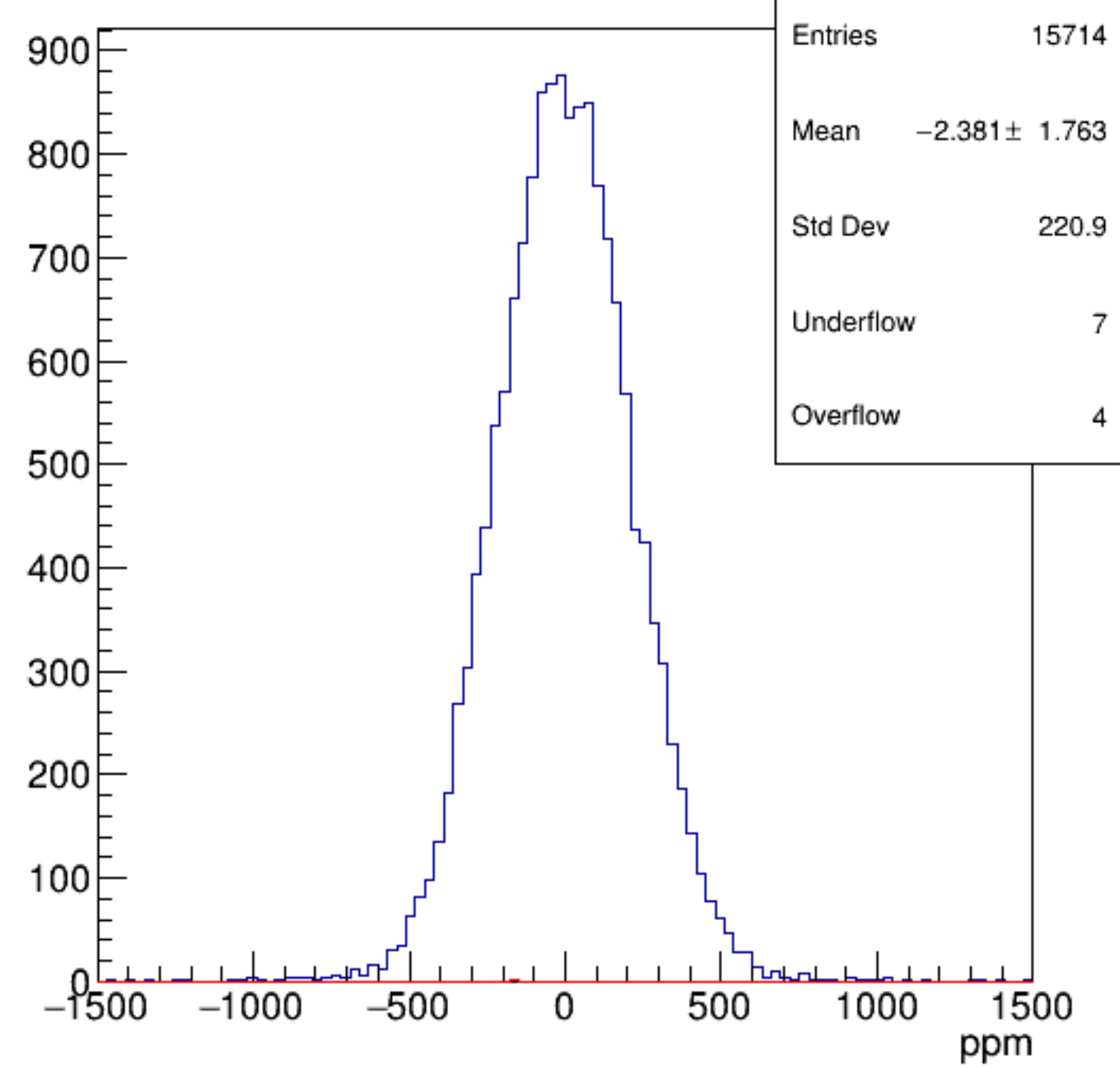
asym_bcm_dg_us
