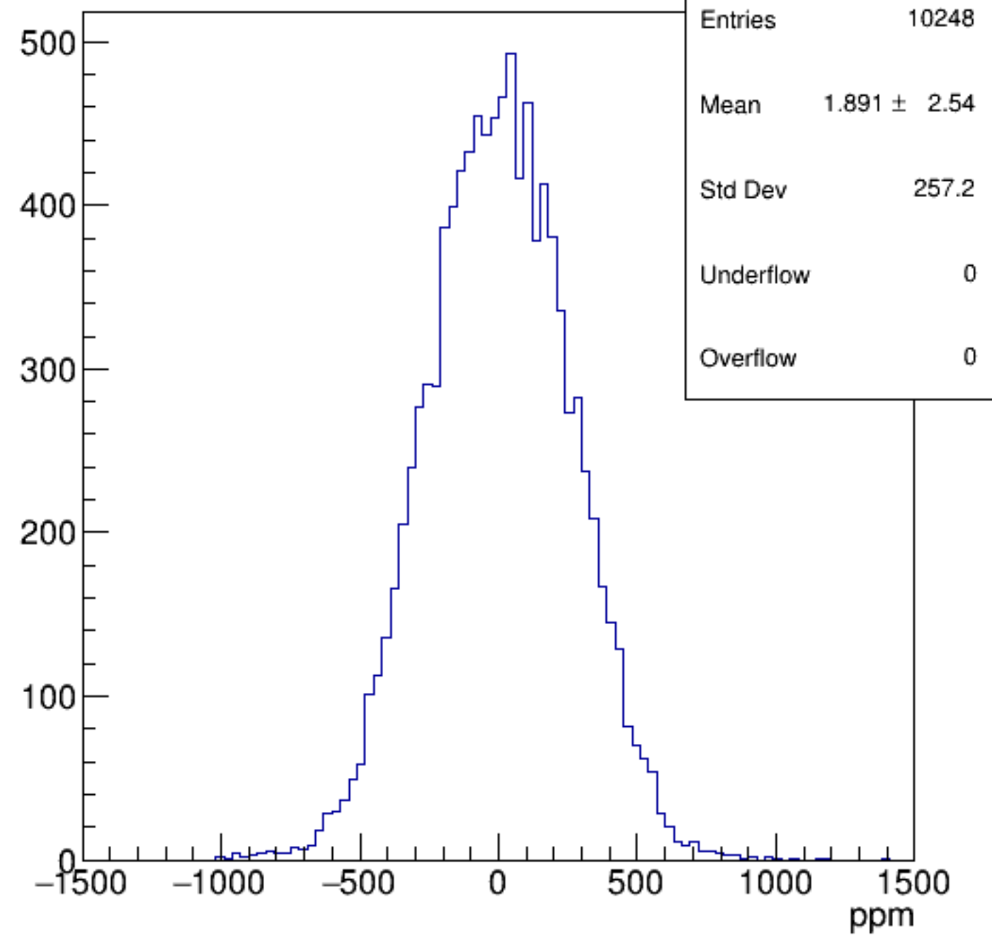
asym_bcm0l02
