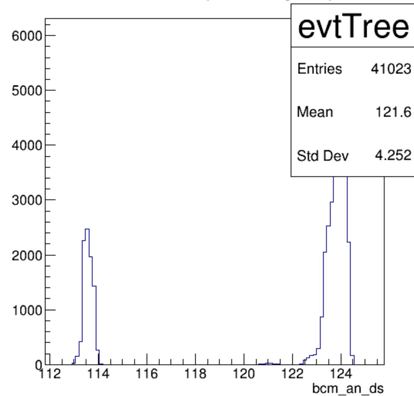
bcm_an_ds {ErrorFlag==0}
