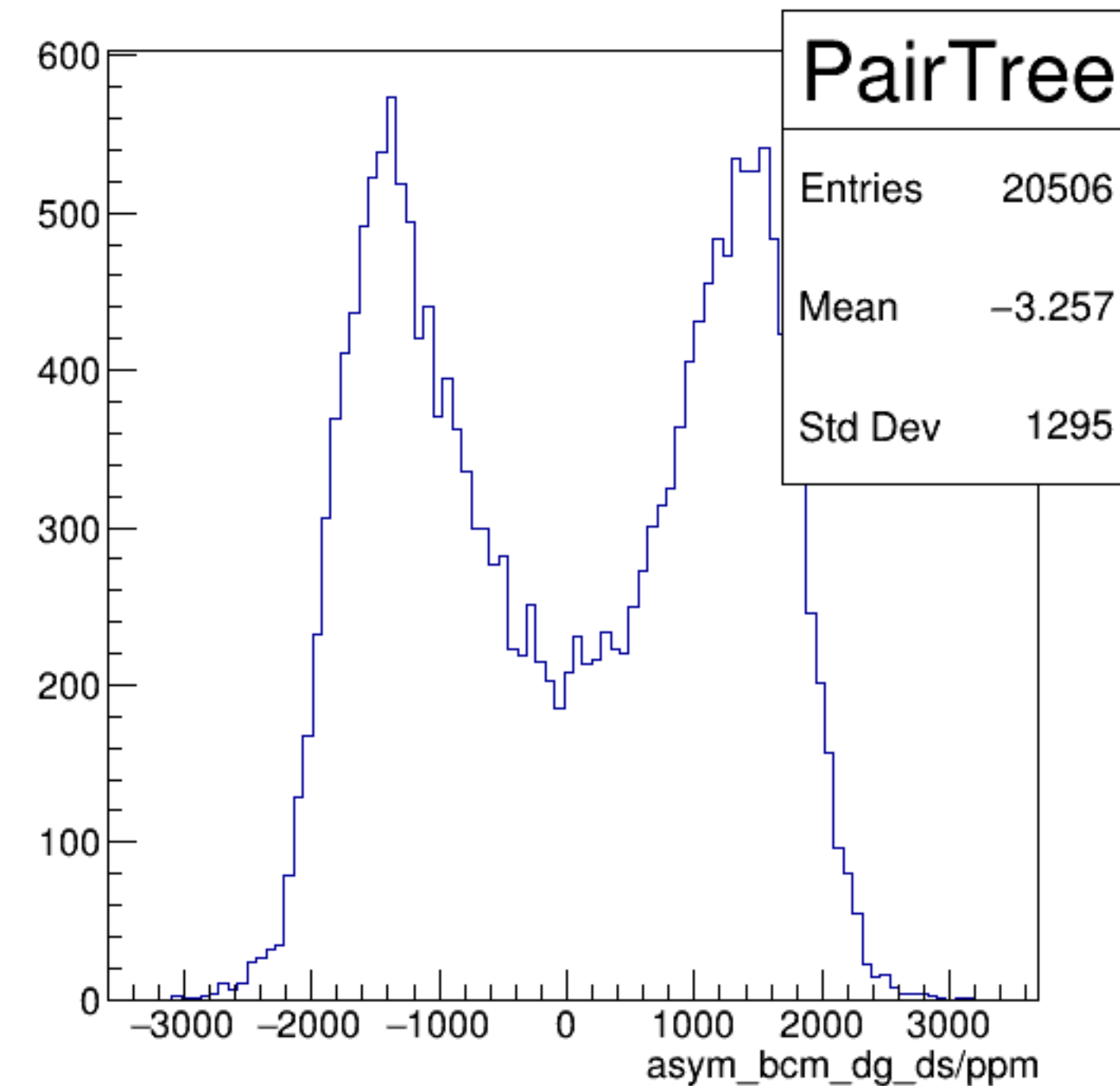
asym_bcm_dg_ds/ppm {ErrorFlag==0}
