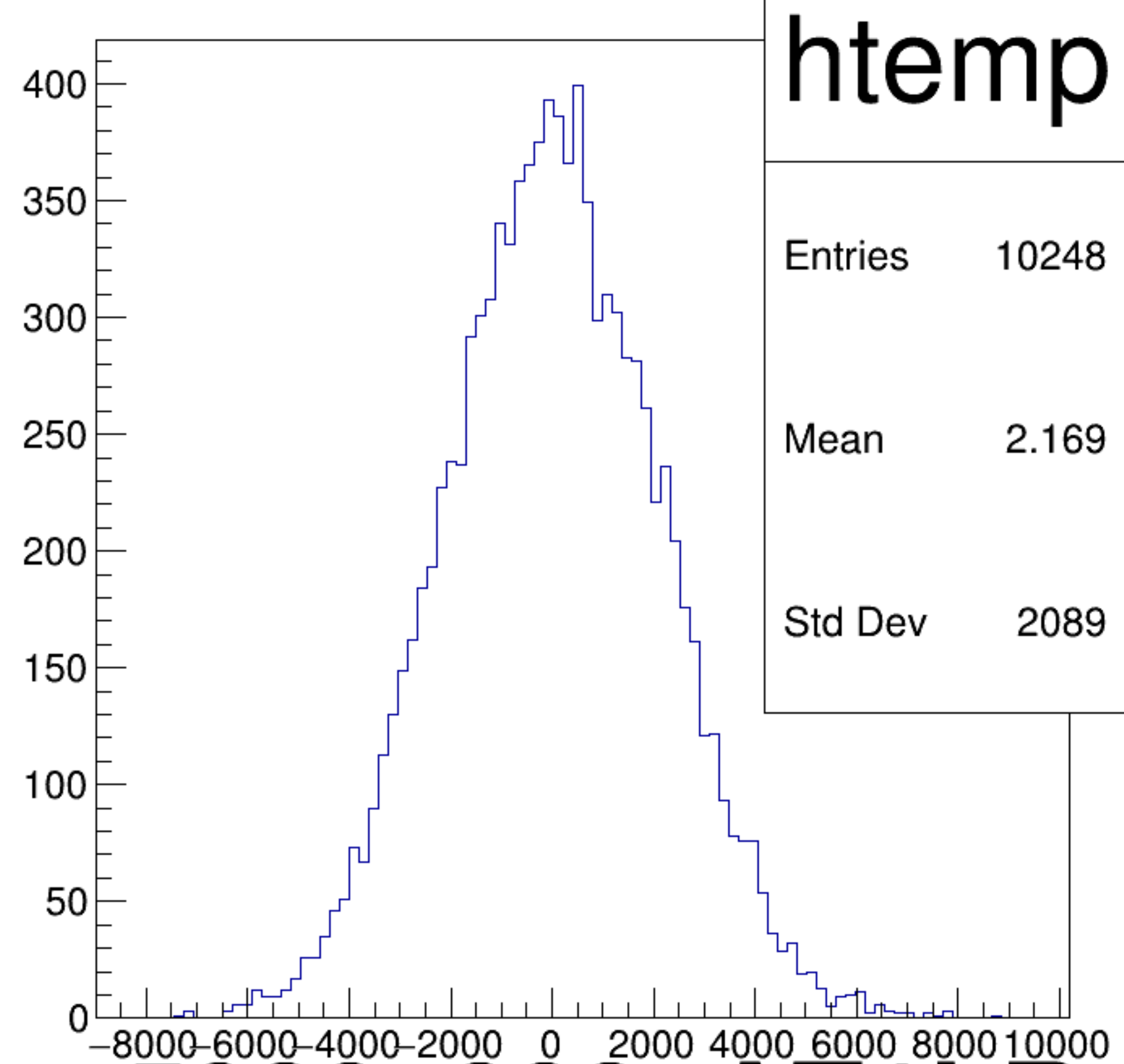
(asym_atl1/ppm-asym_atr1/ppm)/2 {ok_cut}
