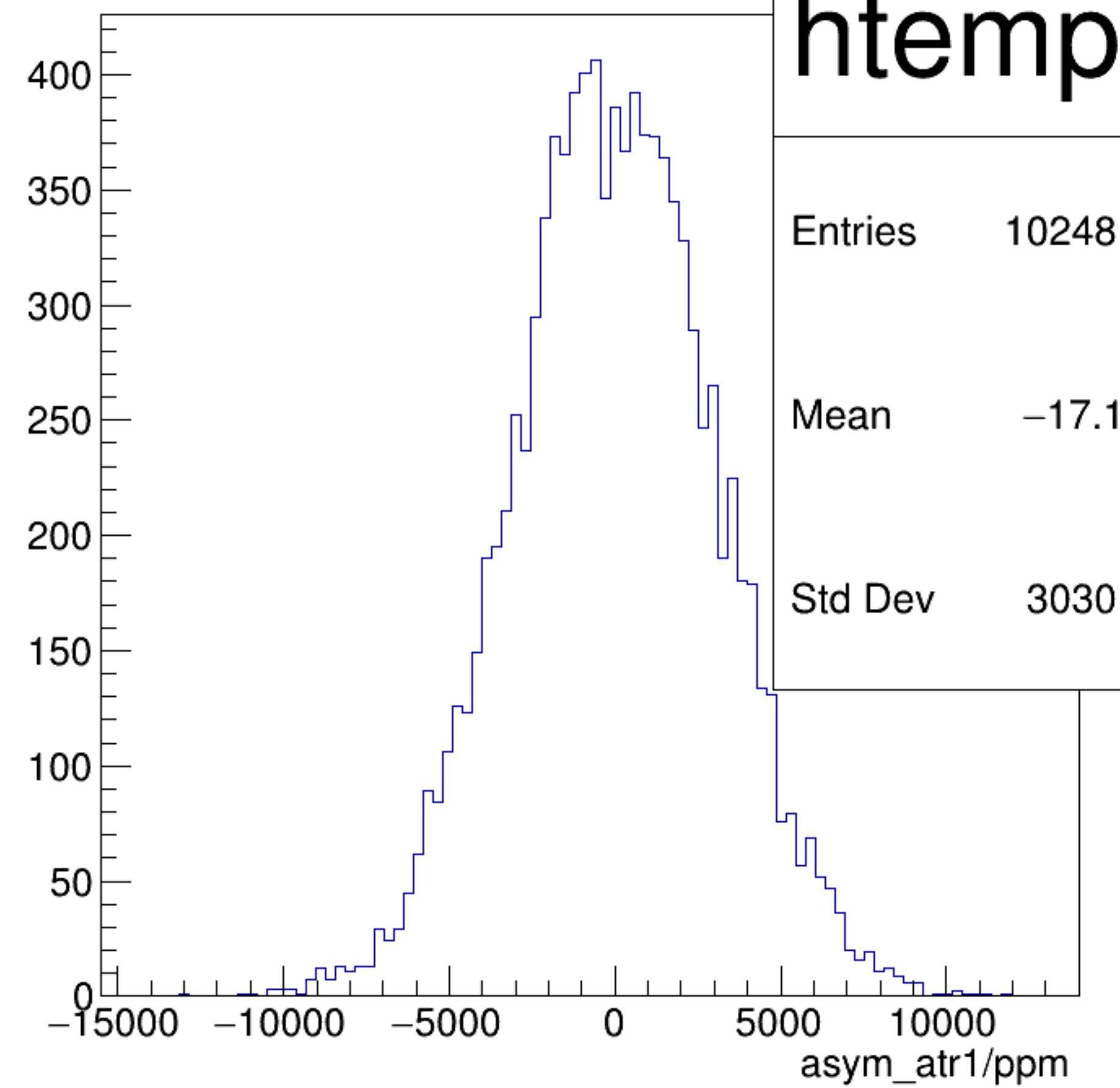
asym_atr1/ppm {ok_cut}
