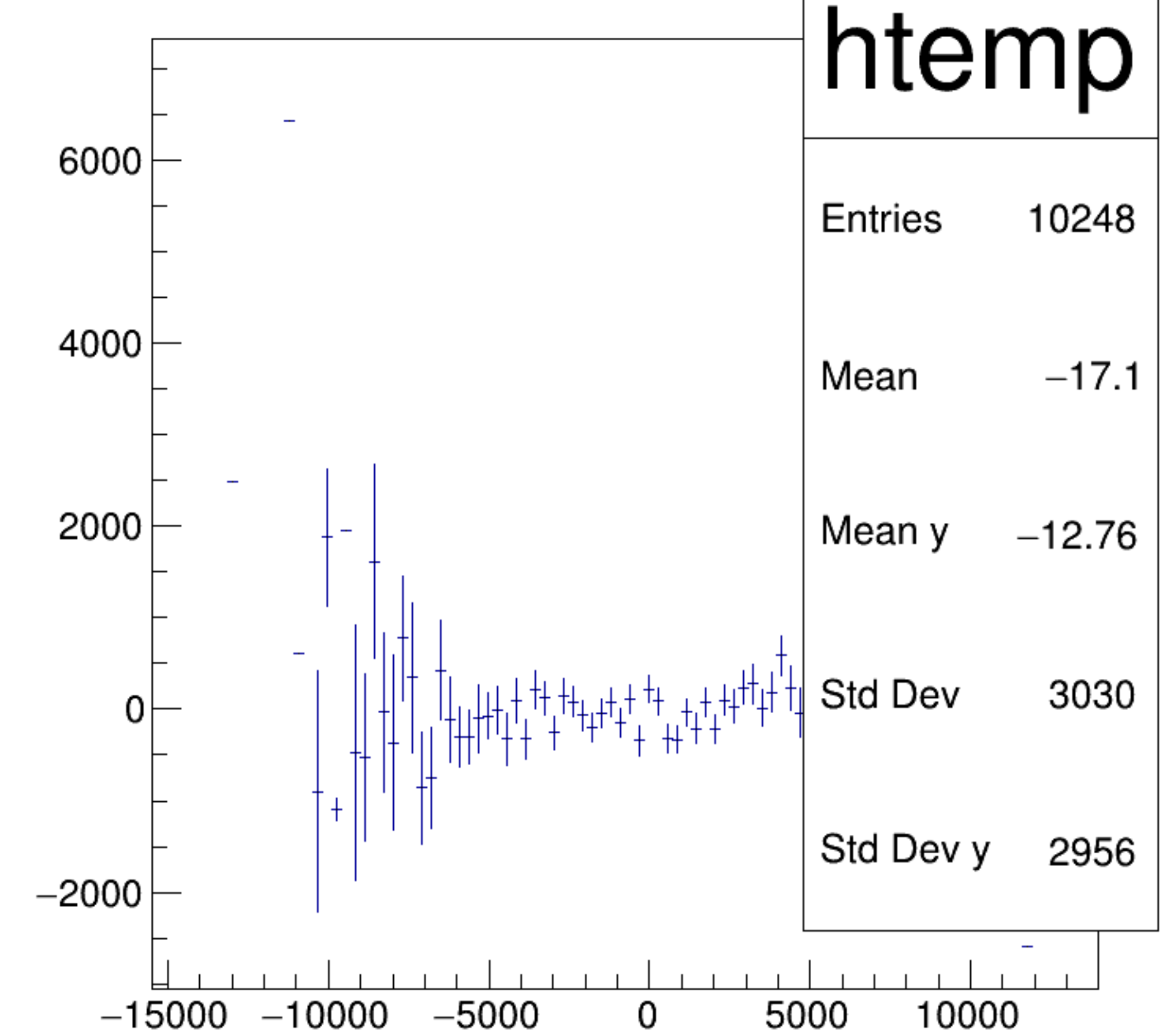
asym_atl1/ppm:asym_atr1/ppm {ok_cut}
