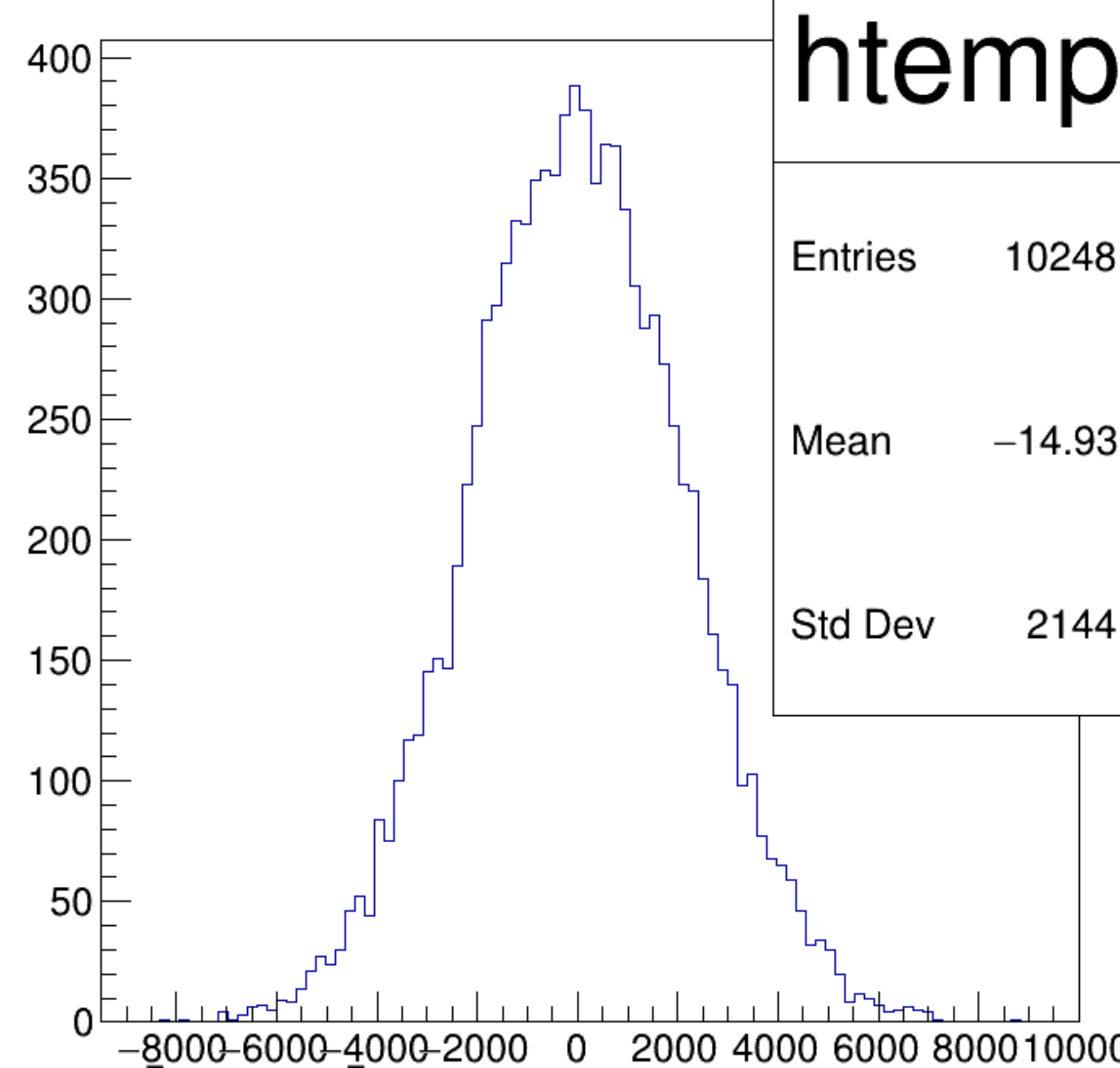
(asym_atl1/ppm+asym_atr1/ppm)/2 {ok_cut}
