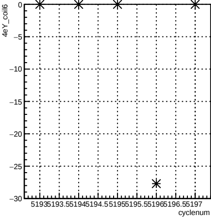
4eY_coil6:cyclenum {run == 5939}
