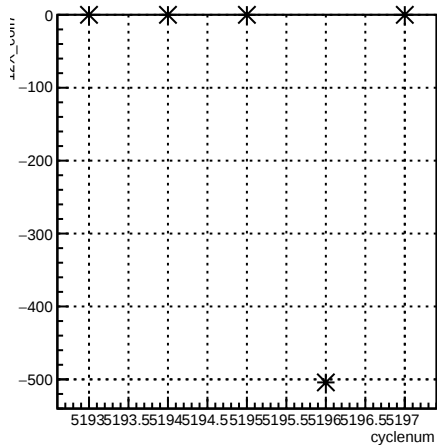
12X_coil7:cyclenum {run == 5939}
