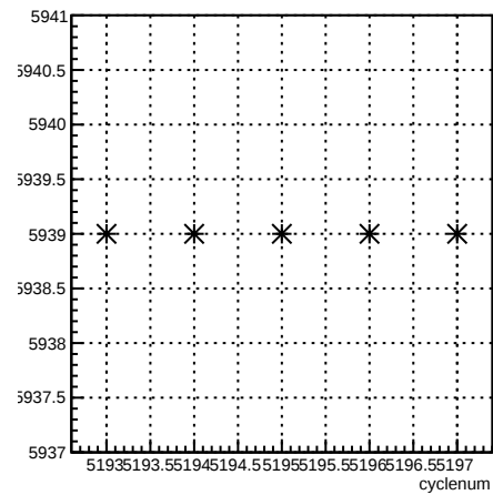
run:cyclenum {run == 5939}
