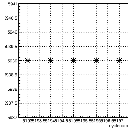
run:cyclenum {run == 5939}
