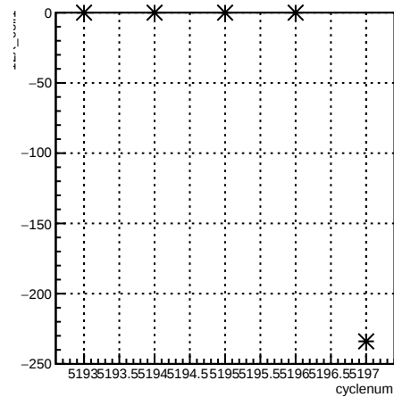
12X_coil1:cyclenum {run == 5939}
