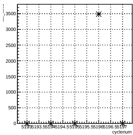
usl_coil3:cyclenum {run == 5939}
