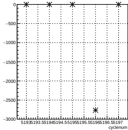
usr_coil3:cyclenum {run == 5939}
