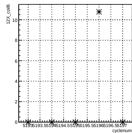
12X_coil6:cyclenum {run == 5939}
