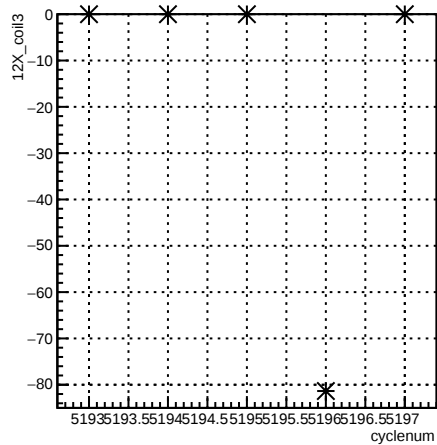
12X_coil3:cyclenum {run == 5939}
