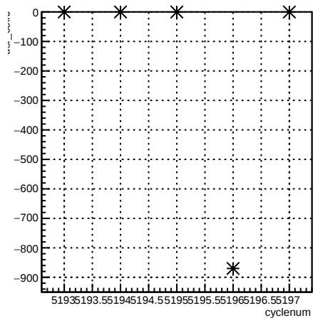
usr_coil6:cyclenum {run == 5939}
