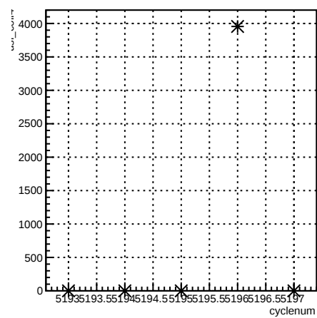
usl_coil4:cyclenum {run == 5939}
