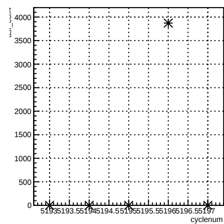
usr_coil4:cyclenum {run == 5939}
