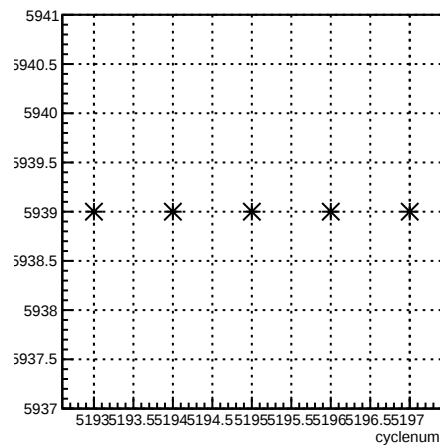
run:cyclenum {run == 5939}
