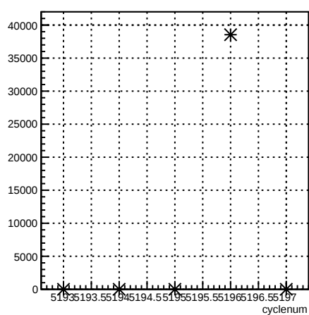
usr_coil7:cyclenum {run == 5939}
