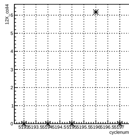
12X_coil4:cyclenum {run == 5939}
