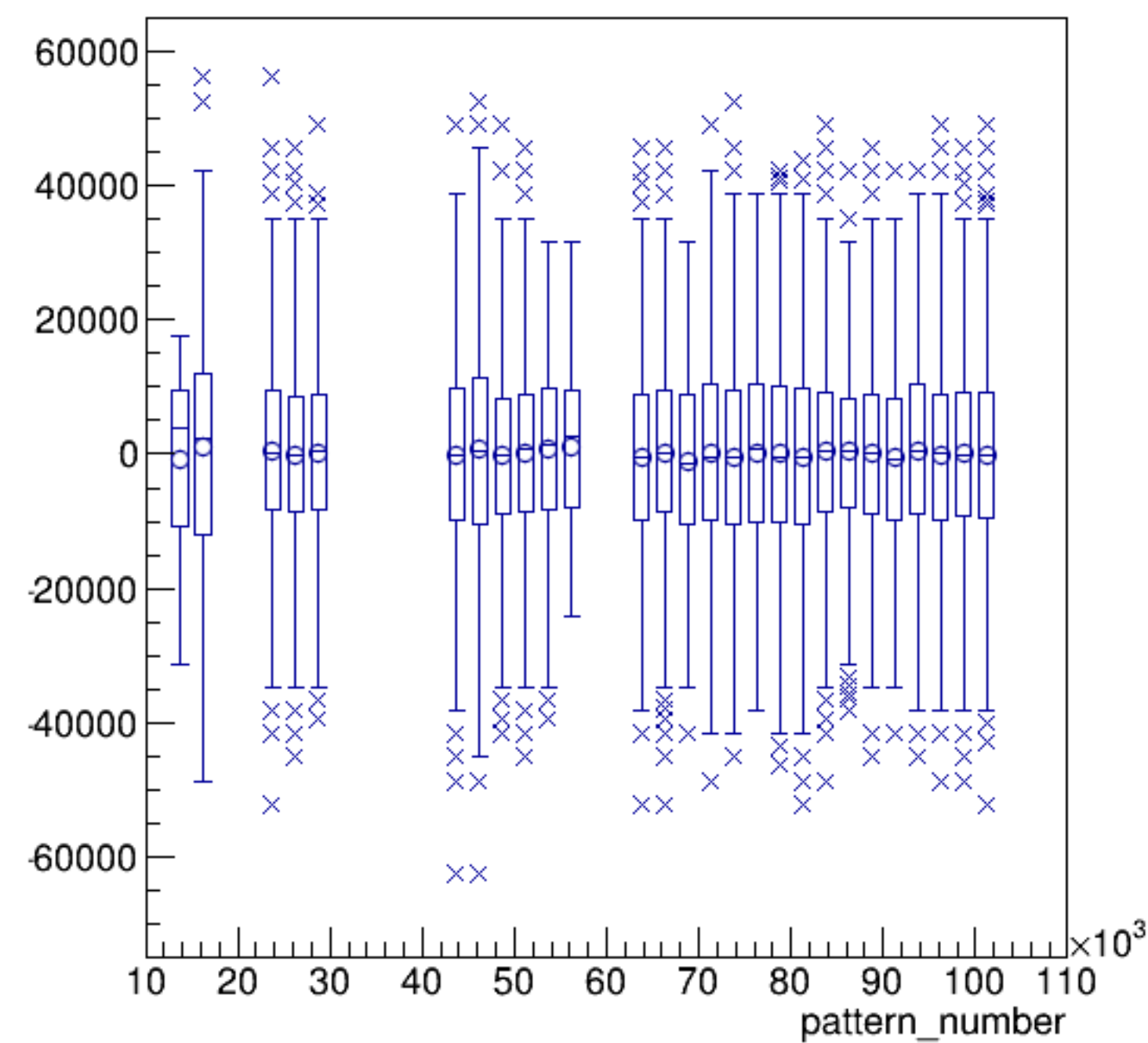
asym_atr2/ppm:pattern_number {ErrorFlag==0}
