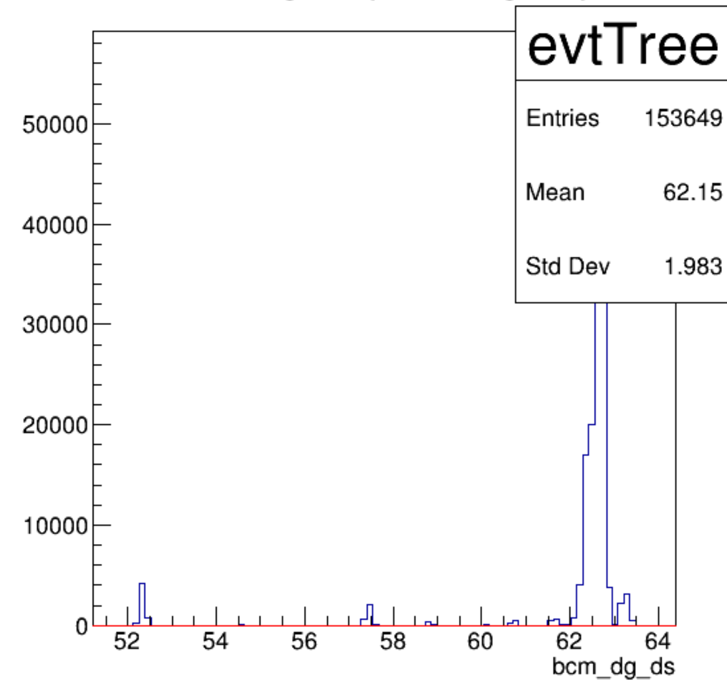
bcm_dg_ds {ErrorFlag==0}
