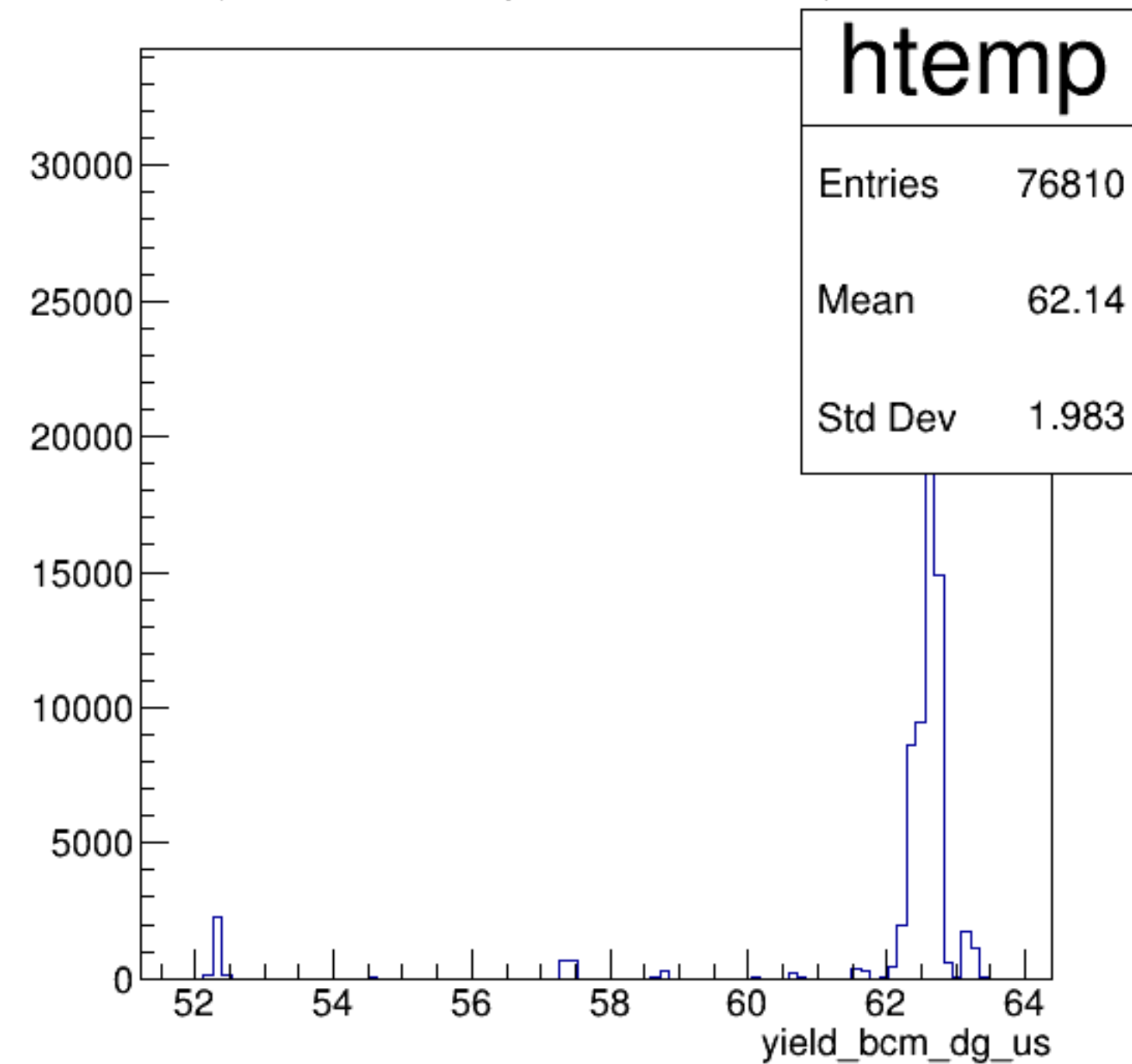
yield_bcm_dg_us {ErrorFlag==0}
