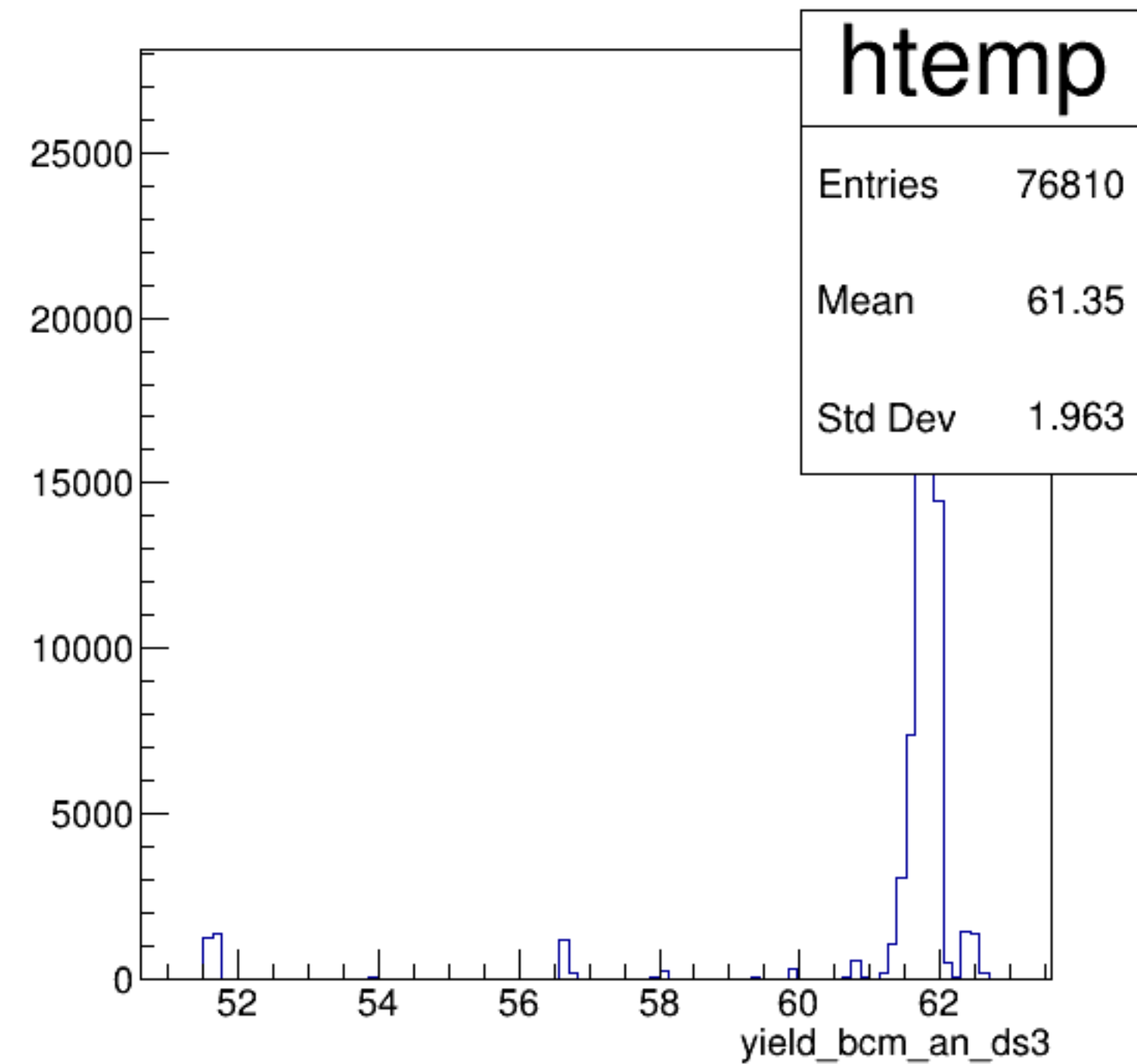
yield_bcm_an_ds3 {ErrorFlag==0}
