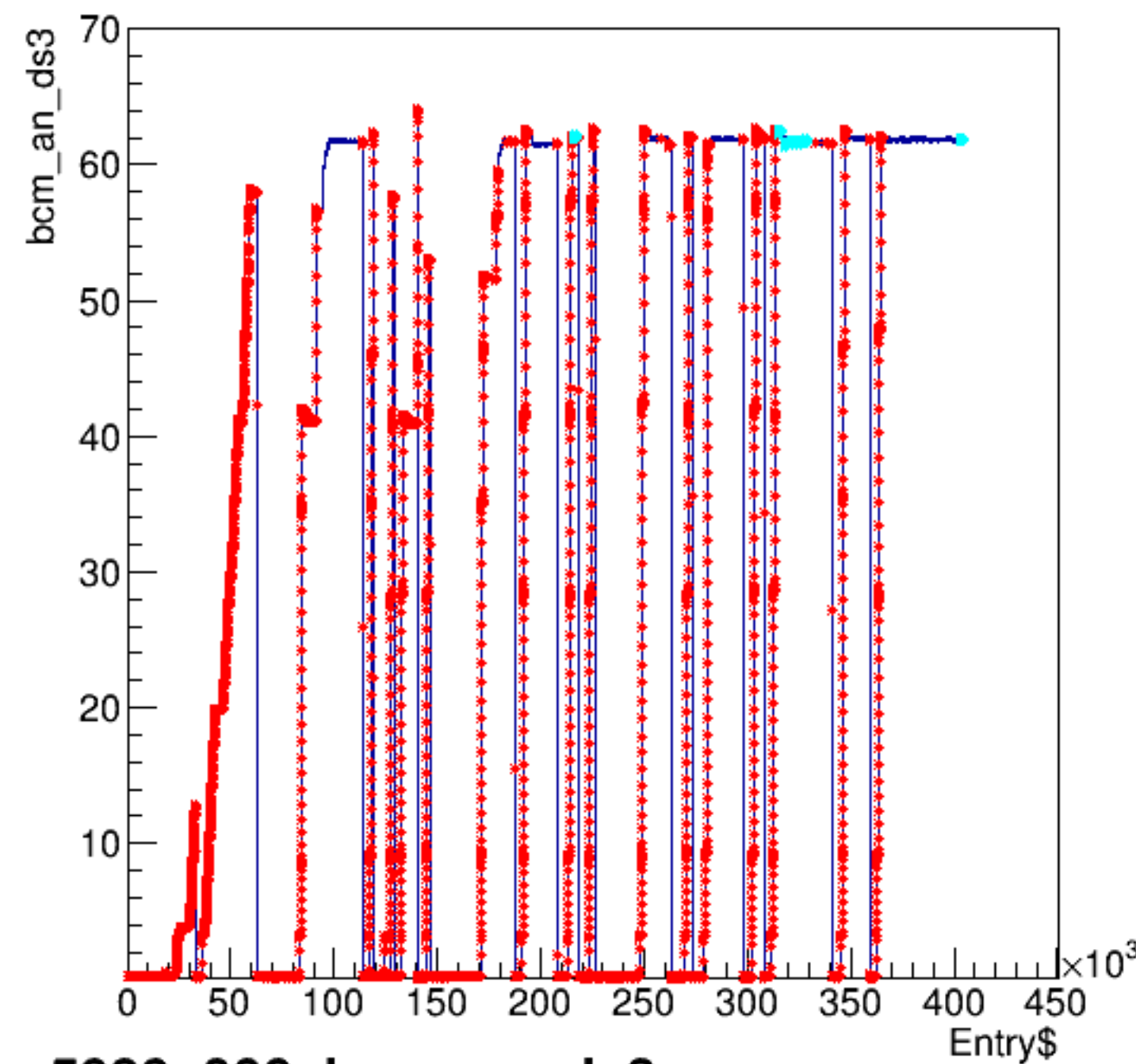
bcm_an_ds3:Entry$
