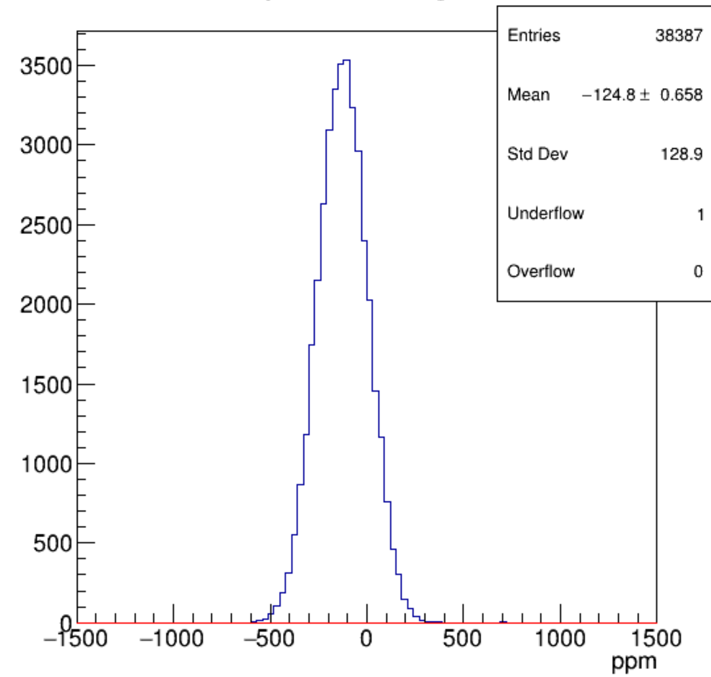
asym_bcm_dg_ds
