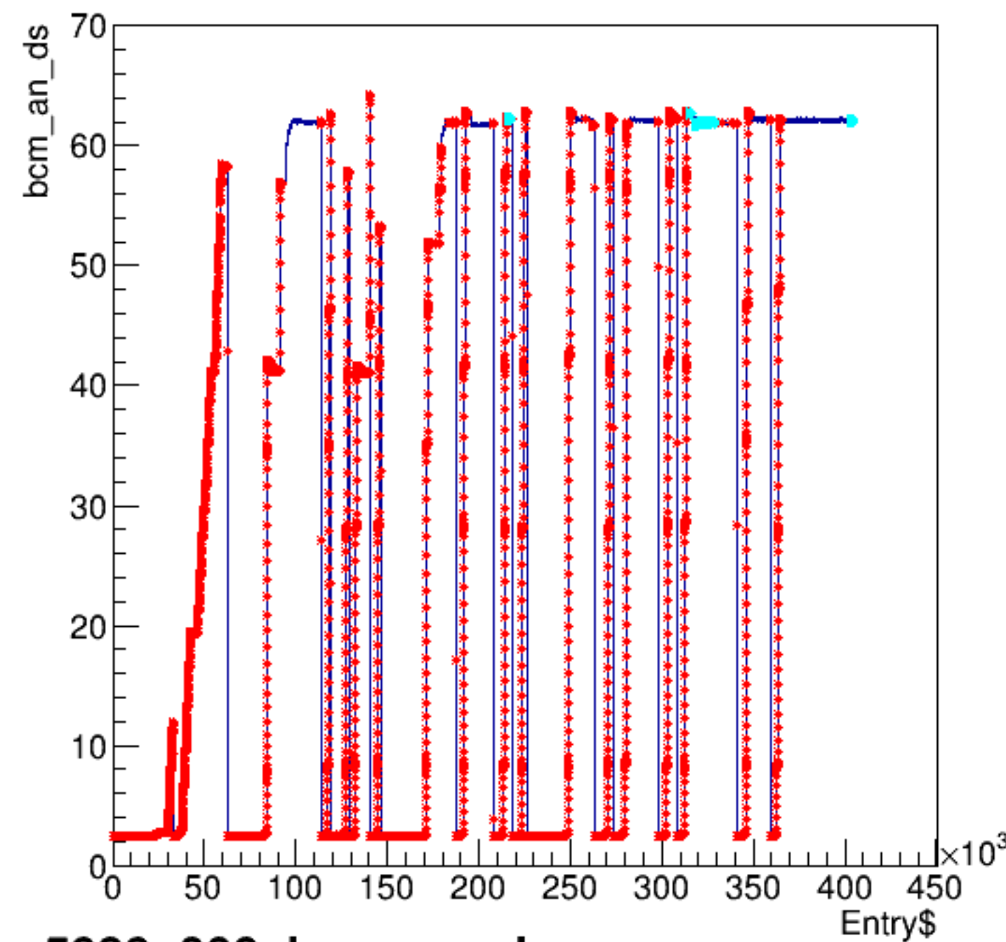
bcm_an_ds:Entry$
