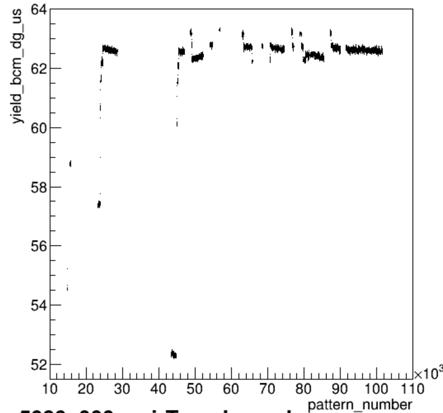
yield_bcm_dg_us:pattern_number {ErrorFlag==0}
