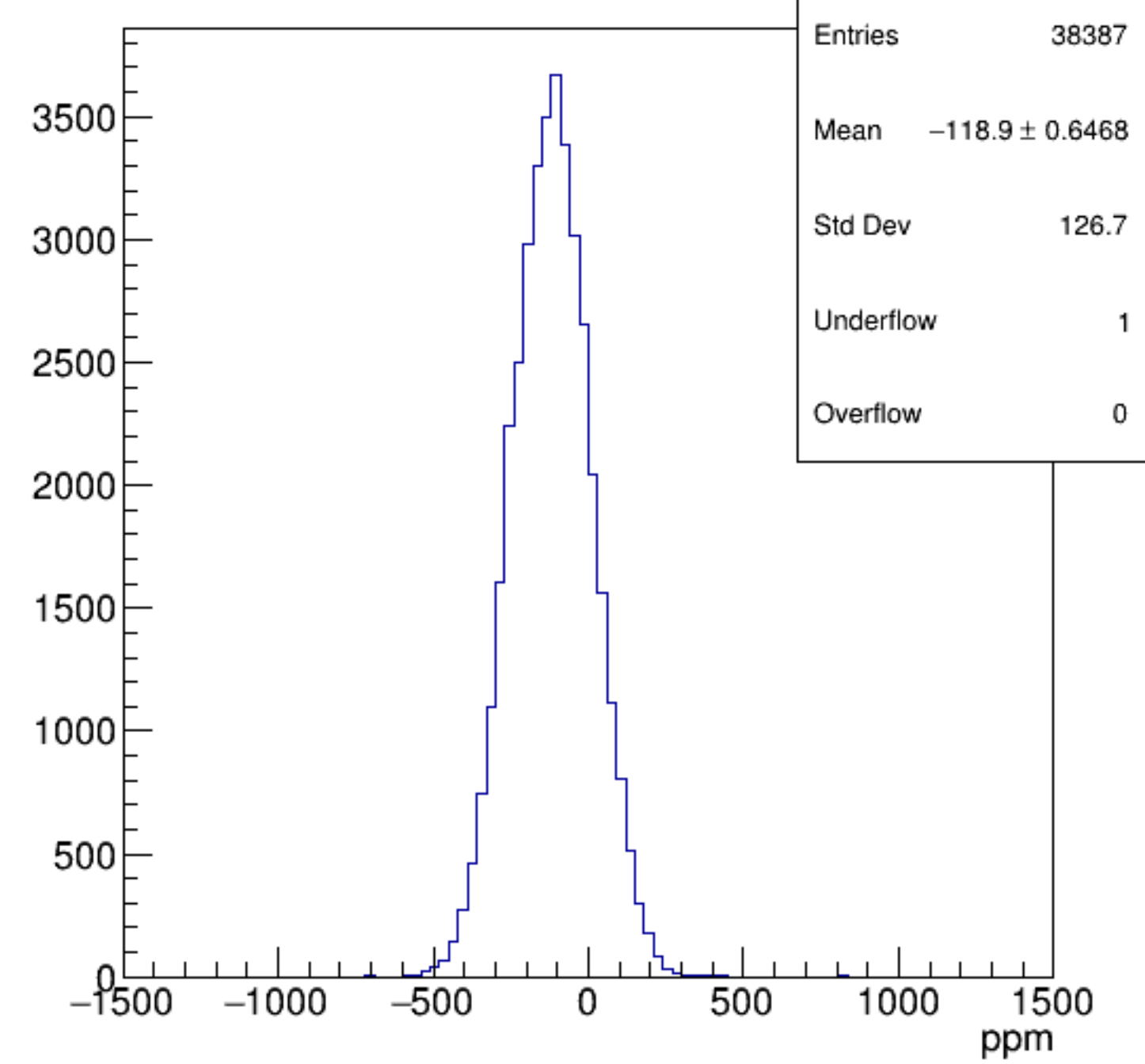
asym_bcm_dg_us
