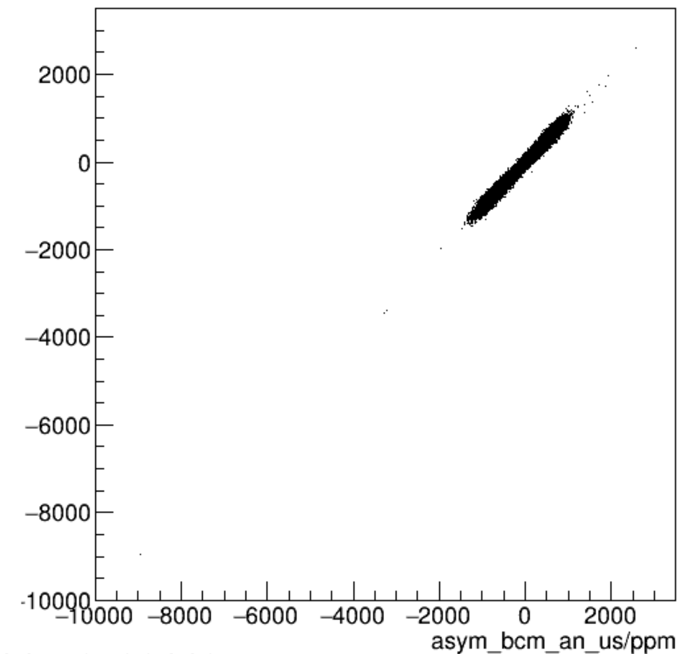
run5939_000_asym_bcm_dg_ds_vs_asym_bcm_an_us_pr.png
