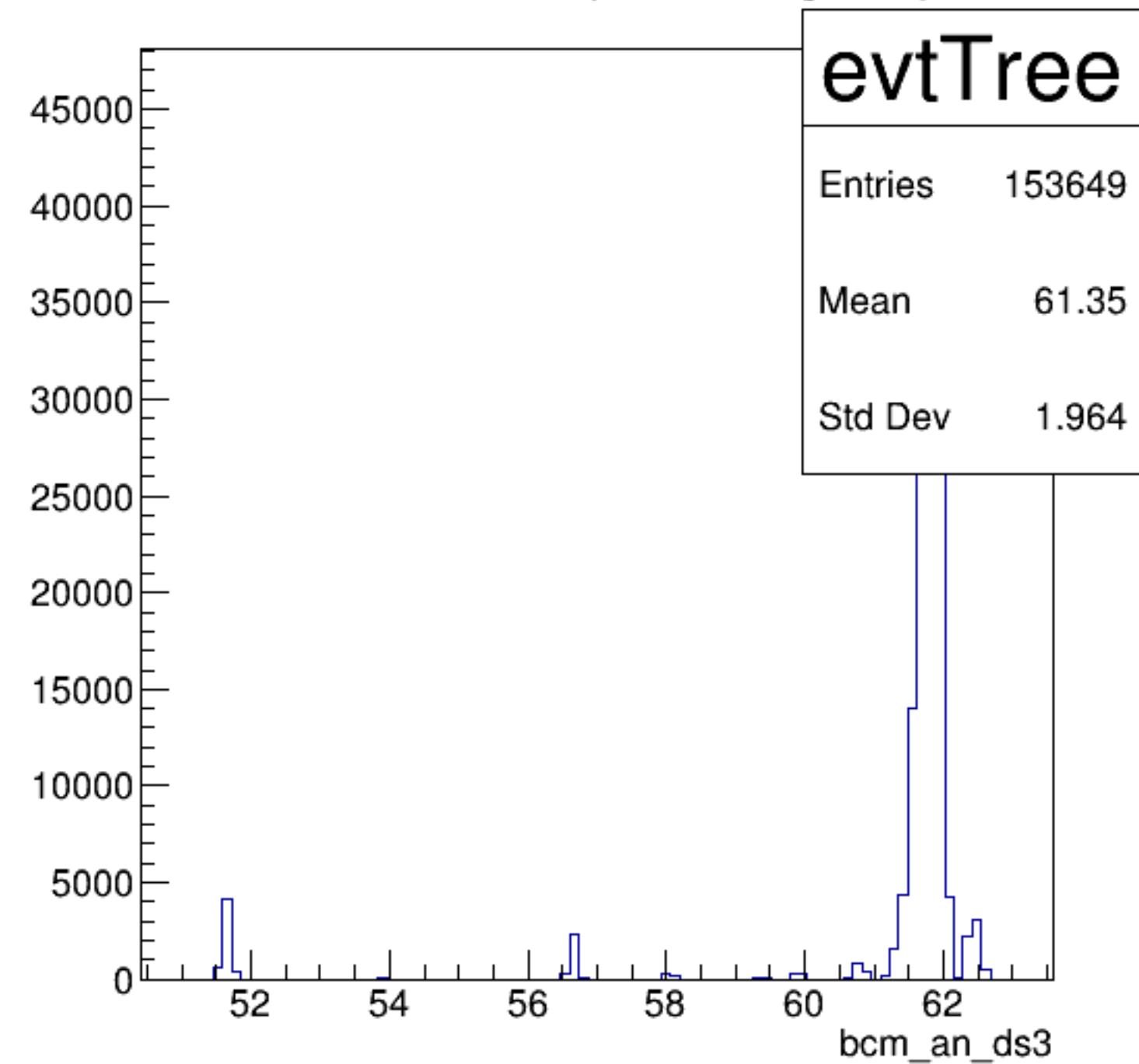
bcm_an_ds3 {ErrorFlag==0}
