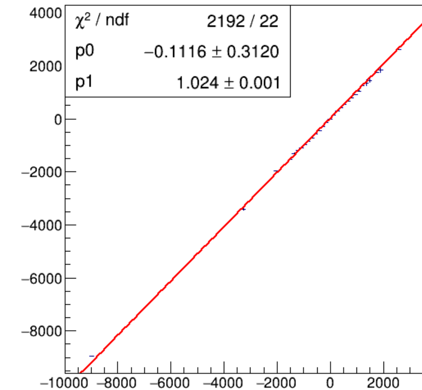
run5939_000_asym_bcm_dg_ds_vs_asym_bcm_an_us_pr.png
