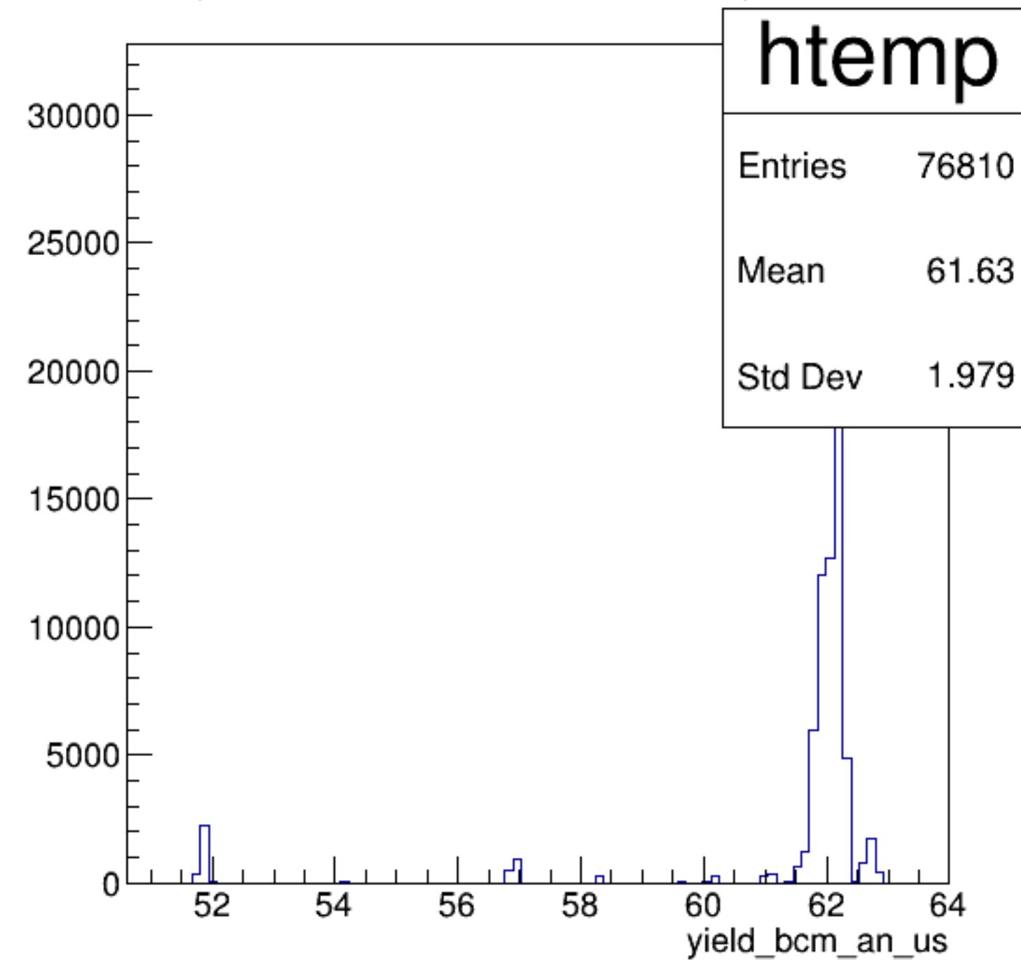
yield_bcm_an_us {ErrorFlag==0}
