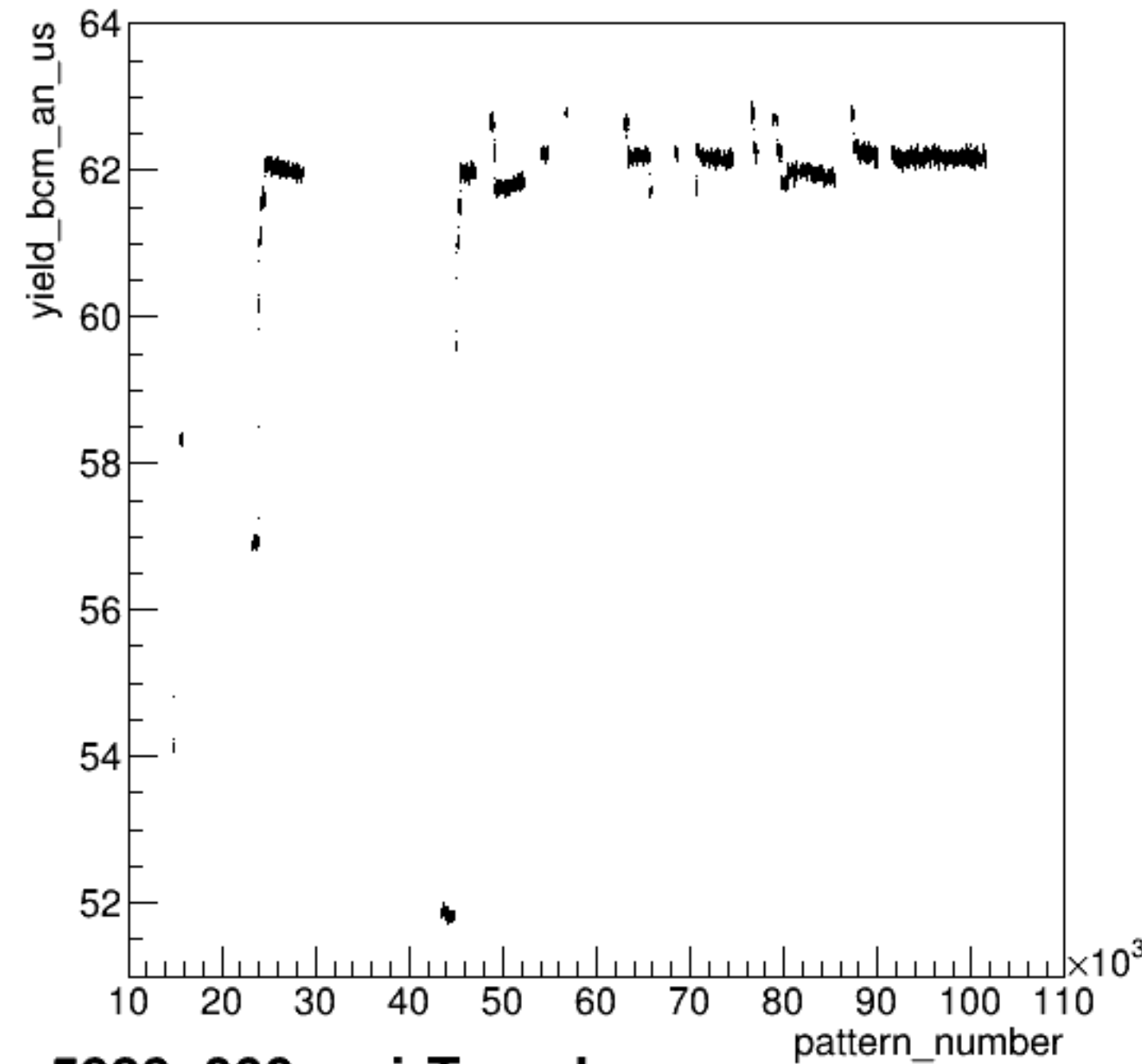
yield_bcm_an_us:pattern_number {ErrorFlag==0}
