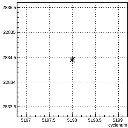
usl_coil6:cyclenum {run == 5940}
