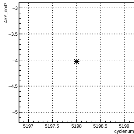
4eY_coil7:cyclenum {run == 5940}
