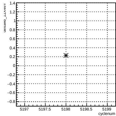
delta46_12X4eY:cyclenum {run == 5940}
