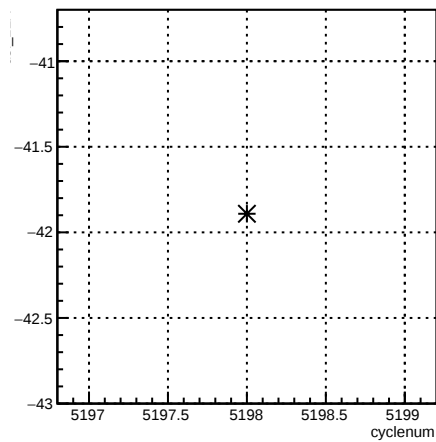
usl_12X:cyclenum {run == 5940}
