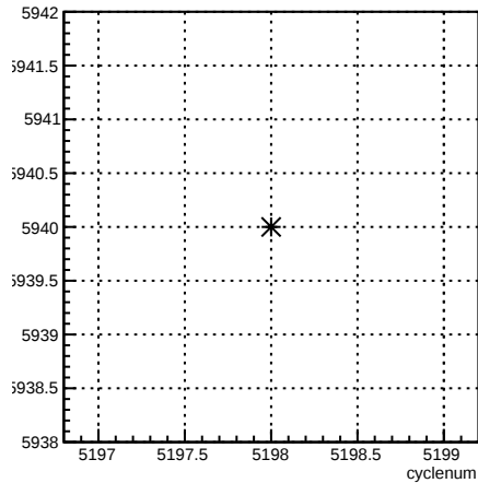
run:cyclenum {run == 5940}
