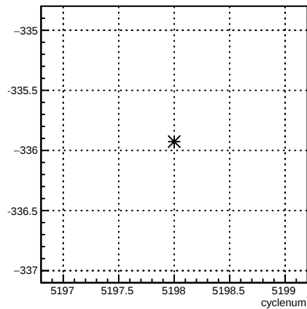
4eX_coil1:cyclenum {run == 5940}
