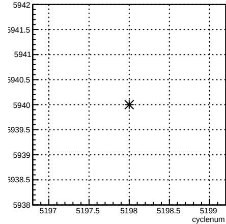
run:cyclenum {run == 5940}
