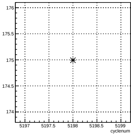
4eY_coil4:cyclenum {run == 5940}
