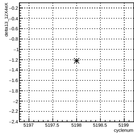
delta13_12X4eX:cyclenum {run == 5940}
