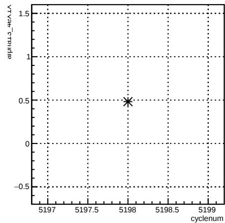
alpha13_4eX1X:cyclenum {run == 5940}
