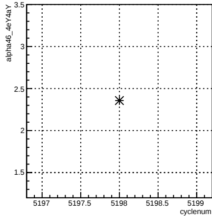
alpha46_4eY4aY:cyclenum {run == 5940}
