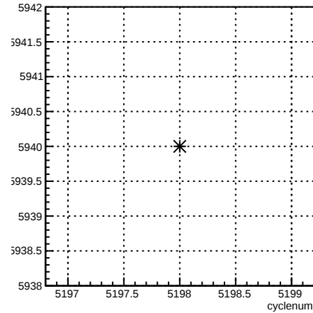
run:cyclenum {run == 5940}
