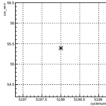
usl_4eX:cyclenum {run == 5940}
