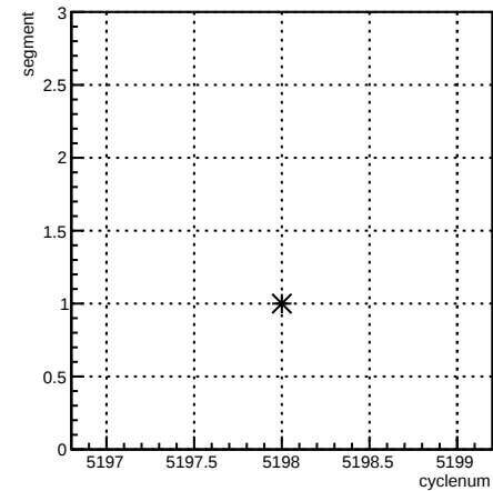
segment:cyclenum {run == 5940}
