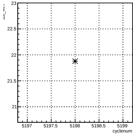
usl_4eY:cyclenum {run == 5940}
