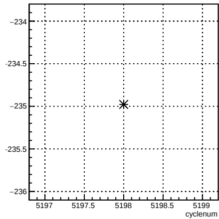
12X_coil6:cyclenum {run == 5940}
