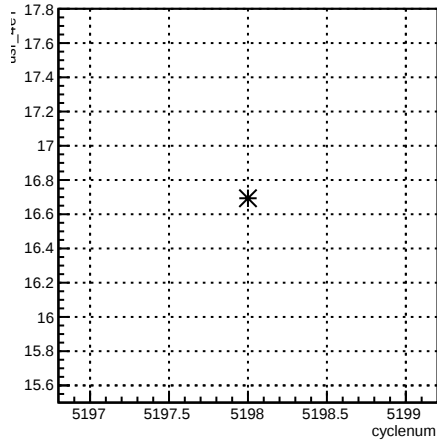
usr_4eY:cyclenum {run == 5940}
