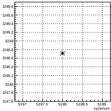
usl_coil7:cyclenum {run == 5940}
