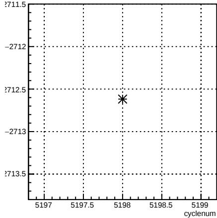
usr_coil7:cyclenum {run == 5940}
