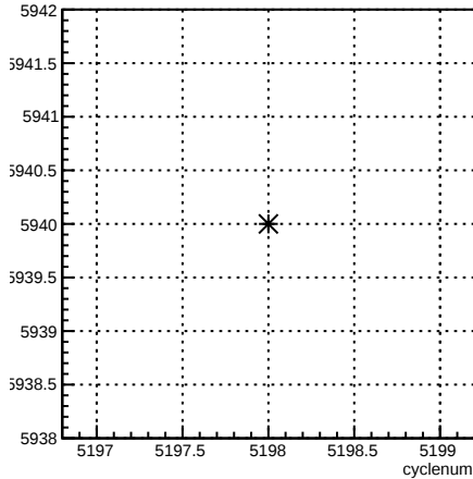
run:cyclenum {run == 5940}
