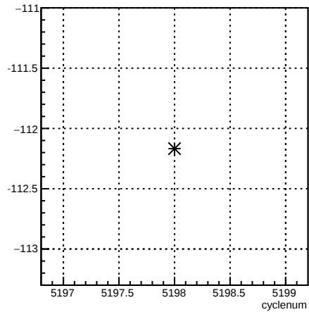
usl_1X:cyclenum {run == 5940}
