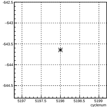
usr_coil6:cyclenum {run == 5940}
