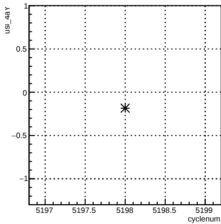
usl_4aY:cyclenum {run == 5940}
