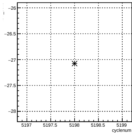
4eY_coil6:cyclenum {run == 5940}
