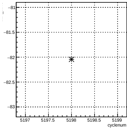
12X_coil7:cyclenum {run == 5940}
