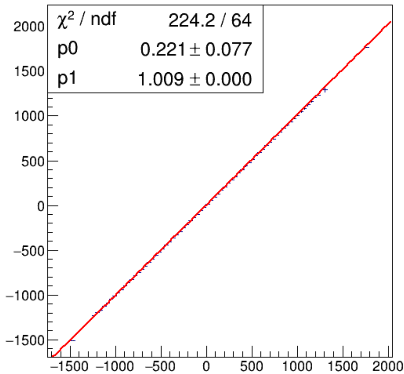
run5940_000_asym_bcm_an_ds_vs_asym_bcm_an_ds3_pr.png
