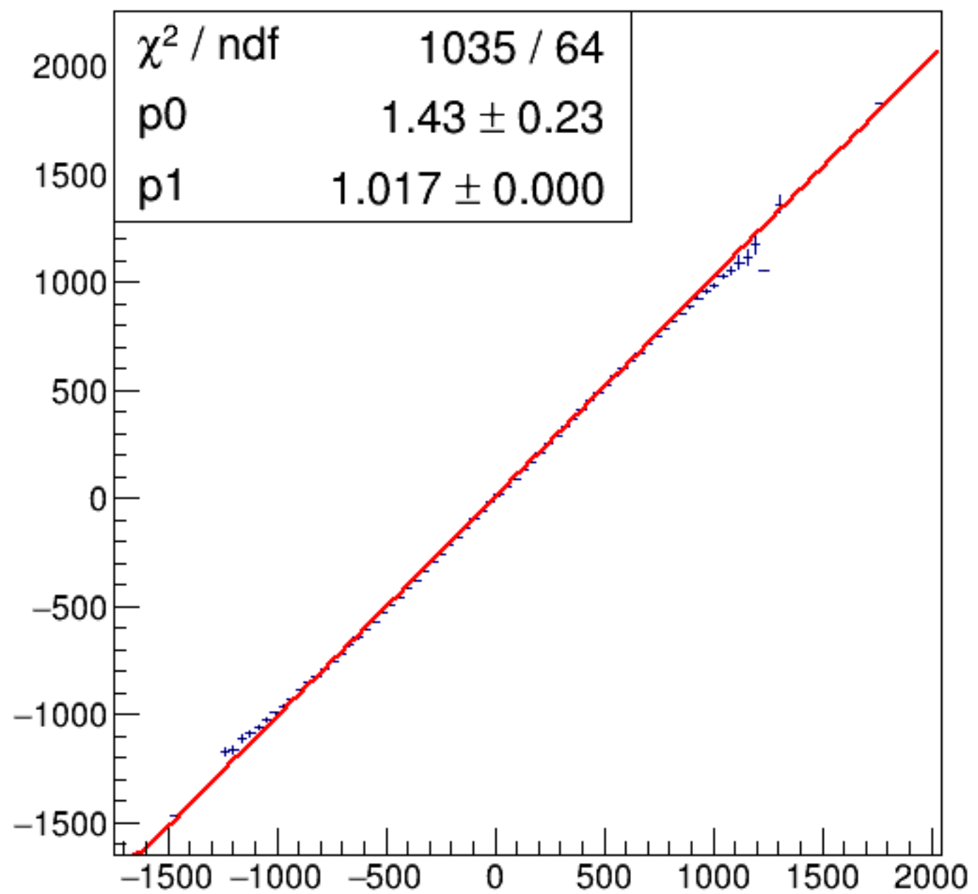
run5940_000_asym_bcm_dg_us_vs_asym_bcm_an_ds3_pr.png
