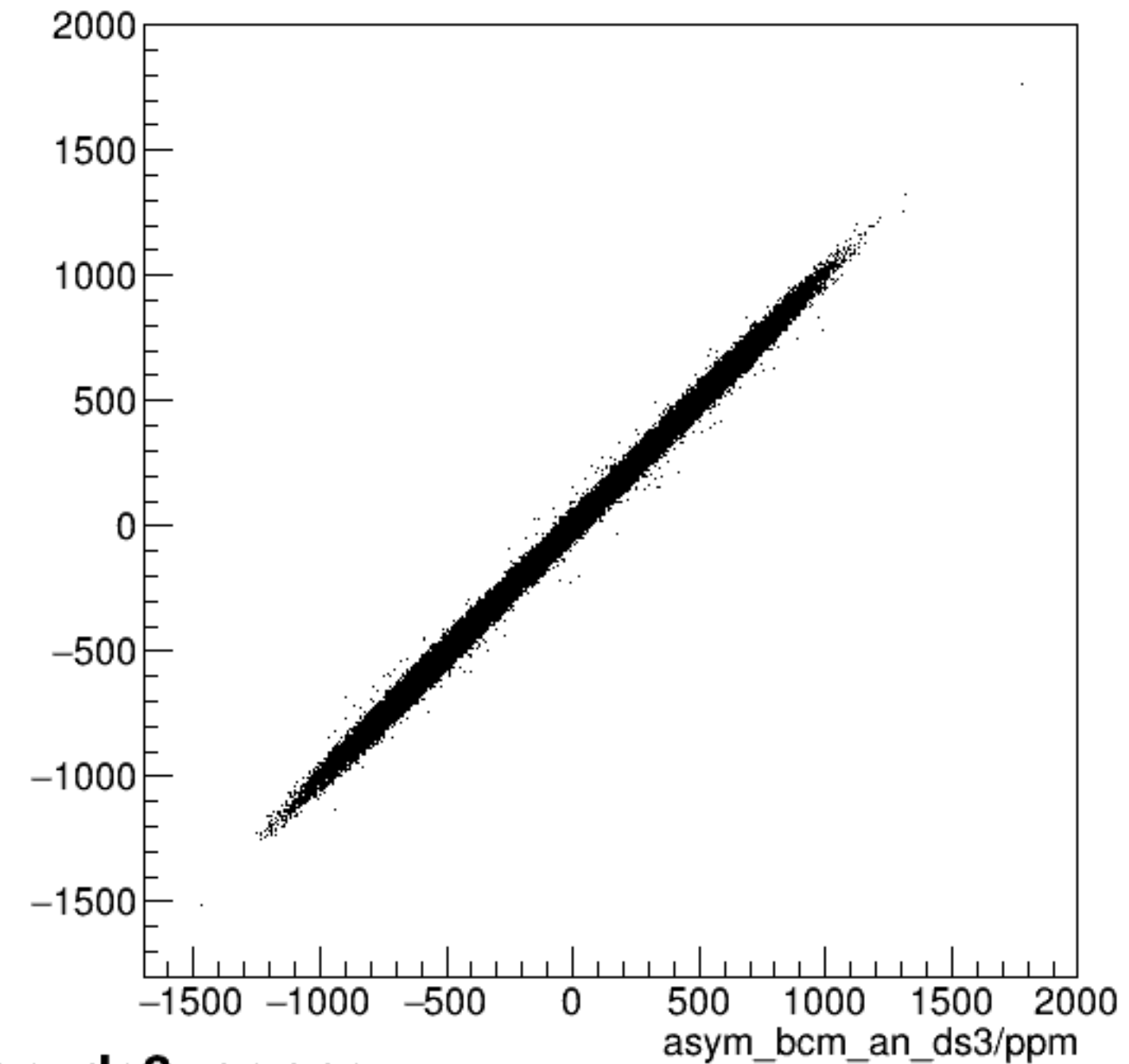
run5940_000_asym_bcm_an_ds_vs_asym_bcm_an_ds3_pr.png
