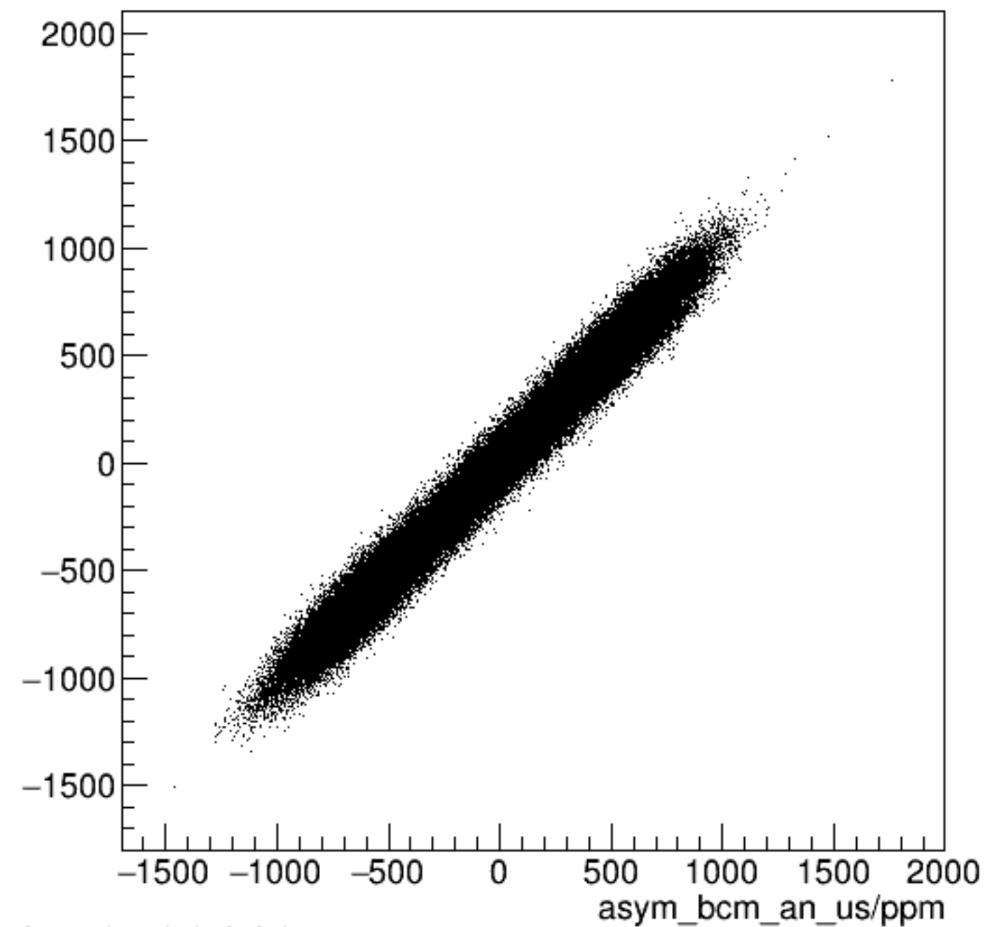
run5940_000_asym_bcm_dg_ds_vs_asym_bcm_an_us_pr.png
