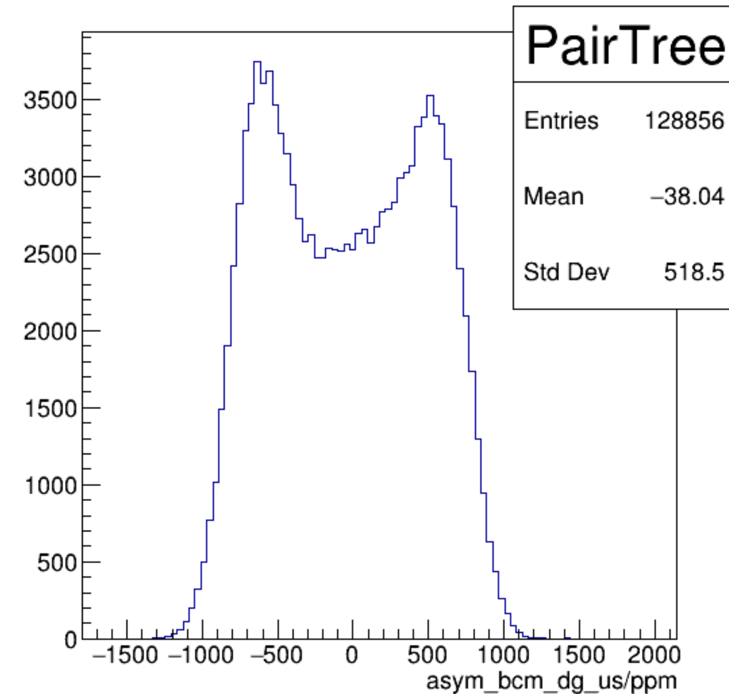
asym_bcm_dg_us/ppm {ErrorFlag==0}
