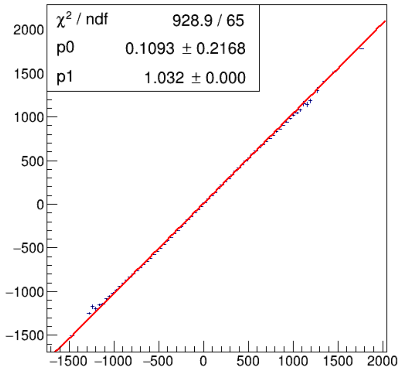
run5940_000_asym_bcm_dg_ds_vs_asym_bcm_an_us_pr.png
