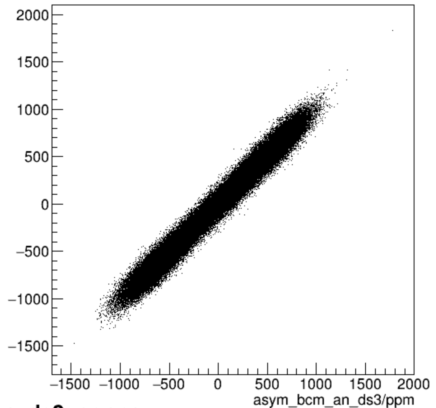
run5940_000_asym_bcm_dg_us_vs_asym_bcm_an_ds3_pr.png
