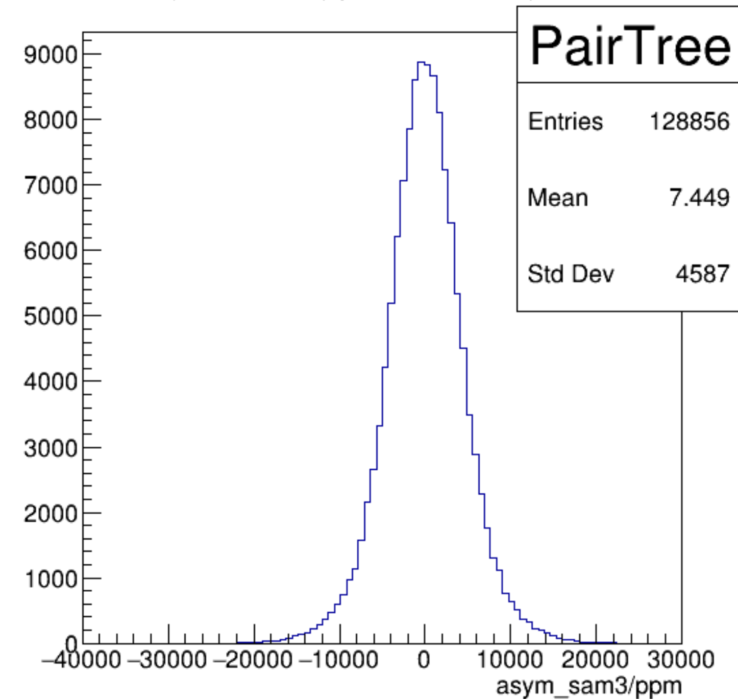
asym_sam3/ppm {ErrorFlag==0}
