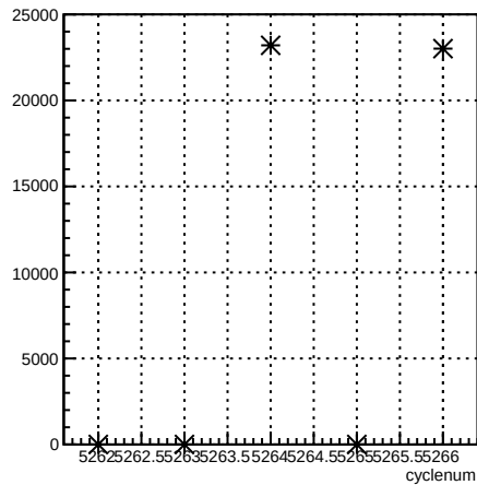
usl_coil1:cyclenum {run == 5958}
