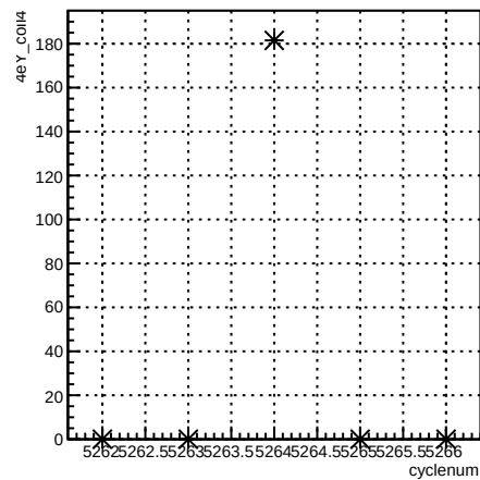
4eY_coil4:cyclenum {run == 5958}
