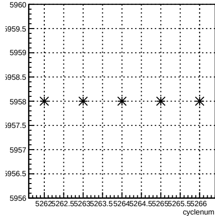
run:cyclenum {run == 5958}
