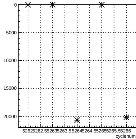
usr_coil1:cyclenum {run == 5958}
