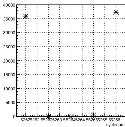
usr_coil7:cyclenum {run == 5958}
