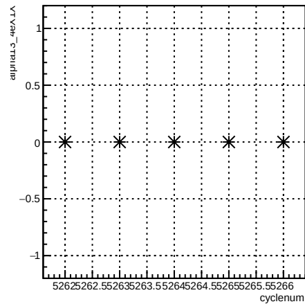
alpha13_4eX1X:cyclenum {run == 5958}
