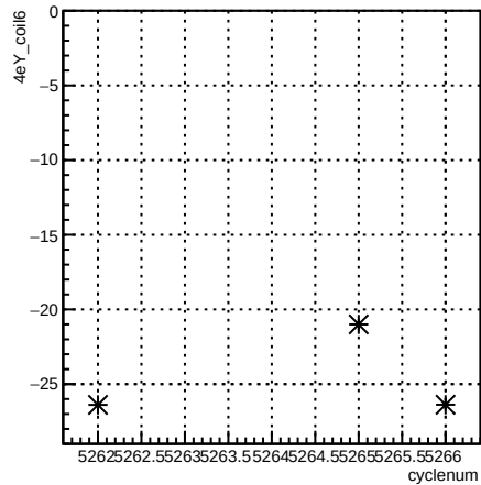
4eY_coil6:cyclenum {run == 5958}
