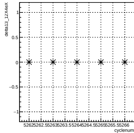
delta13_12X4eX:cyclenum {run == 5958}
