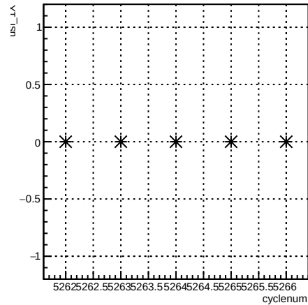
usl_4eY:cyclenum {run == 5958}
