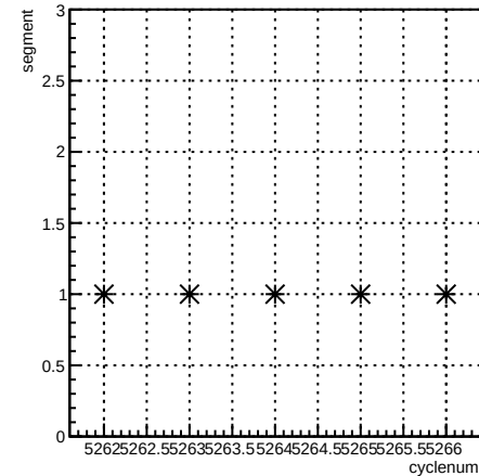
segment:cyclenum {run == 5958}
