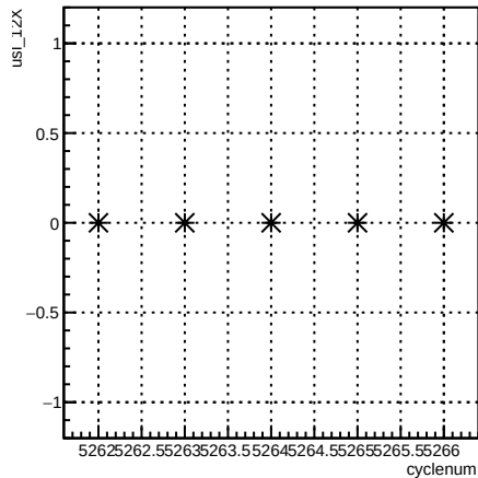
usl_12X:cyclenum {run == 5958}
