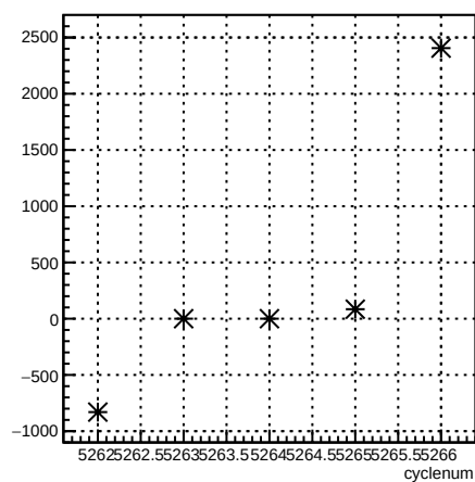
usl_coil7:cyclenum {run == 5958}
