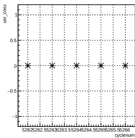
usr_coil3:cyclenum {run == 5958}
