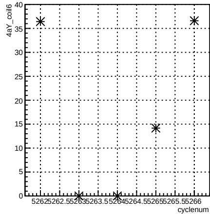
4aY_coil6:cyclenum {run == 5958}
