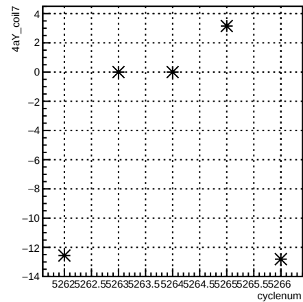
4aY_coil7:cyclenum {run == 5958}
