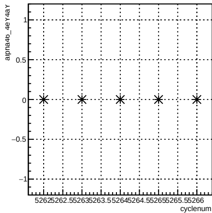
alpha46_4eY4aY:cyclenum {run == 5958}
