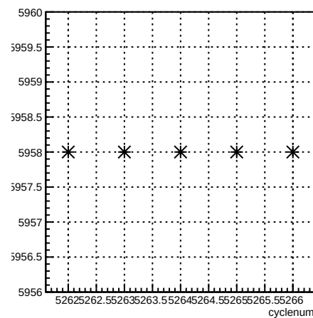
run:cyclenum {run == 5958}
