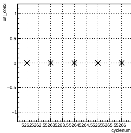
usl_coil3:cyclenum {run == 5958}
