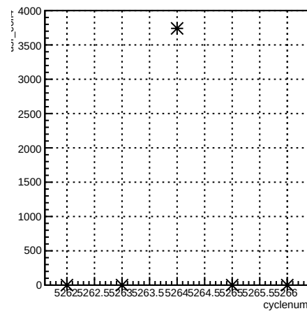
usr_coil4:cyclenum {run == 5958}
