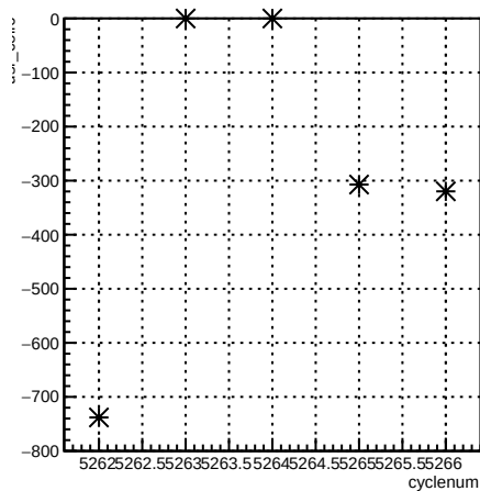
usr_coil6:cyclenum {run == 5958}
