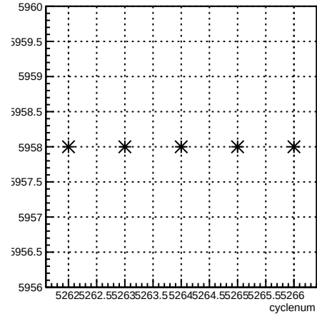
run:cyclenum {run == 5958}
