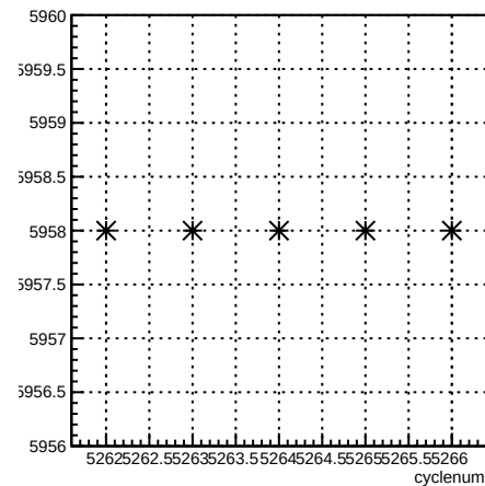
run:cyclenum {run == 5958}
