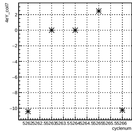
4eY_coil7:cyclenum {run == 5958}
