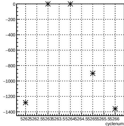
usl_coil6:cyclenum {run == 5958}
