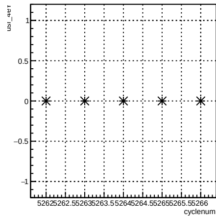
usr_4eY:cyclenum {run == 5958}
