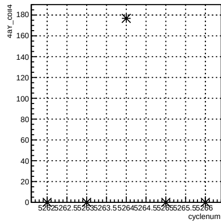
4aY_coil4:cyclenum {run == 5958}
