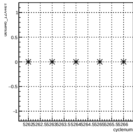
delta46_12X4eY:cyclenum {run == 5958}
