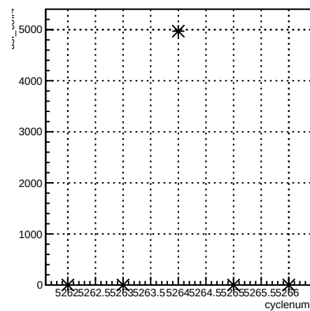
usl_coil4:cyclenum {run == 5958}
