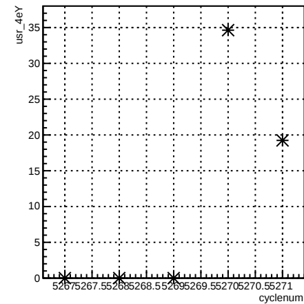
usr_4eY:cyclenum {run == 5959}
