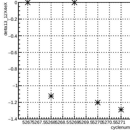
delta13_12X4eX:cyclenum {run == 5959}
