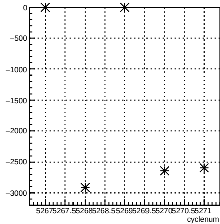
usr_coil3:cyclenum {run == 5959}
