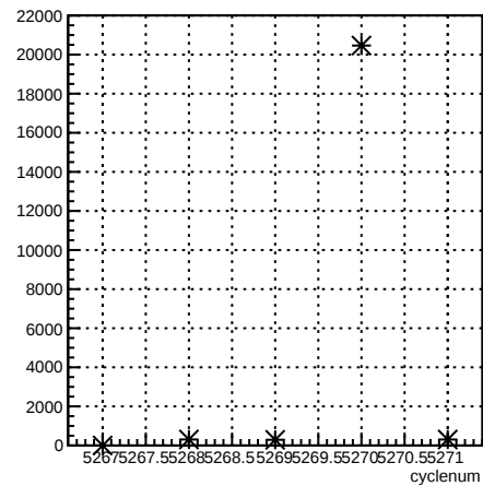
1X_coil7:cyclenum {run == 5959}
