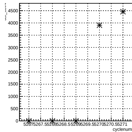
usl_coil4:cyclenum {run == 5959}
