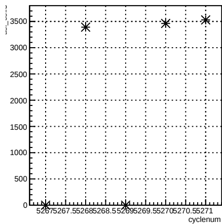
usl_coil3:cyclenum {run == 5959}
