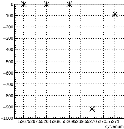
usl_1X:cyclenum {run == 5959}
