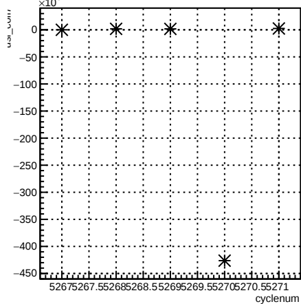
usl_coil7:cyclenum {run == 5959}
