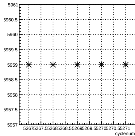
run:cyclenum {run == 5959}
