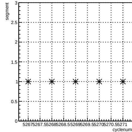
segment:cyclenum {run == 5959}
