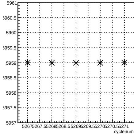
run:cyclenum {run == 5959}
