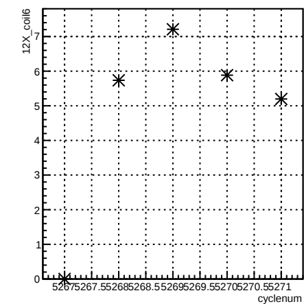
12X_coil6:cyclenum {run == 5959}
