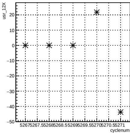
usr_12X:cyclenum {run == 5959}
