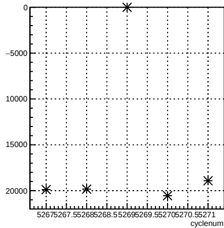
usr_coil1:cyclenum {run == 5959}
