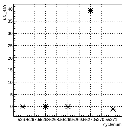
usl_4aY:cyclenum {run == 5959}
