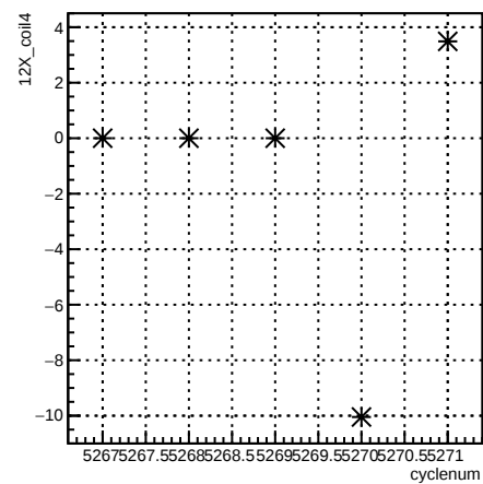
12X_coil4:cyclenum {run == 5959}
