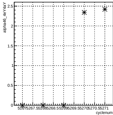
alpha46_4eY4aY:cyclenum {run == 5959}
