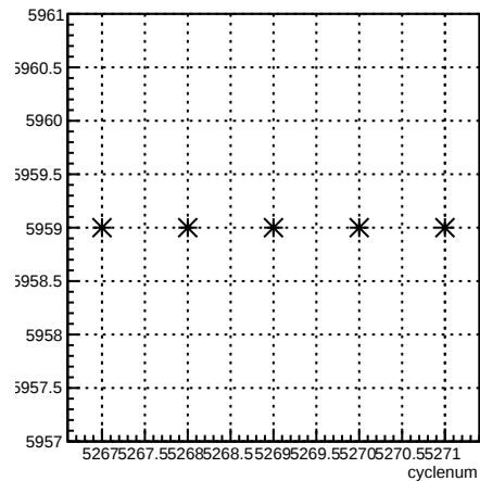
run:cyclenum {run == 5959}
