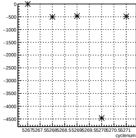
12X_coil7:cyclenum {run == 5959}
