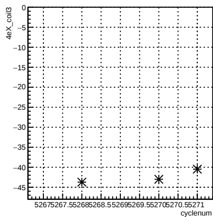
4eX_coil3:cyclenum {run == 5959}
