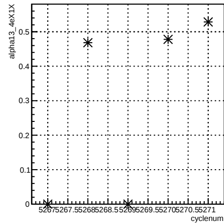
alpha13_4eX1X:cyclenum {run == 5959}
