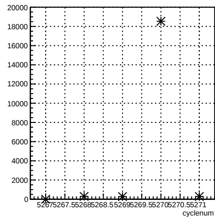
4eX_coil7:cyclenum {run == 5959}
