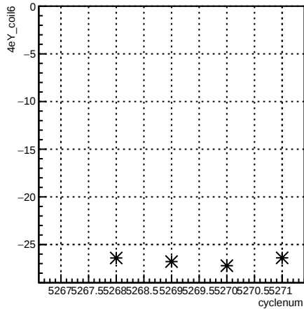
4eY_coil6:cyclenum {run == 5959}
