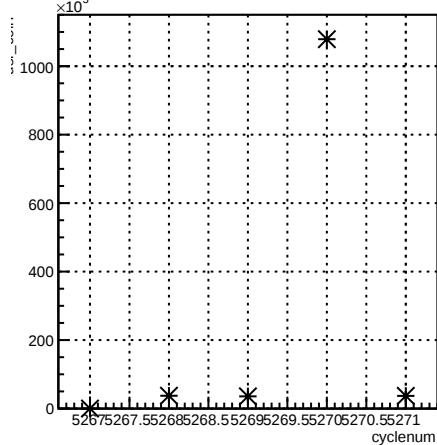
usr_coil7:cyclenum {run == 5959}
