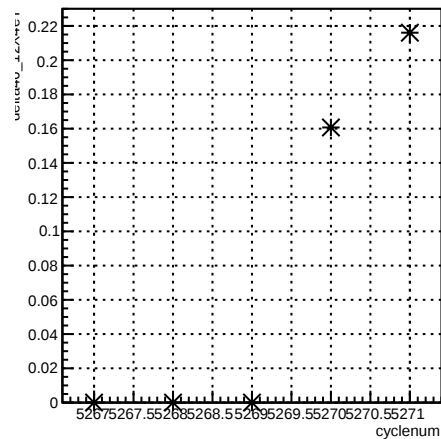
delta46_12X4eY:cyclenum {run == 5959}
