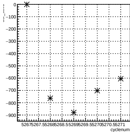
usr_coil6:cyclenum {run == 5959}
