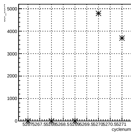
usr_coil4:cyclenum {run == 5959}
