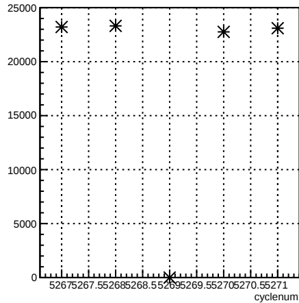
usl_coil1:cyclenum {run == 5959}
