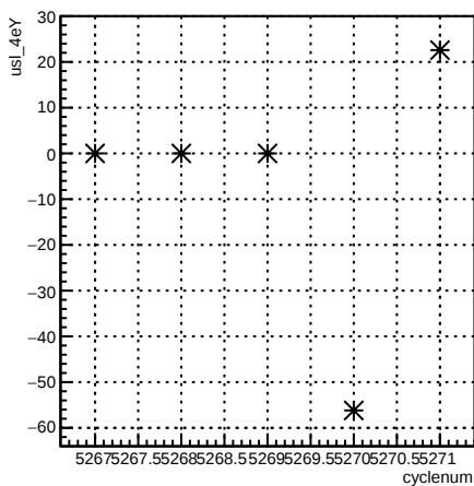
usl_4eY:cyclenum {run == 5959}
