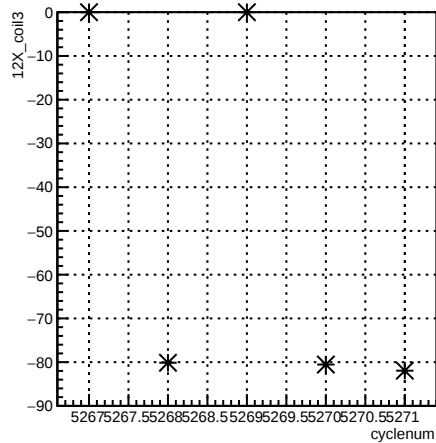
12X_coil3:cyclenum {run == 5959}
