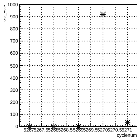
usl_4eX:cyclenum {run == 5959}
