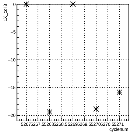
1X_coil3:cyclenum {run == 5959}
