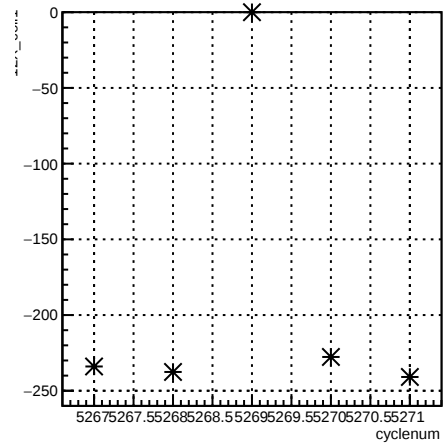
12X_coil1:cyclenum {run == 5959}
