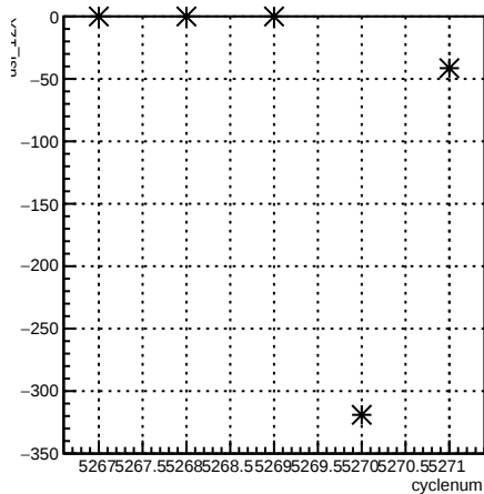
usl_12X:cyclenum {run == 5959}
