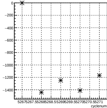
usl_coil6:cyclenum {run == 5959}
