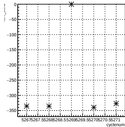
4eX_coil1:cyclenum {run == 5959}
