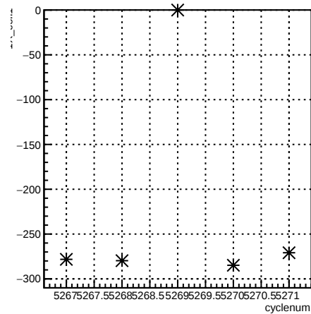
1X_coil1:cyclenum {run == 5959}
