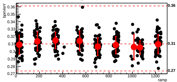
bmod_trim1,cyc=5270
