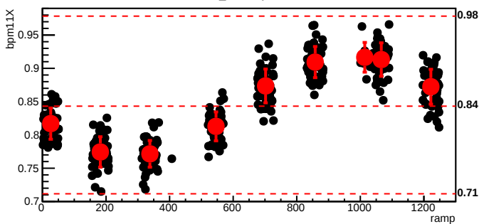
bmod_trim1,cyc=5270
