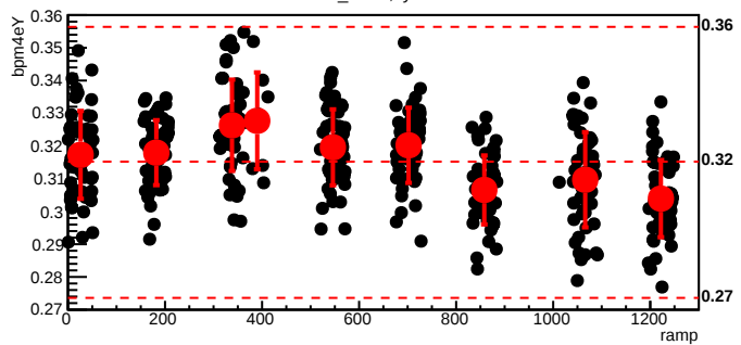
bmod_trim3,cyc=5270
