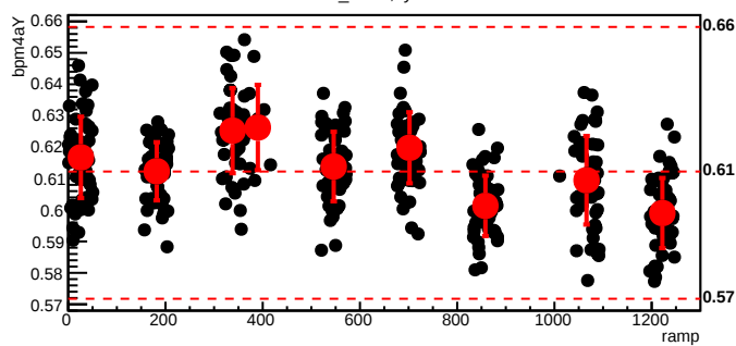
bmod_trim3,cyc=5270
