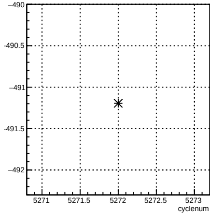
12X_coil7:cyclenum {run == 5960}
