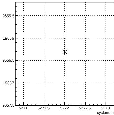
usr_coil1:cyclenum {run == 5960}
