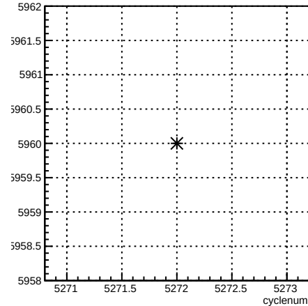
run:cyclenum {run == 5960}
