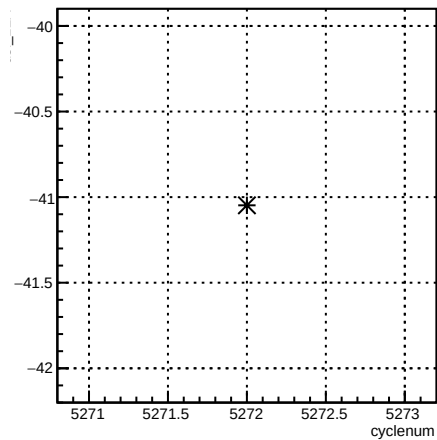
usl_12X:cyclenum {run == 5960}
