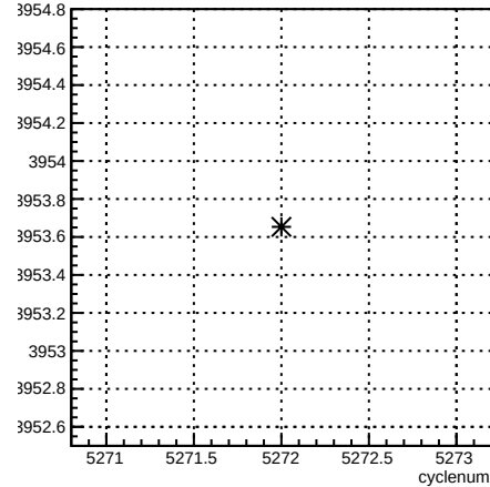
usr_coil4:cyclenum {run == 5960}
