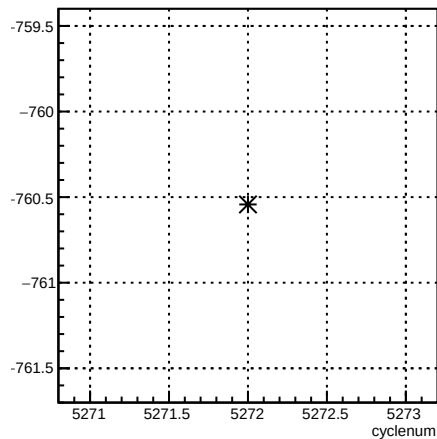
usr_coil6:cyclenum {run == 5960}
