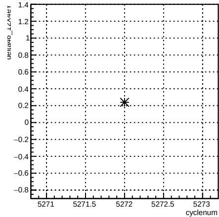
delta46_12X4eY:cyclenum {run == 5960}
