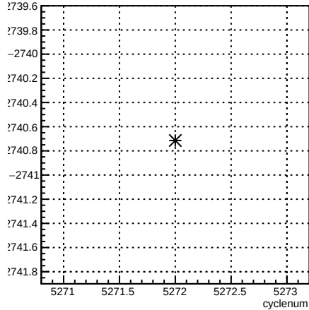
usr_coil3:cyclenum {run == 5960}
