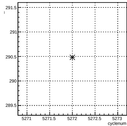
4eX_coil7:cyclenum {run == 5960}
