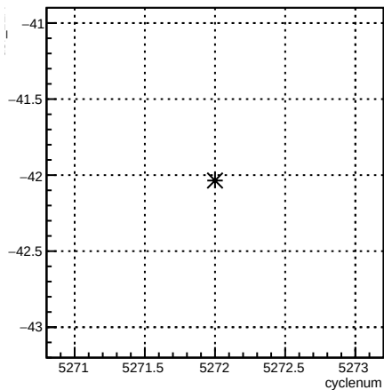
usr_12X:cyclenum {run == 5960}
