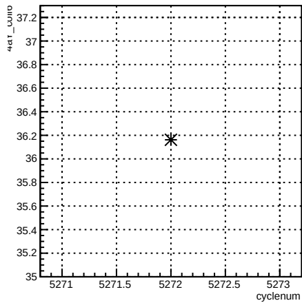
4eY_coil6:cyclenum {run == 5960}
