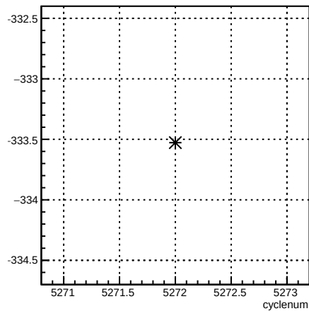
4eX_coil1:cyclenum {run == 5960}
