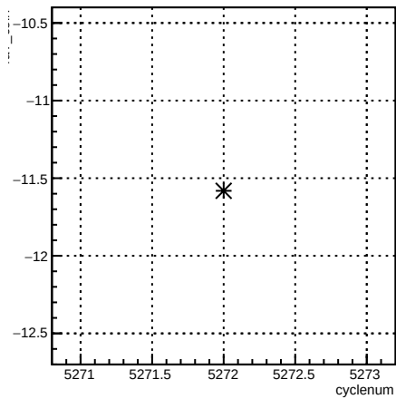
4eY_coil7:cyclenum {run == 5960}
