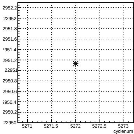
usl_coil6:cyclenum {run == 5960}
