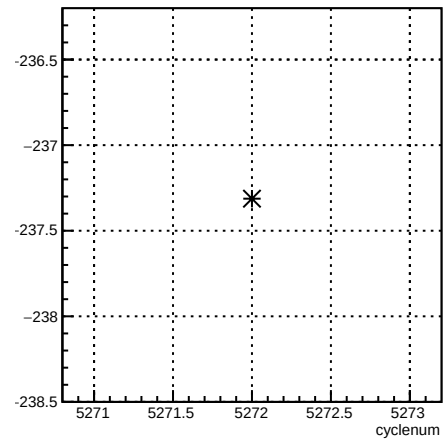
12X_coil6:cyclenum {run == 5960}
