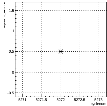
alpha13_4eX1X:cyclenum {run == 5960}
