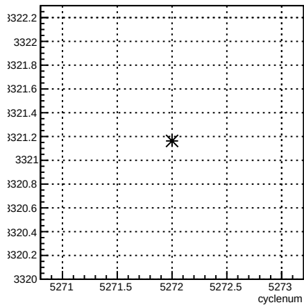
usl_coil7:cyclenum {run == 5960}
