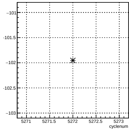
usl_4eY:cyclenum {run == 5960}
