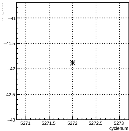
4eX_coil3:cyclenum {run == 5960}
