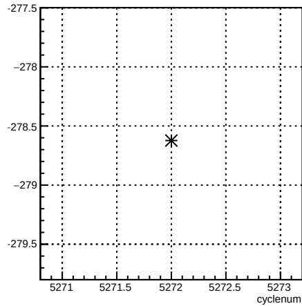
1X_coil1:cyclenum {run == 5960}
