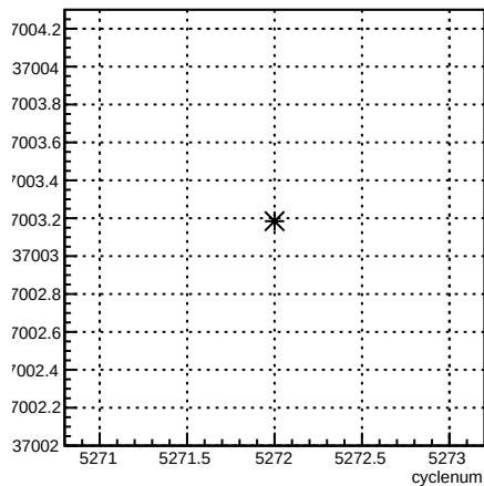
usr_coil7:cyclenum {run == 5960}
