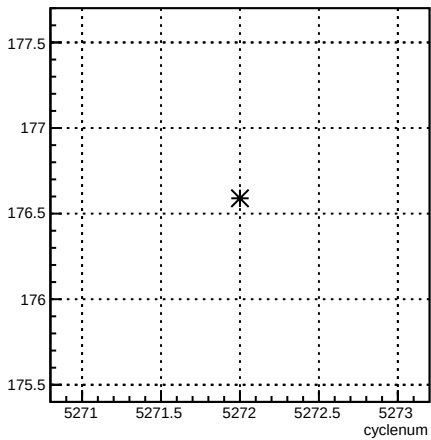
4eY_coil4:cyclenum {run == 5960}
