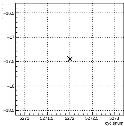
1X_coil3:cyclenum {run == 5960}
