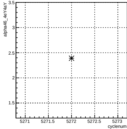
alpha46_4eY4aY:cyclenum {run == 5960}
