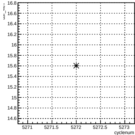
usr_4eY:cyclenum {run == 5960}
