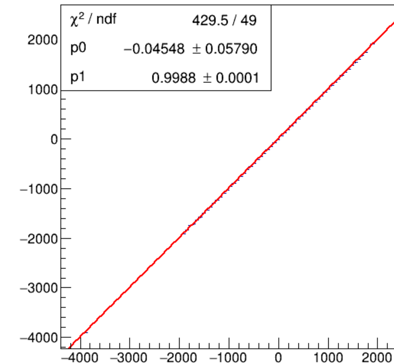
run5960_000_asym_bcm_an_ds_vs_asym_bcm_an_ds3_pr.png
