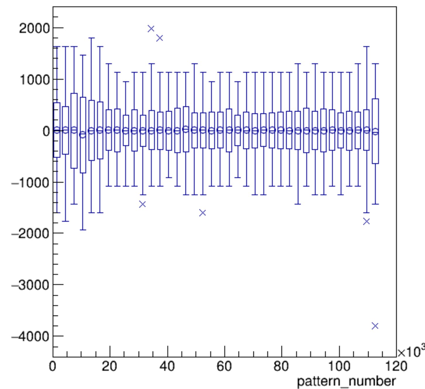
asym_bcm_an_us/ppm:pattern_number {ErrorFlag==0}
