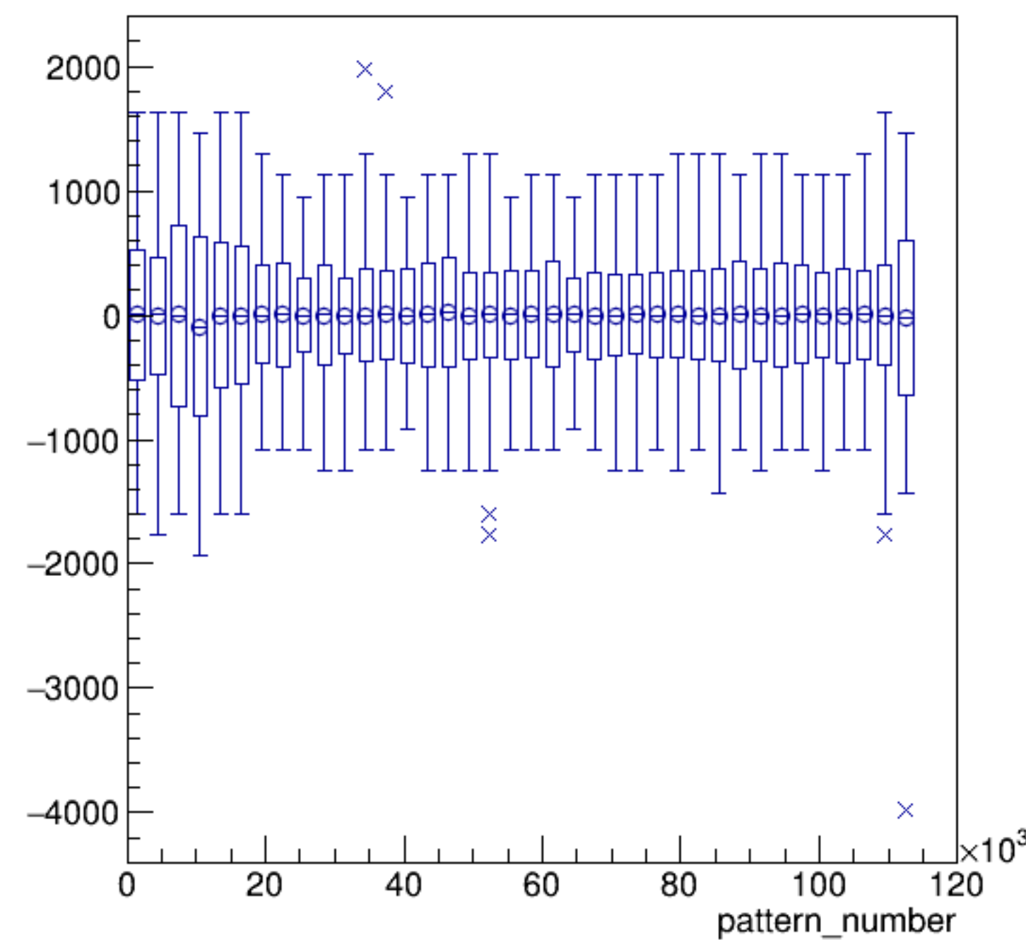
asym_bcm_an_ds/ppm:pattern_number {ErrorFlag==0}
