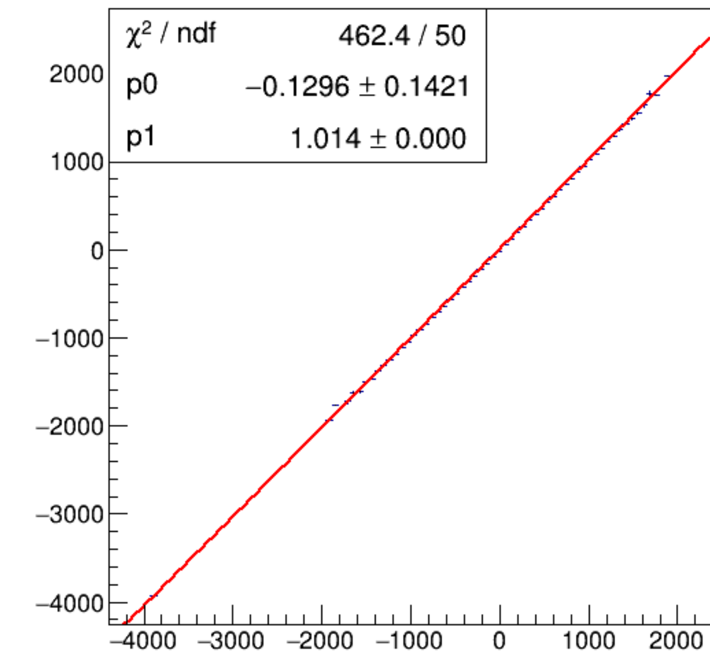
run5960_000_asym_bcm_dg_ds_vs_asym_bcm_an_us_pr.png
