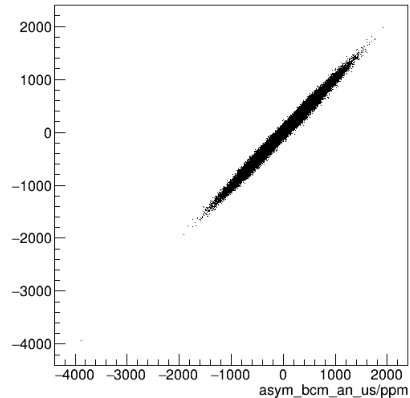
run5960_000_asym_bcm_dg_ds_vs_asym_bcm_an_us_pr.png
