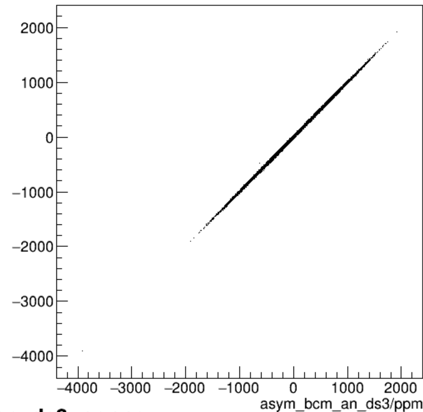
run5960_000_asym_bcm_an_ds_vs_asym_bcm_an_ds3_pr.png
