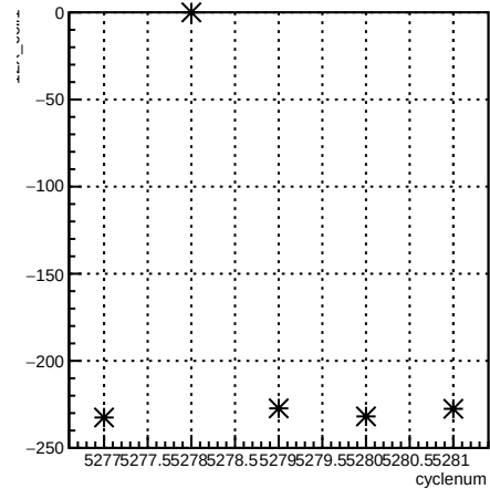
12X_coil1:cyclenum {run == 5961}
