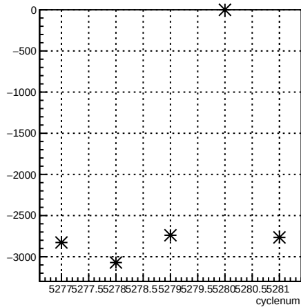
usr_coil3:cyclenum {run == 5961}
