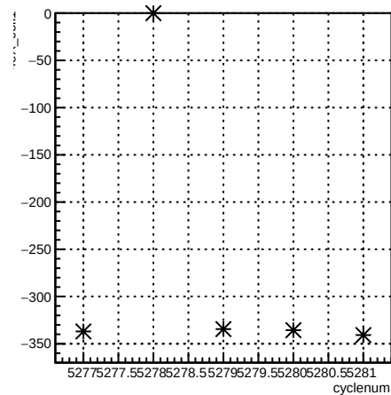
4eX_coil1:cyclenum {run == 5961}
