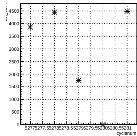
usl_coil4:cyclenum {run == 5961}
