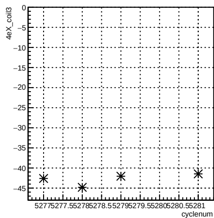
4eX_coil3:cyclenum {run == 5961}
