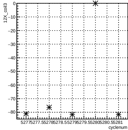
12X_coil3:cyclenum {run == 5961}
