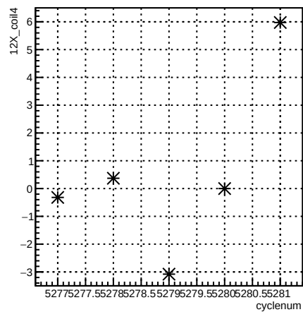
12X_coil4:cyclenum {run == 5961}
