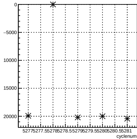
usr_coil1:cyclenum {run == 5961}
