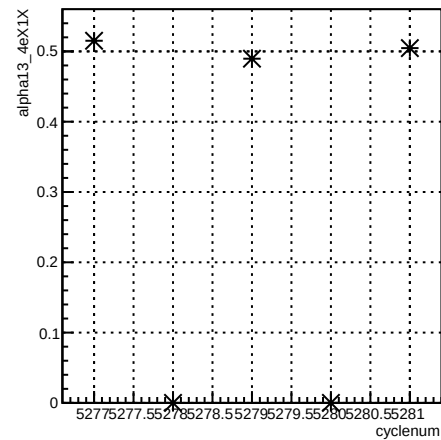
alpha13_4eX1X:cyclenum {run == 5961}
