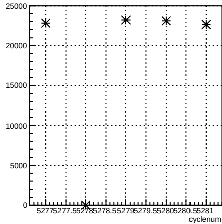
usl_coil1:cyclenum {run == 5961}
