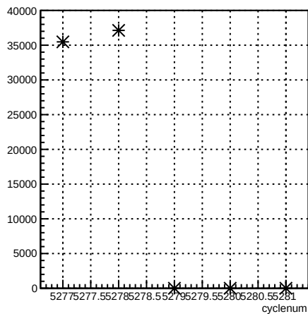
usr_coil7:cyclenum {run == 5961}
