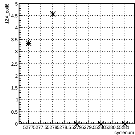
12X_coil6:cyclenum {run == 5961}
