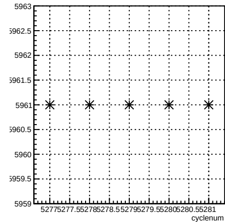
run:cyclenum {run == 5961}
