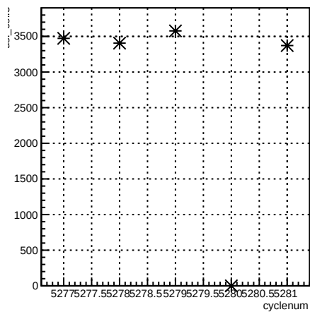
usl_coil3:cyclenum {run == 5961}
