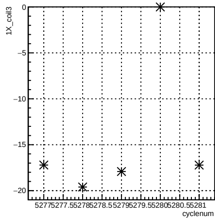
1X_coil3:cyclenum {run == 5961}
