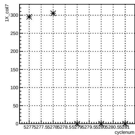
1X_coil7:cyclenum {run == 5961}
