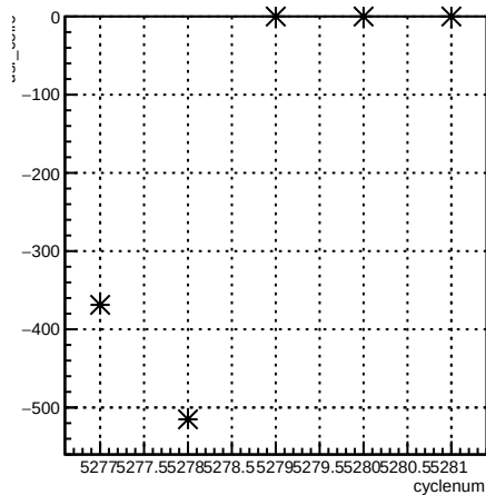
usr_coil6:cyclenum {run == 5961}
