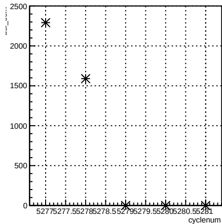
usl_coil7:cyclenum {run == 5961}
