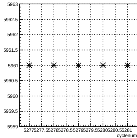
run:cyclenum {run == 5961}
