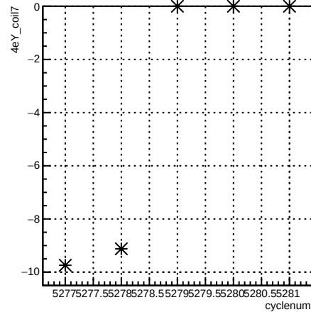
4eY_coil7:cyclenum {run == 5961}
