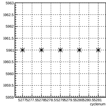
run:cyclenum {run == 5961}
