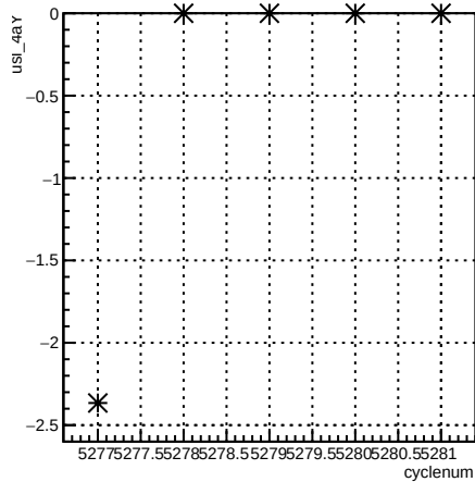
usl_4aY:cyclenum {run == 5961}
