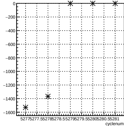
usl_coil6:cyclenum {run == 5961}
