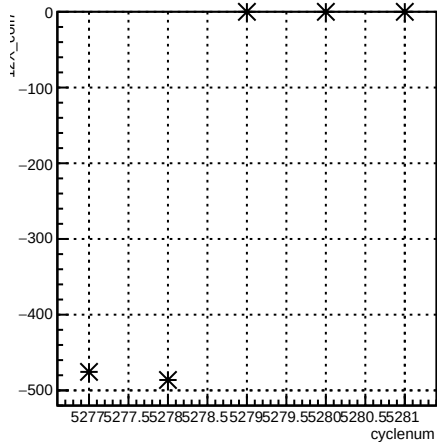
12X_coil7:cyclenum {run == 5961}
