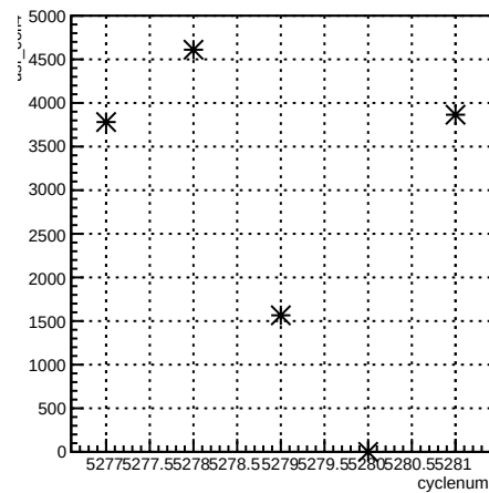
usr_coil4:cyclenum {run == 5961}
