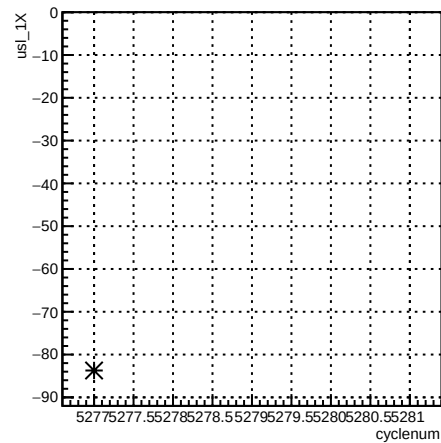
usl_1X:cyclenum {run == 5961}
