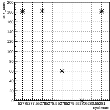
4eY_coil4:cyclenum {run == 5961}
