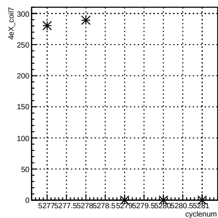
4eX_coil7:cyclenum {run == 5961}
