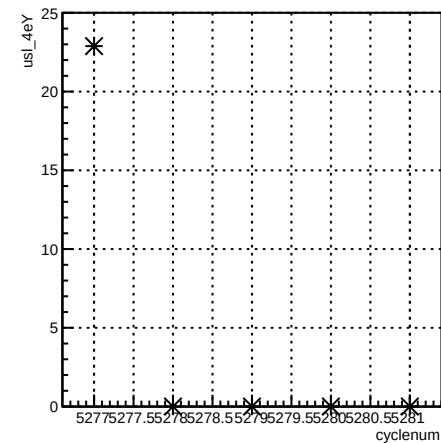
usl_4eY:cyclenum {run == 5961}
