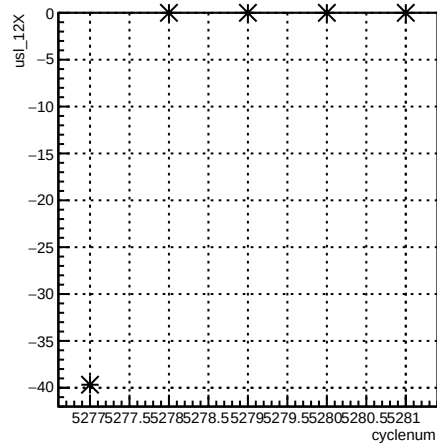
usl_12X:cyclenum {run == 5961}
