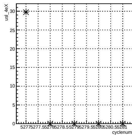
usl_4eX:cyclenum {run == 5961}
