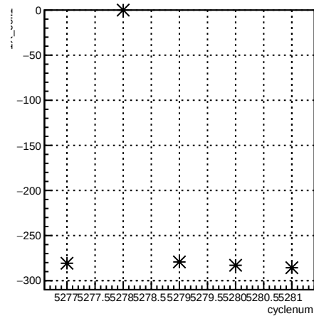
1X_coil1:cyclenum {run == 5961}
