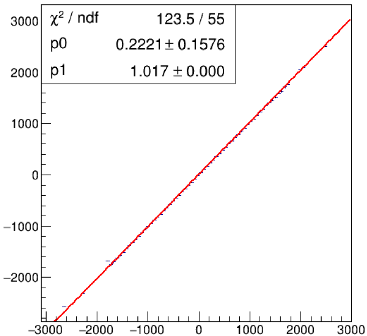
run5961_000_asym_bcm_dg_ds_vs_asym_bcm_an_us_pr.png
