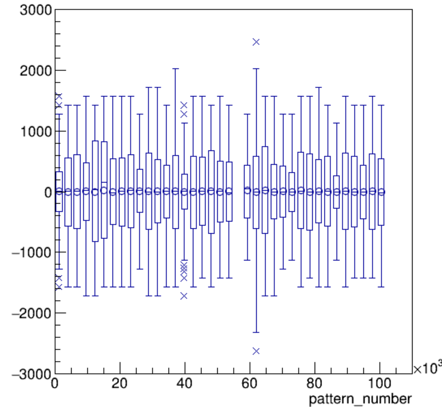
asym_bcm_an_us/ppm:pattern_number {ErrorFlag==0}
