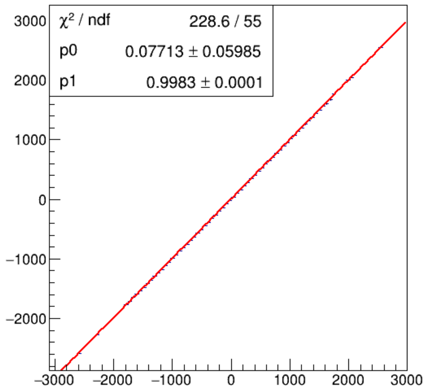
run5961_000_asym_bcm_an_ds_vs_asym_bcm_an_ds3_pr.png
