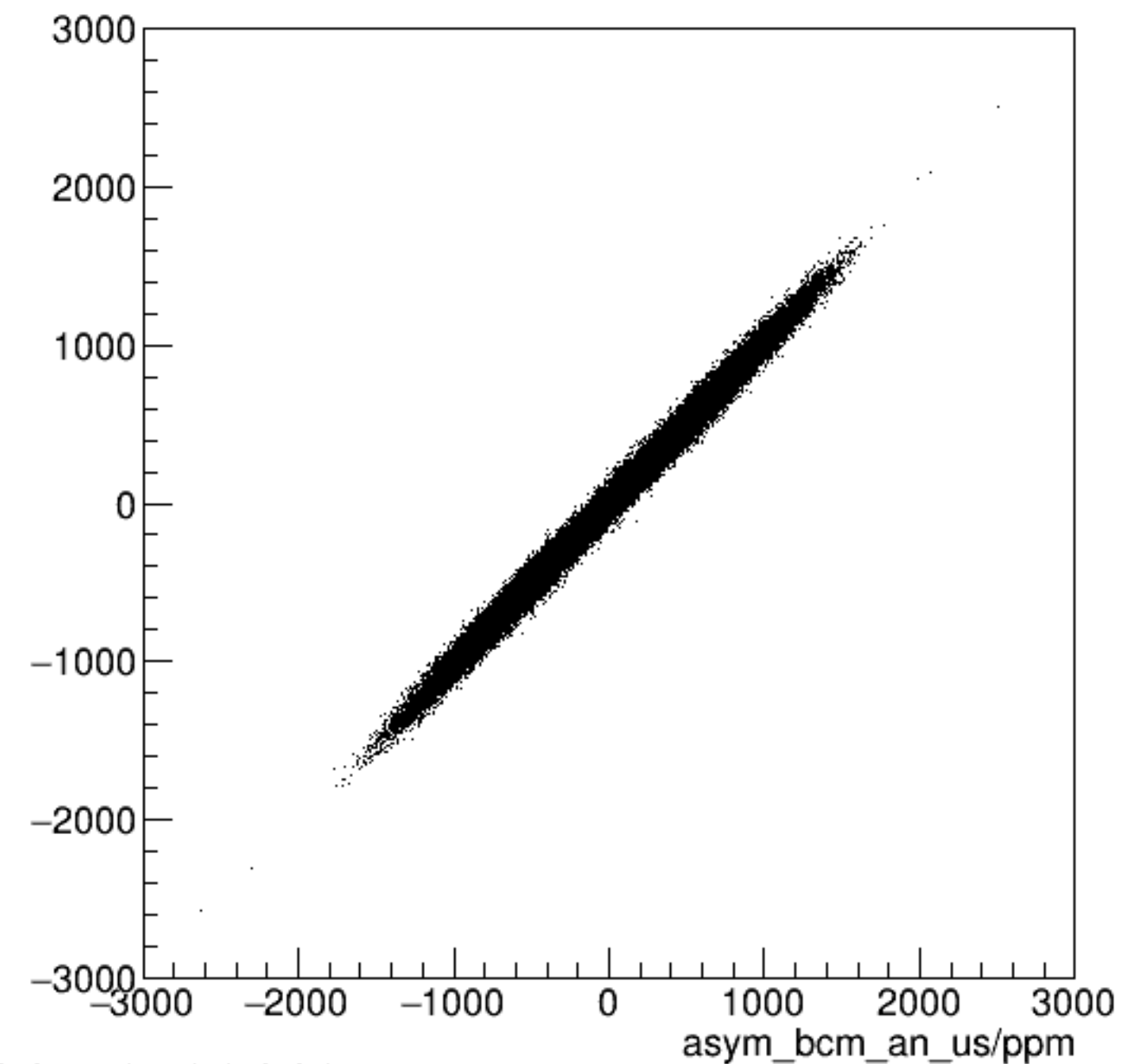
run5961_000_asym_bcm_dg_ds_vs_asym_bcm_an_us_pr.png
