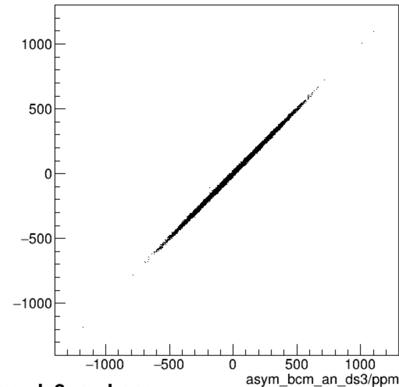
run5961_000_asym_bcm_an_ds_vs_asym_bcm_an_ds3_mul.png
