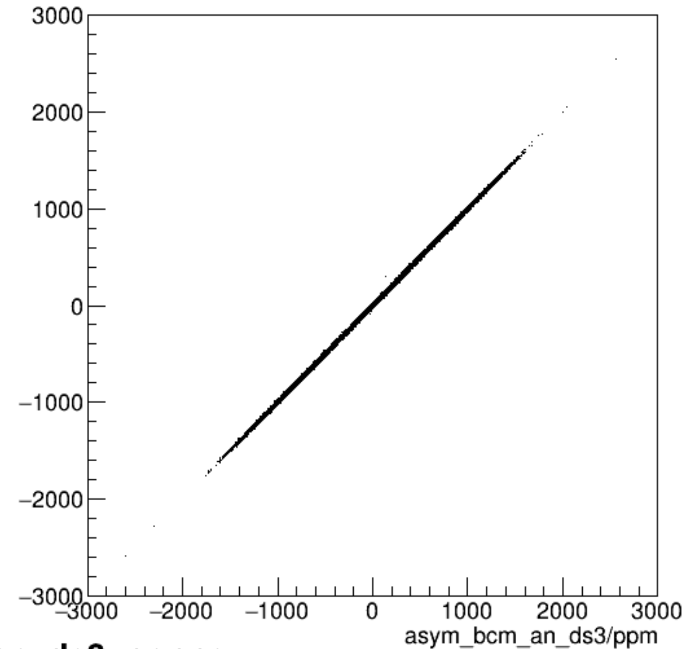
run5961_000_asym_bcm_an_ds_vs_asym_bcm_an_ds3_pr.png
