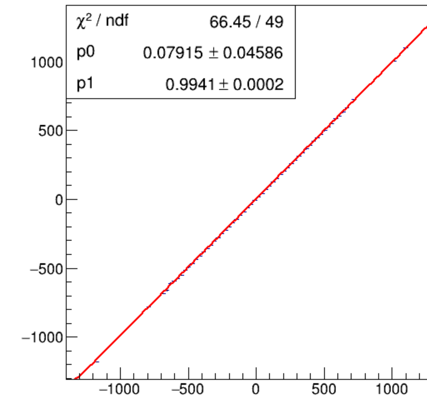
run5961_000_asym_bcm_an_ds_vs_asym_bcm_an_ds3_mul.png
