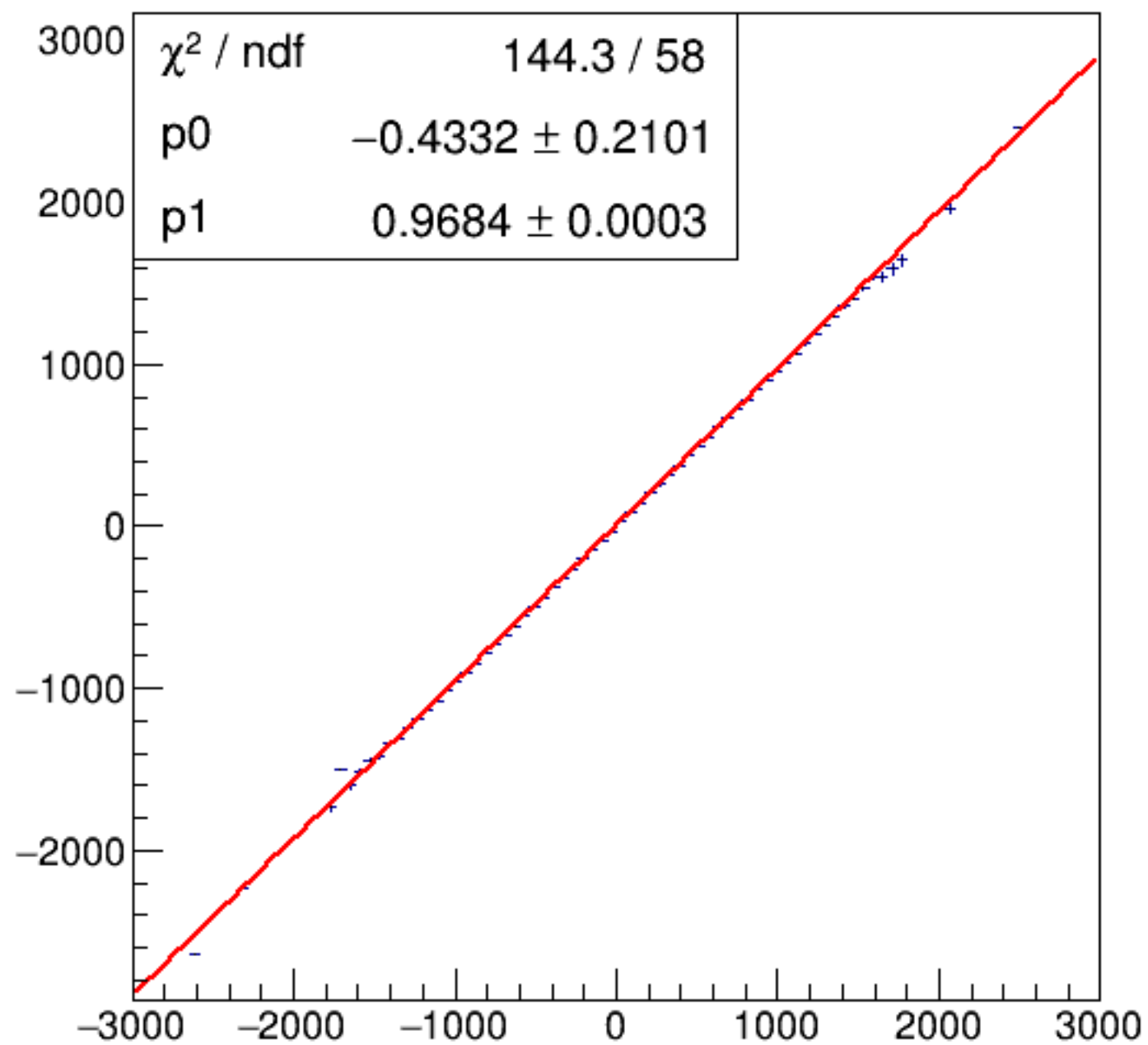
run5961_000_asym_bcm_dg_us_vs_asym_bcm_dg_ds_pr.png
