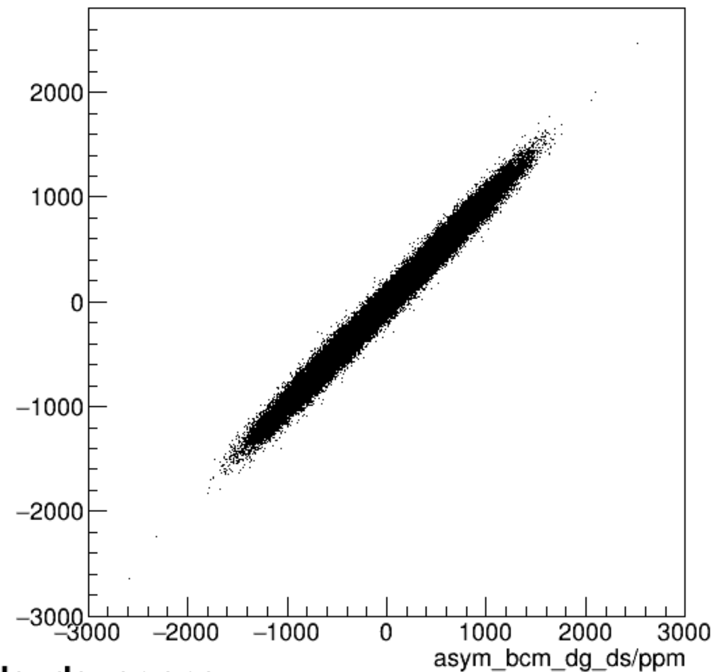
run5961_000_asym_bcm_dg_us_vs_asym_bcm_dg_ds_pr.png
