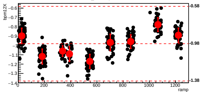
bmod_trim3,cyc=5278
