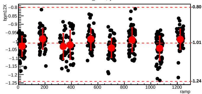
bmod_trim6,cyc=5278
