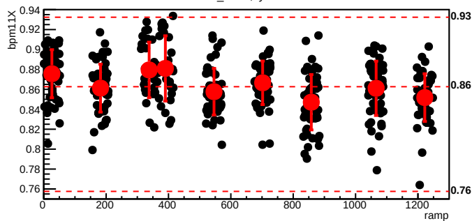
bmod_trim6,cyc=5278
