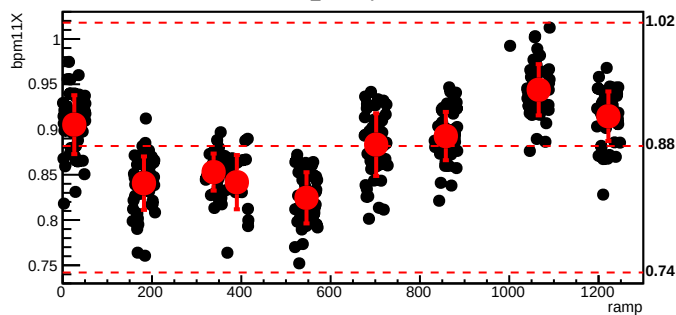
bmod_trim3,cyc=5278
